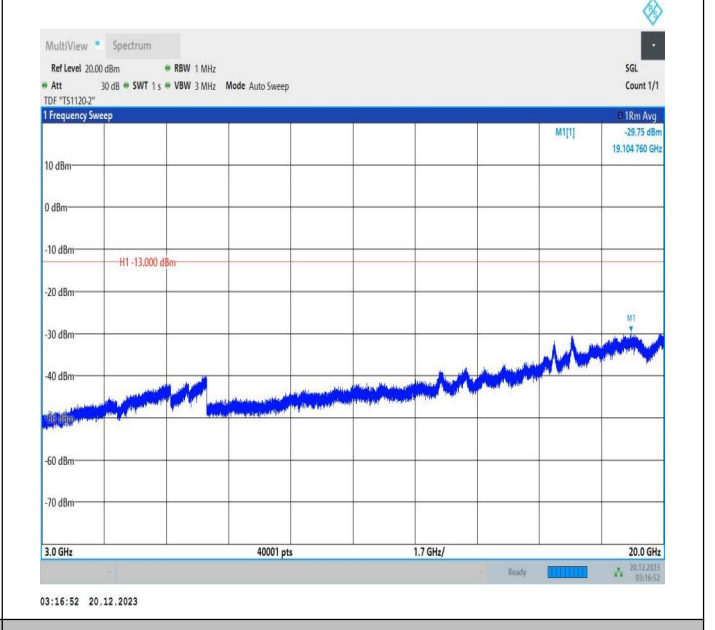
2-2-10MHz-15MHz-QPSK-QPSK-18829-18949-1RB#49-0RB# 0-3000~20000MHz-PASS
