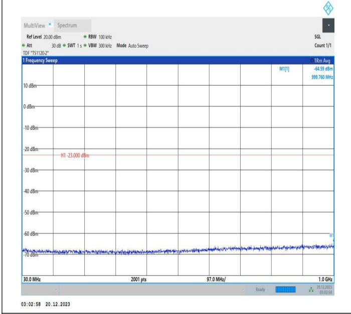
2-2-10MHz-15MHz-QPSK-QPSK-18829-18949-1RB#0-0RB#0 -30~1000MHz-PASS
