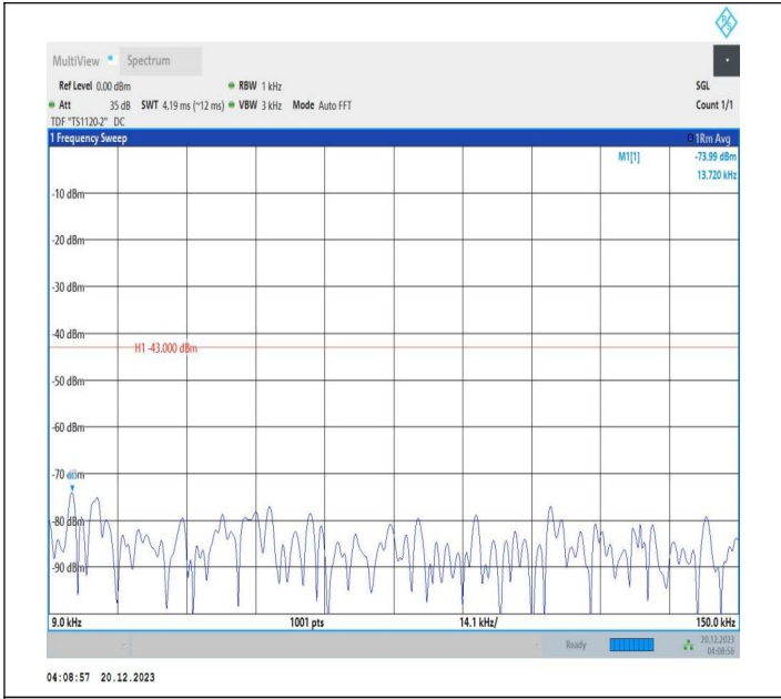
2-2-10MHz-15MHz-64QAM-64QAM-18829-18949-1RB#0-1RB #74-0.009~0.15MHz-PASS
