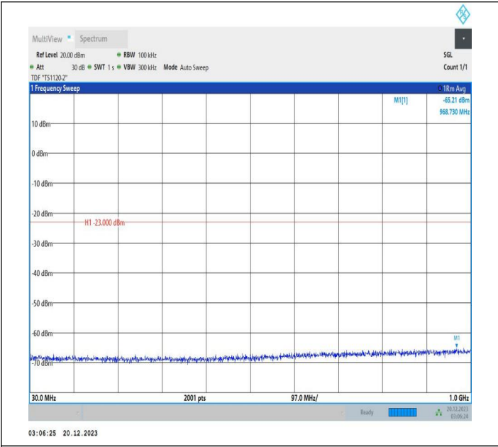
2-2-10MHz-15MHz-64QAM-64QAM-18829-18949-1RB#0-ORB #0-30~1000MHz-PASS
