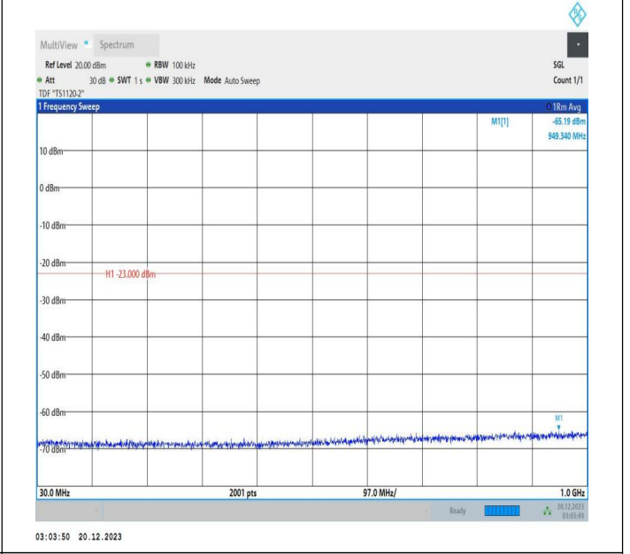
2-2-10MHz-15MHz-16QAM-16QAM-18829-18949-1RB#0-0RB #0-30~1000MHz-PASS
