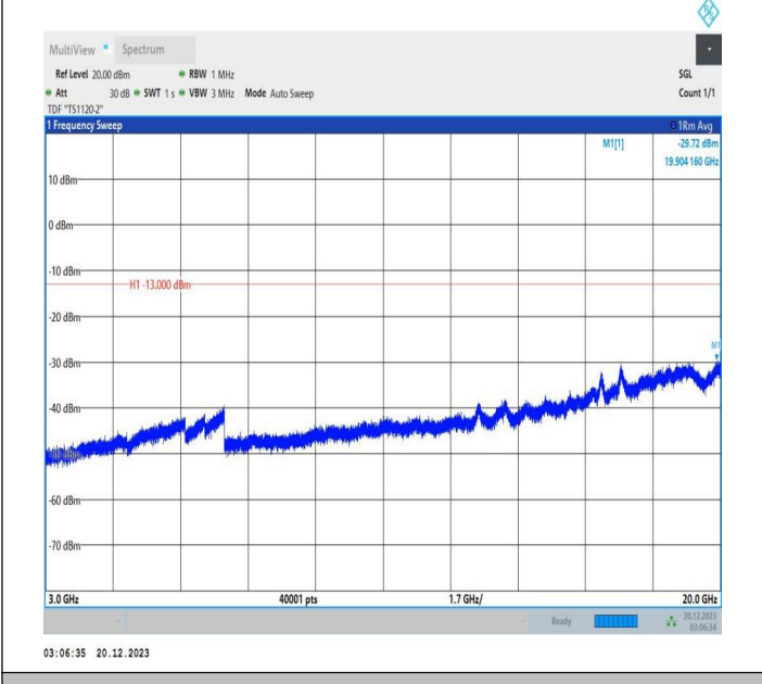
2-2-10MHz-15MHz-64QAM-64QAM-18829-18949-1RB#0-ORB #0-3000~20000MHz-PASS
