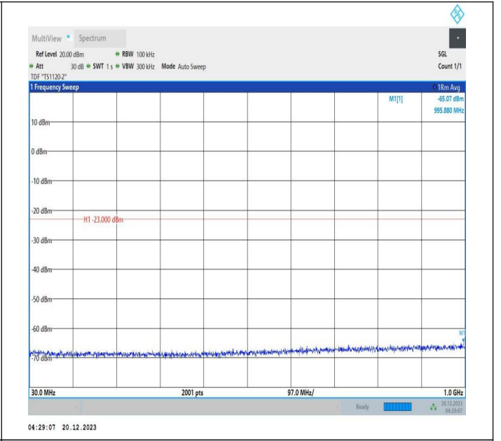
2-2-10MHz-15MHz-64QAM-64QAM-18829-18949-50RB#0-75 RB#0-30~1000MHz-PASS
