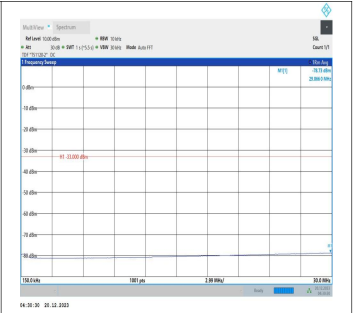
2-2-10MHz-15MHz-QPSK-QPSK-19005-19125-1RB#0-0RB#0 -0.15~30MHz-PASS
