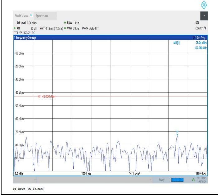
2-2-10MHz-15MHz-16QAM-16QAM-18829-18949-50RB#0-75 RB#0-0.009~0.15MHz-PASS
