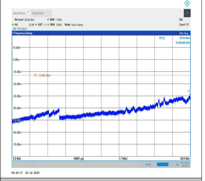
2-2-10MHz-15MHz-64QAM-64QAM-18829-18949-50RB#0-75 RB#0-3000~20000MHz-PASS
