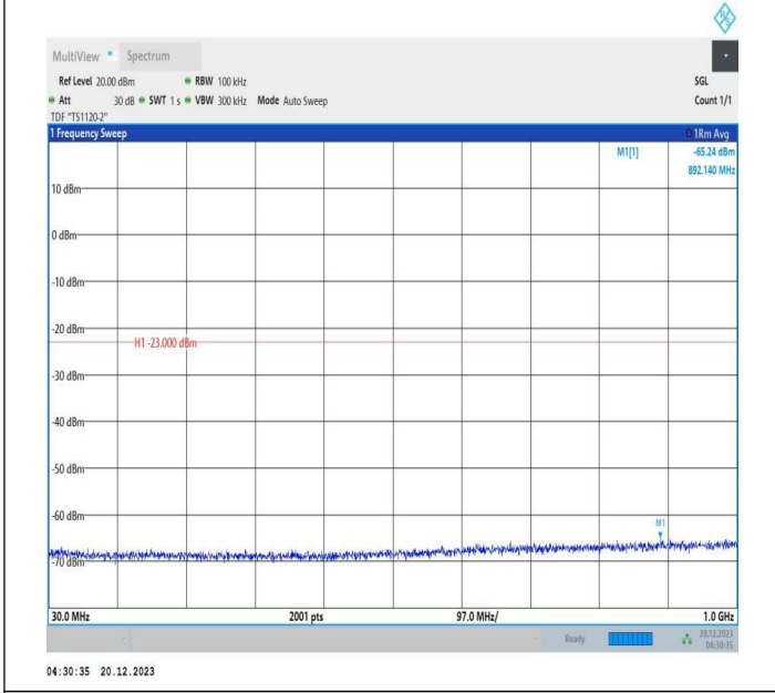
2-2-10MHz-15MHz-QPSK-QPSK-19005-19125-1RB#0-0RB#0 -30~1000MHz-PASS
