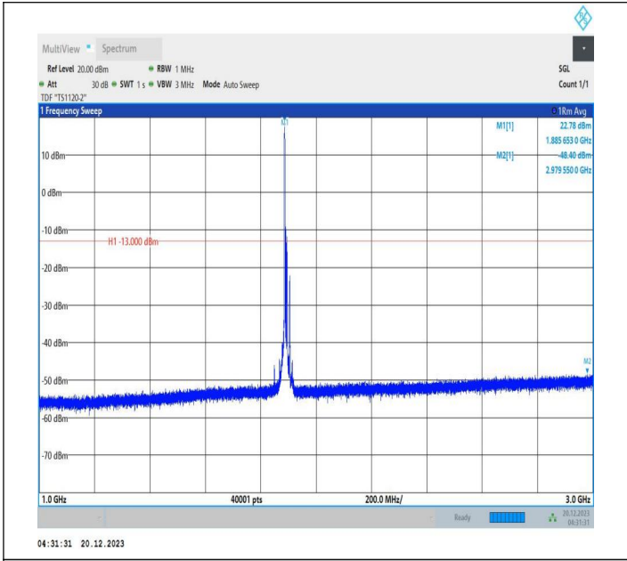
2-2-10MHz-15MHz-16QAM-16QAM-19005-19125-1RB#0-ORB #0-1000~3000MHz-PASS
