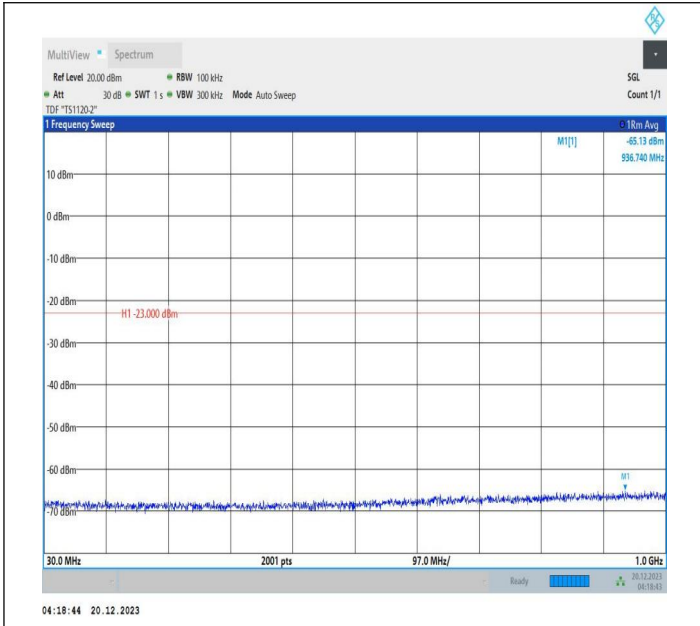
2-2-10MHz-15MHz-16QAM-16QAM-18829-18949-50RB#0-75 RB#0-30~1000MHz-PASS
