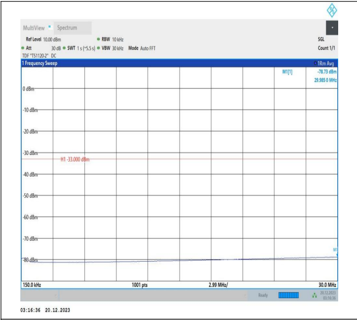
2-2-10MHz-15MHz-QPSK-QPSK-18829-18949-1RB#49-0RB# 0-0.15~30MHz-PASS
