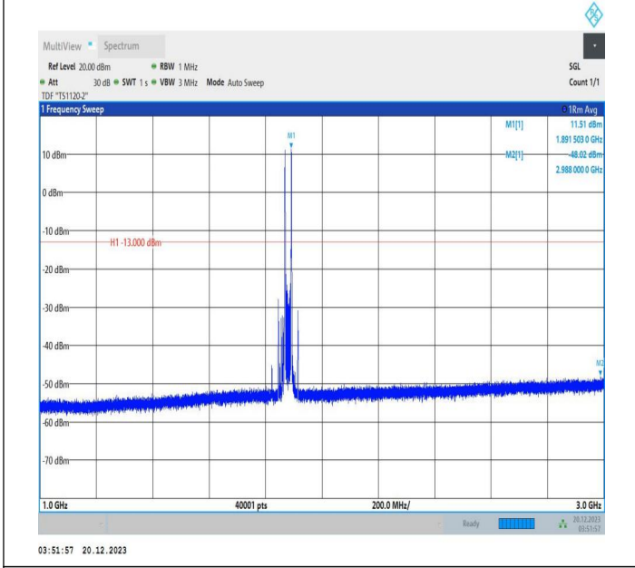
2-2-10MHz-15MHz-16QAM-16QAM-18829-18949-1RB#0-1RB #74-1000~3000MHz-PASS
