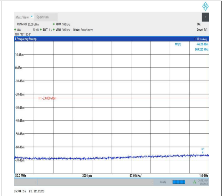
2-2-10MHz-15MHz-QPSK-QPSK-19005-19125-1RB#49-0RB# 0-30~1000MHz-PASS
