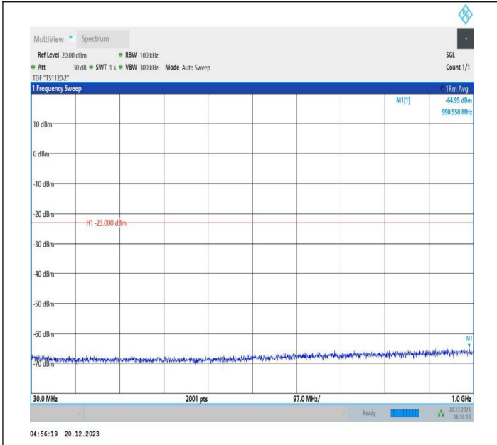
2-2-10MHz-15MHz-64QAM-64QAM-19005-19125-1RB#0-ORB #0-30~1000MHz-PASS
