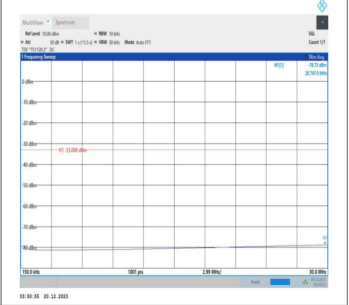
2-2-10MHz-15MHz-QPSK-QPSK-18829-18949-1RB#0-1RB#7 4-0.15~30MHz-PASS
