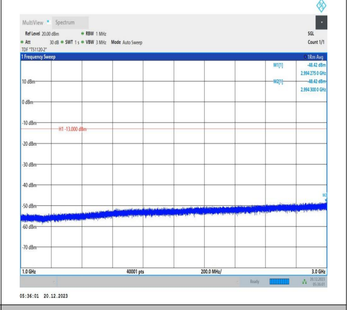
2-2-10MHz-15MHz-64QAM-64QAM-19005-19125-1RB#0-1RB #74-1000~3000MHz-PASS
