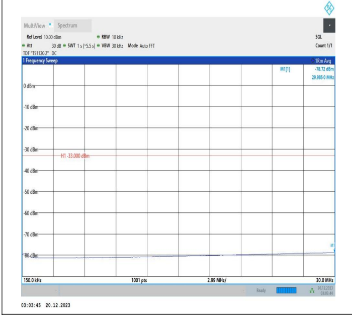
2-2-10MHz-15MHz-16QAM-16QAM-18829-18949-1RB#0-0RB #0-0.15~30MHz-PASS
