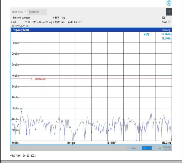
2-2-10MHz-15MHz-16QAM-16QAM-19005-19125-1RB#0-1RB #74-0.009~0.15MHz-PASS
