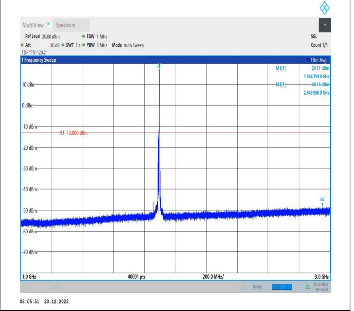
2-2-10MHz-15MHz-16QAM-16QAM-19005-19125-1RB#49-OR B#0-1000~3000MHz-PASS
