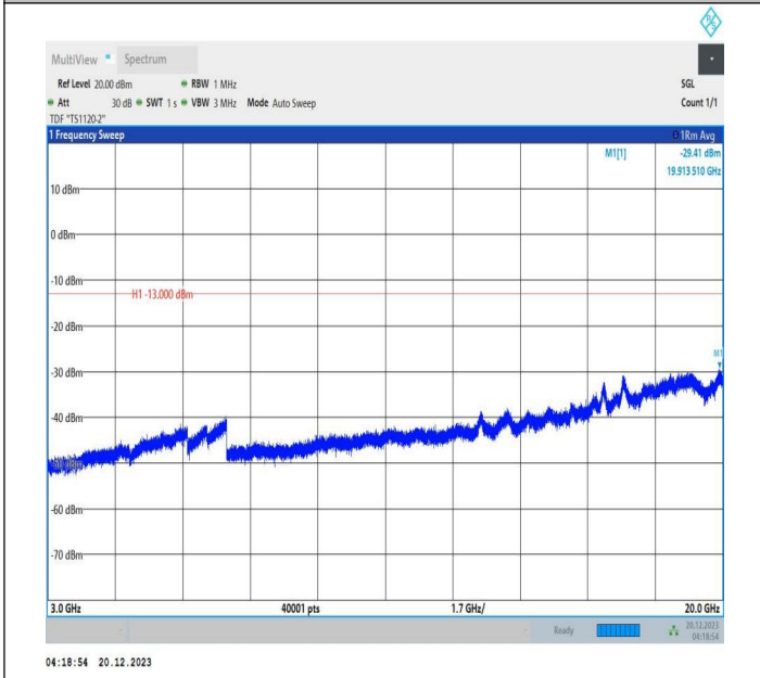
2-2-10MHz-15MHz-16QAM-16QAM-18829-18949-50RB#0-75 RB#0-3000~20000MHz-PASS
