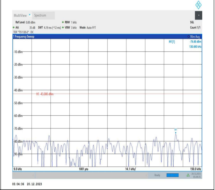
2-2-10MHz-15MHz-QPSK-QPSK-19005-19125-1RB#49-ORB# 0-0.009~0.15MHz-PASS
