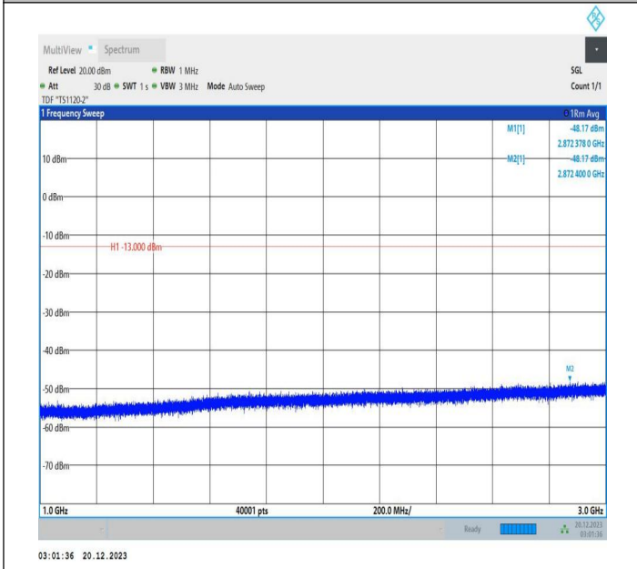
2-2-10MHz-15MHz-64QAM-64QAM-18653-18773-50RB#0-75 RB#0-1000~3000MHz-PASS
