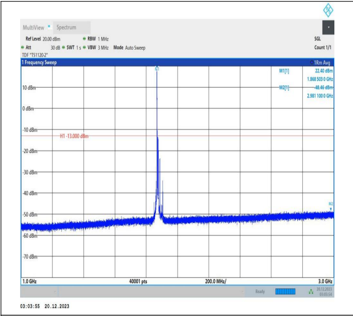
2-2-10MHz-15MHz-16QAM-16QAM-18829-18949-1RB#0-ORB #0-1000~3000MHz-PASS
