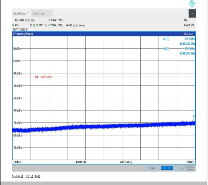
2-2-10MHz-15MHz-64QAM-64QAM-18829-18949-1RB#0-1RB #74-1000~3000MHz-PASS
