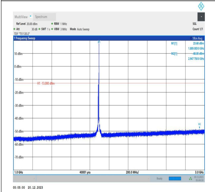
2-2-10MHz-15MHz-QPSK-QPSK-19005-19125-1RB#49-0RB# 0-1000~3000MHz-PASS
