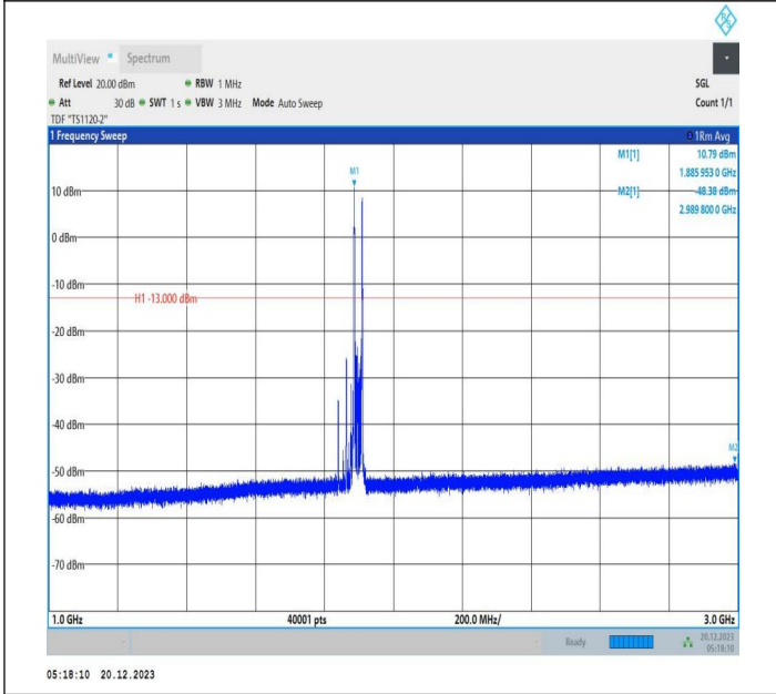
2-2-10MHz-15MHz-16QAM-16QAM-19005-19125-1RB#0-1RB #74-1000~3000MHz-PASS
