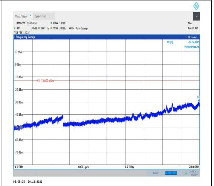
2-2-10MHz-15MHz-QPSK-QPSK-19005-19125-1RB#49-0RB# 0-3000~20000MHz-PASS
