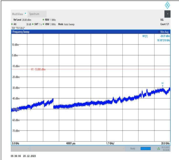
2-2-10MHz-15MHz-64QAM-64QAM-19005-19125-1RB#0-1RB #74-3000~20000MHz-PASS
