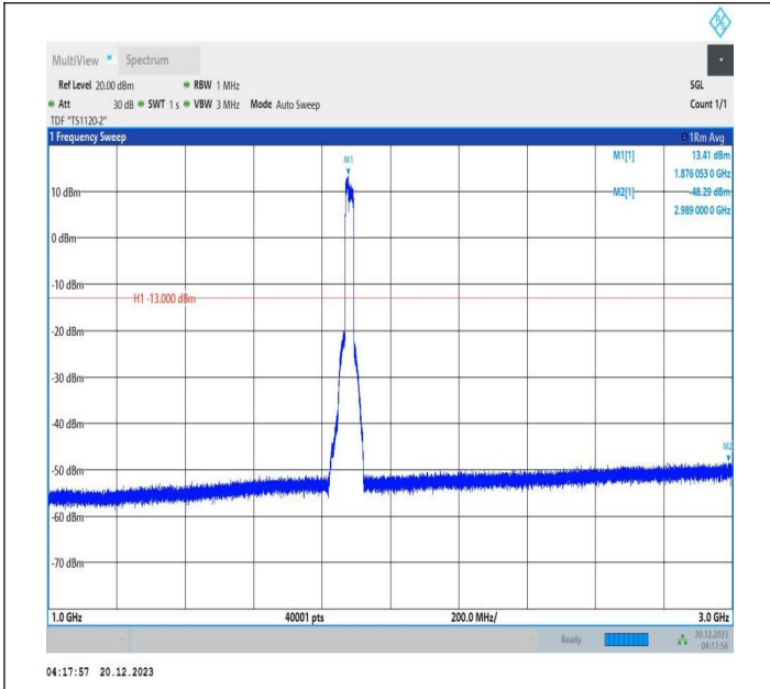
2-2-10MHz-15MHz-QPSK-QPSK-18829-18949-50RB#0-75RB #0-1000~3000MHz-PASS
