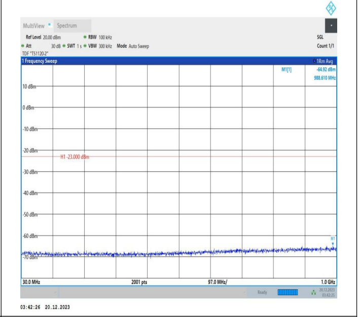
2-2-10MHz-15MHz-64QAM-64QAM-18829-18949-1RB#49-OR B#0-30~1000MHz-PASS
