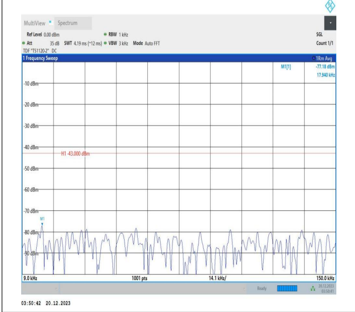
2-2-10MHz-15MHz-QPSK-QPSK-18829-18949-1RB#0-1RB#7 4-0.009~0.15MHz-PASS
