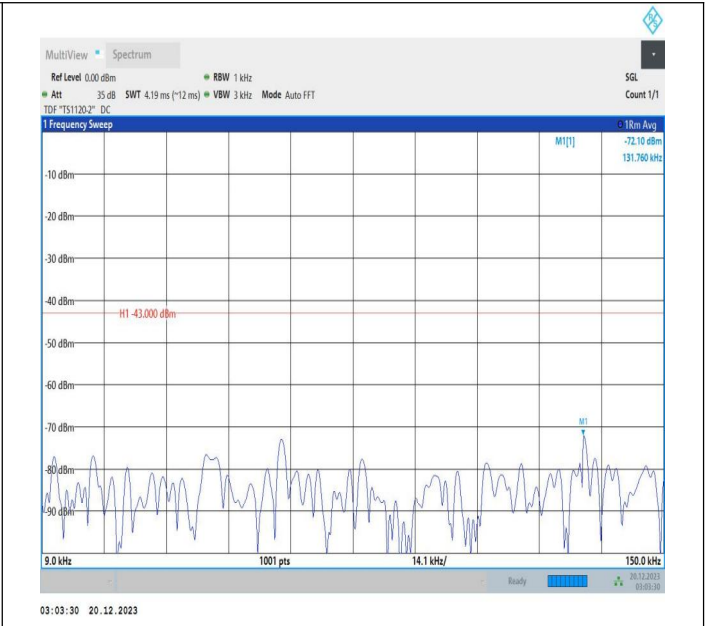
2-2-10MHz-15MHz-16QAM-16QAM-18829-18949-1RB#0-0RB #0-0.009~0.15MHz-PASS
