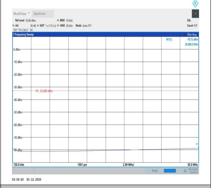
2-2-10MHz-15MHz-64QAM-64QAM-18829-18949-1RB#0-ORB #0-0.15~30MHz-PASS
