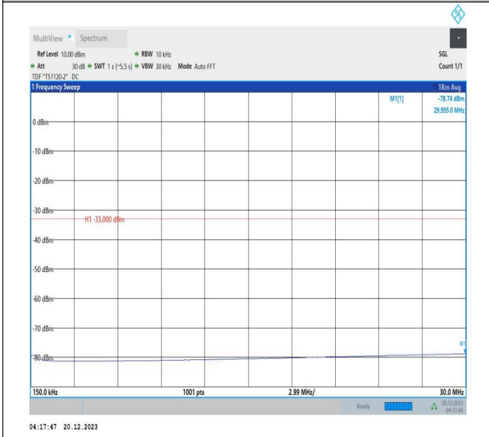
2-2-10MHz-15MHz-QPSK-QPSK-18829-18949-50RB#0-75RB #0-0.15~30MHz-PASS
