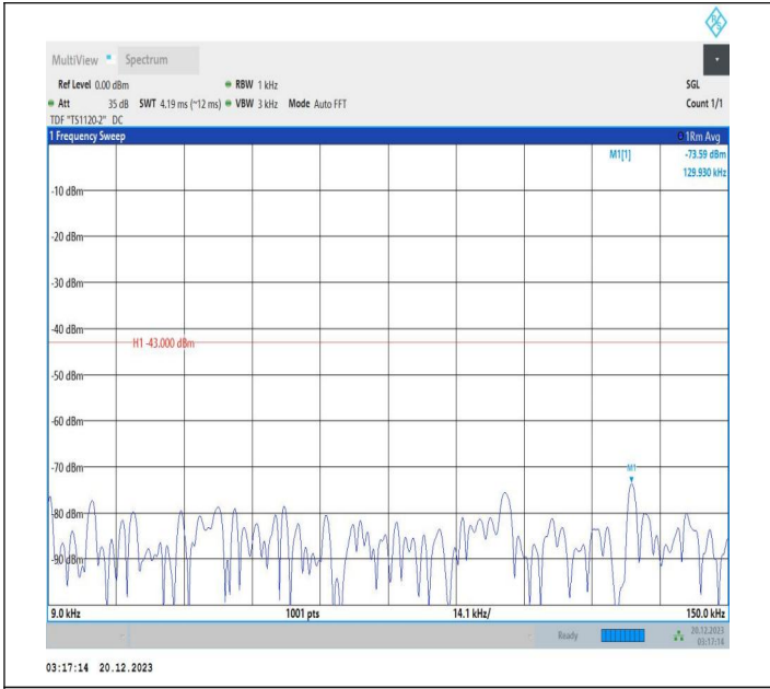
2-2-10MHz-15MHz-16QAM-16QAM-18829-18949-1RB#49-0R B#0-0.009~0.15MHz-PASS
