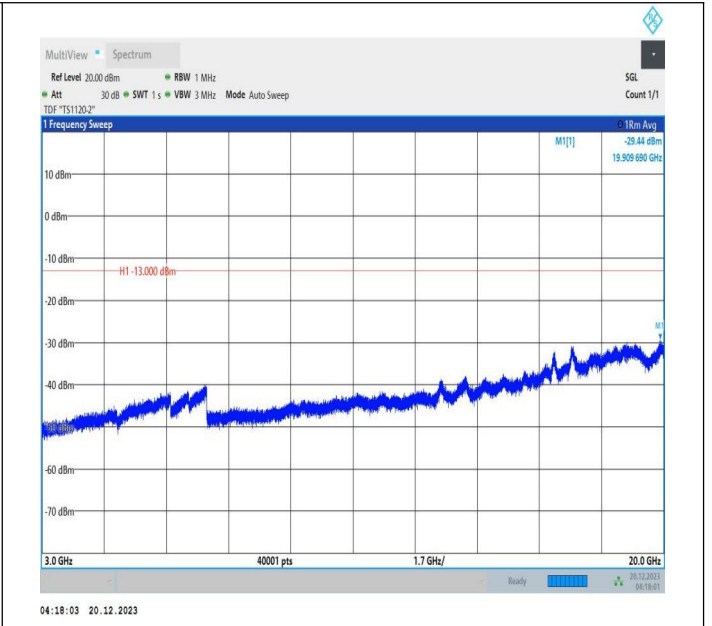
2-2-10MHz-15MHz-QPSK-QPSK-18829-18949-50RB#0-75RB #0-3000~20000MHz-PASS
