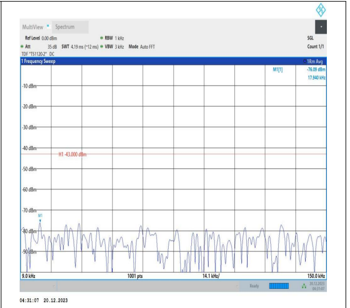
2-2-10MHz-15MHz-16QAM-16QAM-19005-19125-1RB#0-0RB #0-0.009~0.15MHz-PASS
