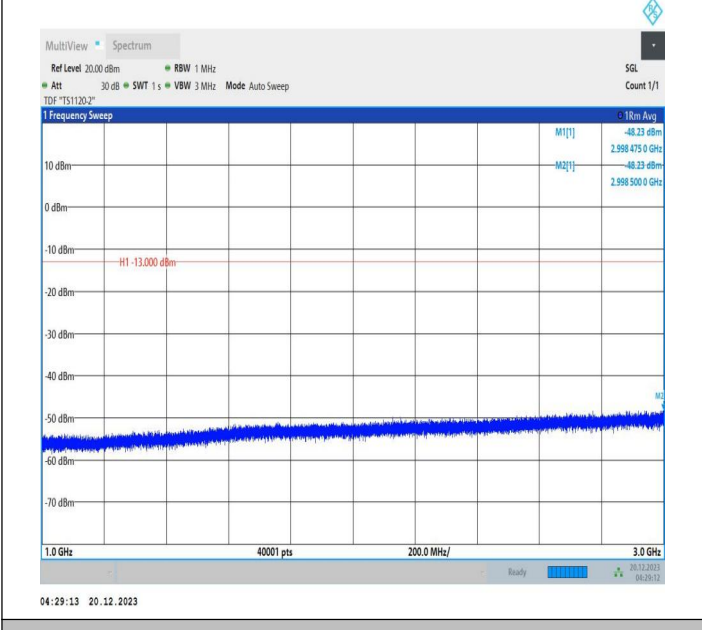
2-2-10MHz-15MHz-64QAM-64QAM-18829-18949-50RB#0-75 RB#0-1000~3000MHz-PASS
