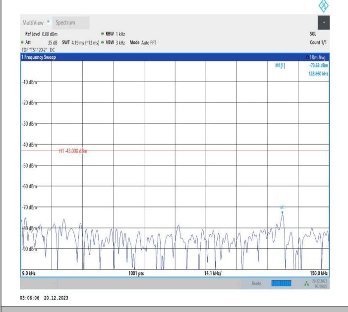
2-2-10MHz-15MHz-64QAM-64QAM-18829-18949-1RB#0-ORB #0-0.009~0.15MHz-PASS
