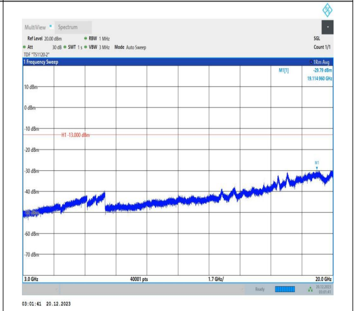
2-2-10MHz-15MHz-64QAM-64QAM-18653-18773-50RB#0-75 RB#0-3000~20000MHz-PASS
