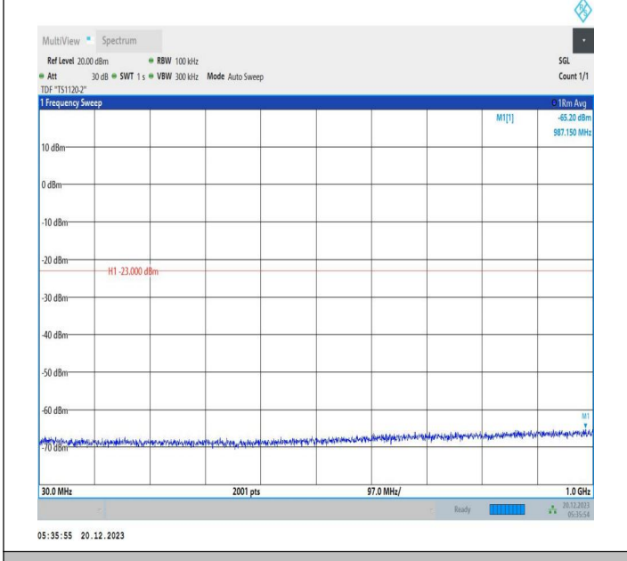
2-2-10MHz-15MHz-64QAM-64QAM-19005-19125-1RB#0-1RB #74-30~1000MHz-PASS
