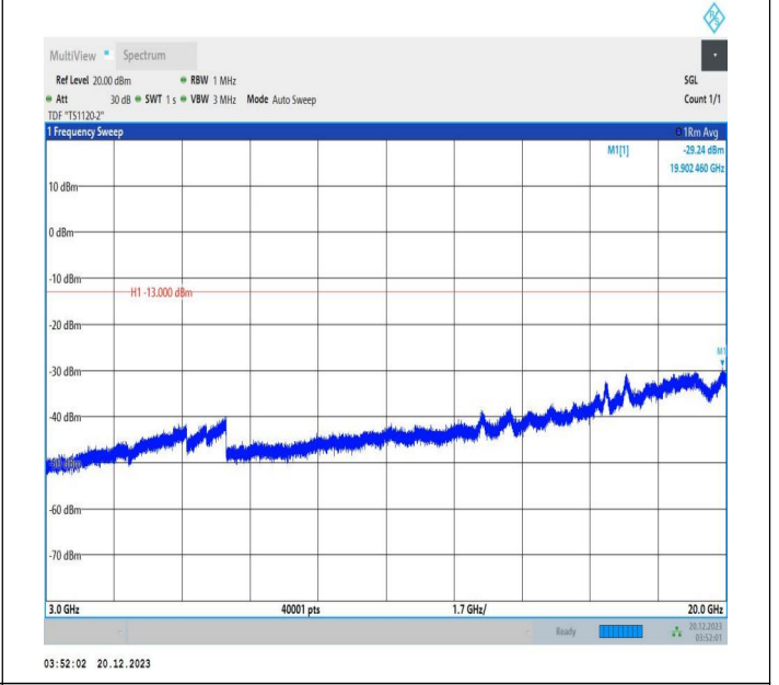
2-2-10MHz-15MHz-16QAM-16QAM-18829-18949-1RB#0-1RB #74-3000~20000MHz-PASS
