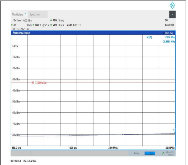
2-2-10MHz-15MHz-QPSK-QPSK-18829-18949-1RB#0-0RB#0 -0.15~30MHz-PASS
