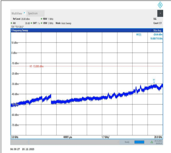
2-2-10MHz-15MHz-64QAM-64QAM-18829-18949-1RB#0-1RB #74-3000~20000MHz-PASS
