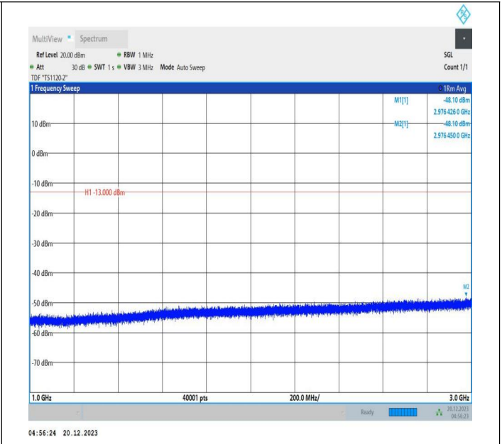
2-2-10MHz-15MHz-64QAM-64QAM-19005-19125-1RB#0-ORB #0-1000~3000MHz-PASS
