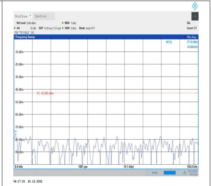
2-2-10MHz-15MHz-QPSK-QPSK-18829-18949-50RB#0-75RB #0-0.009~0.15MHz-PASS
