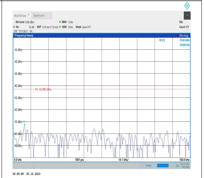
2-2-10MHz-15MHz-64QAM-64QAM-18829-18949-50RB#0-75 RB#0-0.009~0.15MHz-PASS
