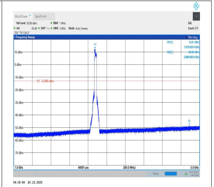
2-2-10MHz-15MHz-16QAM-16QAM-18829-18949-50RB#0-75 RB#0-1000~3000MHz-PASS
