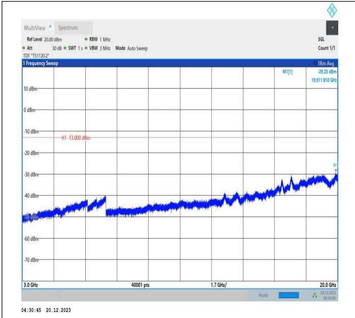
2-2-10MHz-15MHz-QPSK-QPSK-19005-19125-1RB#0-0RB#0 -3000~20000MHz-PASS
