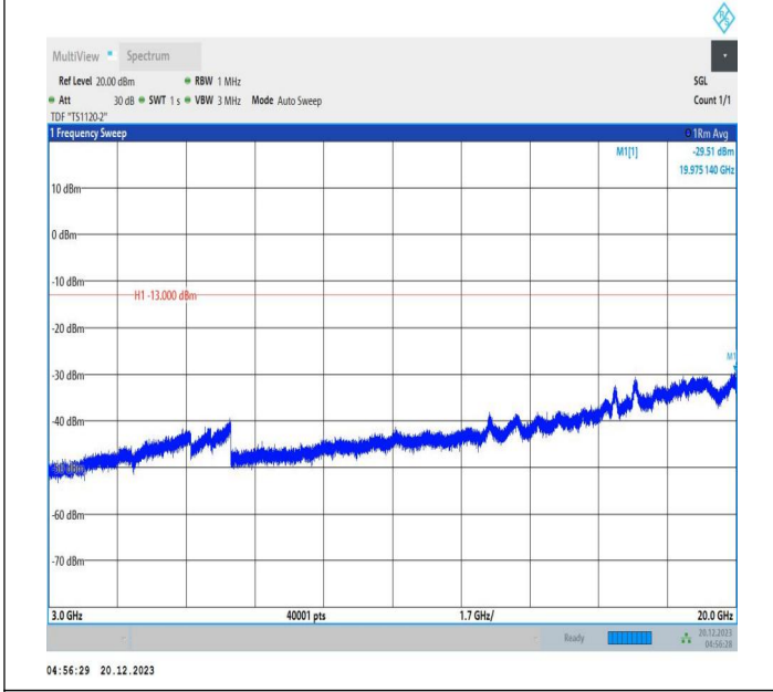
2-2-10MHz-15MHz-64QAM-64QAM-19005-19125-1RB#0-ORB #0-3000~20000MHz-PASS
