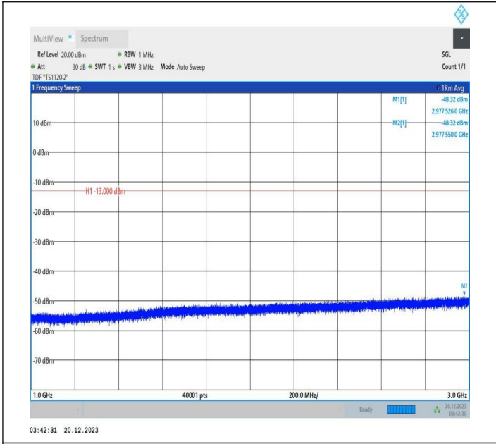
2-2-10MHz-15MHz-64QAM-64QAM-18829-18949-1RB#49-0R B#0-1000~3000MHz-PASS
