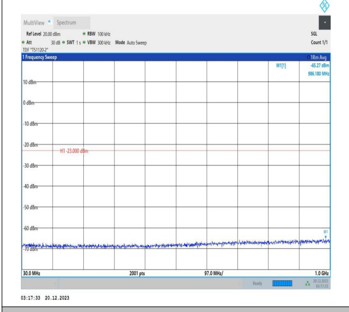
2-2-10MHz-15MHz-16QAM-16QAM-18829-18949-1RB#49-0R B#0-30~1000MHz-PASS
