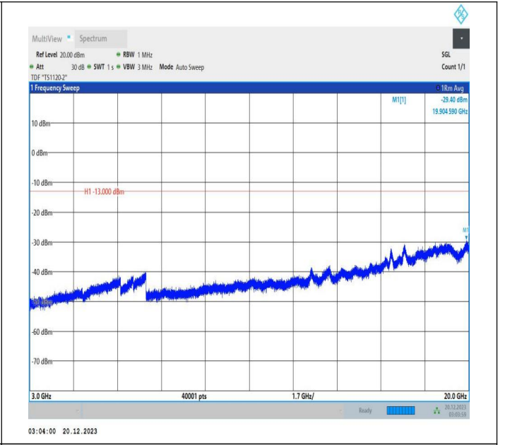
2-2-10MHz-15MHz-16QAM-16QAM-18829-18949-1RB#0-ORB #0-3000~20000MHz-PASS
