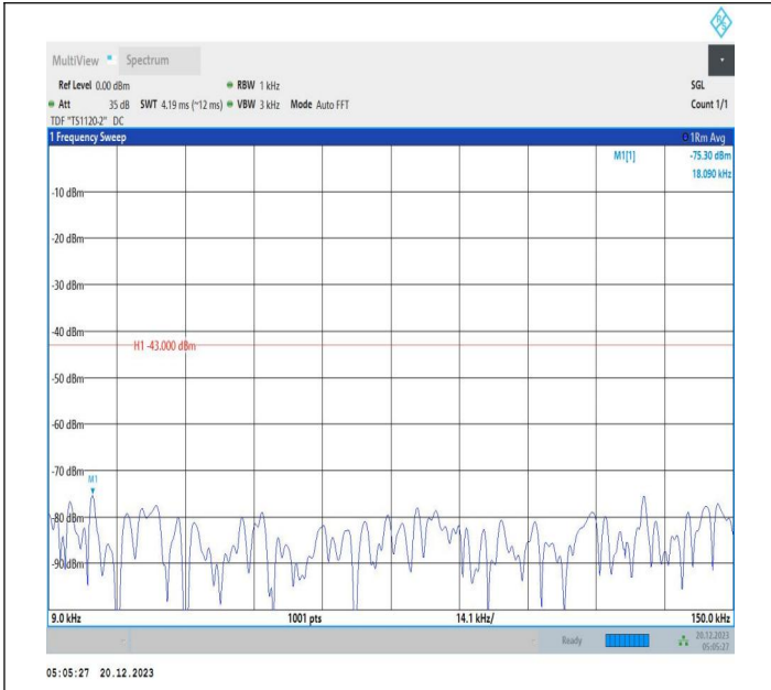
2-2-10MHz-15MHz-16QAM-16QAM-19005-19125-1RB#49-OR B#0-0.009~0.15MHz-PASS
