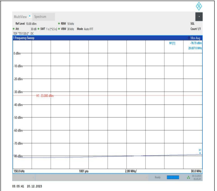
2-2-10MHz-15MHz-16QAM-16QAM-19005-19125-1RB#49-OR B#0-0.15~30MHz-PASS
