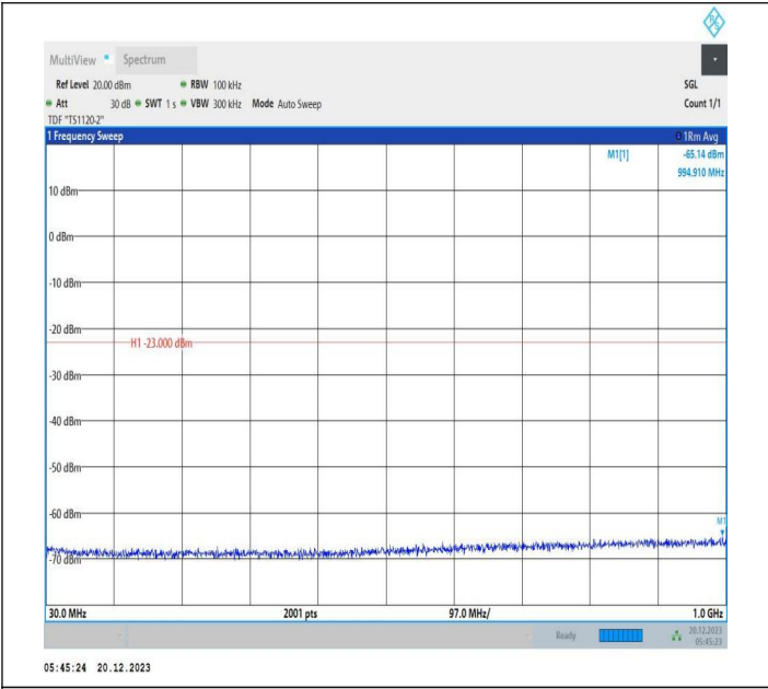
2-2-10MHz-15MHz-16QAM-16QAM-19005-19125-50RB#0-75 RB#0-30~1000MHz-PASS
