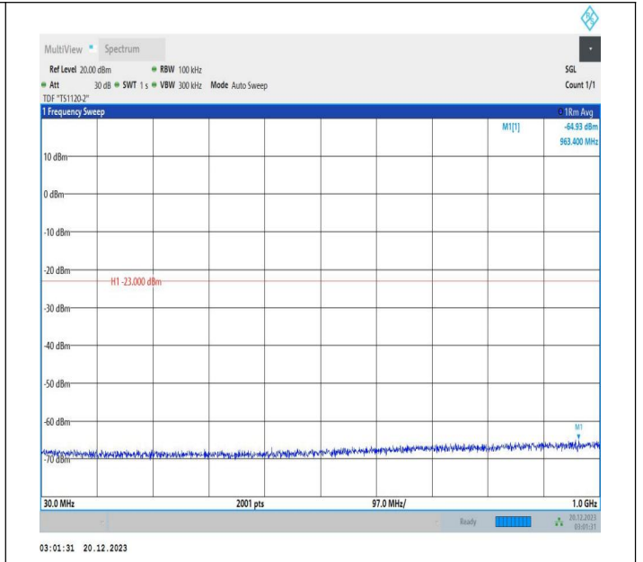
2-2-10MHz-15MHz-64QAM-64QAM-18653-18773-50RB#0-75 RB#0-30~1000MHz-PASS
