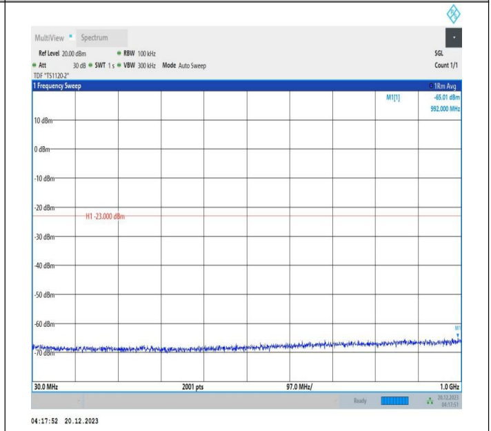
2-2-10MHz-15MHz-QPSK-QPSK-18829-18949-50RB#0-75RB #0-30~1000MHz-PASS
