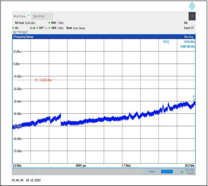
2-2-10MHz-15MHz-64QAM-64QAM-18829-18949-1RB#49-0R B#0-3000~20000MHz-PASS
