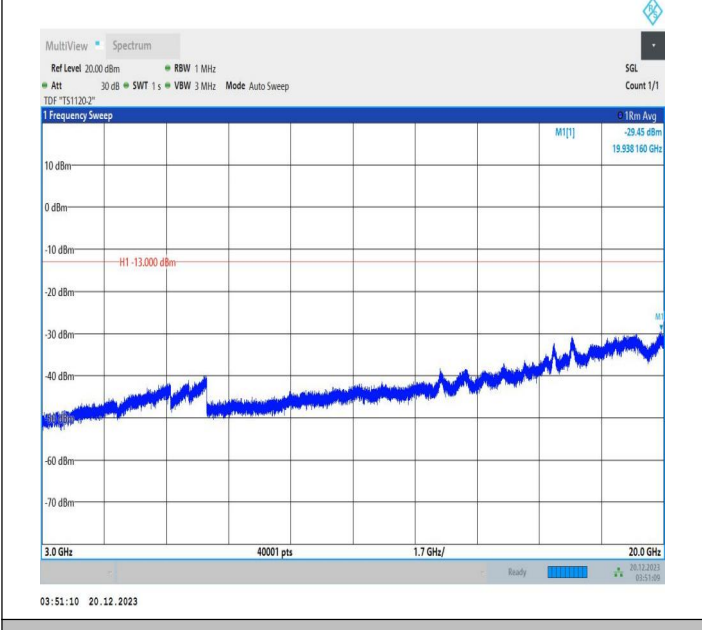
2-2-10MHz-15MHz-QPSK-QPSK-18829-18949-1RB#0-1RB#7 4-3000~20000MHz-PASS
