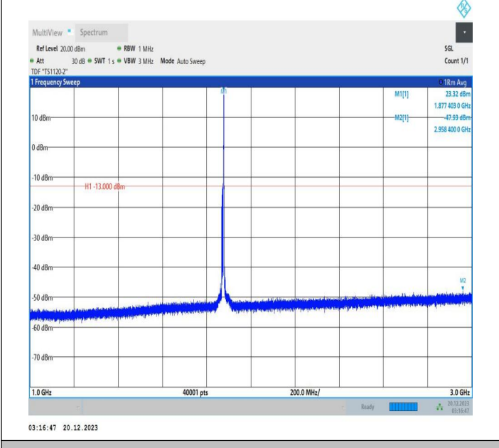
2-2-10MHz-15MHz-QPSK-QPSK-18829-18949-1RB#49-0RB# 0-1000~3000MHz-PASS
