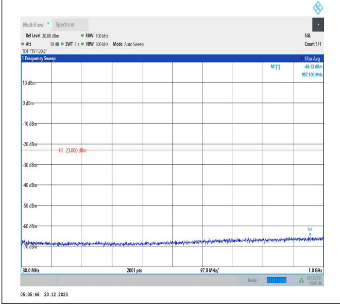
2-2-10MHz-15MHz-16QAM-16QAM-19005-19125-1RB#49-OR B#0-30~1000MHz-PASS
