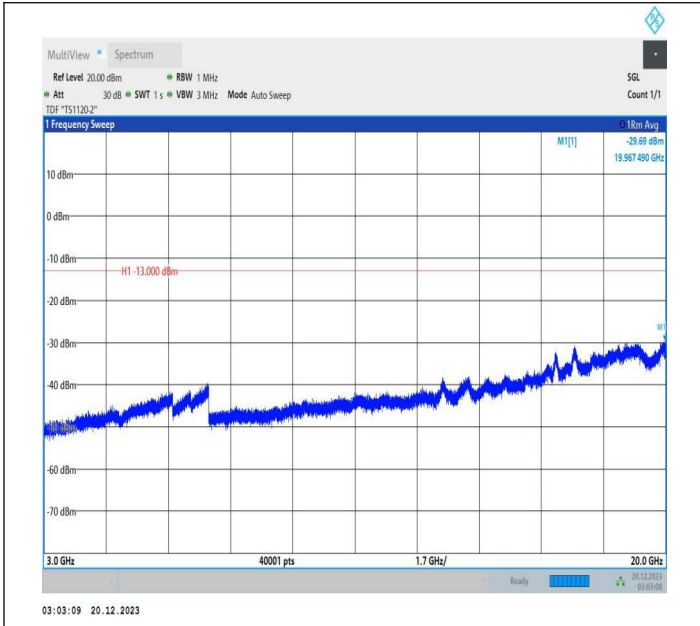
2-2-10MHz-15MHz-QPSK-QPSK-18829-18949-1RB#0-0RB#0 -3000~20000MHz-PASS
