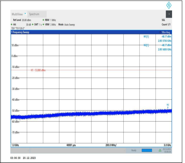
2-2-10MHz-15MHz-64QAM-64QAM-18829-18949-1RB#0-ORB #0-1000~3000MHz-PASS
