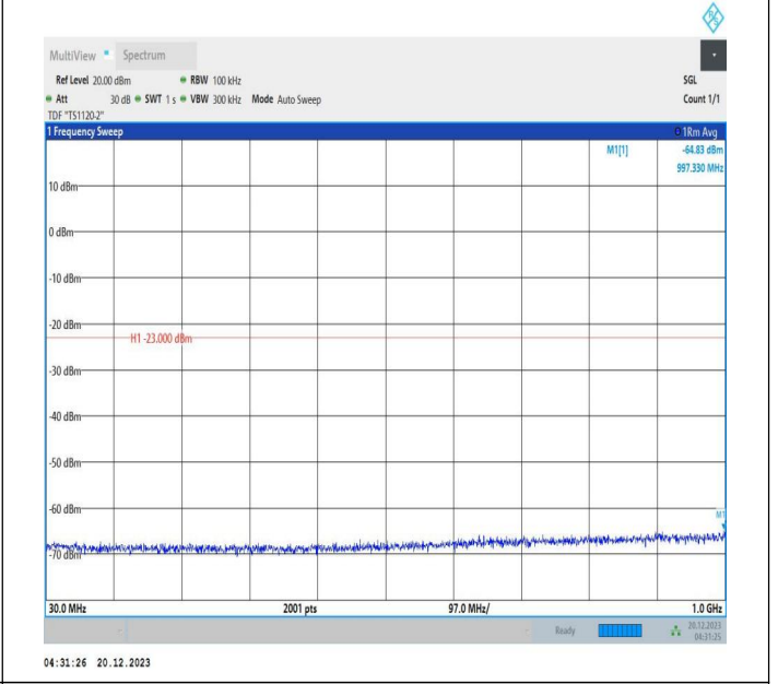
2-2-10MHz-15MHz-16QAM-16QAM-19005-19125-1RB#0-0RB #0-30~1000MHz-PASS
