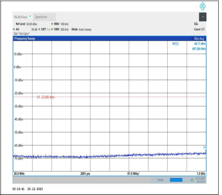
2-2-10MHz-15MHz-QPSK-QPSK-18829-18949-1RB#49-0RB# 0-30~1000MHz-PASS
