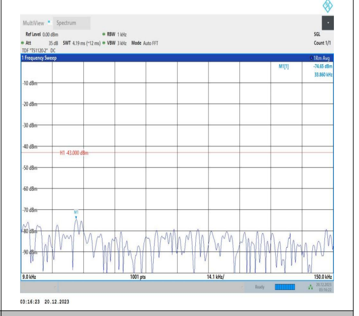
2-2-10MHz-15MHz-QPSK-QPSK-18829-18949-1RB#49-ORB# 0-0.009~0.15MHz-PASS
