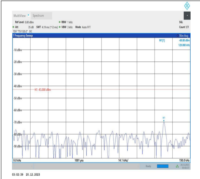
2-2-10MHz-15MHz-QPSK-QPSK-18829-18949-1RB#0-0RB#0 -0.009~0.15MHz-PASS
