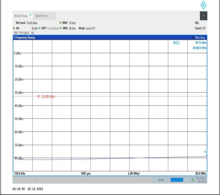
2-2-10MHz-15MHz-16QAM-16QAM-18829-18949-50RB#0-75 RB#0-0.15~30MHz-PASS
