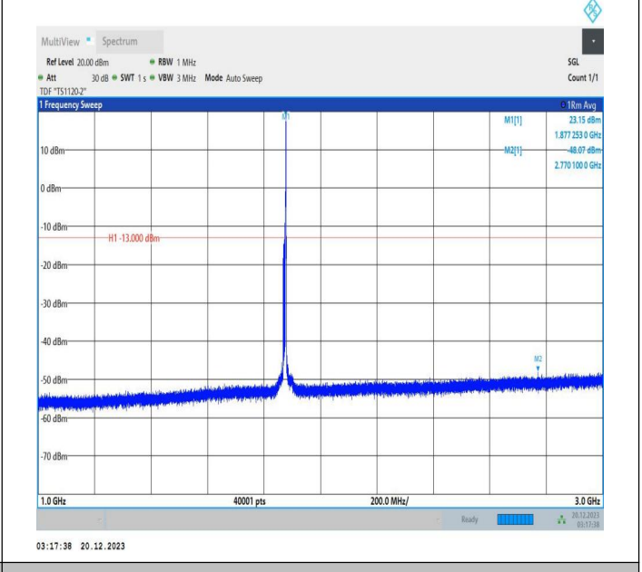
2-2-10MHz-15MHz-16QAM-16QAM-18829-18949-1RB#49-0R B#0-1000~3000MHz-PASS
