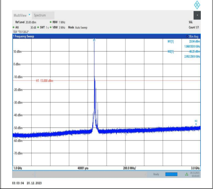
2-2-10MHz-15MHz-QPSK-QPSK-18829-18949-1RB#0-0RB#0 -1000~3000MHz-PASS
