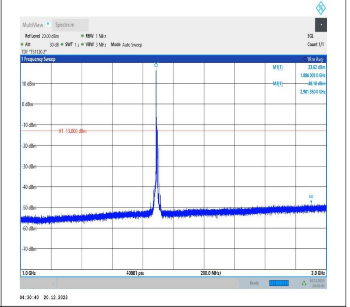
2-2-10MHz-15MHz-QPSK-QPSK-19005-19125-1RB#0-0RB#0 -1000~3000MHz-PASS
