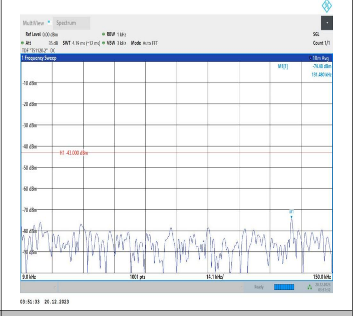
2-2-10MHz-15MHz-16QAM-16QAM-18829-18949-1RB#0-1RB #74-0.009~0.15MHz-PASS
