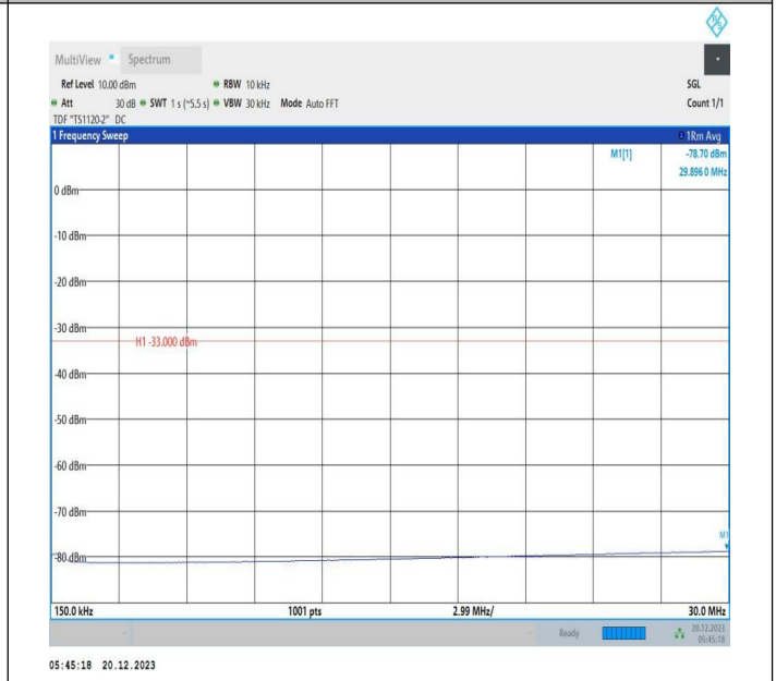
2-2-10MHz-15MHz-16QAM-16QAM-19005-19125-50RB#0-75 RB#0-0.15~30MHz-PASS
