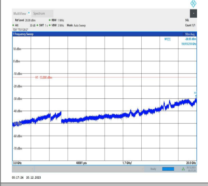
2-2-10MHz-15MHz-QPSK-QPSK-19005-19125-1RB#0-1RB#7 4-3000~20000MHz-PASS
