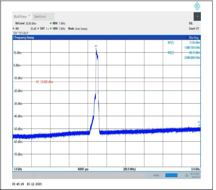
2-2-10MHz-15MHz-16QAM-16QAM-19005-19125-50RB#0-75 RB#0-1000~3000MHz-PASS
