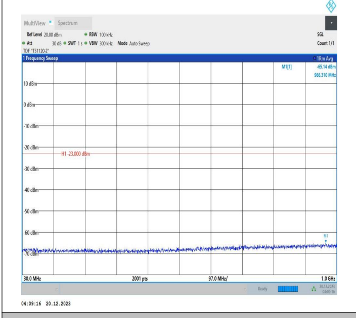
2-2-10MHz-15MHz-64QAM-64QAM-18829-18949-1RB#0-1RB #74-30~1000MHz-PASS
