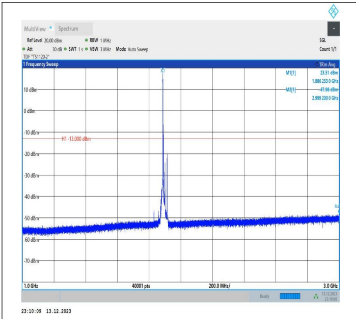
2-2-5MHz-20MHz-16QAM-16QAM-18983-19100-1RB#0-0RB# 0-1000~3000MHz-PASS
