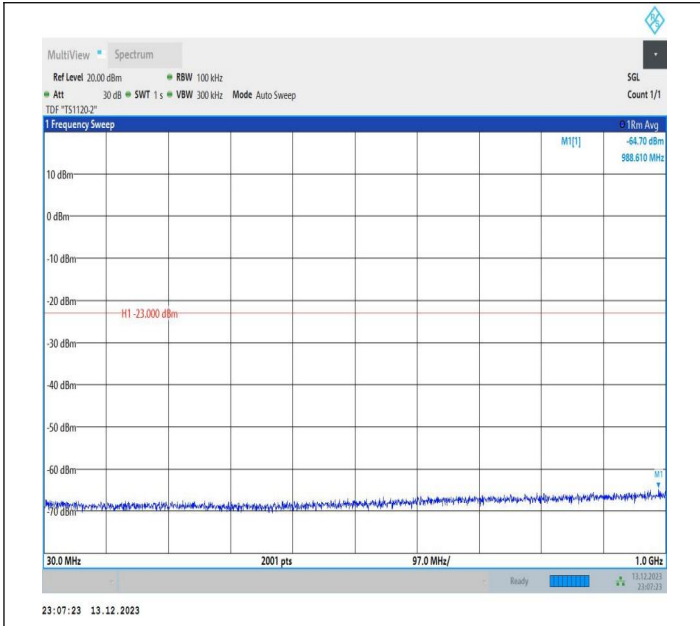
2-2-5MHz-20MHz-QPSK-QPSK-18808-18925-25RB#0-100RB #0-30~1000MHz-PASS
