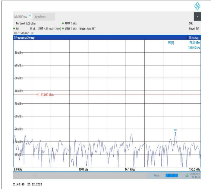
2-2-10MHz-15MHz-QPSK-QPSK-18653-18773-1RB#0-0RB#0 -0.009~0.15MHz-PASS
