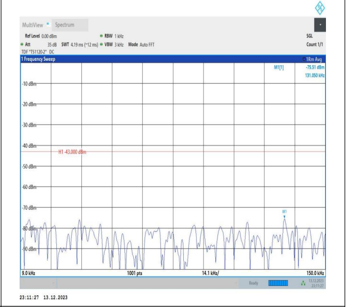
2-2-5MHz-20MHz-16QAM-16QAM-18983-19100-1RB#24-0RB #0-0.009~0.15MHz-PASS
