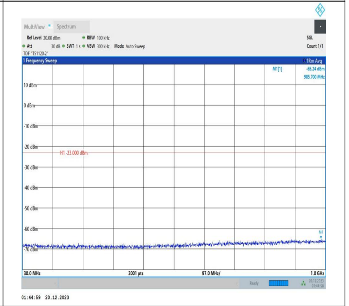
2-2-10MHz-15MHz-16QAM-16QAM-18653-18773-1RB#0-0RB #0-30~1000MHz-PASS
