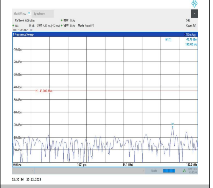
2-2-10MHz-15MHz-16QAM-16QAM-18653-18773-1RB#0-1RB #74-0.009~0.15MHz-PASS
