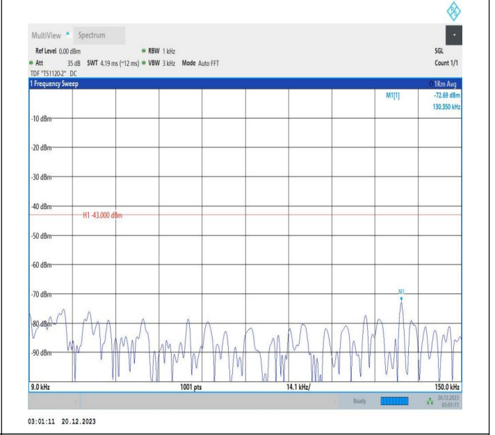
2-2-10MHz-15MHz-64QAM-64QAM-18653-18773-50RB#0-75 RB#0-0.009~0.15MHz-PASS
