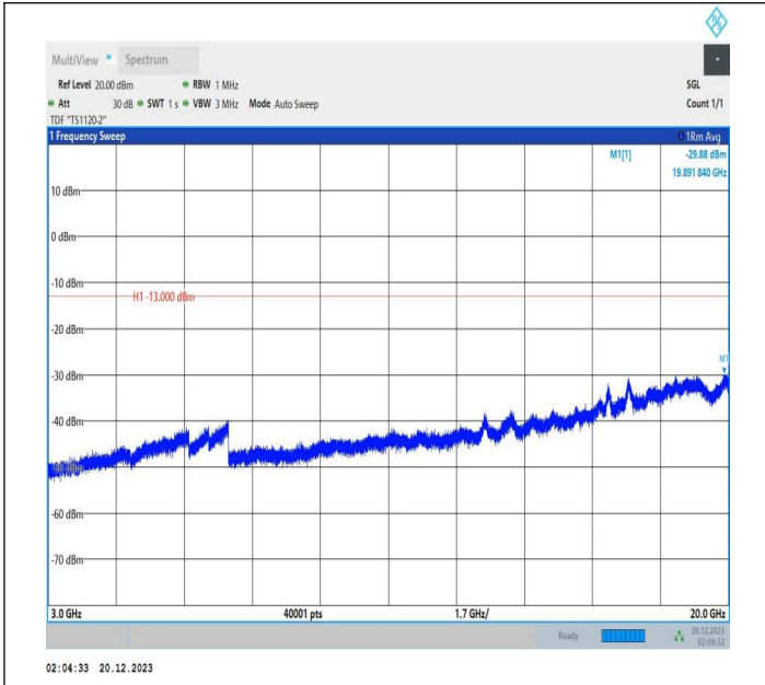
2-2-10MHz-15MHz-16QAM-16QAM-18653-18773-1RB#49-OR B#0-3000~20000MHz-PASS
