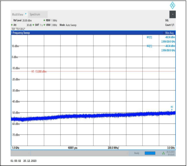
2-2-10MHz-15MHz-64QAM-64QAM-18653-18773-1RB#0-ORB #0-1000~3000MHz-PASS
