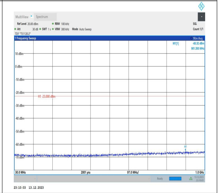
2-2-5MHz-20MHz-16QAM-16QAM-18983-19100-1RB#0-0RB#0-0-30~1000MHz-PASS
