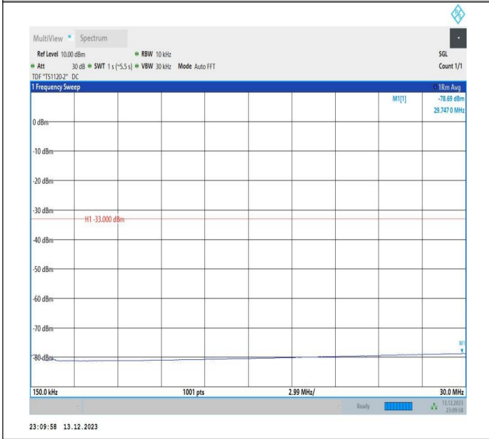
2-2-5MHz-20MHz-16QAM-16QAM-18983-19100-1RB#0-0RB#0-0-0.15~30MHz-PASS
