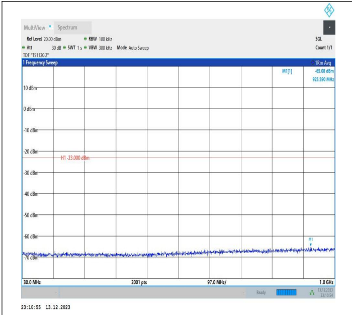
2-2-5MHz-20MHz-QPSK-QPSK-18983-19100-1RB#24-0RB#0 -30~1000MHz-PASS
