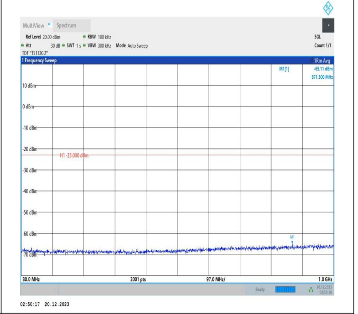
2-2-10MHz-15MHz-QPSK-QPSK-18653-18773-50RB#0-75RB #0-30~1000MHz-PASS
