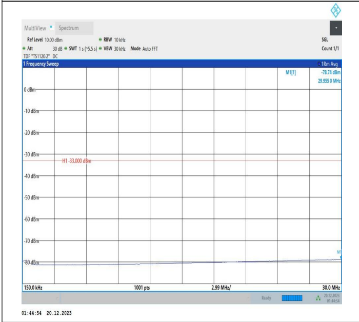
2-2-10MHz-15MHz-16QAM-16QAM-18653-18773-1RB#0-0RB #0-0.15~30MHz-PASS
