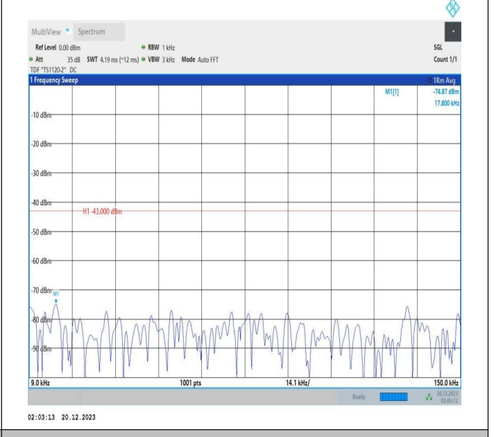
2-2-10MHz-15MHz-QPSK-QPSK-18653-18773-1RB#49-ORB# 0-0.009~0.15MHz-PASS
