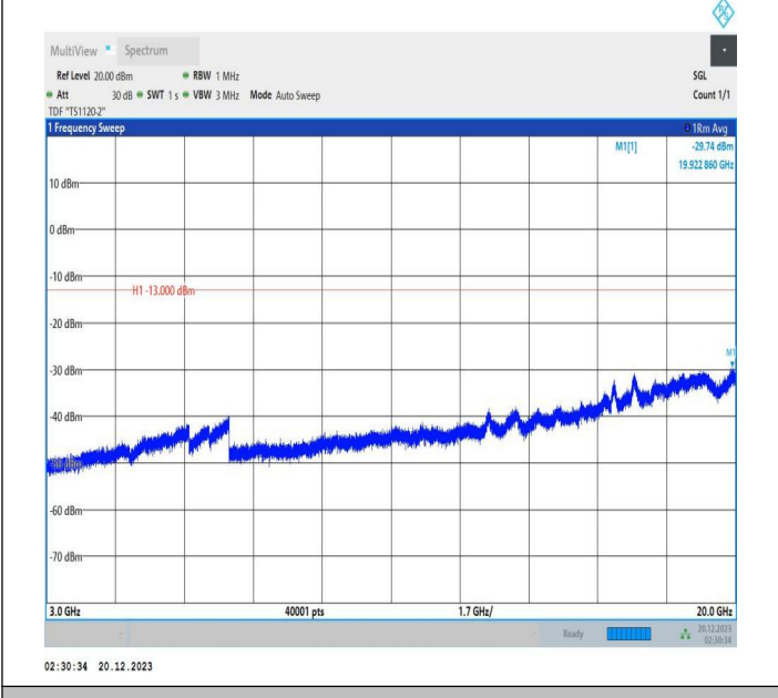
2-2-10MHz-15MHz-QPSK-QPSK-18653-18773-1RB#0-1RB#7 4-3000~20000MHz-PASS
