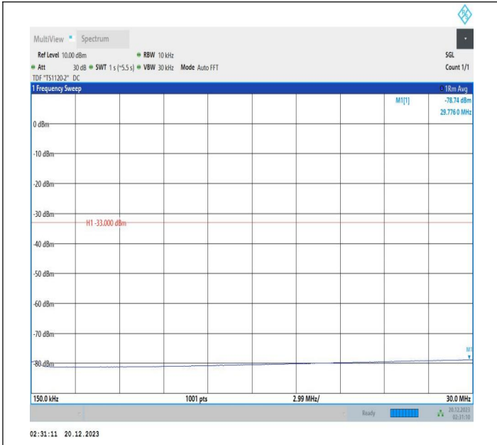
2-2-10MHz-15MHz-16QAM-16QAM-18653-18773-1RB#0-1RB #74-0.15~30MHz-PASS
