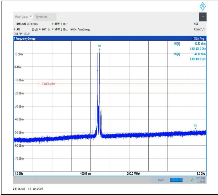
2-2-5MHz-20MHz-16QAM-16QAM-18808-18925-1RB#0-1RB# 99-1000~3000MHz-PASS
