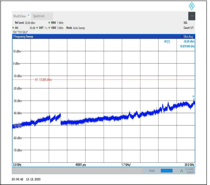
2-2-5MHz-20MHz-16QAM-16QAM-18808-18925-1RB#0-1RB# 99-3000~20000MHz-PASS
