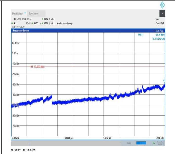
2-2-10MHz-15MHz-QPSK-QPSK-18653-18773-50RB#0-75RB #0-3000~20000MHz-PASS
