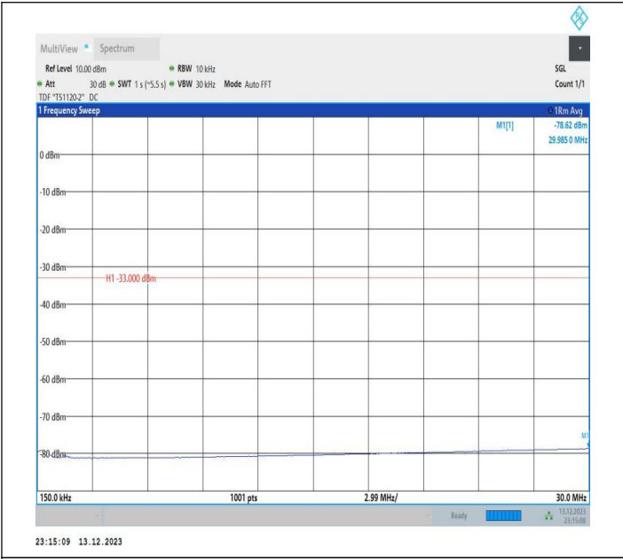
2-2-5MHz-20MHz-16QAM-16QAM-18983-19100-25RB#0-100 RB#0-0.15~30MHz-PASS
