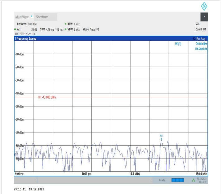
2-2-5MHz-20MHz-16QAM-16QAM-18983-19100-1RB#0-1RB# 99-0.009~0.15MHz-PASS
