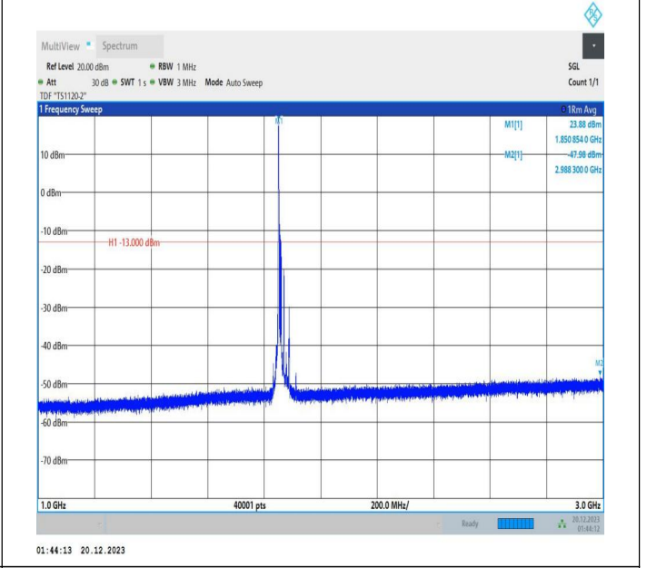
2-2-10MHz-15MHz-QPSK-QPSK-18653-18773-1RB#0-0RB#0 -1000~3000MHz-PASS
