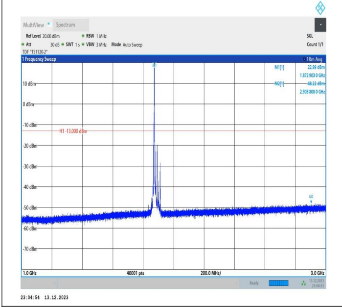
2-2-5MHz-20MHz-16QAM-16QAM-18808-18925-1RB#24-0RB #0-1000~3000MHz-PASS
