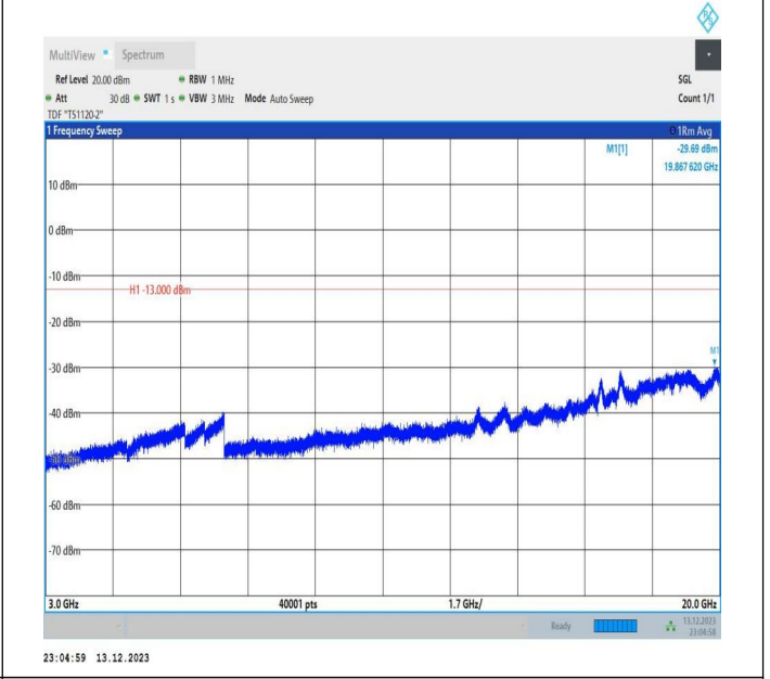
2-2-5MHz-20MHz-16QAM-16QAM-18808-18925-1RB#24-0RB #0-3000~20000MHz-PASS
