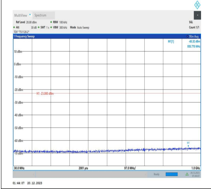
2-2-10MHz-15MHz-QPSK-QPSK-18653-18773-1RB#0-0RB#0 -30~1000MHz-PASS
