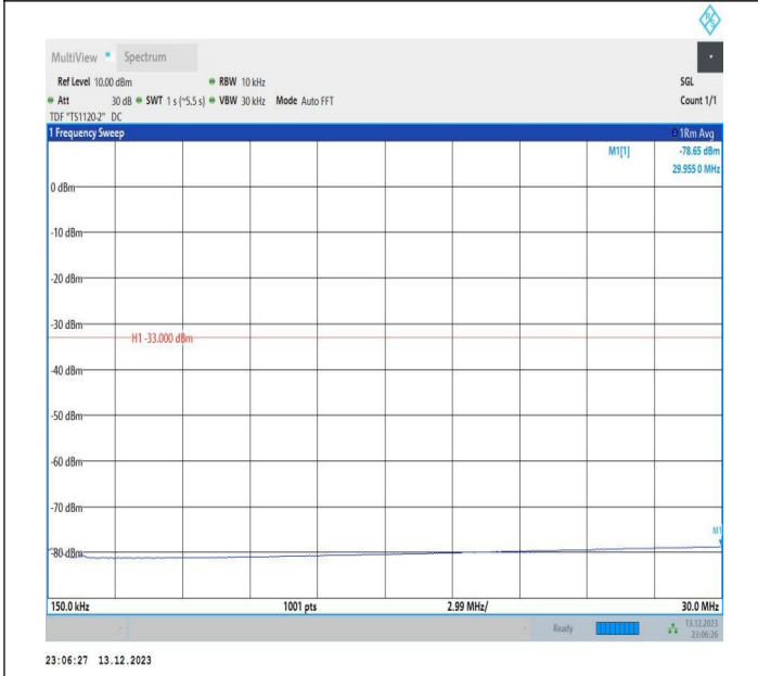
2-2-5MHz-20MHz-16QAM-16QAM-18808-18925-1RB#0-1RB# 99-0.15~30MHz-PASS
