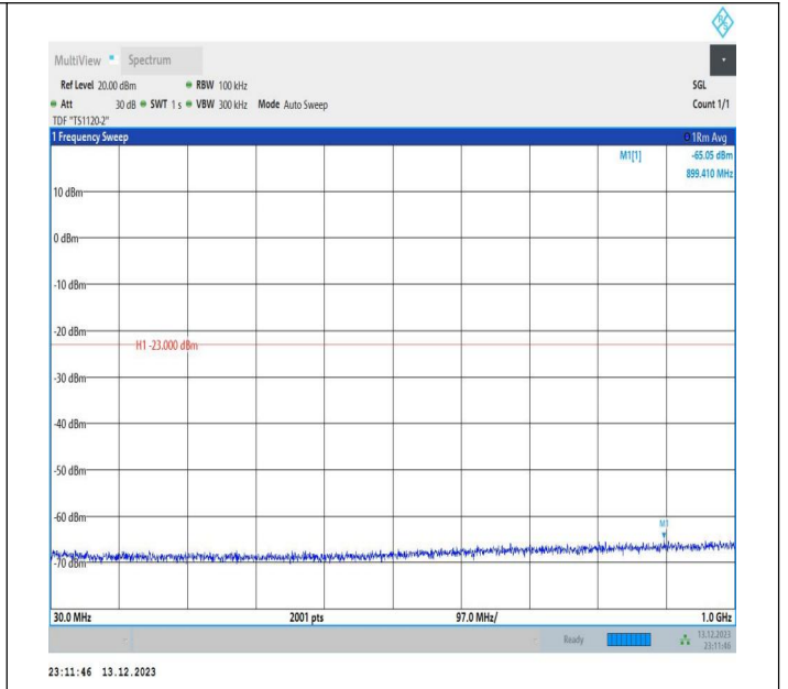
2-2-5MHz-20MHz-16QAM-16QAM-18983-19100-1RB#24-0RB #0-30~1000MHz-PASS
