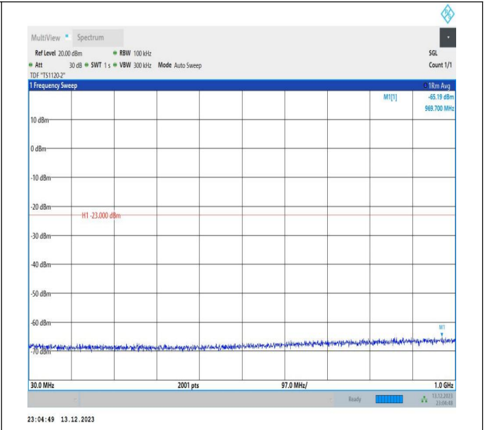
2-2-5MHz-20MHz-16QAM-16QAM-18808-18925-1RB#24-0RB #0-30~1000MHz-PASS
