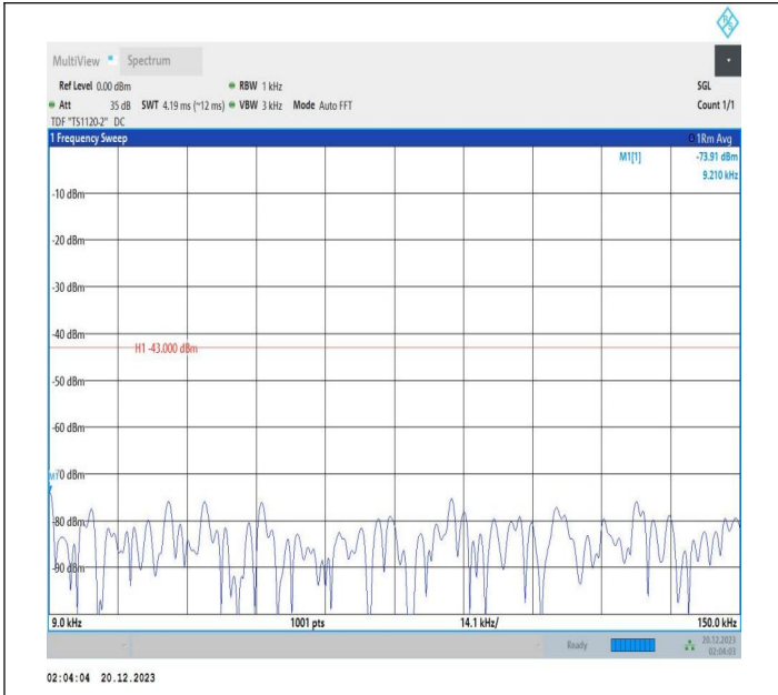
2-2-10MHz-15MHz-16QAM-16QAM-18653-18773-1RB#49-OR B#0-0.009~0.15MHz-PASS
