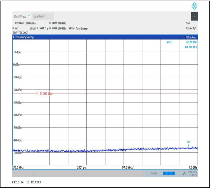
2-2-5MHz-20MHz-16QAM-16QAM-18983-19100-25RB#0-100 RB#0-30~1000MHz-PASS
