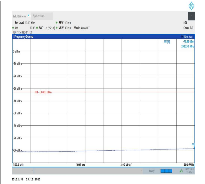
2-2-5MHz-20MHz-QPSK-QPSK-18983-19100-1RB#0-1RB#99 -0.15~30MHz-PASS
