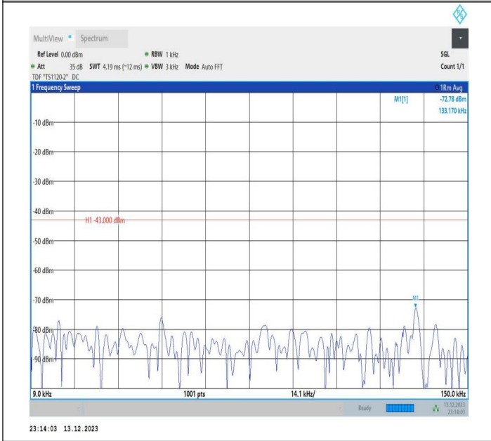
2-2-5MHz-20MHz-QPSK-QPSK-18983-19100-25RB#0-100RB #0-0.009~0.15MHz-PASS
