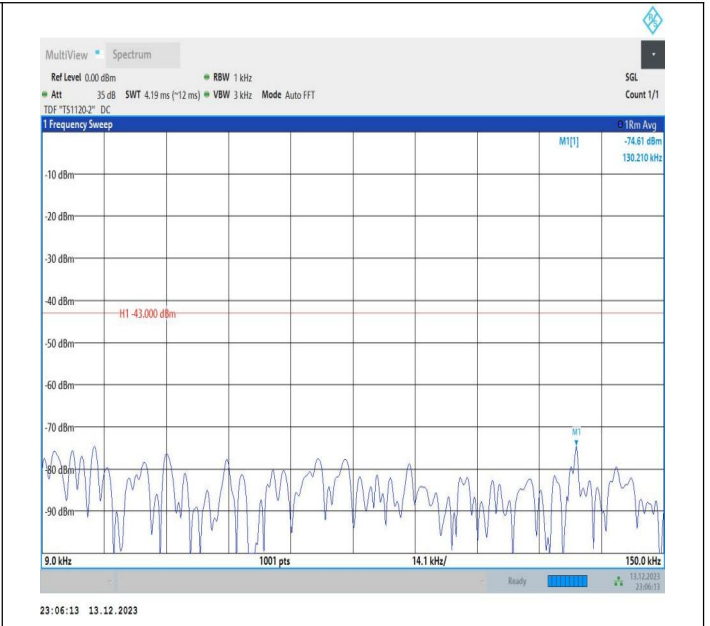
2-2-5MHz-20MHz-16QAM-16QAM-18808-18925-1RB#0-1RB# 99-0.009~0.15MHz-PASS
