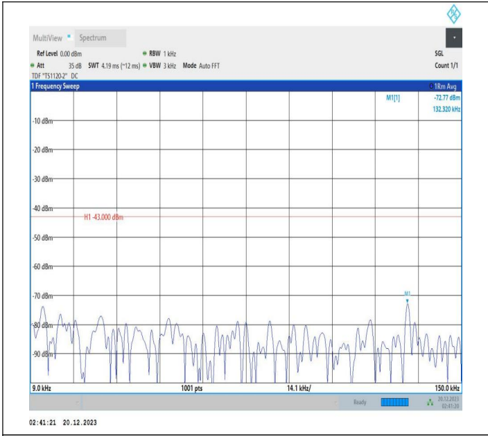
2-2-10MHz-15MHz-64QAM-64QAM-18653-18773-1RB#0-1RB #74-0.009~0.15MHz-PASS
