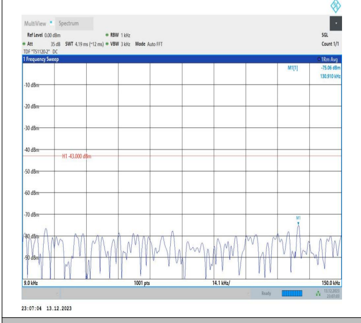
2-2-5MHz-20MHz-QPSK-QPSK-18808-18925-25RB#0-100RB #0-0.009~0.15MHz-PASS
