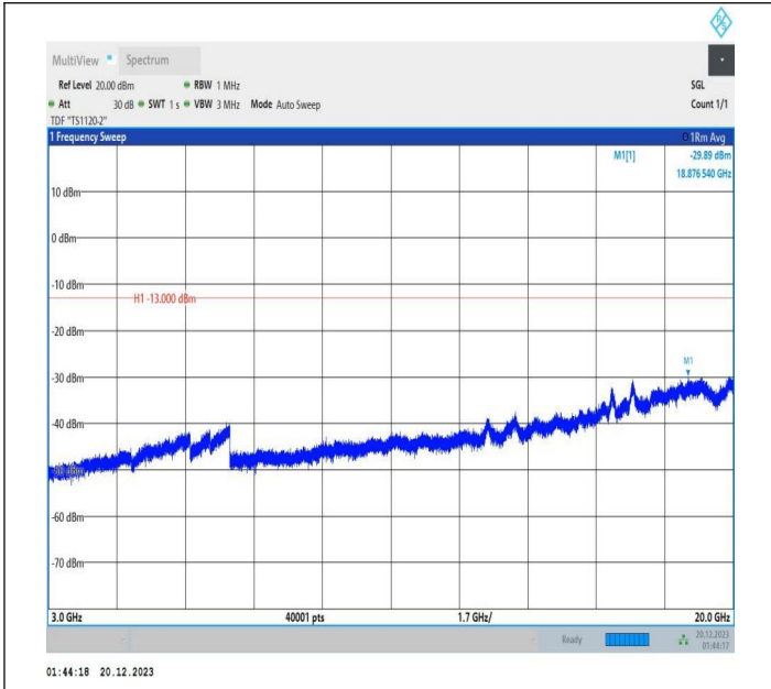
2-2-10MHz-15MHz-QPSK-QPSK-18653-18773-1RB#0-0RB#0 -3000~20000MHz-PASS
