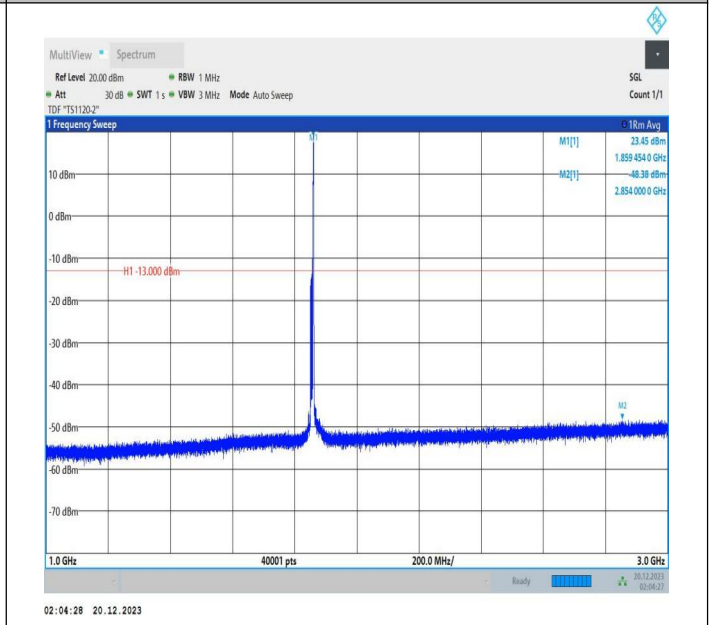
2-2-10MHz-15MHz-16QAM-16QAM-18653-18773-1RB#49-OR B#0-1000~3000MHz-PASS
