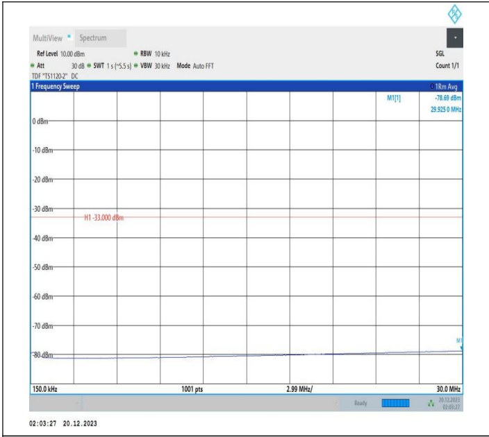
2-2-10MHz-15MHz-QPSK-QPSK-18653-18773-1RB#49-0RB# 0-0.15~30MHz-PASS
