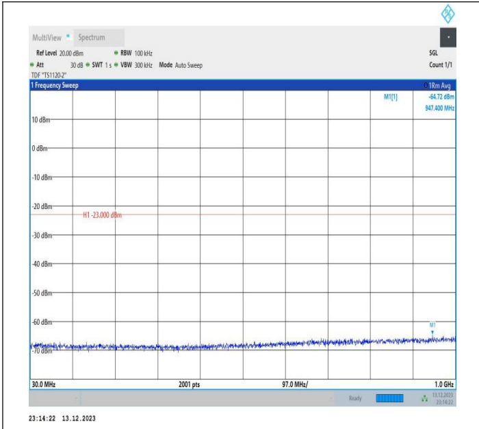
2-2-5MHz-20MHz-QPSK-QPSK-18983-19100-25RB#0-100RB #0-30~1000MHz-PASS
