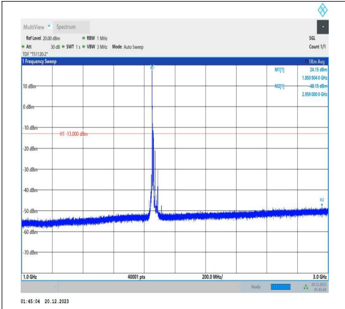
2-2-10MHz-15MHz-16QAM-16QAM-18653-18773-1RB#0-ORB #0-1000~3000MHz-PASS
