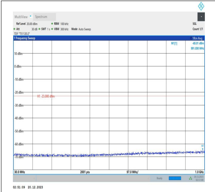
2-2-10MHz-15MHz-16QAM-16QAM-18653-18773-50RB#0-75 RB#0-30~1000MHz-PASS
