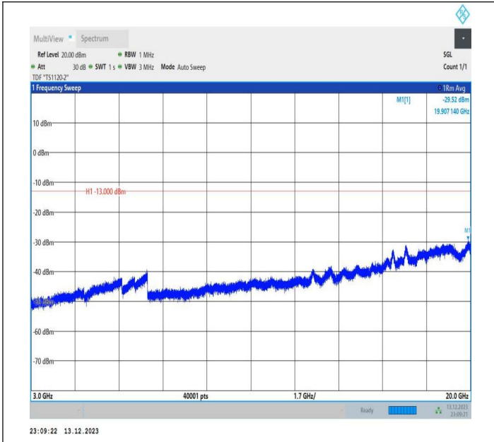
2-2-5MHz-20MHz-QPSK-QPSK-18983-19100-1RB#0-0RB#0-3000~20000MHz-PASS
