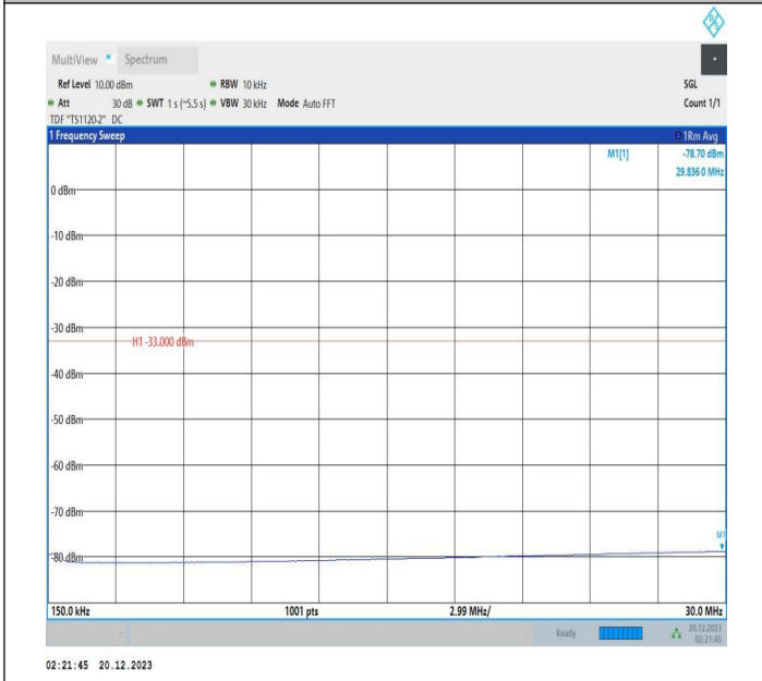
2-2-10MHz-15MHz-64QAM-64QAM-18653-18773-1RB#49-OR B#0-0.15~30MHz-PASS
