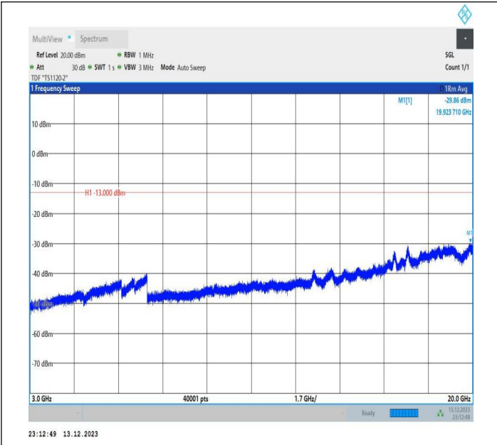
2-2-5MHz-20MHz-QPSK-QPSK-18983-19100-1RB#0-1RB#99 -3000~20000MHz-PASS
