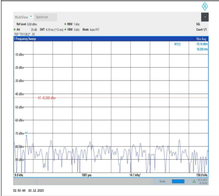
2-2-10MHz-15MHz-16QAM-16QAM-18653-18773-50RB#0-75 RB#0-0.009~0.15MHz-PASS
