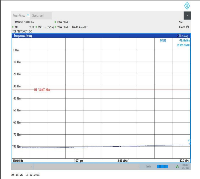
2-2-5MHz-20MHz-16QAM-16QAM-18983-19100-1RB#0-1RB# 99-0.15~30MHz-PASS
