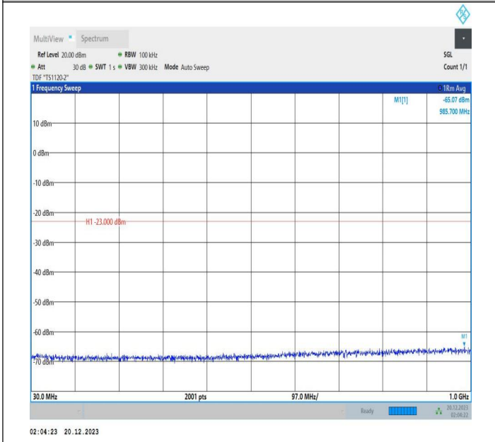
2-2-10MHz-15MHz-16QAM-16QAM-18653-18773-1RB#49-OR B#0-30~1000MHz-PASS
