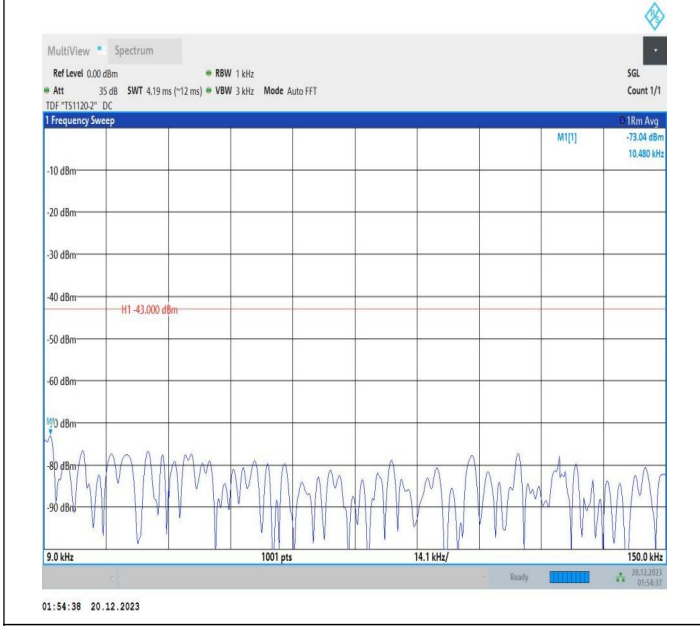
2-2-10MHz-15MHz-64QAM-64QAM-18653-18773-1RB#0-ORB #0-0.009~0.15MHz-PASS
