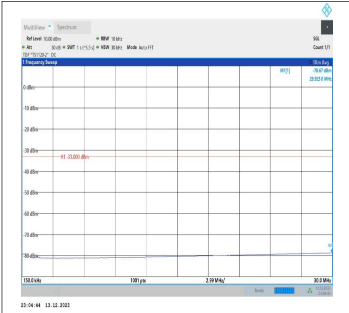
2-2-5MHz-20MHz-16QAM-16QAM-18808-18925-1RB#24-0RB #0-0.15~30MHz-PASS
