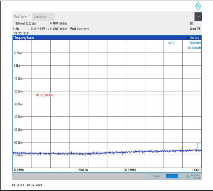
2-2-10MHz-15MHz-64QAM-64QAM-18653-18773-1RB#0-ORB #0-30~1000MHz-PASS
