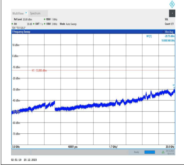
2-2-10MHz-15MHz-16QAM-16QAM-18653-18773-50RB#0-75 RB#0-3000~20000MHz-PASS
