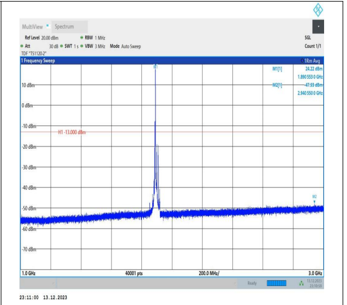
2-2-5MHz-20MHz-QPSK-QPSK-18983-19100-1RB#24-0RB#0 -1000~3000MHz-PASS
