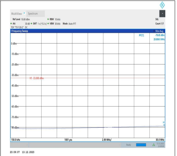
2-2-5MHz-20MHz-QPSK-QPSK-18983-19100-1RB#0-0RB#0-0.15~30MHz-PASS
