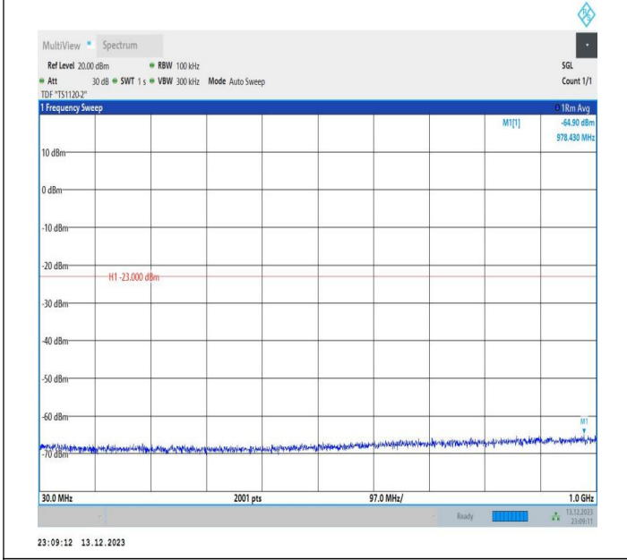
2-2-5MHz-20MHz-QPSK-QPSK-18983-19100-1RB#0-0RB#0-30~1000MHz-PASS
