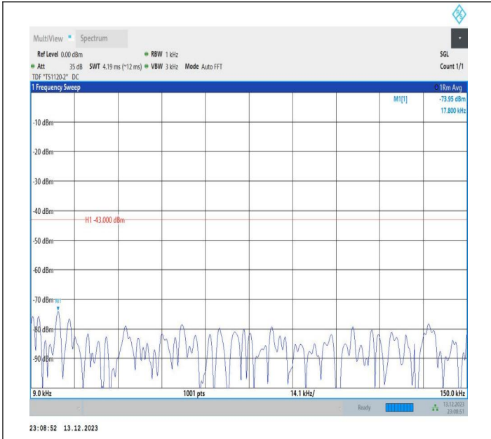
2-2-5MHz-20MHz-QPSK-QPSK-18983-19100-1RB#0-0RB#0-0.009~0.15MHz-PASS
