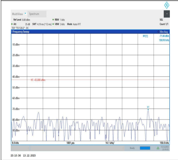
2-2-5MHz-20MHz-QPSK-QPSK-18983-19100-1RB#24-0RB# -0.009~0.15MHz-PASS
