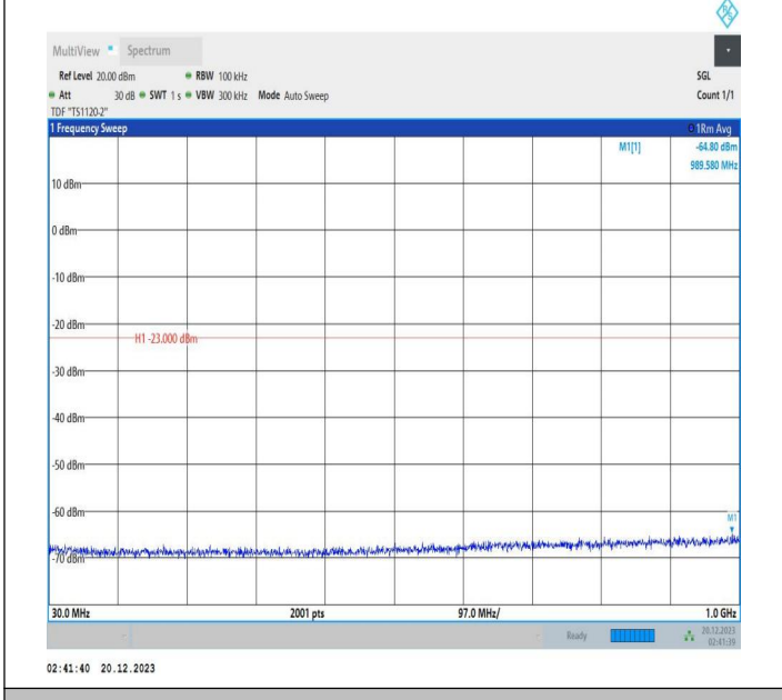
2-2-10MHz-15MHz-64QAM-64QAM-18653-18773-1RB#0-1RB #74-30~1000MHz-PASS
