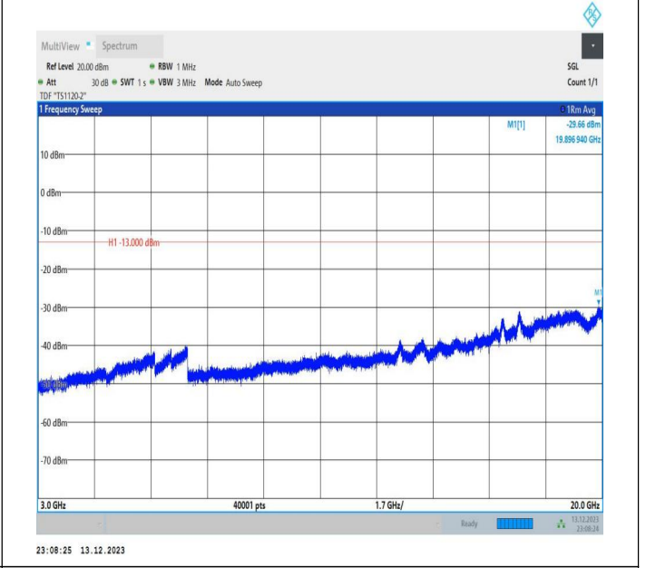
2-2-5MHz-20MHz-16QAM-16QAM-18808-18925-25RB#0-100 RB#0-3000~20000MHz-PASS
