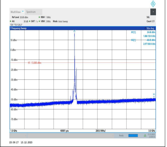
2-2-5MHz-20MHz-QPSK-QPSK-18983-19100-1RB#0-0RB#0-1000~3000MHz-PASS
