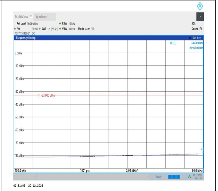
2-2-10MHz-15MHz-16QAM-16QAM-18653-18773-50RB#0-75 RB#0-0.15~30MHz-PASS
