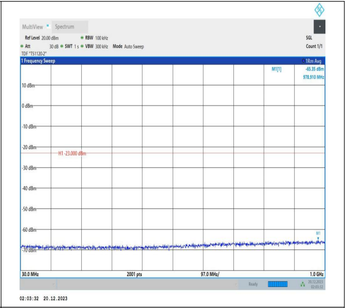
2-2-10MHz-15MHz-QPSK-QPSK-18653-18773-1RB#49-0RB# 0-30~1000MHz-PASS
