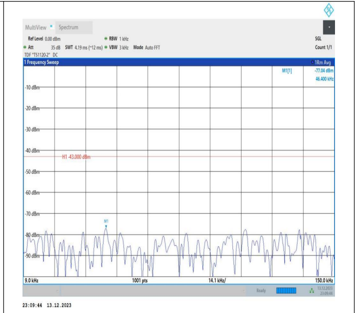
2-2-5MHz-20MHz-16QAM-16QAM-18983-19100-1RB#0-0RB#0-0-0.009~0.15MHz-PASS
