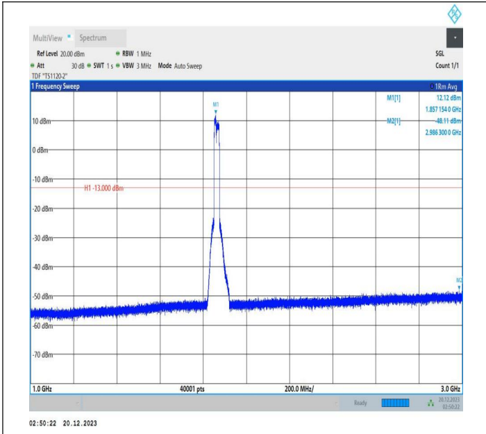
2-2-10MHz-15MHz-QPSK-QPSK-18653-18773-50RB#0-75RB #0-1000~3000MHz-PASS
