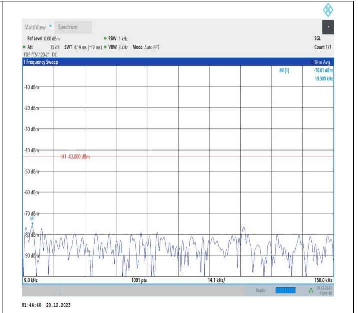
2-2-10MHz-15MHz-16QAM-16QAM-18653-18773-1RB#0-0RB #0-0.009~0.15MHz-PASS
