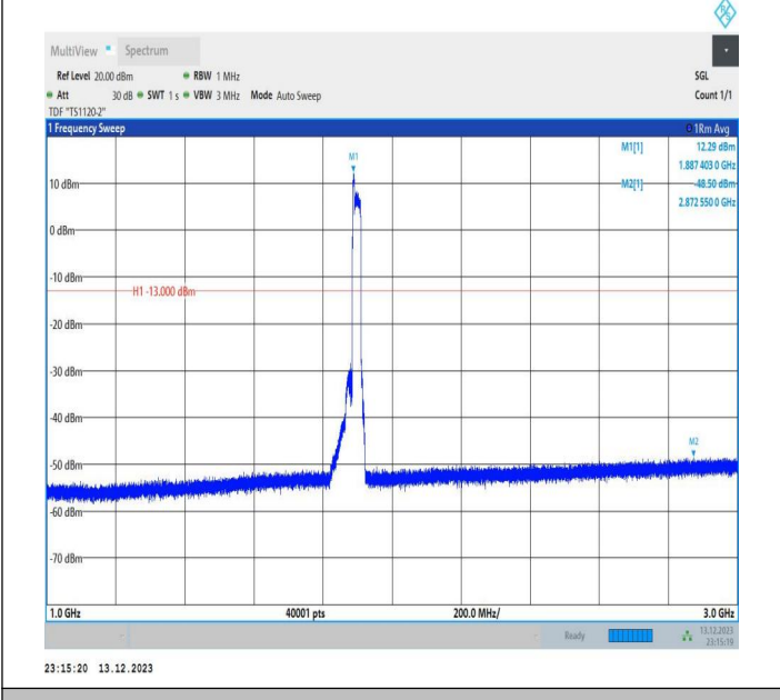
2-2-5MHz-20MHz-16QAM-16QAM-18983-19100-25RB#0-100 RB#0-1000~3000MHz-PASS
