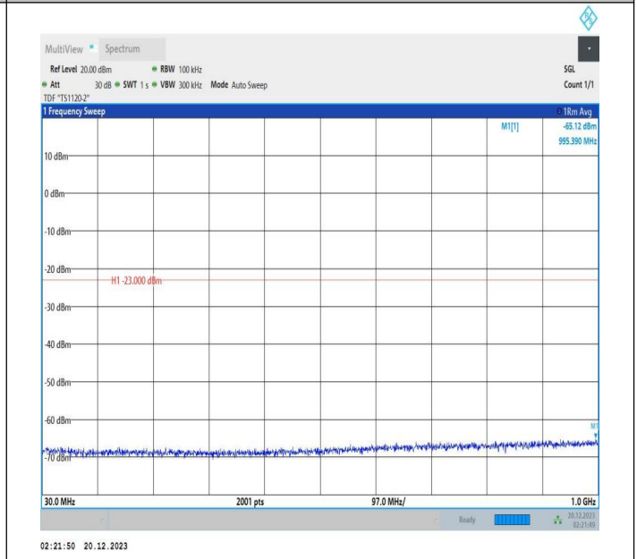
2-2-10MHz-15MHz-64QAM-64QAM-18653-18773-1RB#49-OR B#0-30~1000MHz-PASS
