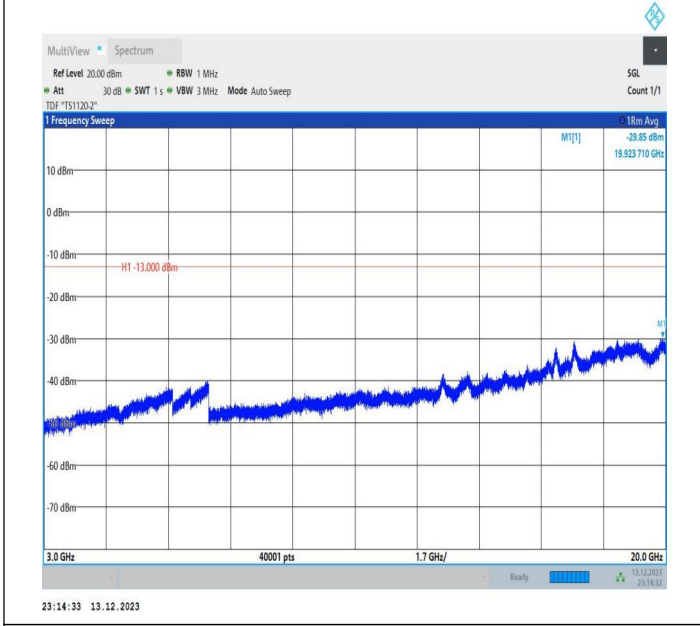
2-2-5MHz-20MHz-QPSK-QPSK-18983-19100-25RB#0-100RB #0-3000~20000MHz-PASS
