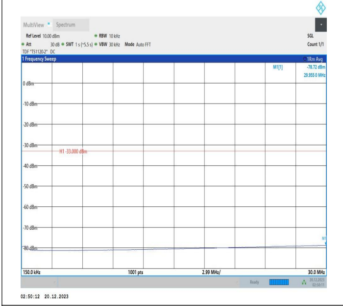
2-2-10MHz-15MHz-QPSK-QPSK-18653-18773-50RB#0-75RB #0-0.15~30MHz-PASS
