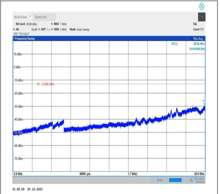
2-2-10MHz-15MHz-16QAM-16QAM-18653-18773-1RB#0-ORB #0-3000~20000MHz-PASS
