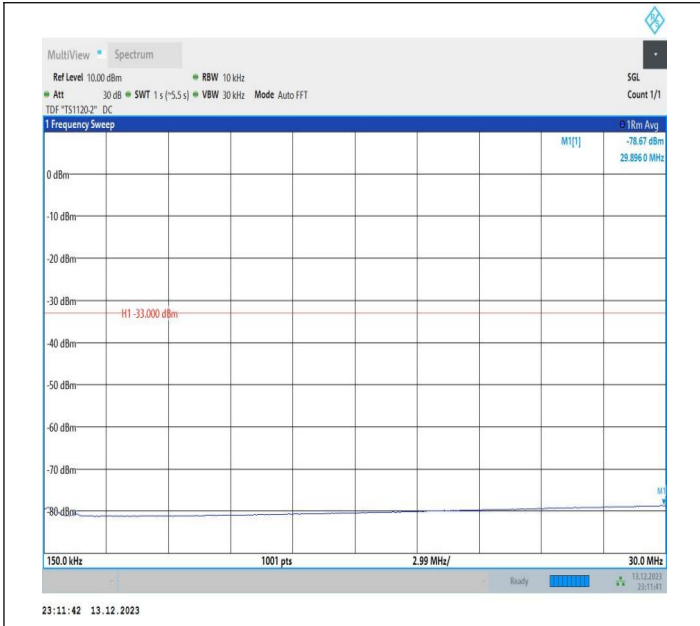
2-2-5MHz-20MHz-16QAM-16QAM-18983-19100-1RB#24-0RB #0-0.15~30MHz-PASS
