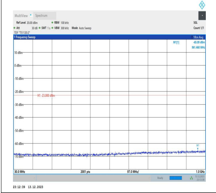
2-2-5MHz-20MHz-QPSK-QPSK-18983-19100-1RB#0-1RB#99 -30~1000MHz-PASS
