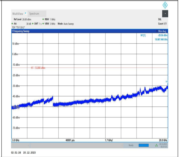
2-2-10MHz-15MHz-16QAM-16QAM-18653-18773-1RB#0-1RB #74-3000~20000MHz-PASS
