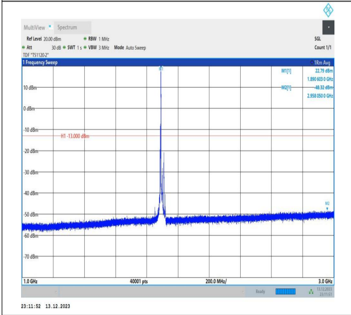
2-2-5MHz-20MHz-16QAM-16QAM-18983-19100-1RB#24-0RB #0-1000~3000MHz-PASS
