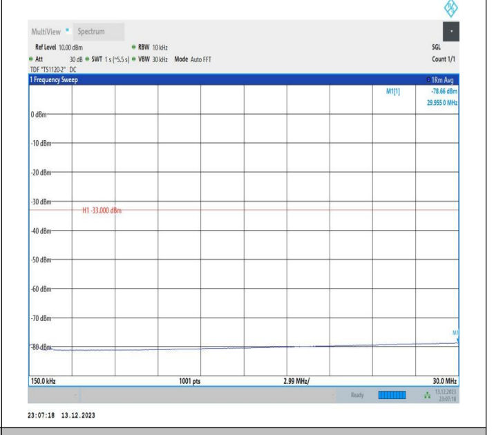
2-2-5MHz-20MHz-QPSK-QPSK-18808-18925-25RB#0-100RB #0-0.15~30MHz-PASS
