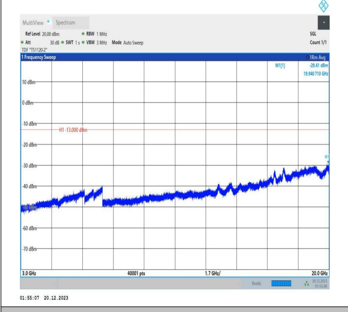
2-2-10MHz-15MHz-64QAM-64QAM-18653-18773-1RB#0-ORB #0-3000~20000MHz-PASS
