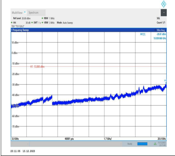
2-2-5MHz-20MHz-QPSK-QPSK-18983-19100-1RB#24-0RB#0 -3000~20000MHz-PASS
