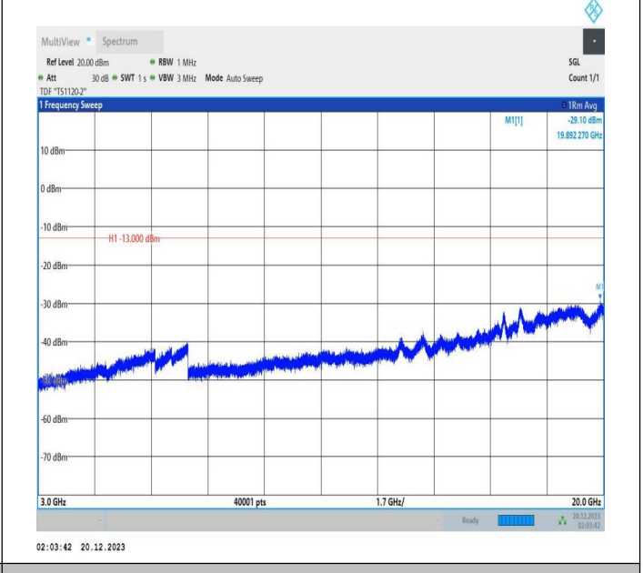
2-2-10MHz-15MHz-QPSK-QPSK-18653-18773-1RB#49-0RB# 0-3000~20000MHz-PASS
