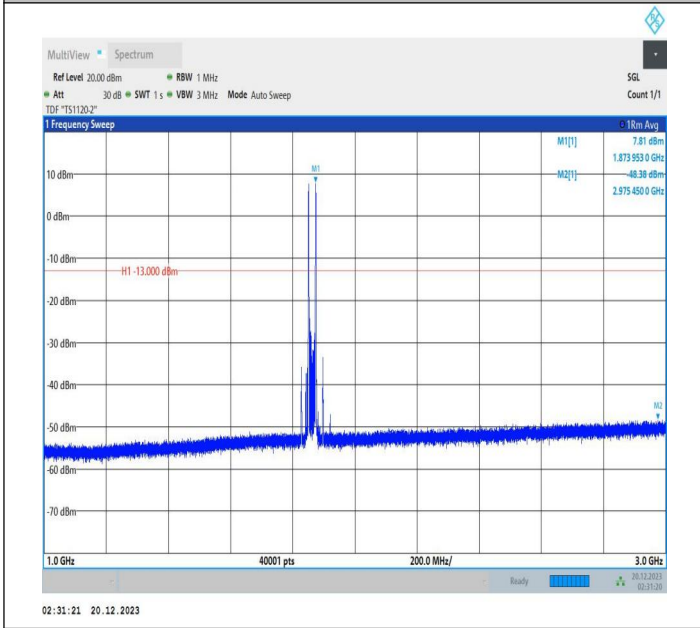
2-2-10MHz-15MHz-16QAM-16QAM-18653-18773-1RB#0-1RB #74-1000~3000MHz-PASS
