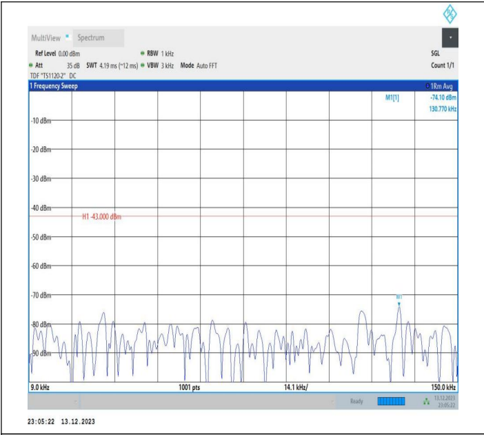
2-2-5MHz-20MHz-QPSK-QPSK-18808-18925-1RB#0-1RB#99 -0.009~0.15MHz-PASS
