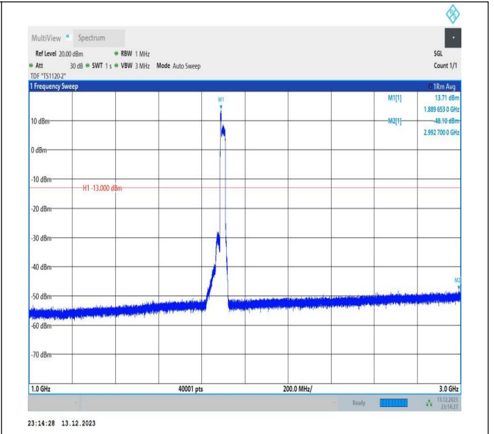
2-2-5MHz-20MHz-QPSK-QPSK-18983-19100-25RB#0-100RB #0-1000~3000MHz-PASS
