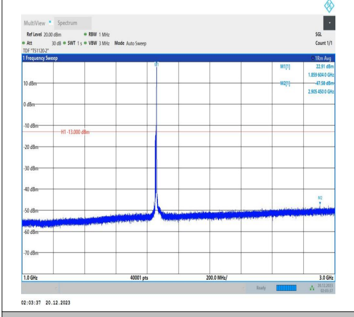
2-2-10MHz-15MHz-QPSK-QPSK-18653-18773-1RB#49-0RB# 0-1000~3000MHz-PASS
