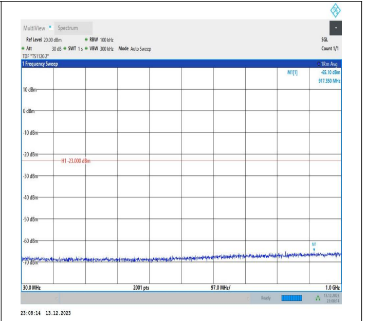
2-2-5MHz-20MHz-16QAM-16QAM-18808-18925-25RB#0-100 RB#0-30~1000MHz-PASS
