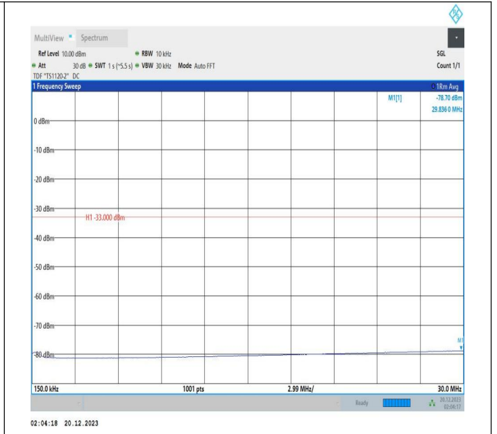
2-2-10MHz-15MHz-16QAM-16QAM-18653-18773-1RB#49-OR B#0-0.15~30MHz-PASS
