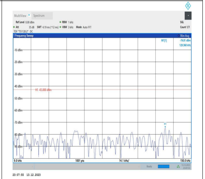
2-2-5MHz-20MHz-16QAM-16QAM-18808-18925-25RB#0-100 RB#0-0.009~0.15MHz-PASS
