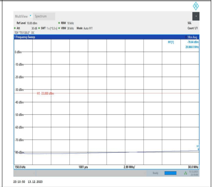
2-2-5MHz-20MHz-QPSK-QPSK-18983-19100-1RB#24-0RB# -0.15~30MHz-PASS
