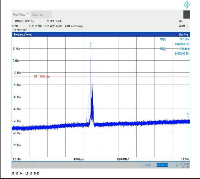
2-2-5MHz-20MHz-QPSK-QPSK-18983-19100-1RB#0-1RB#99 -1000~3000MHz-PASS
