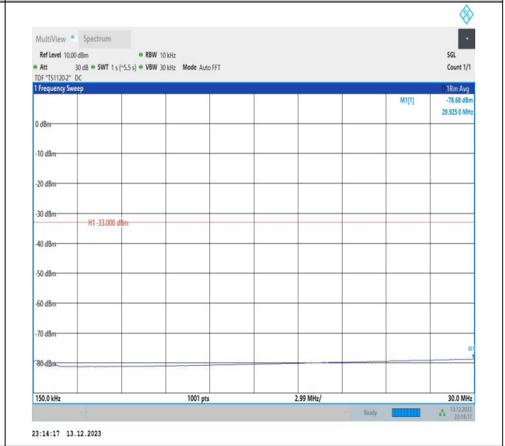
2-2-5MHz-20MHz-QPSK-QPSK-18983-19100-25RB#0-100RB #0-0.15~30MHz-PASS
