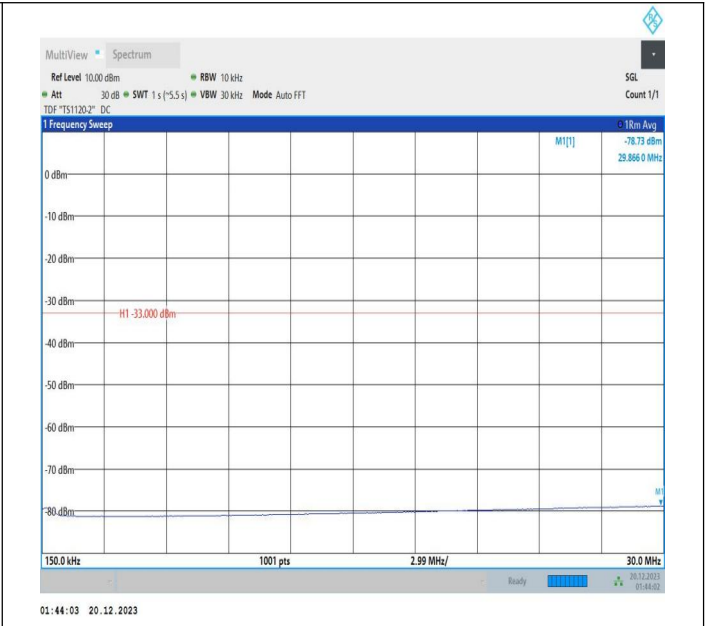
2-2-10MHz-15MHz-QPSK-QPSK-18653-18773-1RB#0-0RB#0 -0.15~30MHz-PASS
