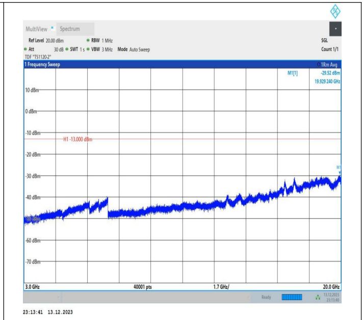
2-2-5MHz-20MHz-16QAM-16QAM-18983-19100-1RB#0-1RB# 99-3000~20000MHz-PASS
