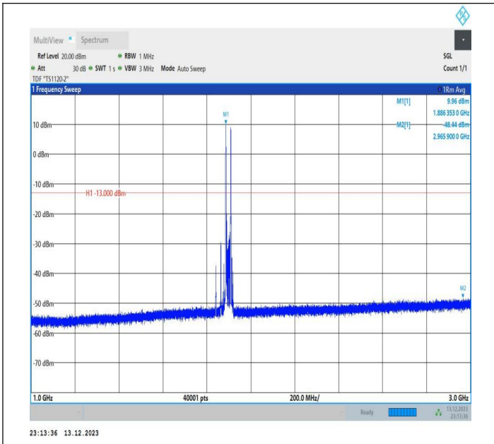
2-2-5MHz-20MHz-16QAM-16QAM-18983-19100-1RB#0-1RB# 99-1000~3000MHz-PASS
