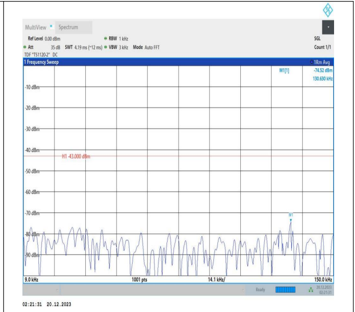
2-2-10MHz-15MHz-64QAM-64QAM-18653-18773-1RB#49-OR B#0-0.009~0.15MHz-PASS
