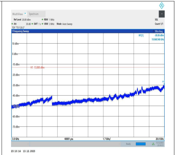
2-2-5MHz-20MHz-16QAM-16QAM-18983-19100-1RB#0-0RB# 0-3000~20000MHz-PASS
