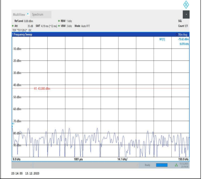
2-2-5MHz-20MHz-16QAM-16QAM-18983-19100-25RB#0-100 RB#0-0.009~0.15MHz-PASS
