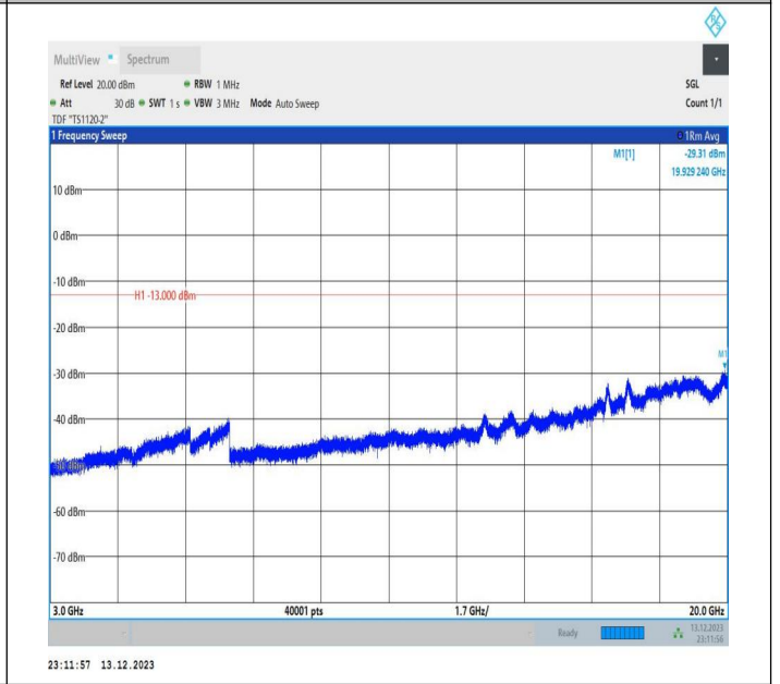
2-2-5MHz-20MHz-16QAM-16QAM-18983-19100-1RB#24-0RB #0-3000~20000MHz-PASS
