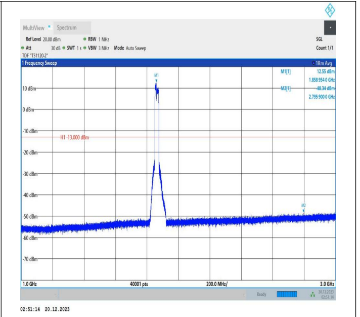
2-2-10MHz-15MHz-16QAM-16QAM-18653-18773-50RB#0-75 RB#0-1000~3000MHz-PASS
