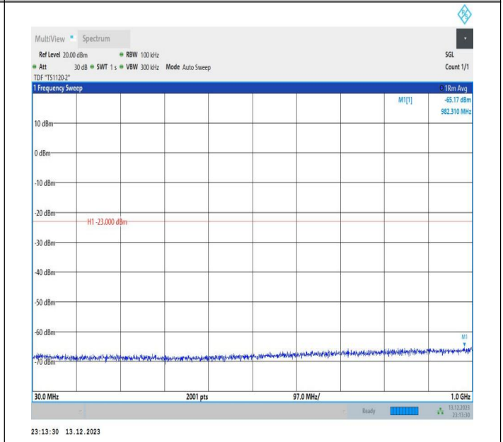
2-2-5MHz-20MHz-16QAM-16QAM-18983-19100-1RB#0-1RB# 99-30~1000MHz-PASS
