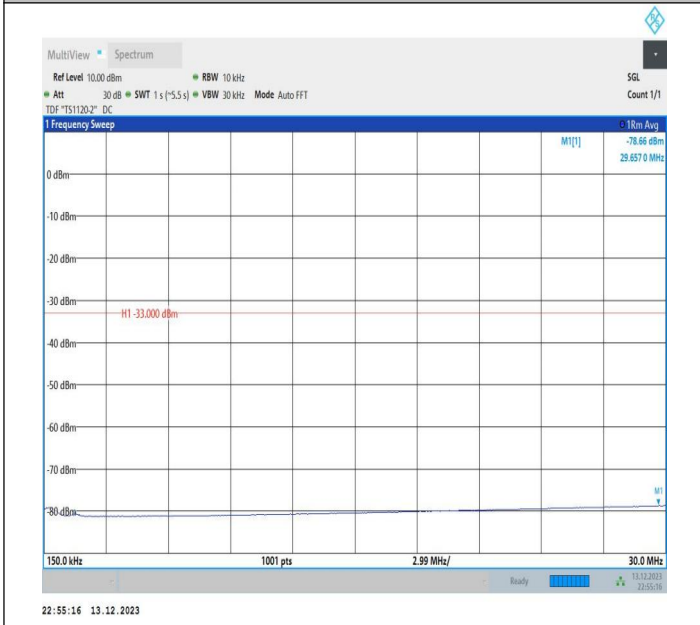
2-2-5MHz-20MHz-16QAM-16QAM-18633-18750-1RB#0-0RB#0-0-0.15~30MHz-PASS
