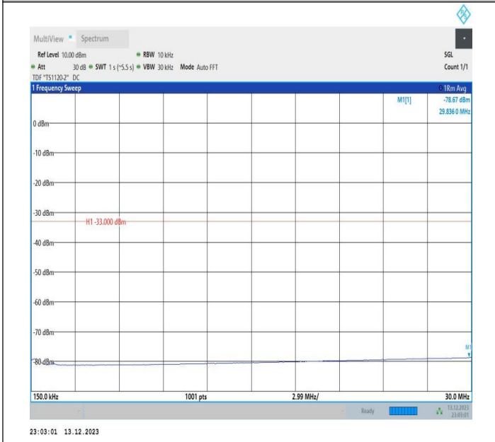
2-2-5MHz-20MHz-16QAM-16QAM-18808-18925-1RB#0-0RB#0-0-0.15~30MHz-PASS
