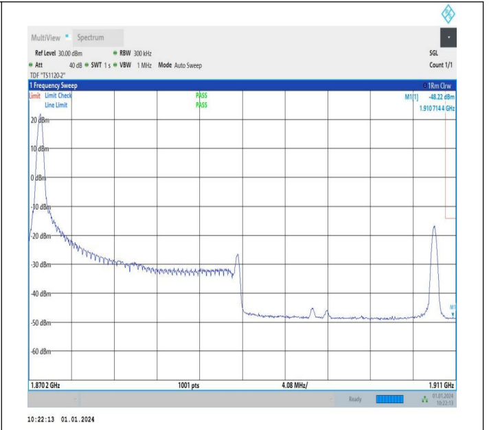
20MHz-20MHz_64QAM@64QAM-64QAM@64QAM_18902-19100_1RB#0@100RB#0-0RB#0@100RB#0
