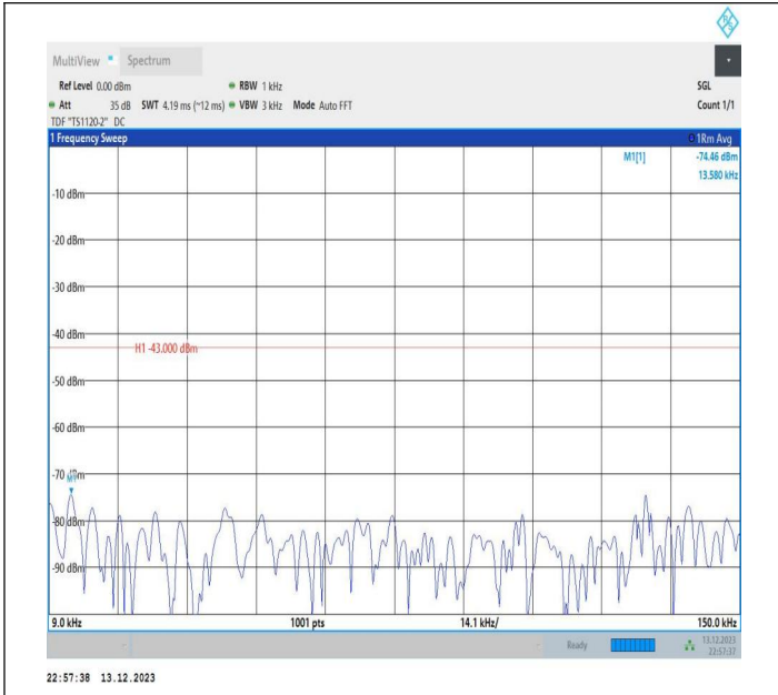
2-2-5MHz-20MHz-QPSK-QPSK-18633-18750-1RB#0-1RB#99 -0.009~0.15MHz-PASS
