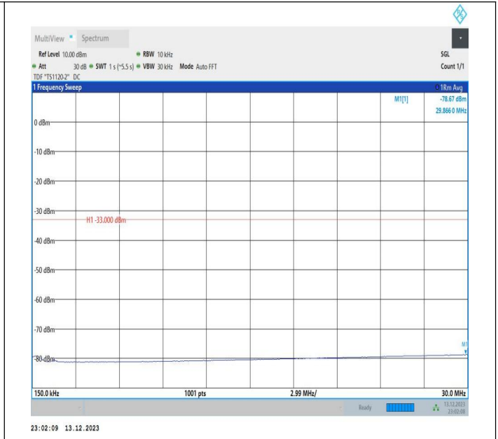
2-2-5MHz-20MHz-QPSK-QPSK-18808-18925-1RB#0-0RB#0-0.15~30MHz-PASS
