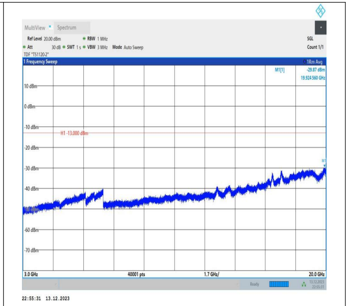
2-2-5MHz-20MHz-16QAM-16QAM-18633-18750-1RB#0-0RB# 0-3000~20000MHz-PASS
