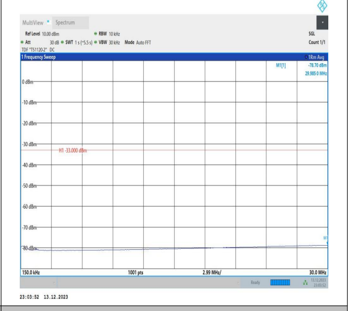
2-2-5MHz-20MHz-QPSK-QPSK-18808-18925-1RB#24-0RB#0 -0.15~30MHz-PASS
