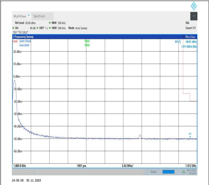
20MHz-5MHz_16QAM@16QAM-16QAM@16QAM_19050-19167_1 RB#0@100RB#0-0RB#0@25RB#0
