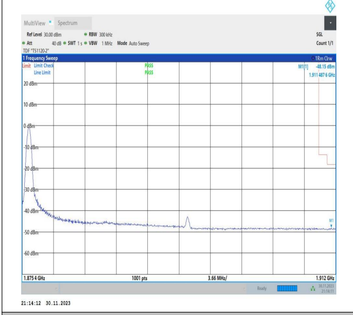
20MHz-15MHz_QPSK@QPSK-QPSK@QPSK_18951-19122_1RB#0@100RB#0-0RB#0@75RB#0
