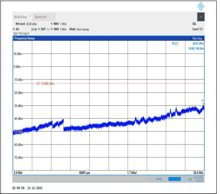
2-2-5MHz-20MHz-16QAM-16QAM-18633-18750-1RB#0-1RB# 99-3000~20000MHz-PASS
