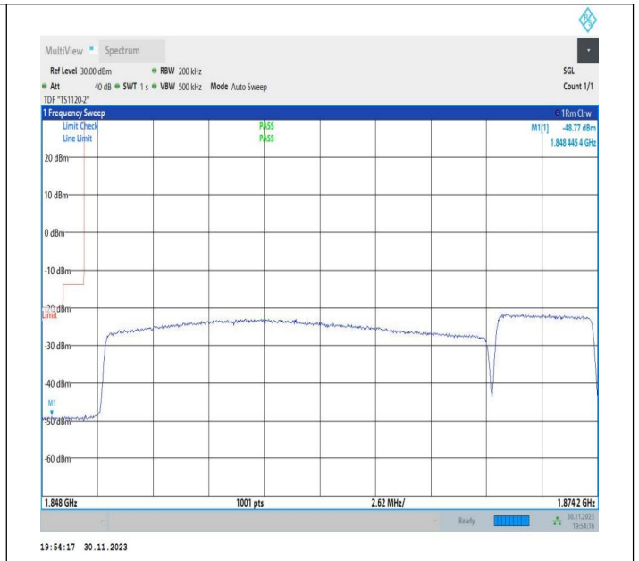
20MHz-5MHz_16QAM@16QAM-16QAM@16QAM_18700-18817_100RB#0@100RB#0-25RB#0@25RB#0
