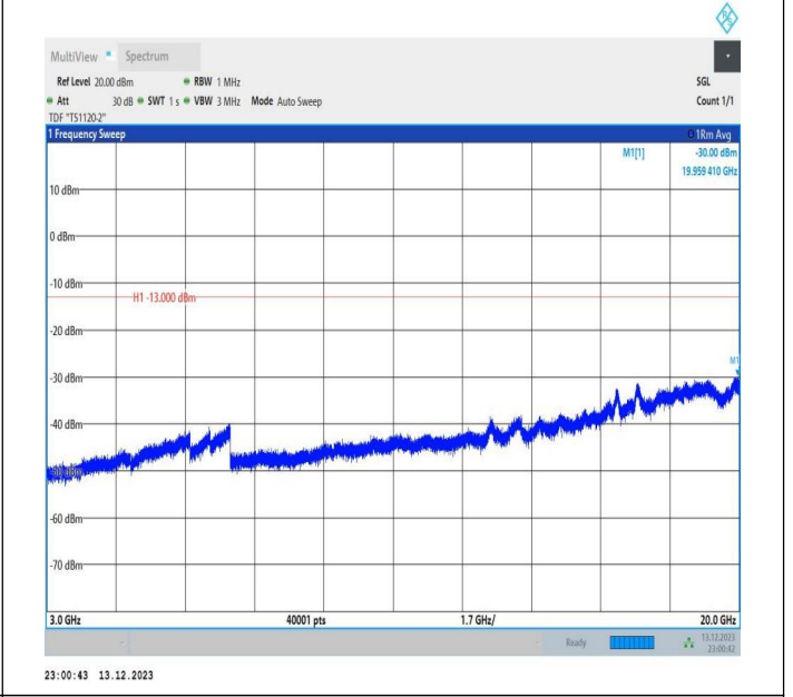
2-2-5MHz-20MHz-16QAM-16QAM-18633-18750-25RB#0-100 RB#0-3000~20000MHz-PASS
