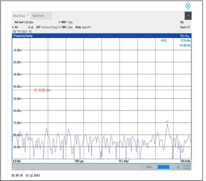
2-2-5MHz-20MHz-16QAM-16QAM-18633-18750-1RB#0-1RB# 99-0.009~0.15MHz-PASS
