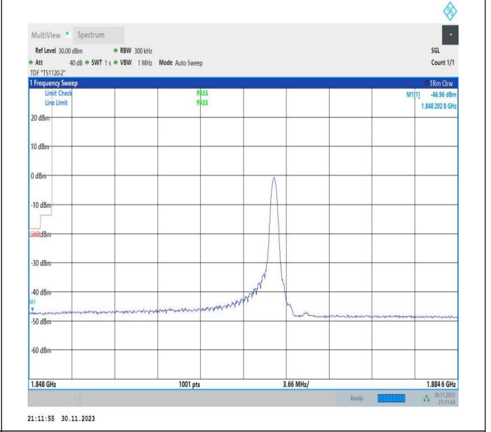
20MHz-15MHz_QPSK@QPSK-QPSK@QPSK_18700-18871_1RB#99@100RB#0-0RB#0@75RB#0
