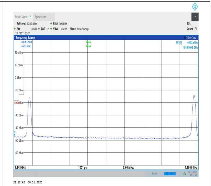
20MHz-15MHz_QPSK@QPSK-QPSK@QPSK_18700-18871_1RB#0@100RB#0-1RB#74@75RB#0
