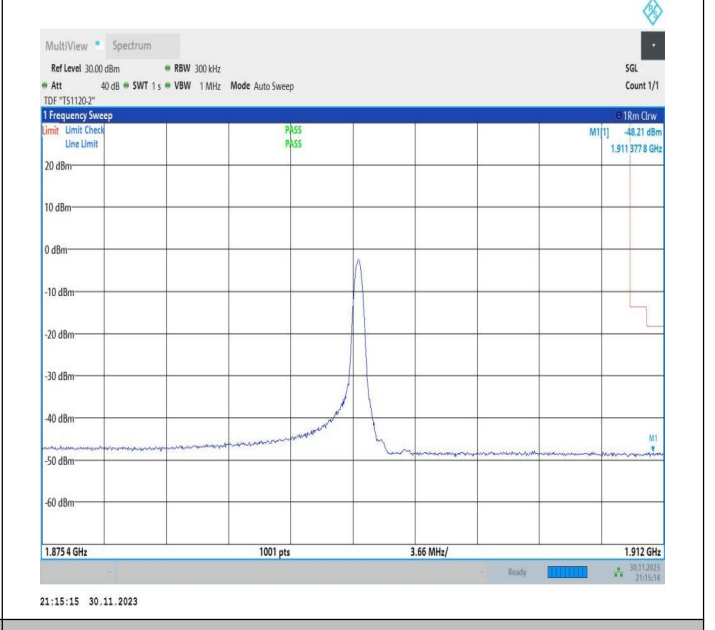
20MHz-15MHz_16QAM@16QAM-16QAM@16QAM_18951-19122_1RB#99@100RB#0-0RB#0@75RB#0
