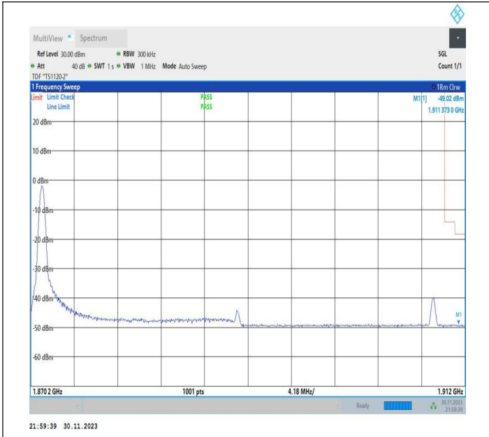
20MHz-20MHz_16QAM@16QAM-16QAM@16QAM_18902-19100_1RB#0@100RB#0-0RB#0@100RB#0
