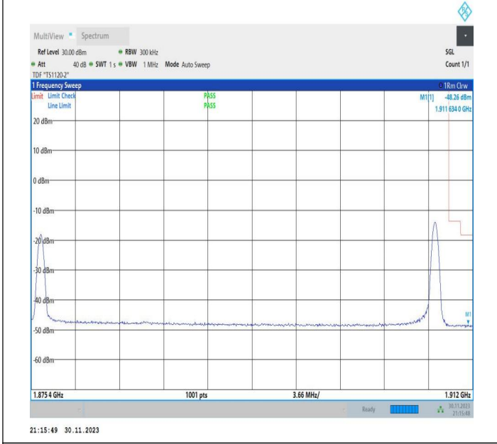
20MHz-15MHz_QPSK@QPSK-QPSK@QPSK_18951-19122_1RB#0@100RB#0-1RB#74@75RB#0
