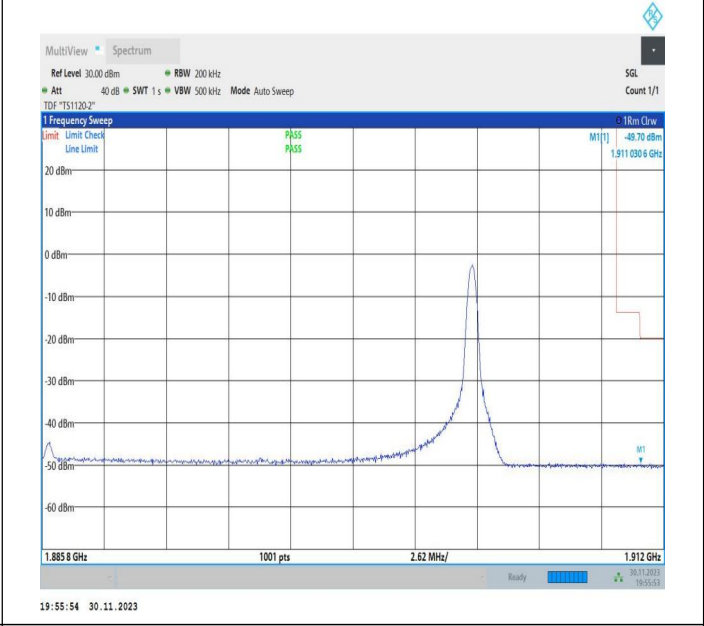
20MHz-5MHz_16QAM@16QAM-16QAM@16QAM_19050-19167_1 RB#99@100RB#0-0RB#0@25RB#0
