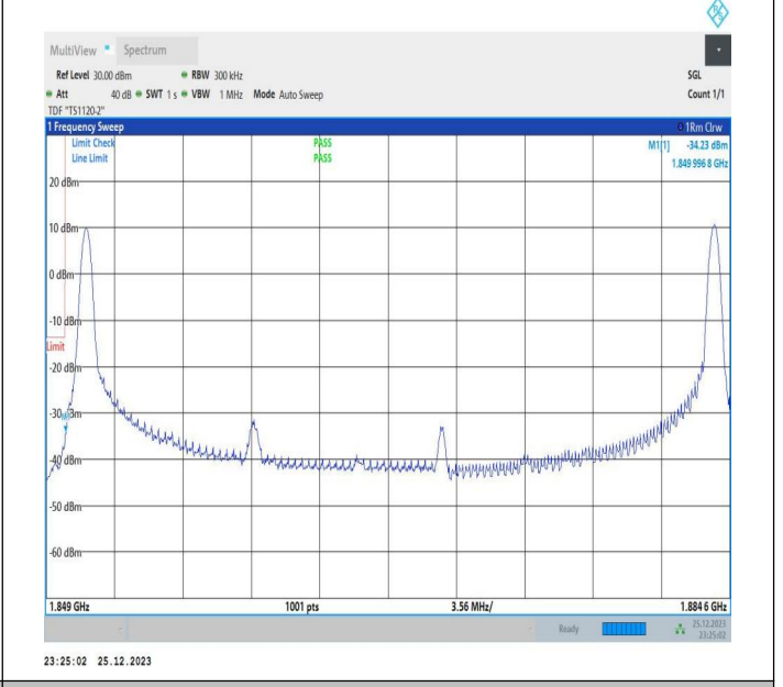
20MHz-15MHz_64QAM@64QAM-64QAM@64QAM_18700-18871_1RB#0@100RB#0-1RB#74@75RB#0
