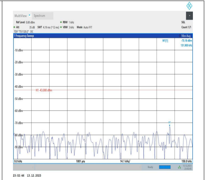
2-2-5MHz-20MHz-16QAM-16QAM-18808-18925-1RB#0-0RB#0-0-0.009~0.15MHz-PASS
