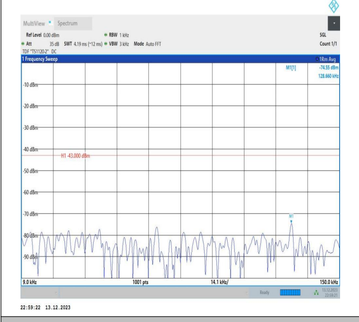
2-2-5MHz-20MHz-QPSK-QPSK-18633-18750-25RB#0-100RB #0-0.009~0.15MHz-PASS
