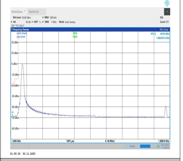
20MHz-20MHz_QPSK@QPSK-QPSK@QPSK_18700-18898_1RB#0@100RB#0-0RB#0@100RB#0
