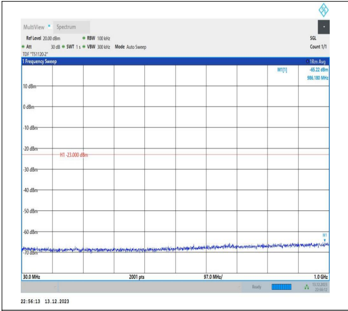
2-2-5MHz-20MHz-QPSK-QPSK-18633-18750-1RB#24-0RB#0 -30~1000MHz-PASS
