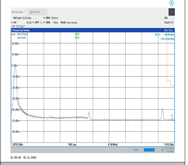
20MHz-20MHz_QPSK@QPSK-QPSK@QPSK_18902-19100_1RB#0@100RB#0-0RB#0@100RB#0
