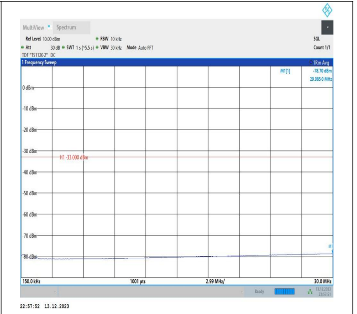
2-2-5MHz-20MHz-QPSK-QPSK-18633-18750-1RB#0-1RB#99 -0.15~30MHz-PASS
