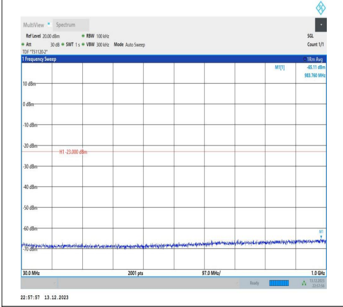
2-2-5MHz-20MHz-QPSK-QPSK-18633-18750-1RB#0-1RB#99 -30~1000MHz-PASS
