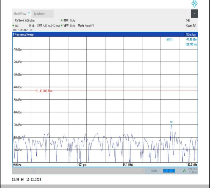
2-2-5MHz-20MHz-16QAM-16QAM-18633-18750-1RB#24-0RB #0-0.009~0.15MHz-PASS
