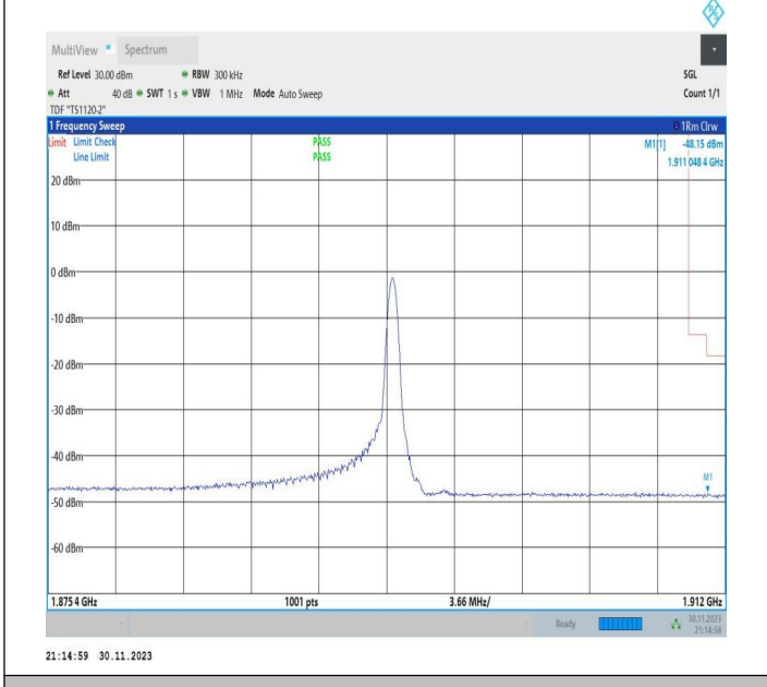
20MHz-15MHz_QPSK@QPSK-QPSK@QPSK_18951-19122_1RB#99@100RB#0-0RB#0@75RB#0
