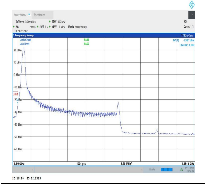
20MHz-15MHz_64QAM@64QAM-64QAM@64QAM_18700-18871_1RB#0@100RB#0-0RB#0@75RB#0
