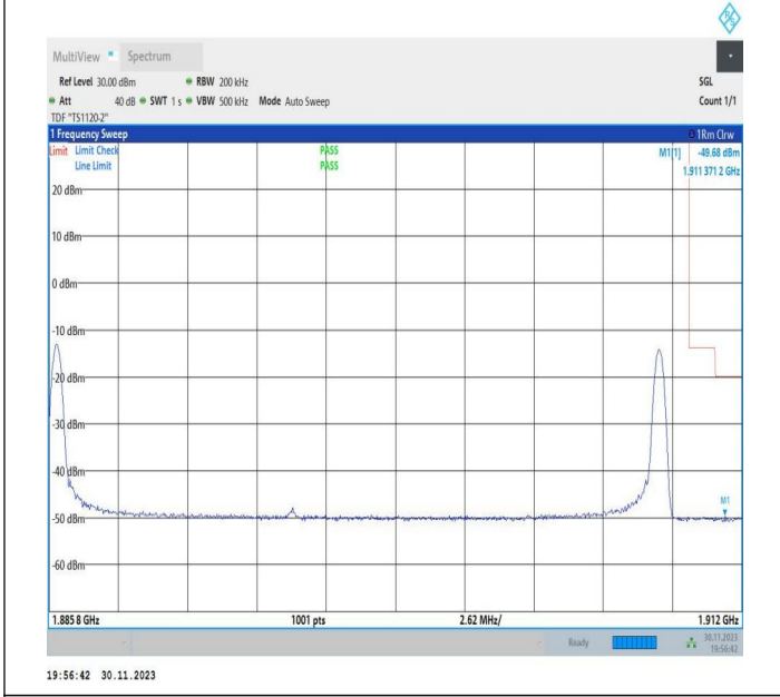
20MHz-5MHz_16QAM@16QAM-16QAM@16QAM_19050-19167_1RB#0@100RB#0-1RB#24@25RB#0
