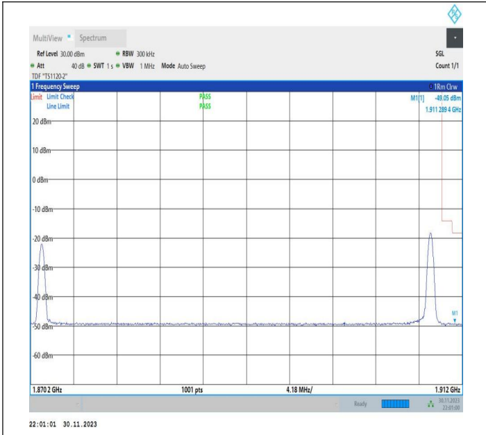
20MHz-20MHz_QPSK@QPSK-QPSK@QPSK_18902-19100_1RB#0@100RB#0-1RB#99@100RB#0
