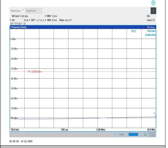
2-2-5MHz-20MHz-QPSK-QPSK-18633-18750-25RB#0-100RB #0-0.15~30MHz-PASS
