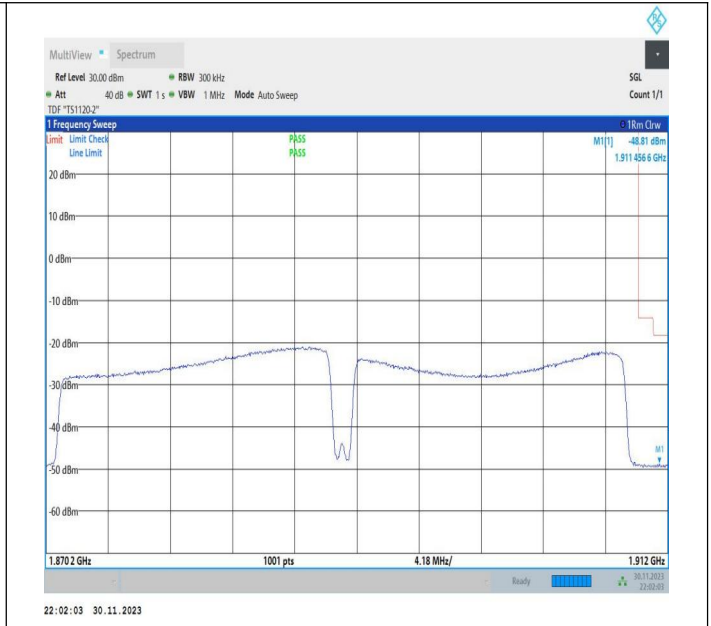
20MHz-20MHz_16QAM@16QAM-16QAM@16QAM_18902-19100_100RB#0@100RB#0-100RB#0@100RB#0
