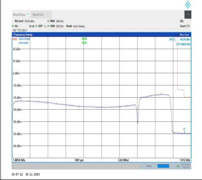
20MHz-5MHz_QPSK@QPSK-QPSK@QPSK_19050-19167_100RB#0@100RB#0-25RB#0@25RB#0
