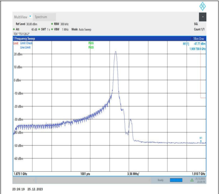
20MHz-15MHz_64QAM@64QAM-64QAM@64QAM_18951-19122_1RB#99@100RB#0-0RB#0@75RB#0
