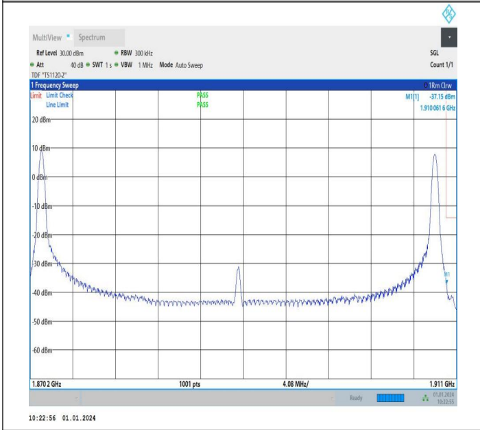
20MHz-20MHz_64QAM@64QAM-64QAM@64QAM_18902-19100_1RB#0@100RB#0-1RB#99@100RB#0
