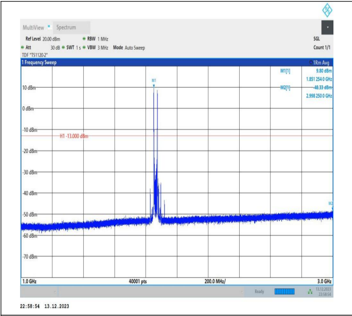
2-2-5MHz-20MHz-16QAM-16QAM-18633-18750-1RB#0-1RB# 99-1000~3000MHz-PASS
