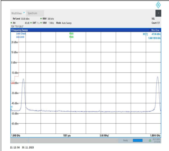
20MHz-15MHz_16QAM@16QAM-16QAM@16QAM_18700-18871_1RB#0@100RB#0-1RB#74@75RB#0
