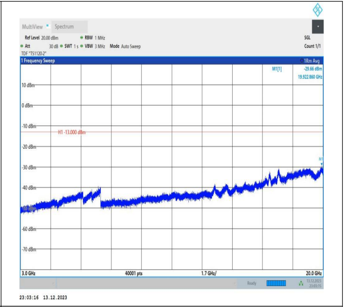
2-2-5MHz-20MHz-16QAM-16QAM-18808-18925-1RB#0-0RB# 0-3000~20000MHz-PASS
