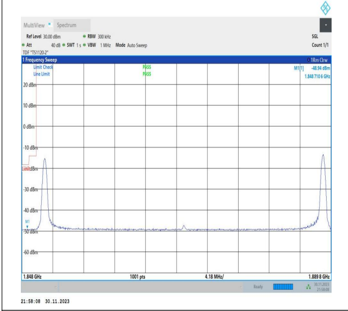
20MHz-20MHz_16QAM@16QAM-16QAM@16QAM_18700-18898_1RB#0@100RB#0-1RB#99@100RB#0
