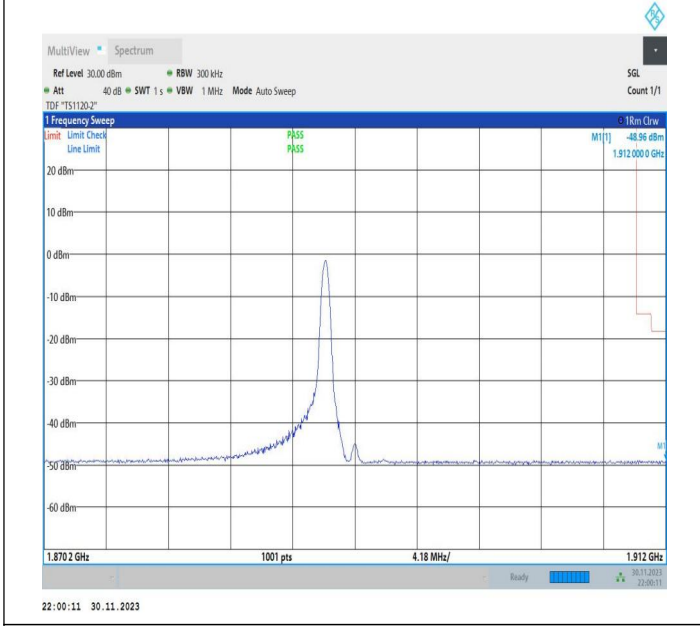
20MHz-20MHz_QPSK@QPSK-QPSK@QPSK_18902-19100_1RB#99@100RB#0-0RB#0@100RB#0
