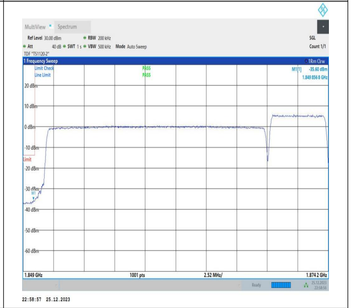
20MHz-5MHz_64QAM@64QAM-64QAM@64QAM_18700-18817_100RB#0@100RB#0-25RB#0@25RB#0
