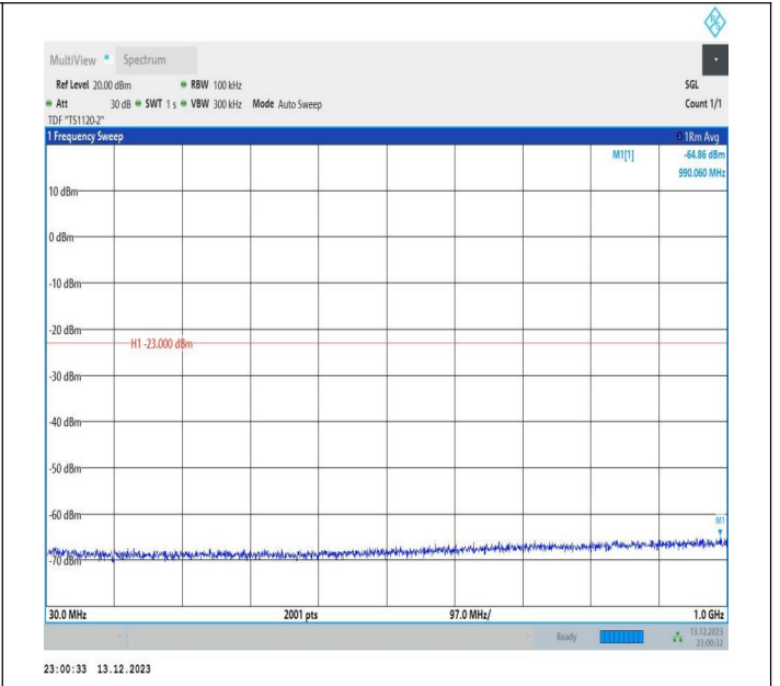
2-2-5MHz-20MHz-16QAM-16QAM-18633-18750-25RB#0-100 RB#0-30~1000MHz-PASS
