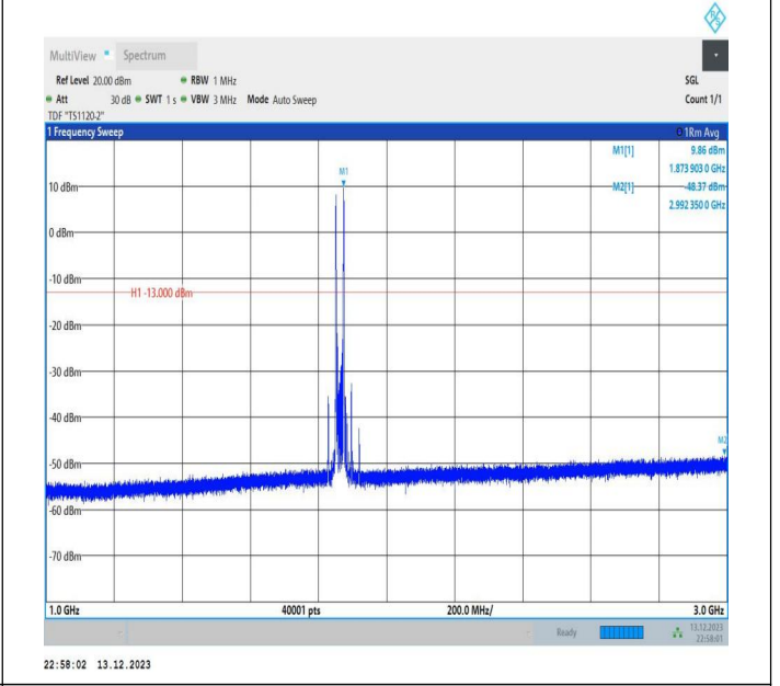
2-2-5MHz-20MHz-QPSK-QPSK-18633-18750-1RB#0-1RB#99 -1000~3000MHz-PASS
