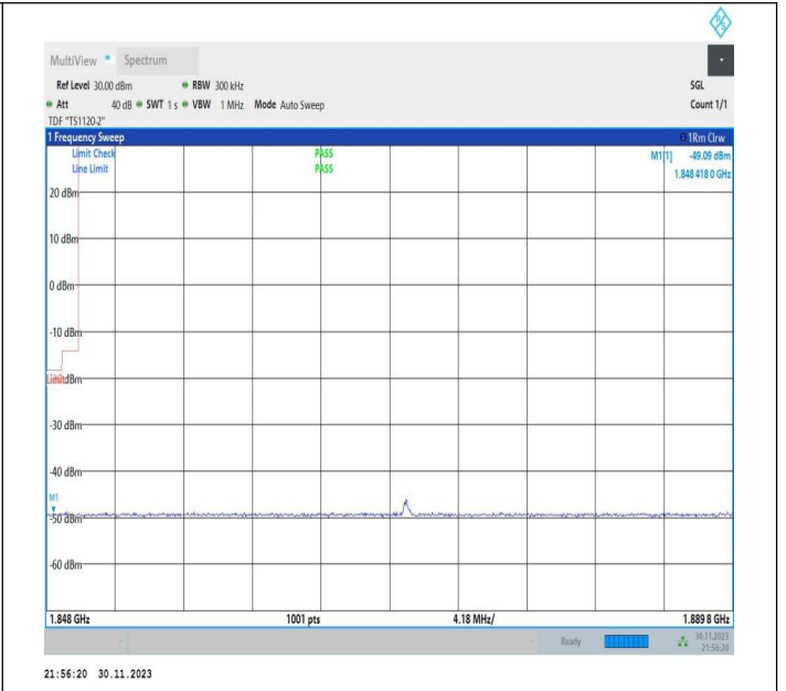
20MHz-20MHz_QPSK@QPSK-QPSK@QPSK_18700-18898_1RB#99@100RB#0-0RB#0@100RB#0
