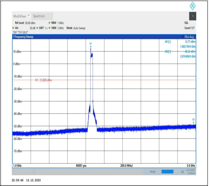
2-2-5MHz-20MHz-QPSK-QPSK-18633-18750-25RB#0-100RB #0-1000~3000MHz-PASS
