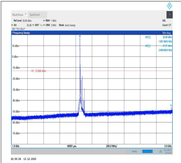
2-2-5MHz-20MHz-16QAM-16QAM-18633-18750-1RB#0-0RB# 0-1000~3000MHz-PASS
