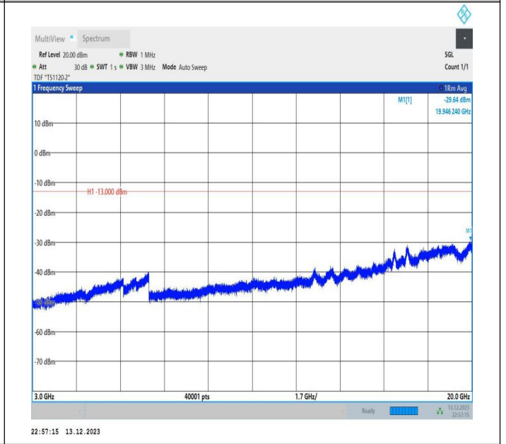
2-2-5MHz-20MHz-16QAM-16QAM-18633-18750-1RB#24-0RB #0-3000~20000MHz-PASS
