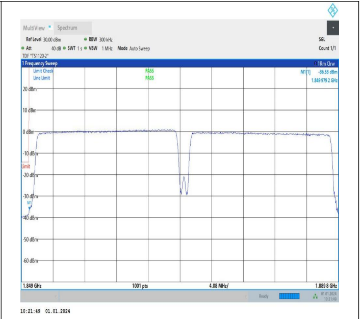
20MHz-20MHz_64QAM@64QAM-64QAM@64QAM_18700-18898_100RB#0@100RB#0-100RB#0@100RB#0
