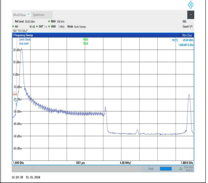
20MHz-20MHz_64QAM@64QAM-64QAM@64QAM_18700-18989_1RB#0@100RB#0-0RB#0@100RB#0
