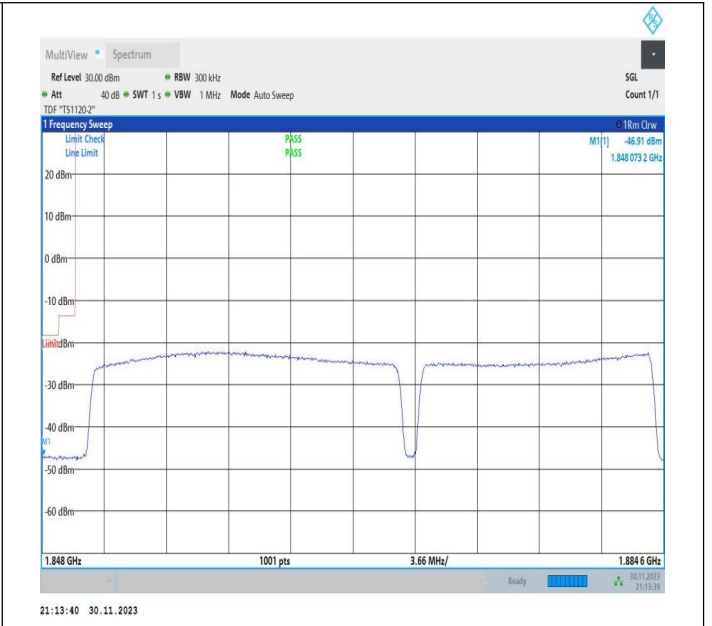
20MHz-15MHz_16QAM@16QAM-16QAM@16QAM_18700-18871_100RB#0@100RB#0-75RB#0@75RB#0
