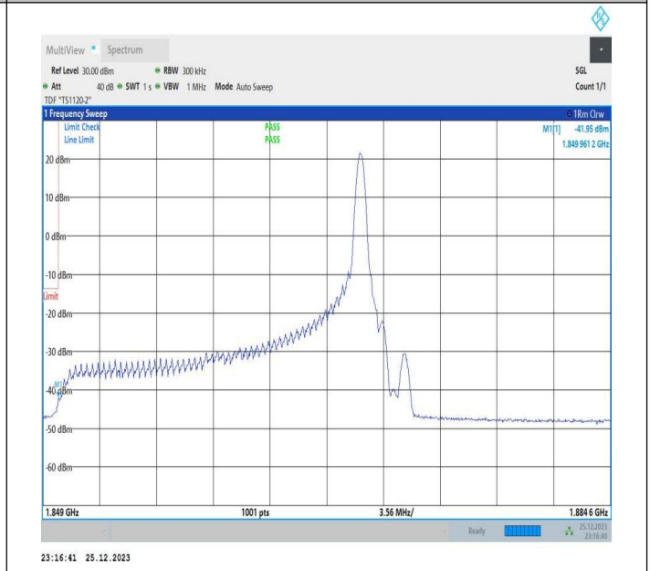
20MHz-15MHz_64QAM@64QAM-64QAM@64QAM_18700-18871_1RB#99@100RB#0-0RB#0@75RB#0
