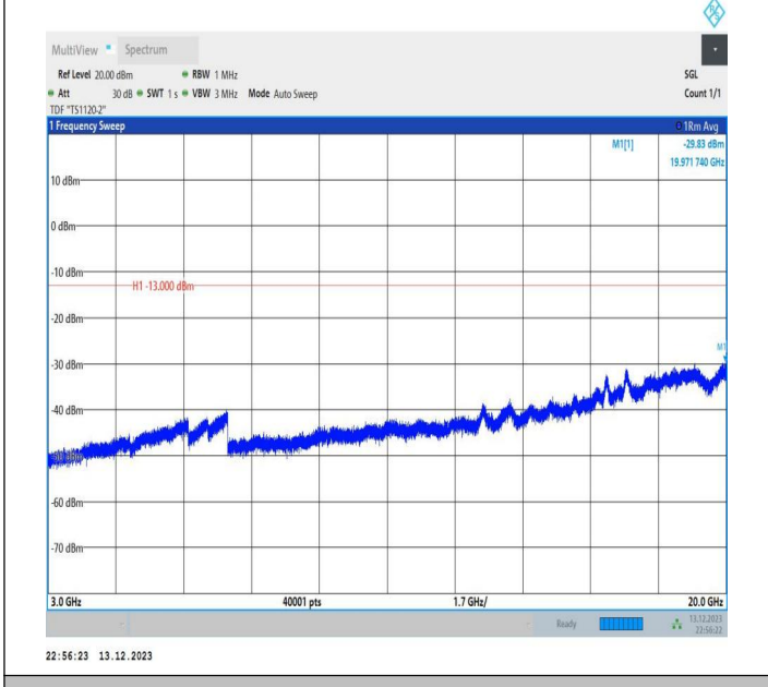
2-2-5MHz-20MHz-QPSK-QPSK-18633-18750-1RB#24-0RB#0 -3000~20000MHz-PASS
