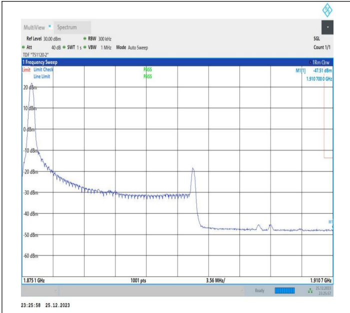
20MHz-15MHz_64QAM@64QAM-64QAM@64QAM_18951-19122_1RB#0@100RB#0-0RB#0@75RB#0
