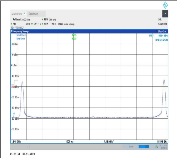
20MHz-20MHz_QPSK@QPSK-QPSK@QPSK_18700-18898_1RB#0@100RB#0-1RB#99@100RB#0
