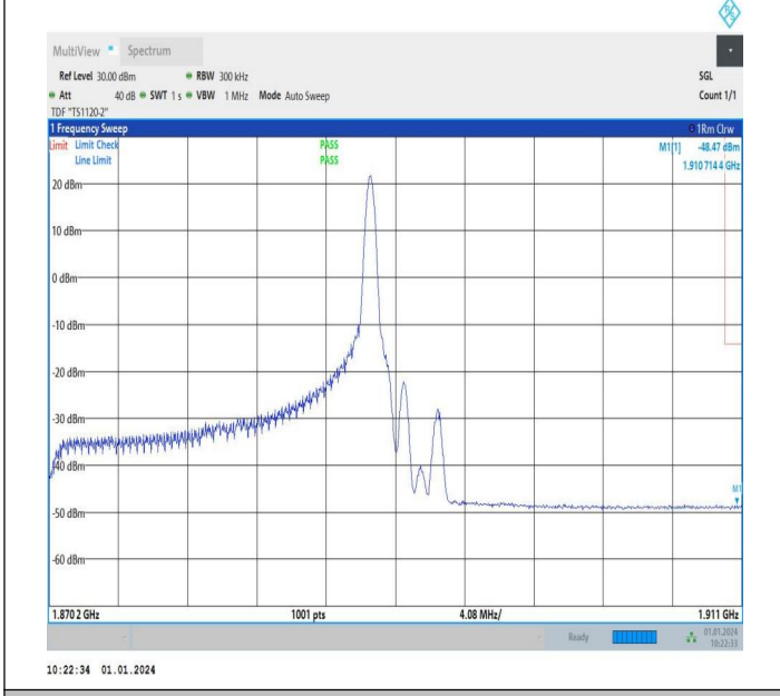
20MHz-20MHz_64QAM@64QAM-64QAM@64QAM_18902-19100_1RB#99@100RB#0-0RB#0@100RB#0
