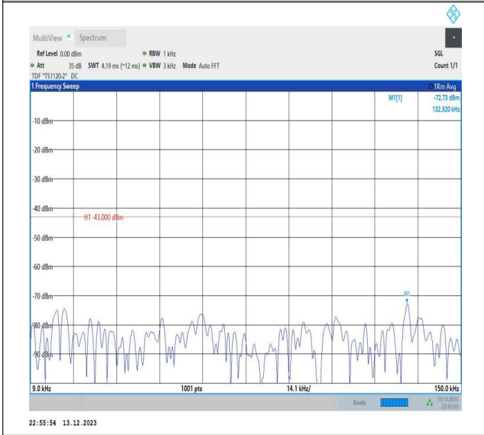
2-2-5MHz-20MHz-QPSK-QPSK-18633-18750-1RB#24-0RB#0 -0.009~0.15MHz-PASS
