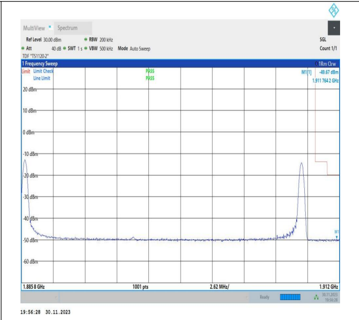
20MHz-5MHz_QPSK@QPSK-QPSK@QPSK_19050-19167_1RB#0@100RB#0-1RB#24@25RB#0
