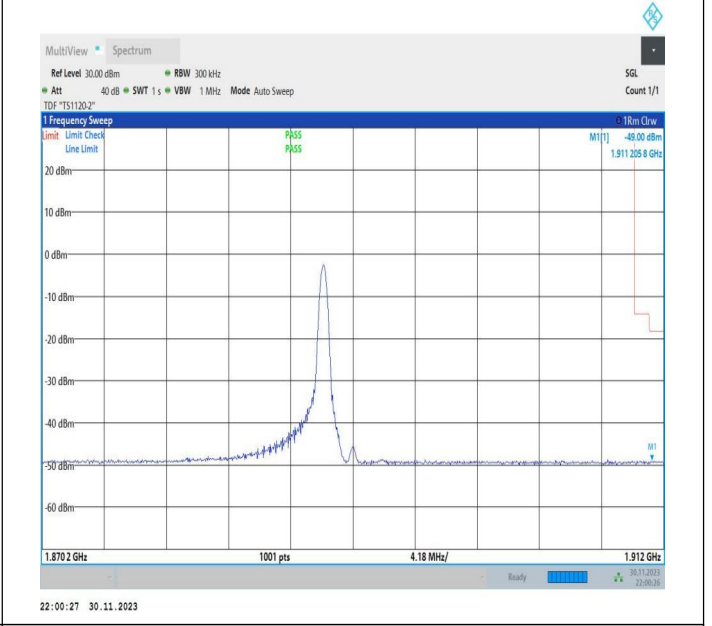
20MHz-20MHz_16QAM@16QAM-16QAM@16QAM_18902-19100_1RB#99@100RB#0-0RB#0@100RB#0
