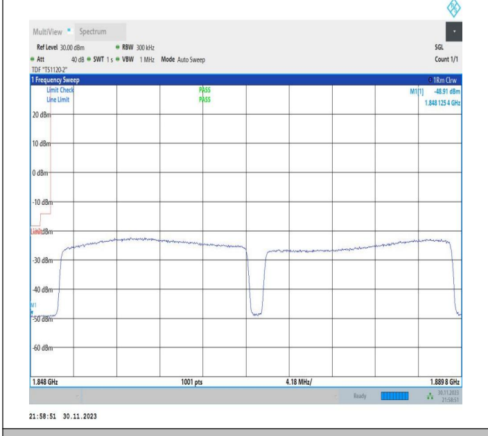
20MHz-20MHz_16QAM@16QAM-16QAM@16QAM_18700-1898_100RB#0@100RB#0-100RB#0@100RB#0
