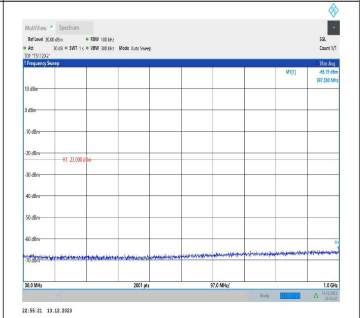
2-2-5MHz-20MHz-16QAM-16QAM-18633-18750-1RB#0-0RB#0-0-30~1000MHz-PASS
