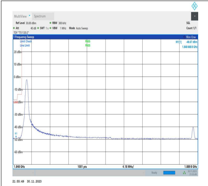
20MHz-20MHz_16QAM@16QAM-16QAM@16QAM_18700-18989_1RB#0@100RB#0-0RB#0@100RB#0
