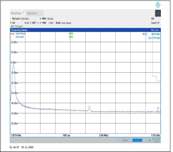
20MHz-15MHz_16QAM@16QAM-16QAM@16QAM_18951-19122_1RB#0@100RB#0-0RB#0@75RB#0
