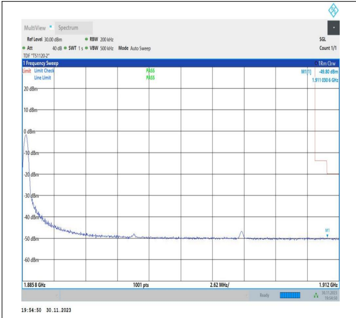
20MHz-5MHz_QPSK@QPSK-QPSK@QPSK_19050-19167_1 RB#0@100RB#0-0RB#0@25RB#0
