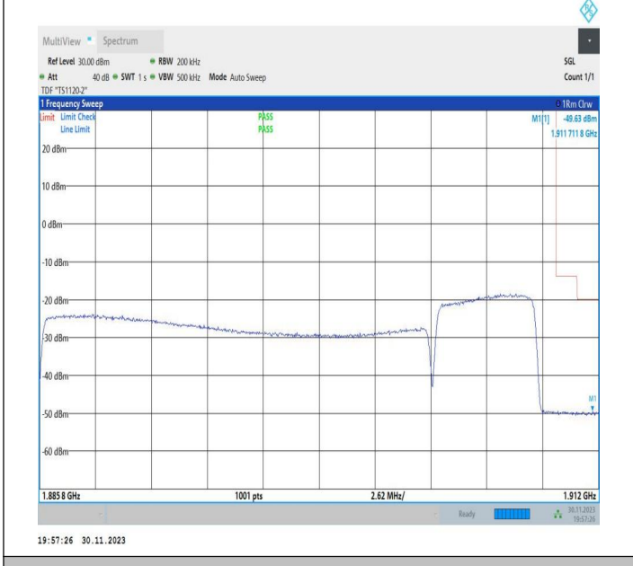
20MHz-5MHz_16QAM@16QAM-16QAM@16QAM_19050-19167_100RB#0@100RB#0-25RB#0@25RB#0
