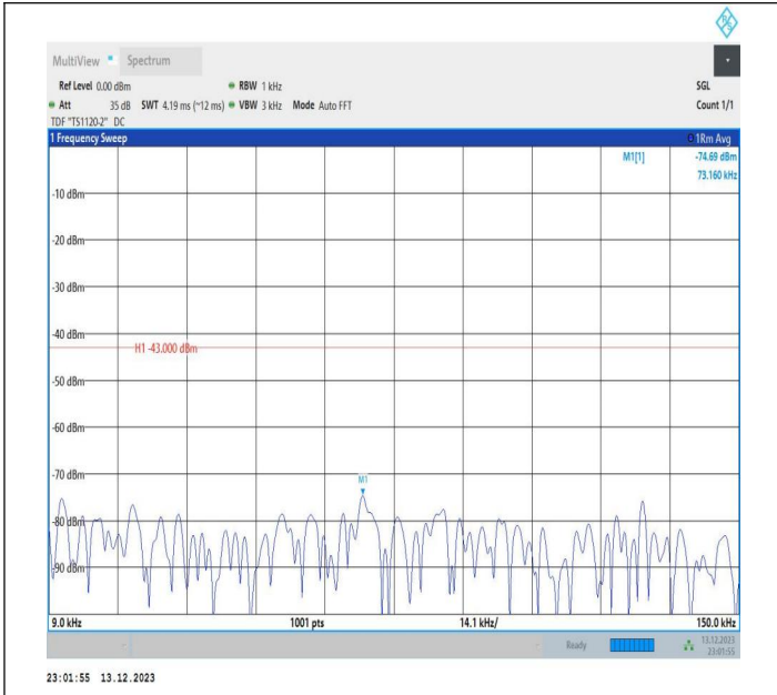
2-2-5MHz-20MHz-QPSK-QPSK-18808-18925-1RB#0-0RB#0-0.009~0.15MHz-PASS
