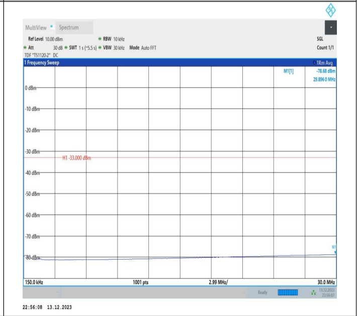
2-2-5MHz-20MHz-QPSK-QPSK-18633-18750-1RB#24-0RB#0 -0.15~30MHz-PASS
