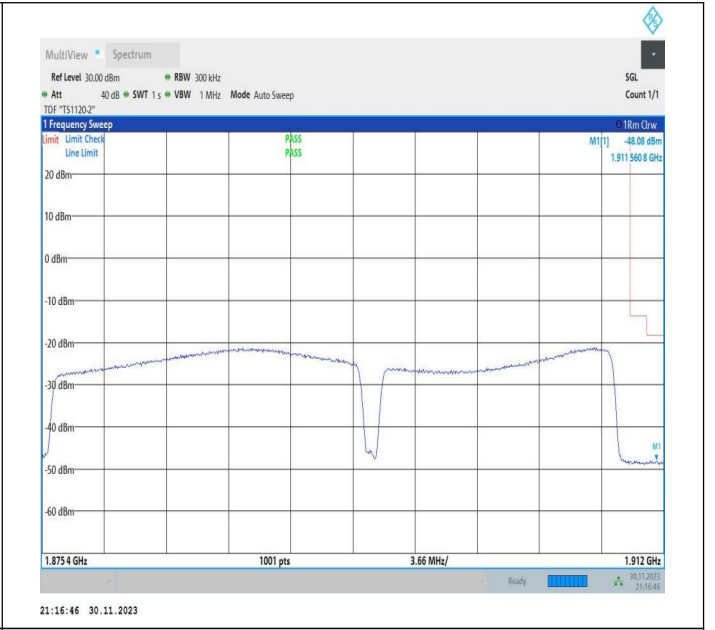
20MHz-15MHz_16QAM@16QAM-16QAM@16QAM_18951-19122_100RB#0@100RB#0-75RB#0@75RB#0
