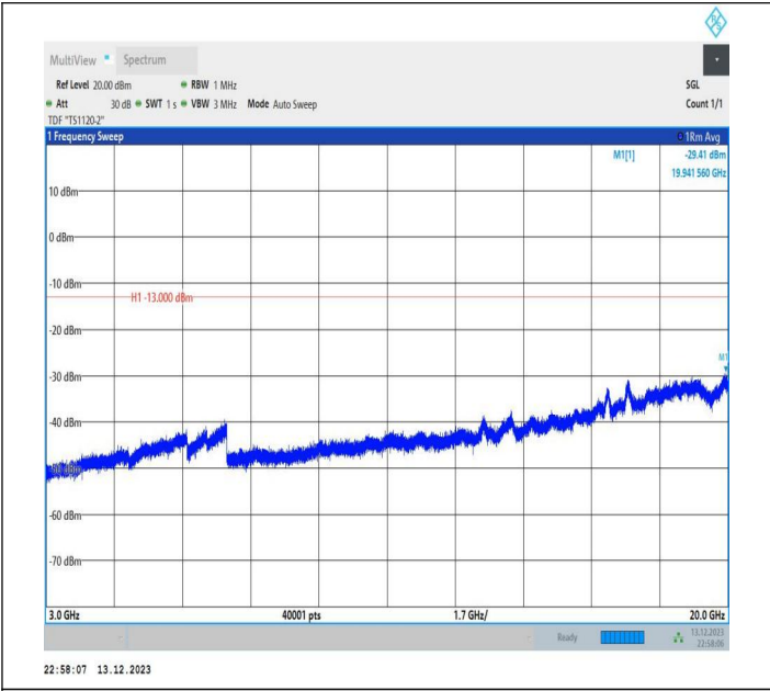
2-2-5MHz-20MHz-QPSK-QPSK-18633-18750-1RB#0-1RB#99 -3000~20000MHz-PASS
