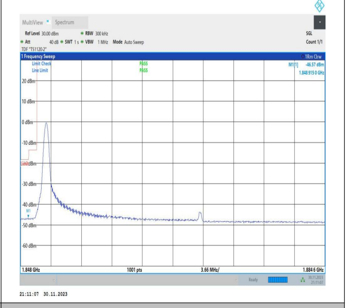
20MHz-15MHz_QPSK@QPSK-QPSK@QPSK_18700-18871_1RB#0@100RB#0-0RB#0@75RB#0
