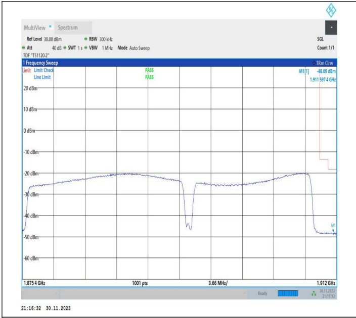
20MHz-15MHz_QPSK@QPSK-QPSK@QPSK_18951-19122_100RB#0@100RB#0-75RB#0@75RB#0
