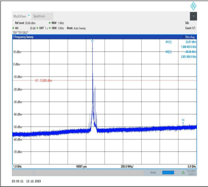
2-2-5MHz-20MHz-16QAM-16QAM-18808-18925-1RB#0-0RB# 0-1000~3000MHz-PASS
