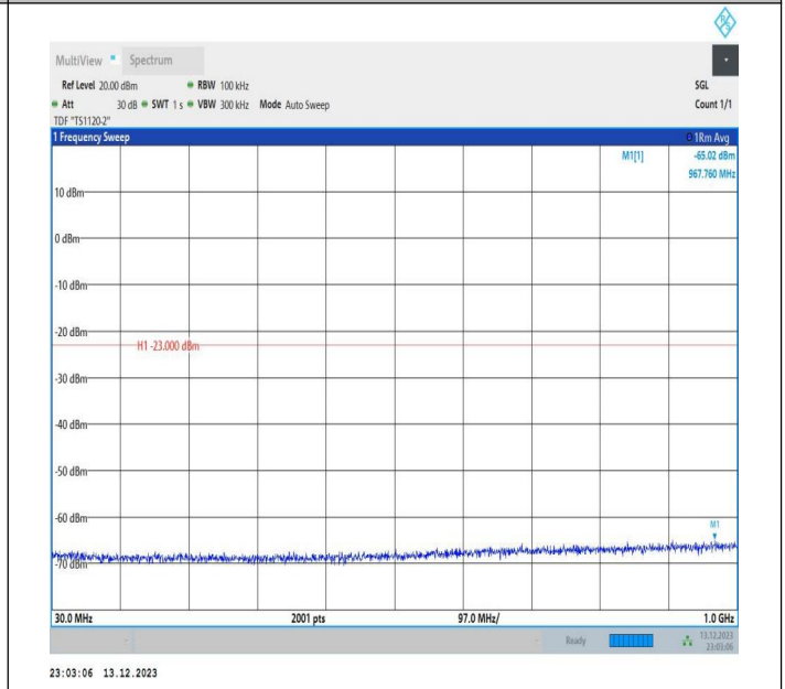
2-2-5MHz-20MHz-16QAM-16QAM-18808-18925-1RB#0-0RB#0-0-30~1000MHz-PASS
