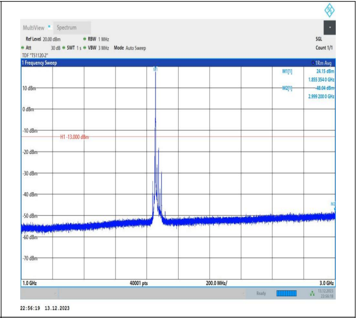
2-2-5MHz-20MHz-QPSK-QPSK-18633-18750-1RB#24-0RB#0 -1000~3000MHz-PASS
