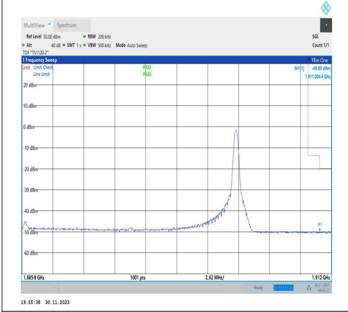
20MHz-5MHz_QPSK@QPSK-QPSK@QPSK_19050-19167_1 RB#99@100RB#0-0RB#0@25RB#0
