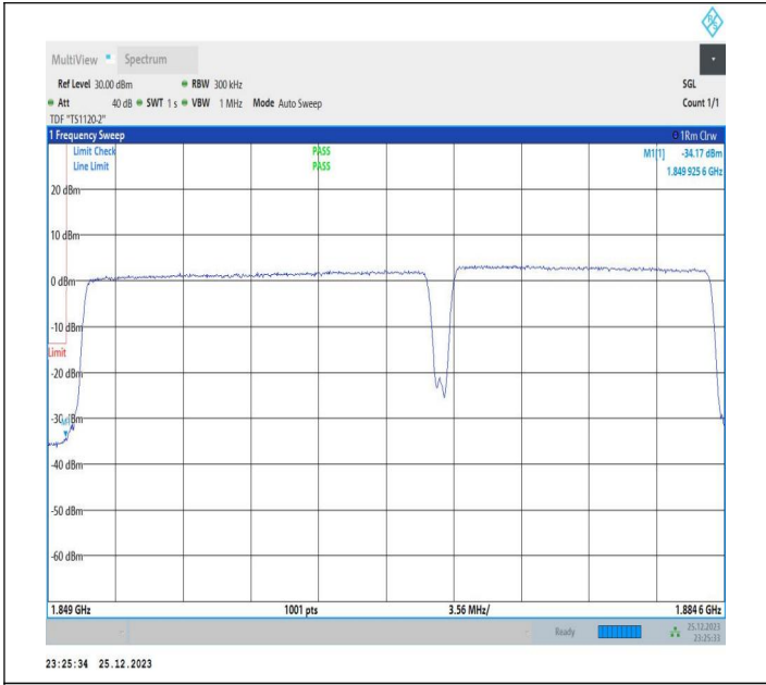
20MHz-15MHz_64QAM@64QAM-64QAM_18700-18871_100RB#0@100RB#0-75RB#0@75RB#0
