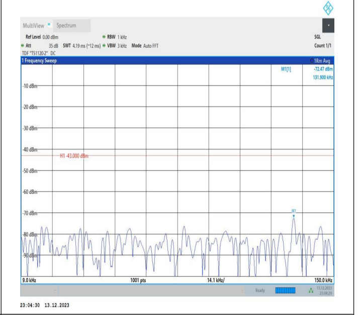
2-2-5MHz-20MHz-16QAM-16QAM-18808-18925-1RB#24-0RB #0-0.009~0.15MHz-PASS
