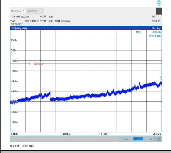
2-2-5MHz-20MHz-QPSK-QPSK-18633-18750-25RB#0-100RB #0-3000~20000MHz-PASS
