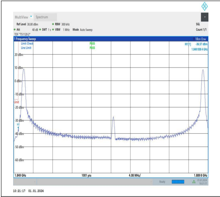
20MHz-20MHz_64QAM@64QAM-64QAM@64QAM_18700-1898_1RB#0@100RB#0-1RB#99@100RB#0
