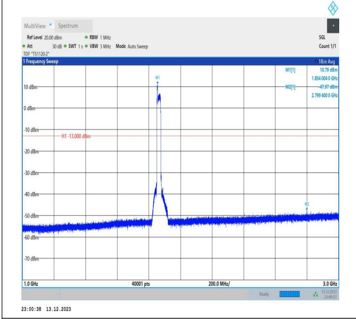
2-2-5MHz-20MHz-16QAM-16QAM-18633-18750-25RB#0-100 RB#0-1000~3000MHz-PASS
