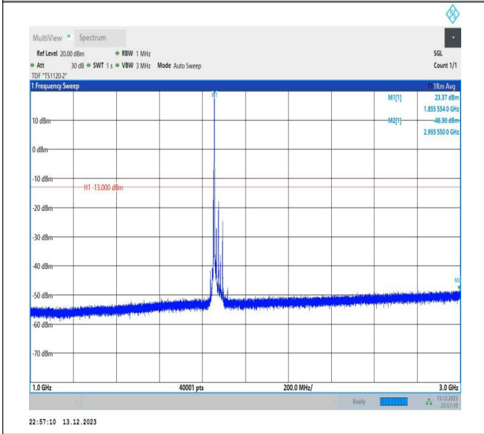
2-2-5MHz-20MHz-16QAM-16QAM-18633-18750-1RB#24-0RB #0-1000~3000MHz-PASS
