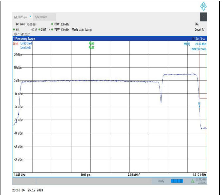
20MHz-5MHz_64QAM@64QAM-64QAM@64QAM_19050-19167_100RB#0@100RB#0-25RB#0@25RB#0
