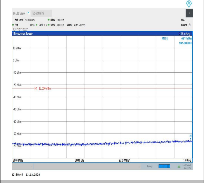
2-2-5MHz-20MHz-16QAM-16QAM-18633-18750-1RB#0-1RB# 99-30~1000MHz-PASS
