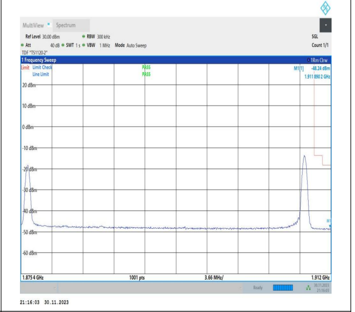
20MHz-15MHz_16QAM@16QAM-16QAM@16QAM_18951-19122_1RB#0@100RB#0-1RB#74@75RB#0
