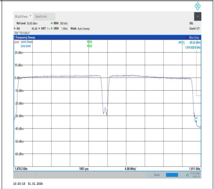
20MHz-20MHz_64QAM@64QAM-64QAM@64QAM_18902-19100_100RB#0@100RB#0-100RB#0@100RB#0
