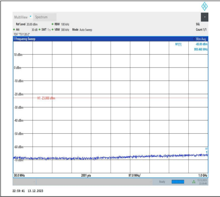
2-2-5MHz-20MHz-QPSK-QPSK-18633-18750-25RB#0-100RB #0-30~1000MHz-PASS
