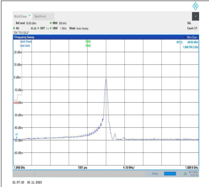
20MHz-20MHz_16QAM@16QAM-16QAM@16QAM_18700-18898_1RB#99@100RB#0-0RB#0@100RB#0
