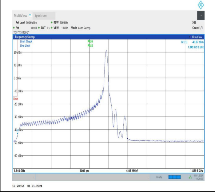
20MHz-20MHz_64QAM@64QAM-64QAM@64QAM_18700-18898_1RB#99@100RB#0-0RB#0@100RB#0
