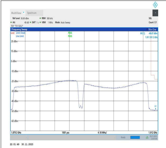
20MHz-20MHz_QPSK@QPSK-QPSK@QPSK_18902-19100_100RB#0@100RB#0-100RB#0@100RB#0
