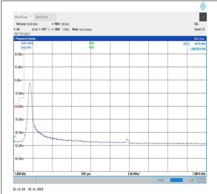
20MHz-15MHz_16QAM@16QAM-16QAM@16QAM_18700-18871_1RB#0@100RB#0-0RB#0@75RB#0
