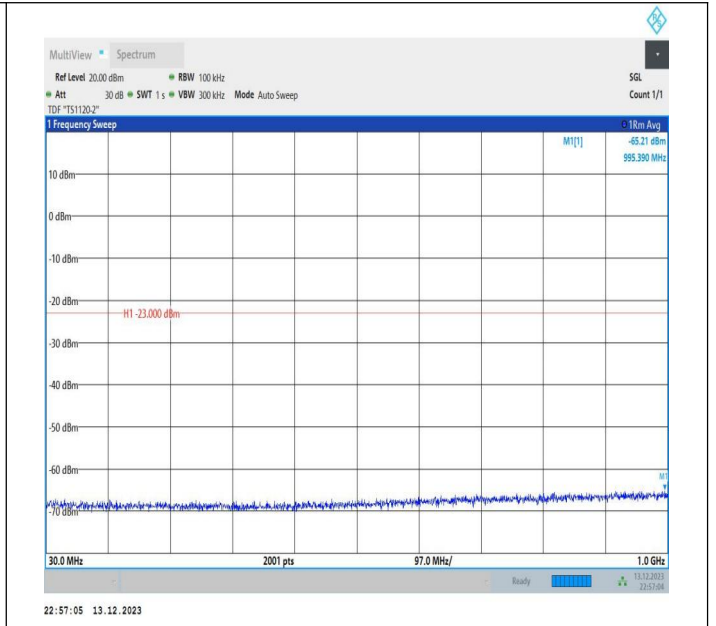
2-2-5MHz-20MHz-16QAM-16QAM-18633-18750-1RB#24-0RB #0-30~1000MHz-PASS
