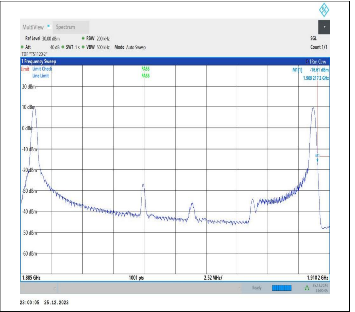
20MHz-5MHz_64QAM@64QAM-64QAM@64QAM_19050-19167_1RB#0@100RB#0-1RB#24@25RB#0
