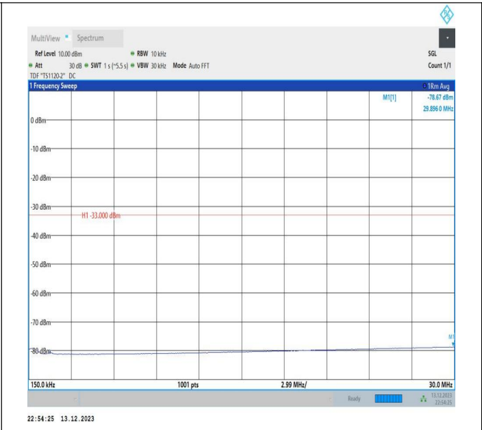
2-2-5MHz-20MHz-QPSK-QPSK-18633-18750-1RB#0-0RB#0-0.15~30MHz-PASS
