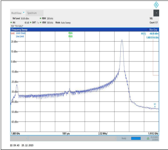
20MHz-5MHz_64QAM@64QAM-64QAM@64QAM_19050-19167_1RB#99@100RB#0-0RB#0@25RB#0
