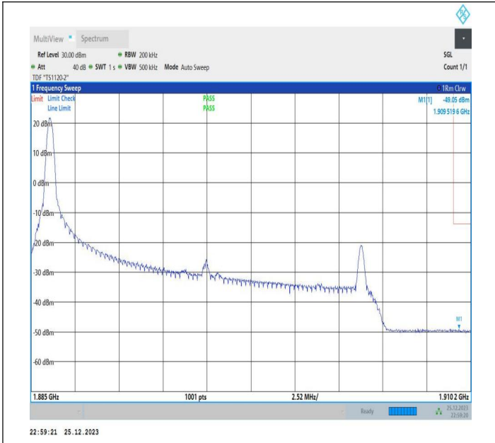
20MHz-5MHz_64QAM@64QAM-64QAM@64QAM_19050-19167_1RB#0@100RB#0-0RB#0@25RB#0
