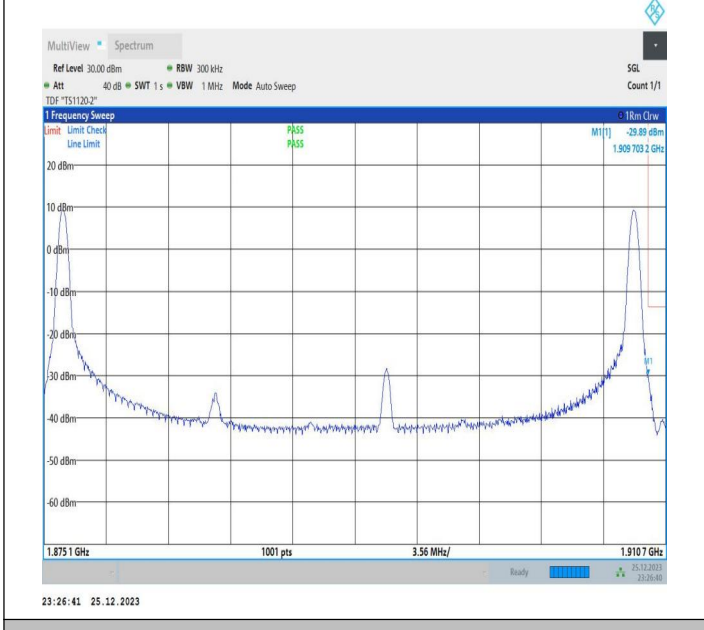
20MHz-15MHz_64QAM@64QAM-64QAM@64QAM_18951-19122_1RB#0@100RB#0-1RB#74@75RB#0
