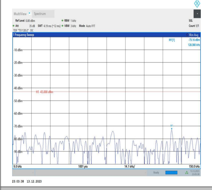
2-2-5MHz-20MHz-QPSK-QPSK-18808-18925-1RB#24-0RB#0 -0.009~0.15MHz-PASS
