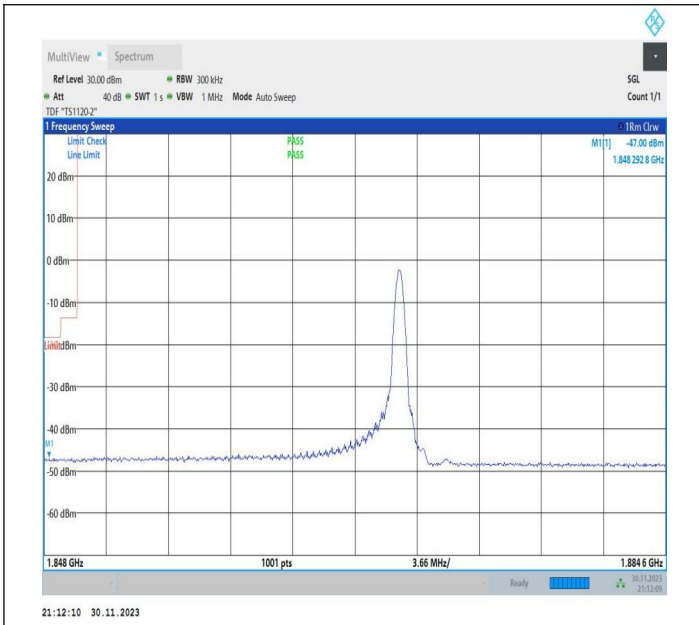
20MHz-15MHz_16QAM@16QAM-16QAM@16QAM_18700-18871_1RB#99@100RB#0-0RB#0@75RB#0
