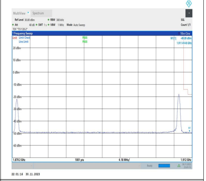
20MHz-20MHz_16QAM@16QAM-16QAM@16QAM_18902-19100_1RB#0@100RB#0-1RB#99@100RB#0
