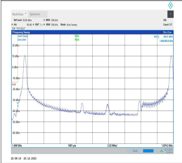
20MHz-5MHz_64QAM@64QAM-64QAM@64QAM_18700-18817_1RB#0@100RB#0-1RB#24@25RB#0
