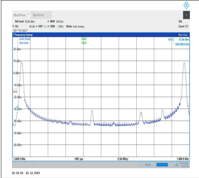
15MHz-20MHz_64QAM@64QAM-64QAM@64QAM_18678-18849_1RB#0@75RB#0-1RB#99@100RB#0
