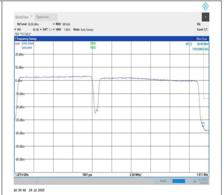
15MHz-20MHz_64QAM@64QAM-64QAM@64QAM_18929-19100_75RB#0@75RB#0-100RB#0@100RB#0
