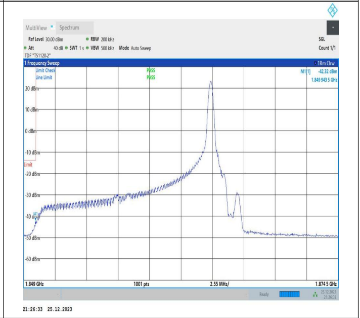
15MHz-10MHz_64QAM@64QAM-64QAM@64QAM_18675-18795_1RB#74@75RB#0-0RB#0@50RB#0
