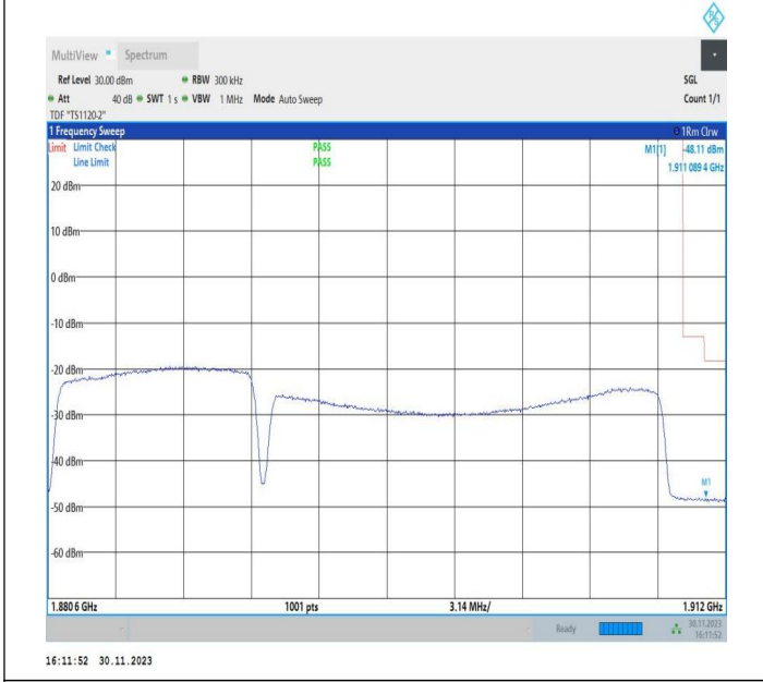
10MHz-20MHz_16QAM@16QAM-16QAM@16QAM_18956-19 100_50RB#0@50RB#0-100RB#0@100RB#0
