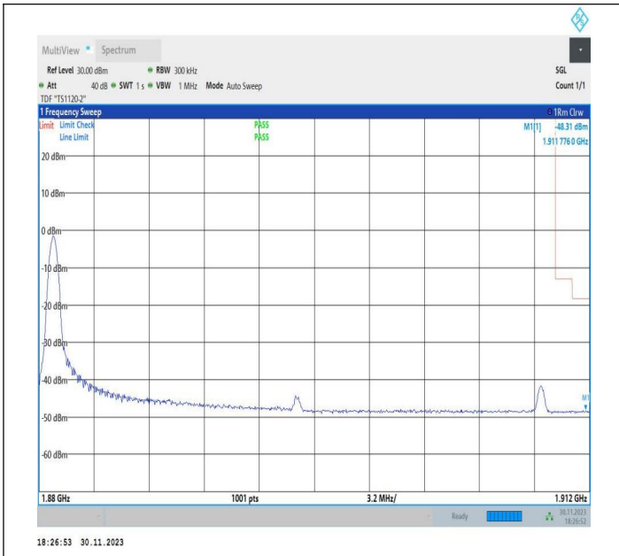
15MHz-15MHz_16QAM@16QAM-16QAM@16QAM_18975-19125_1RB#0@75RB#0-0RB#0@75RB#0
