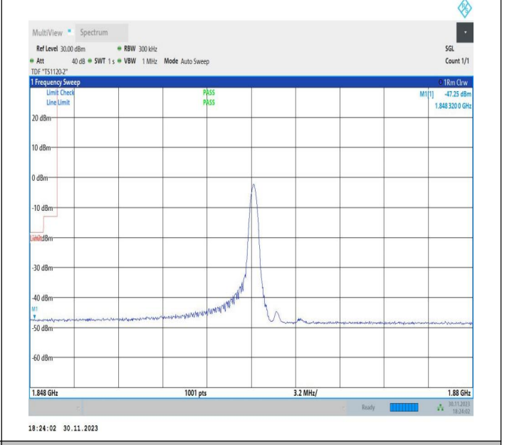
15MHz-15MHz_16QAM@16QAM-16QAM@16QAM_18675-18825_1RB#74@75RB#0-0RB#0@75RB#0
