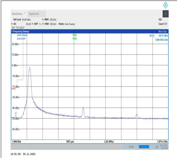
20MHz-5MHz_16QAM@16QAM-16QAM@16QAM_18700-18817_1RB#0@100RB#0-0RB#0@25RB#0
