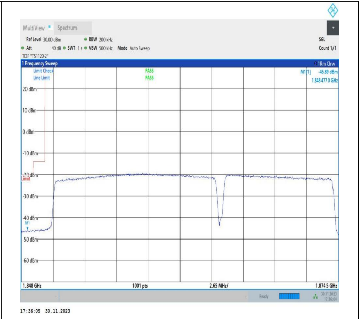
15MHz-10MHz_QPSK@QPSK-QPSK@QPSK_18675-18795_75RB#0@75RB#0-50RB#0@50RB#0
