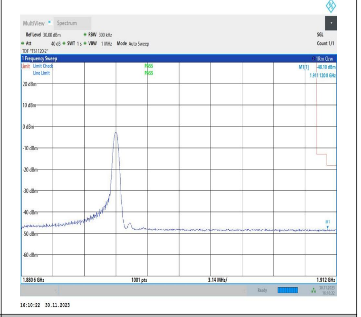
10MHz-20MHz_16QAM@16QAM-16QAM@16QAM_18956-19100_1RB#49@50RB#0-0RB#0@100RB#0
