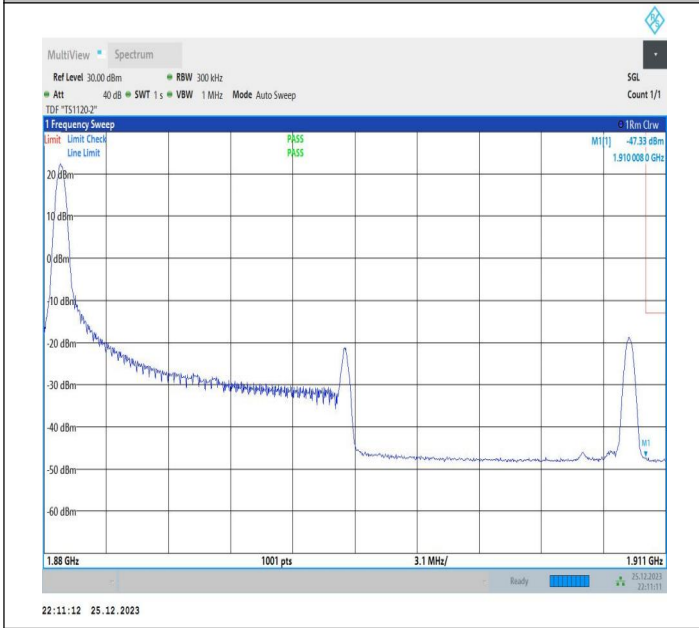
15MHz-15MHz_64QAM@64QAM-64QAM@64QAM_18975-19125_1RB#0@75RB#0-0RB#0@75RB#0
