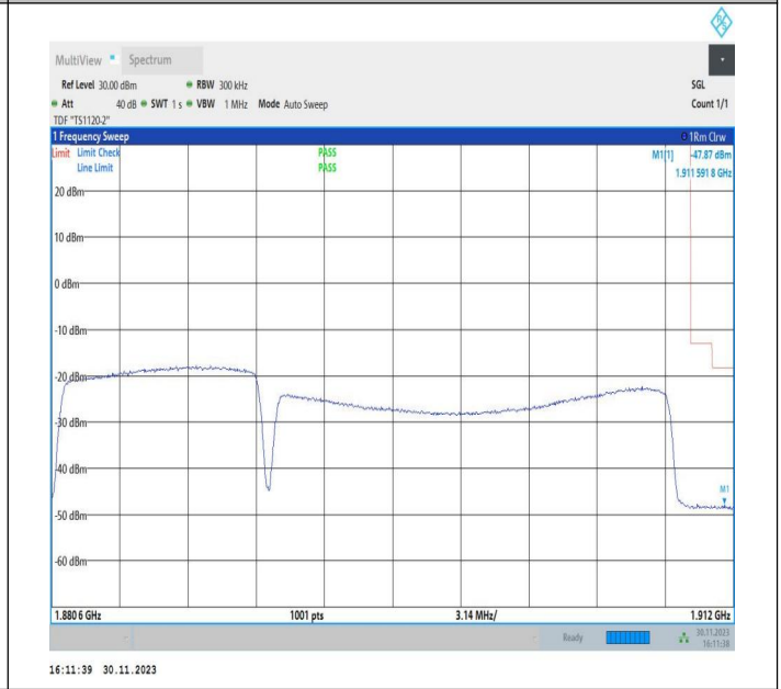
10MHz-20MHz_QPSK@QPSK-QPSK@QPSK_18956-19100_50RB#0@50RB#0-100RB#0@100RB#0
