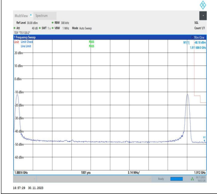
20MHz-10MHz_QPSK@QPSK-QPSK@QPSK_19001-19145_1RB#0@100RB#0-1RB#49@50RB#0
