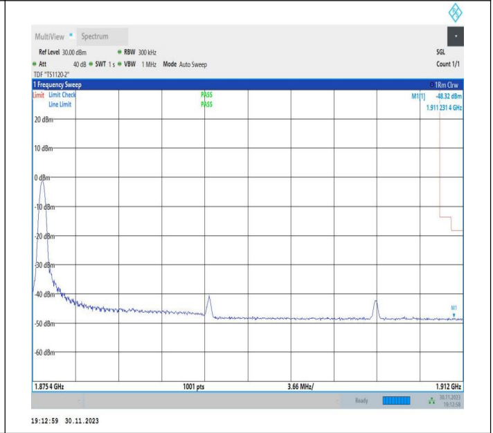
15MHz-20MHz_QPSK@QPSK-QPSK@QPSK_18929-19100_1RB#0@75RB#0-0RB#0@100RB#0
