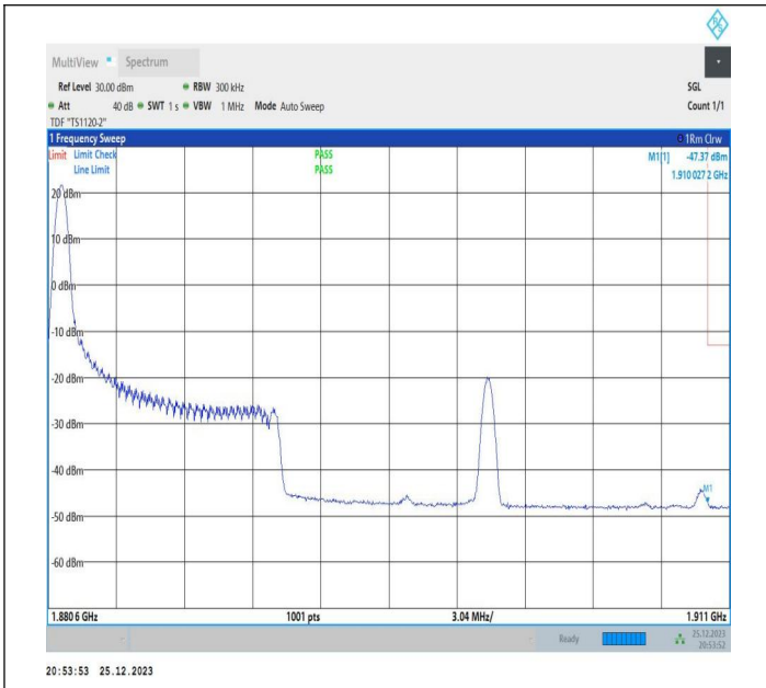
10MHz-20MHz_64QAM@64QAM-64QAM@64QAM_18956-19100_1RB#0@50RB#0-0RB#0@100RB#0
