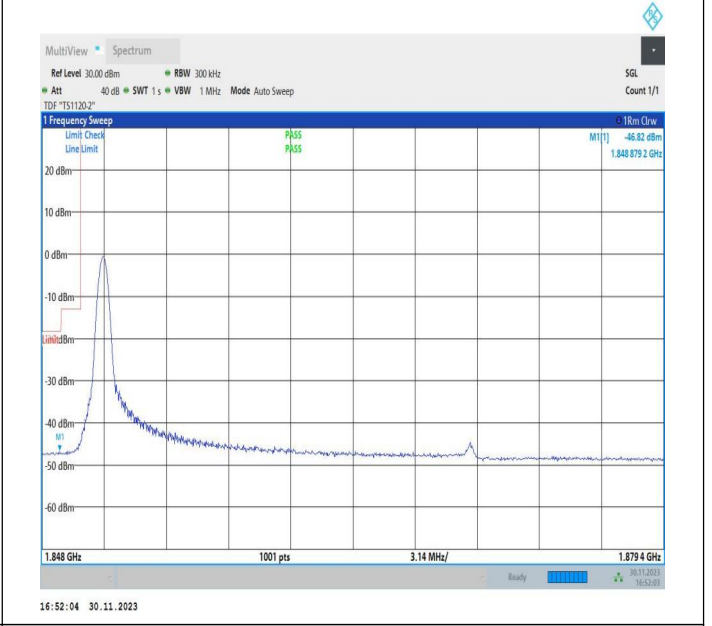
20MHz-10MHz_QPSK@QPSK-QPSK@QPSK_18700-18844_ 1RB#0@100RB#0-0RB#0@50RB#0
