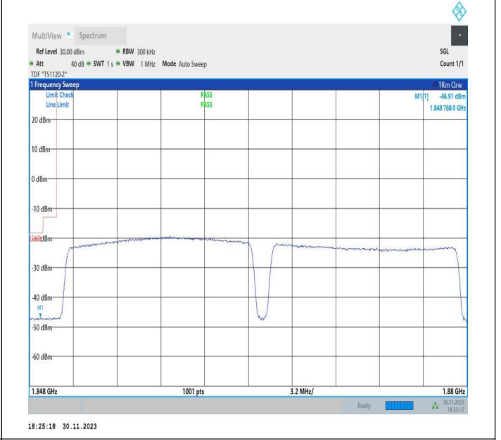
15MHz-15MHz_QPSK@QPSK-QPSK@QPSK_18675-18825_75RB#0@75RB#0-75RB#0@75RB#0
