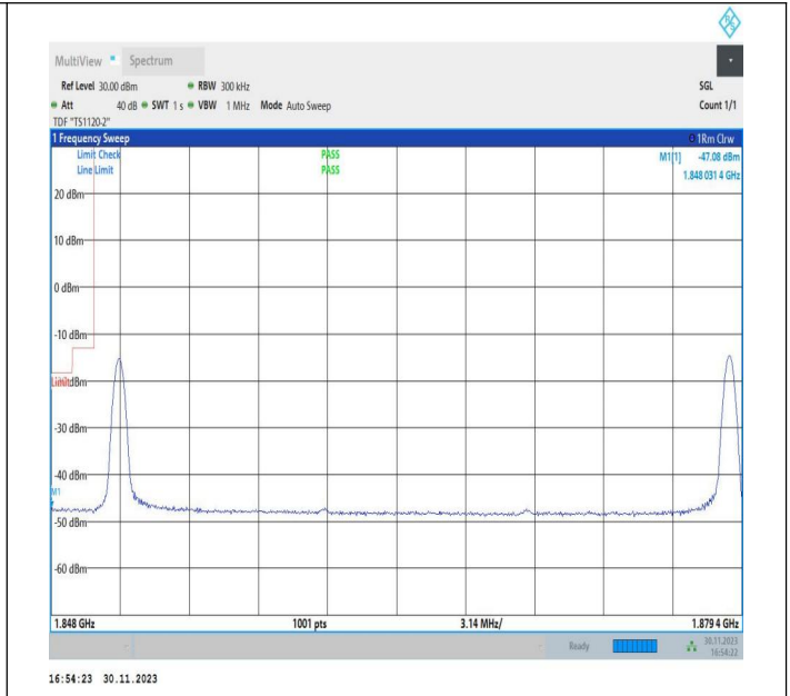
20MHz-10MHz_QPSK@QPSK-QPSK@QPSK_18700-18844_1RB#0@100RB#0-1RB#49@50RB#0
