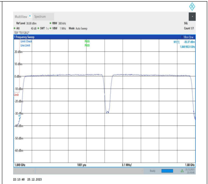
15MHz-15MHz_64QAM@64QAM-64QAM@64QAM_18675-18825_75RB#0@75RB#0-75RB#0@75RB#0
