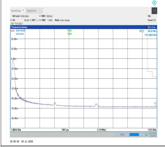
20MHz-10MHz_QPSK@QPSK-QPSK@QPSK_19001-19145_1RB#0@100RB#0-0RB#0@50RB#0
