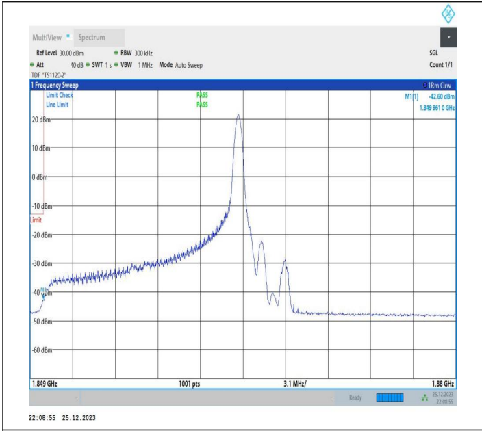
15MHz-15MHz_64QAM@64QAM-64QAM@64QAM_18675-18825_1RB#74@75RB#0-0RB#0@75RB#0
