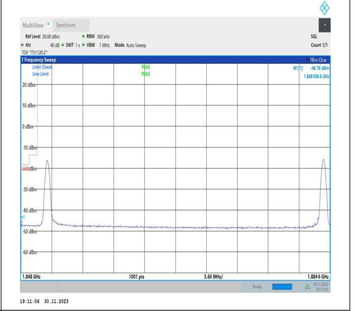
15MHz-20MHz_16QAM@16QAM-16QAM@16QAM_18678-18849_1RB#0@75RB#0-1RB#99@100RB#0
