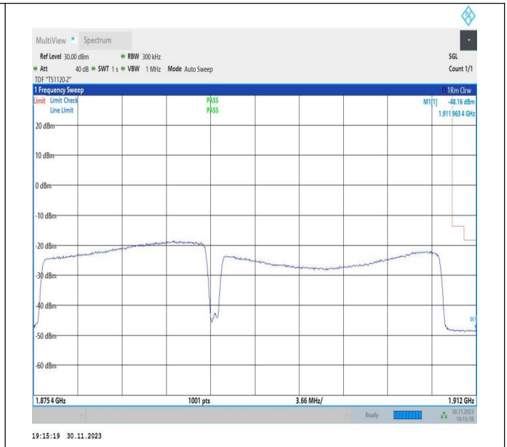
15MHz-20MHz_QPSK@QPSK-QPSK@QPSK_18929-19100_75RB#0@75RB#0-100RB#0@100RB#0
