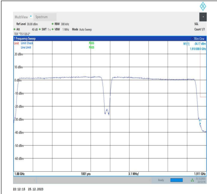
15MHz-15MHz_64QAM@64QAM-64QAM_18975-19125_75RB#0@75RB#0-75RB#0@75RB#0
