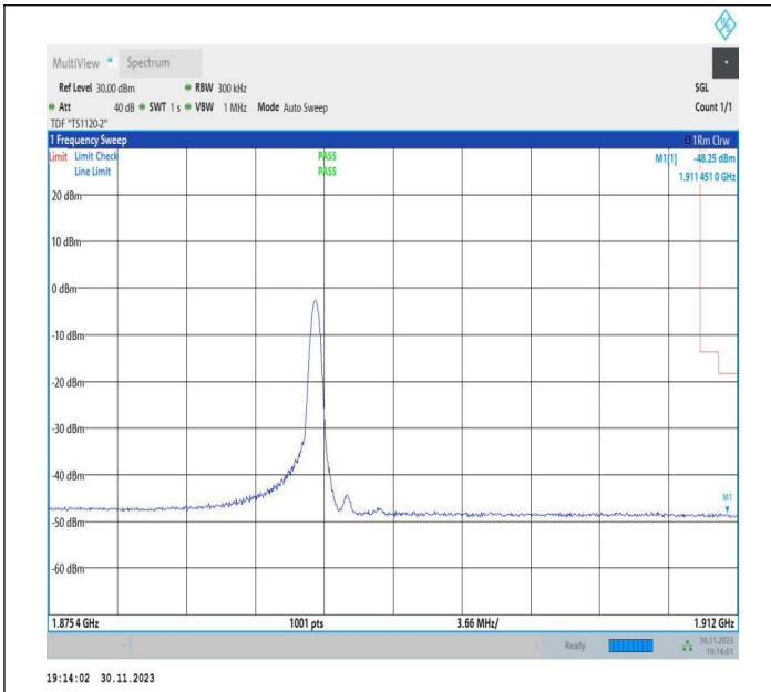
15MHz-20MHz_16QAM@16QAM-16QAM@16QAM_18929-19100_1RB#74@75RB#0-0RB#0@100RB#0
