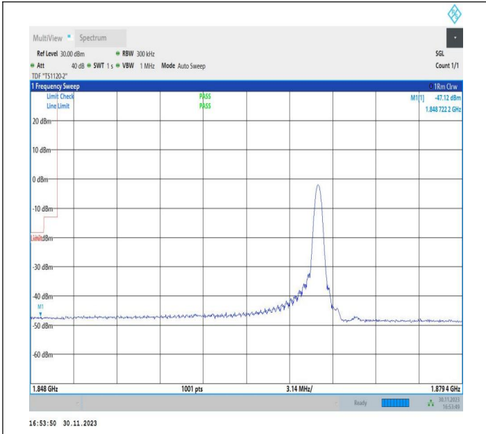
20MHz-10MHz_16QAM@16QAM-16QAM@16QAM_18700-18844_1RB#99@100RB#0-0RB#0@50RB#0
