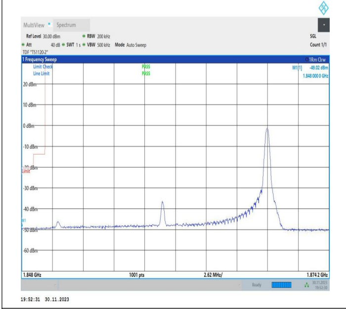
20MHz-5MHz_QPSK@QPSK-QPSK@QPSK_18700-18817_1RB#99@100RB#0-0RB#0@25RB#0
