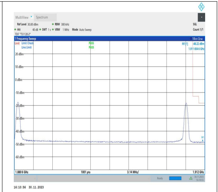
10MHz-20MHz_QPSK@QPSK-QPSK@QPSK_18956-19100_1RB#0@50RB#0-1RB#99@100RB#0
