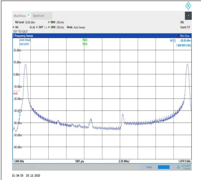
15MHz-10MHz_64QAM@64QAM-64QAM_18675-18795_1RB#0@75RB#0-1RB#49@50RB#0
