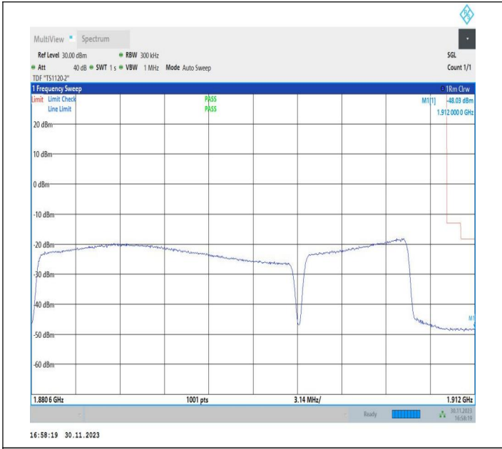
20MHz-10MHz_QPSK@QPSK-QPSK@QPSK_19001-19145_100RB#0@100RB#0-40RB#0@50RB#0
