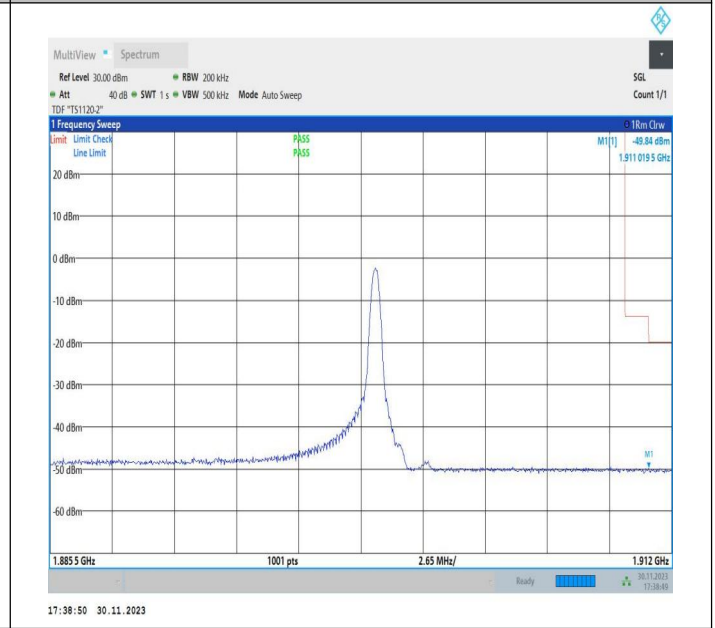
15MHz-10MHz_16QAM@16QAM-16QAM@16QAM_19027-19147_1RB#74@75RB#0-0RB#0@50RB#0
