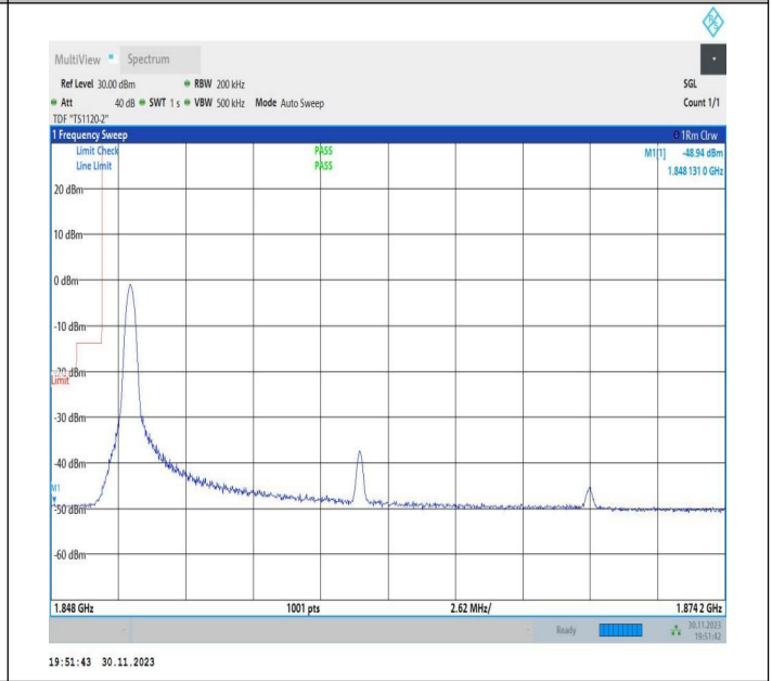
20MHz-5MHz_QPSK@QPSK-QPSK@QPSK_18700-18817_1RB#0@100RB#0-0RB#0@25RB#0
