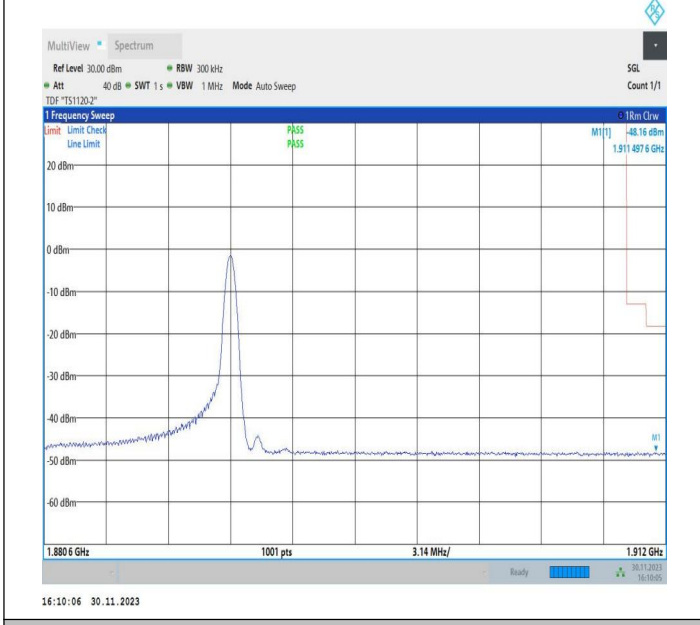
10MHz-20MHz_QPSK@QPSK-QPSK@QPSK_18956-19100_1RB#49@50RB#0-0RB#0@100RB#0
