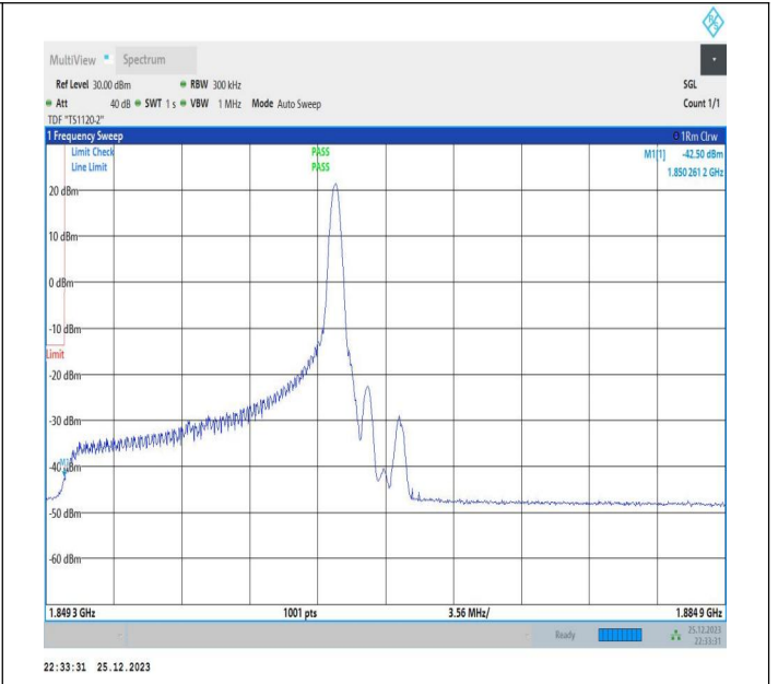
15MHz-20MHz_64QAM@64QAM-64QAM@64QAM_18678-18849_1RB#74@75RB#0-0RB#0@100RB#0
