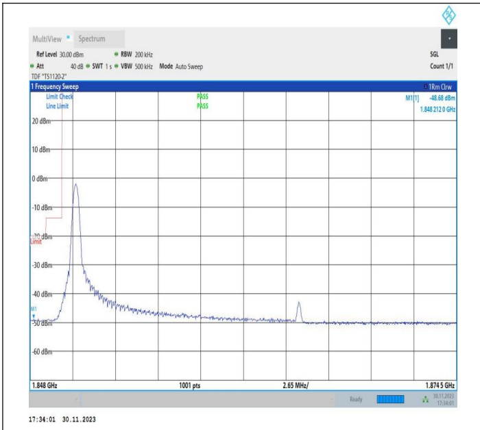
15MHz-10MHz_16QAM@16QAM-16QAM@16QAM_18675-18795_1RB#0@75RB#0-0RB#0@50RB#0
