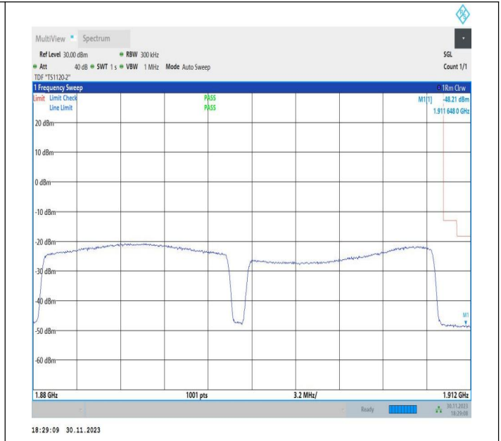
15MHz-15MHz_16QAM@16QAM-16QAM@16QAM_18975-19125_75RB#0@75RB#0-75RB#0@75RB#0
