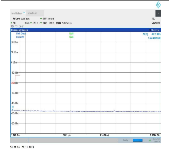
20MHz-10MHz_16QAM@16QAM-16QAM@16QAM_18700-18844_1RB#0@100RB#0-0RB#0@50RB#0
