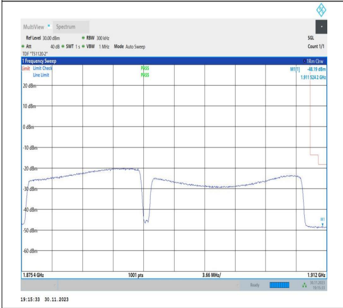
15MHz-20MHz_16QAM@16QAM-16QAM@16QAM_18929-19100_100_75RB#0@75RB#0-100RB#0@100RB#0
