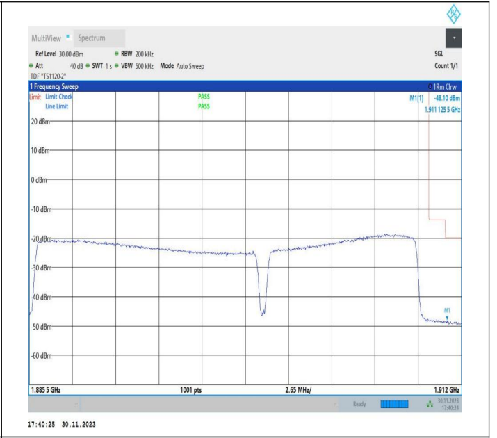
15MHz-10MHz_16QAM@16QAM-16QAM@16QAM_19027-19147_75RB#0@75RB#0-50RB#0@50RB#0
