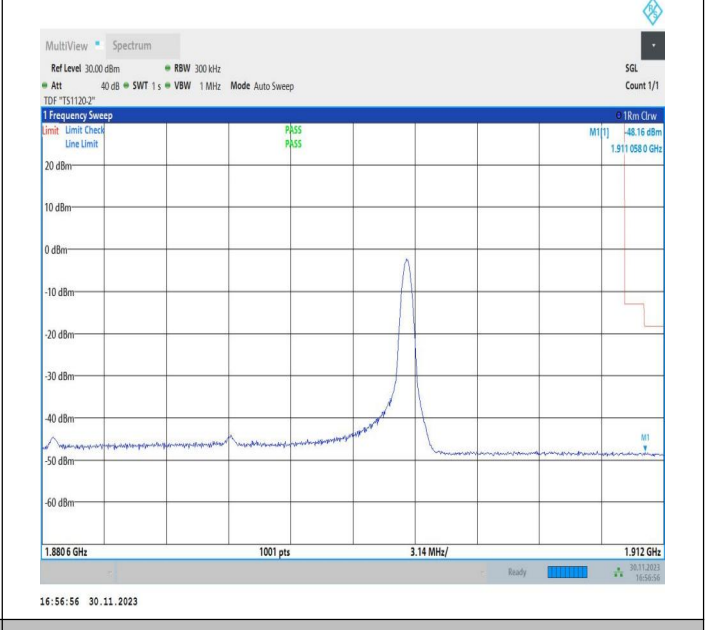
20MHz-10MHz_16QAM@16QAM-16QAM@16QAM_19001-19145_1RB#99@100RB#0-0RB#0@50RB#0
