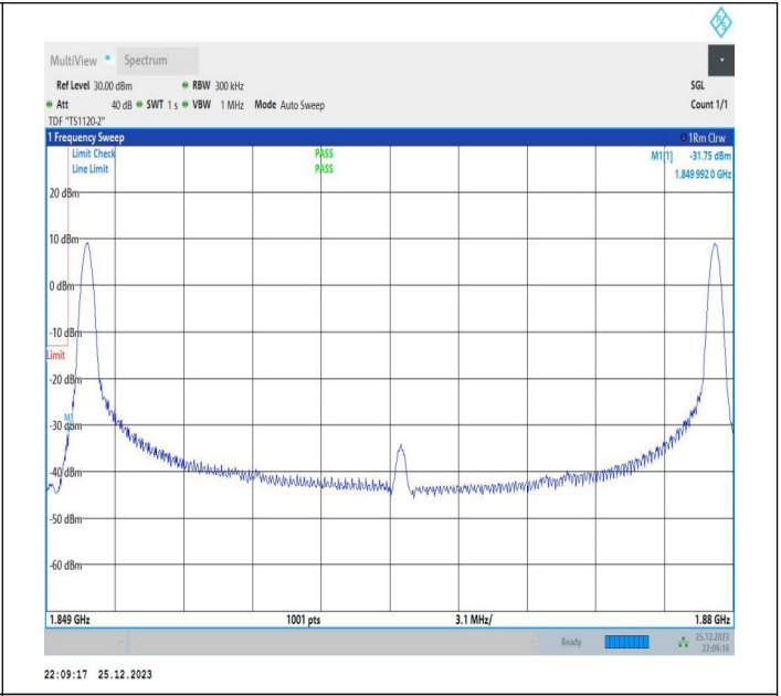
15MHz-15MHz_64QAM@64QAM-64QAM@64QAM_18675-18825_1RB#0@75RB#0-1RB#74@75RB#0
