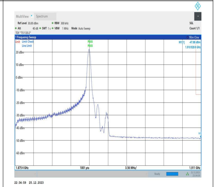
15MHz-20MHz_64QAM@64QAM-64QAM@64QAM_18929-19100_1RB#74@75RB#0-0RB#0@100RB#0
