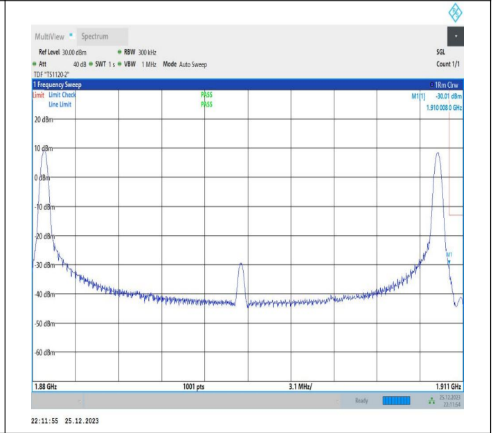
15MHz-15MHz_64QAM@64QAM-64QAM@64QAM_18975-19125_1RB#0@75RB#0-1RB#74@75RB#0
