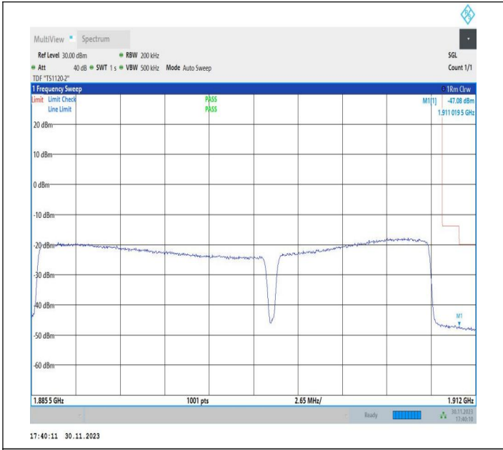
15MHz-10MHz_QPSK@QPSK-QPSK@QPSK_19027-19147_75RB#0@75RB#0-50RB#0@50RB#0
