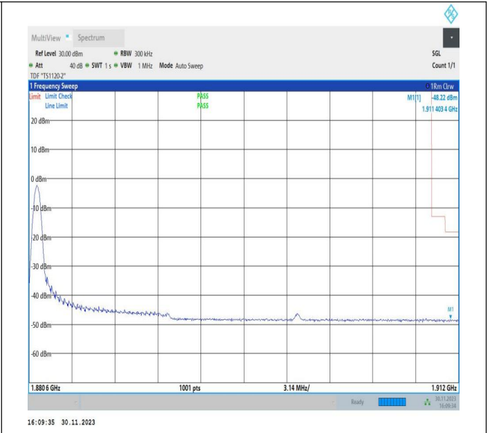
10MHz-20MHz_16QAM@16QAM-16QAM@16QAM_18956-19100_1RB#0@50RB#0-0RB#0@100RB#0
