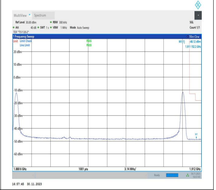
20MHz-10MHz_16QAM@16QAM-16QAM@16QAM_19001-19145_1RB#0@100RB#0-1RB#49@50RB#0
