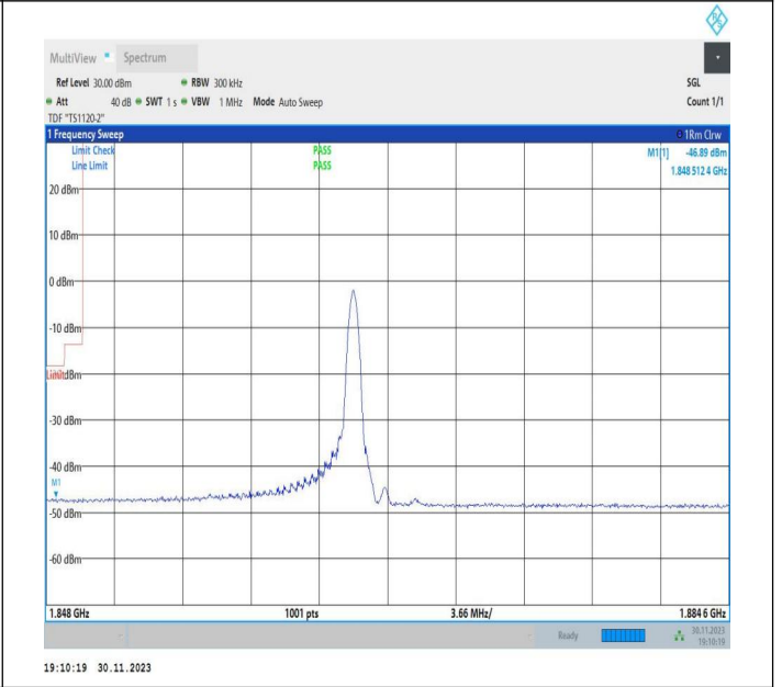
15MHz-20MHz_16QAM@16QAM-16QAM@16QAM_18678-18849_1RB#74@75RB#0-0RB#0@100RB#0
