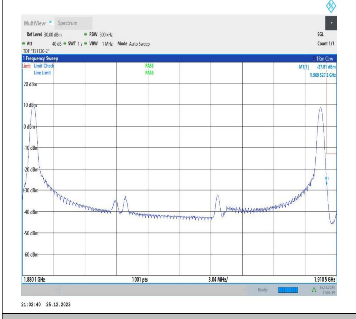
20MHz-10MHz_64QAM@64QAM-64QAM@64QAM_19001-19145_1RB#0@100RB#0-1RB#49@50RB#0
