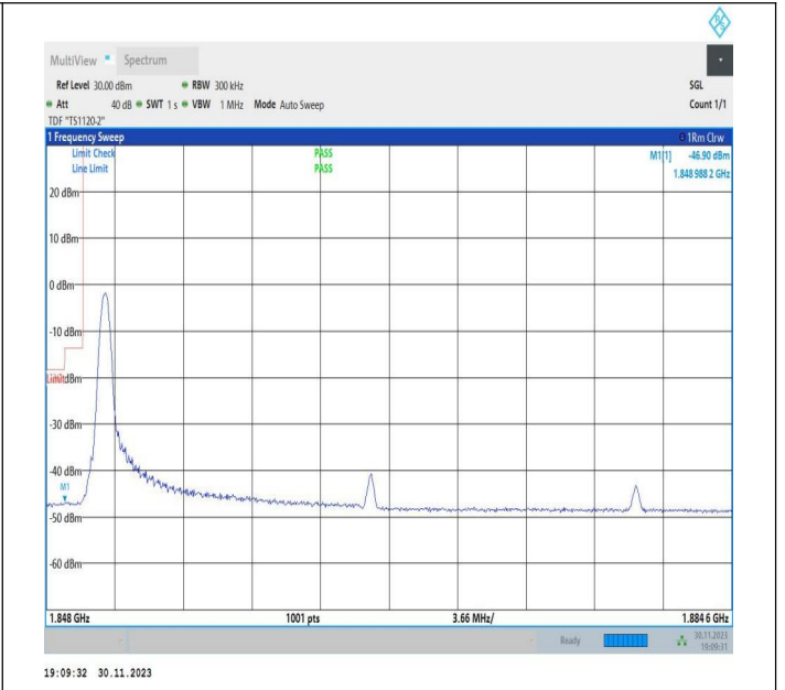
15MHz-20MHz_16QAM@16QAM-16QAM@16QAM_18678-18849_1RB#0@75RB#0-0RB#0@100RB#0
