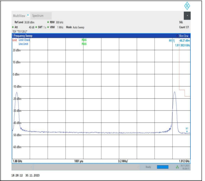
15MHz-15MHz_QPSK@QPSK-QPSK@QPSK_18975-19125_1RB#0@75RB#0-1RB#74@75RB#0
