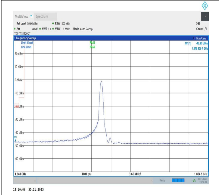
15MHz-20MHz_QPSK@QPSK-QPSK@QPSK_18678-18849_1RB#74@75RB#0-0RB#0@100RB#0
