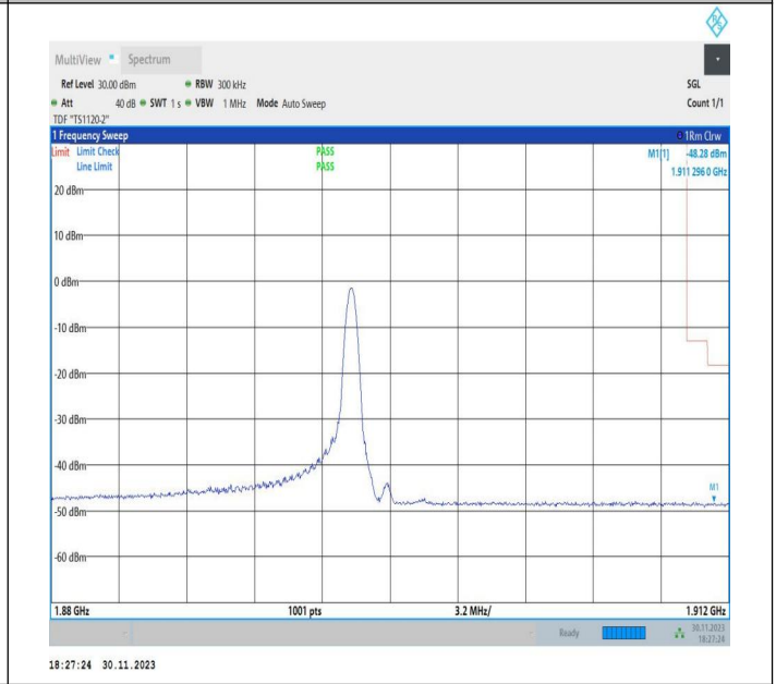
15MHz-15MHz_QPSK@QPSK-QPSK@QPSK_18975-19125_1RB#74@75RB#0-0RB#0@75RB#0
