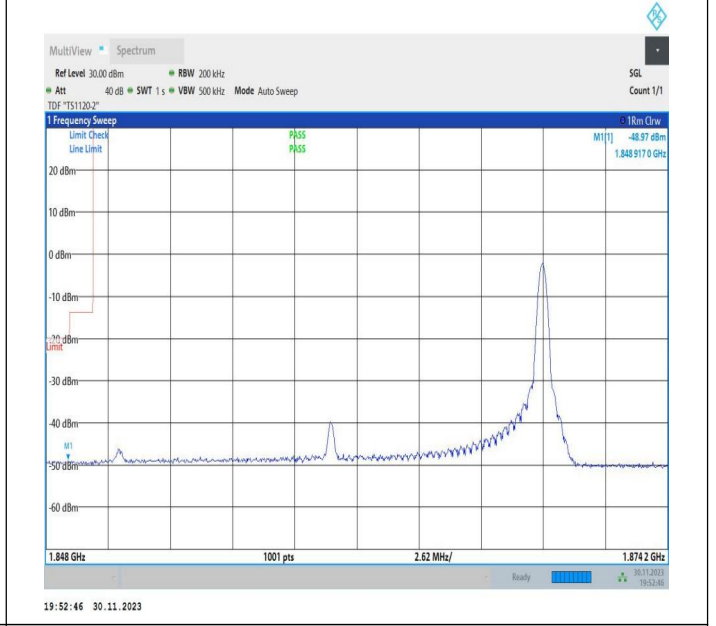
20MHz-5MHz_16QAM@16QAM-16QAM@16QAM_18700-18817_1RB#99@100RB#0-0RB#0@25RB#0
