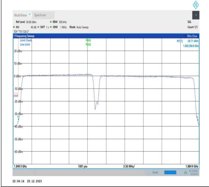
15MHz-20MHz_64QAM@64QAM-64QAM@64QAM_18678-18849_75RB#0@75RB#0-100RB#0@100RB#0
