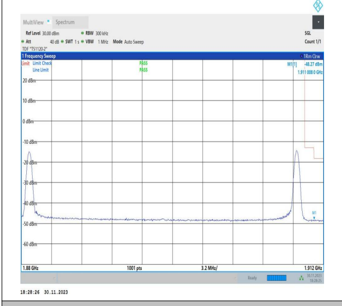
15MHz-15MHz_16QAM@16QAM-16QAM@16QAM_18975-19125_1RB#0@75RB#0-1RB#74@75RB#0
