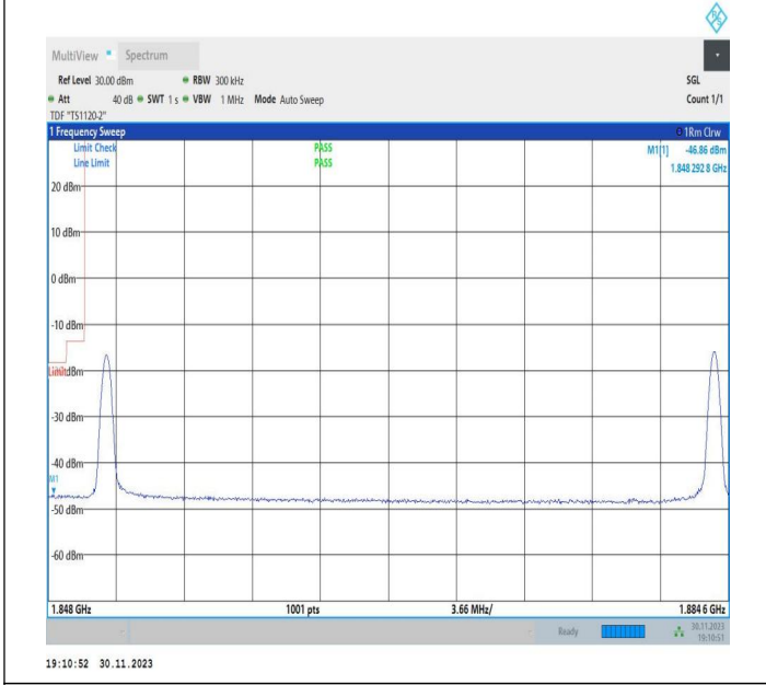
15MHz-20MHz_QPSK@QPSK-QPSK@QPSK_18678-18849_1RB#0@75RB#0-1RB#99@100RB#0
