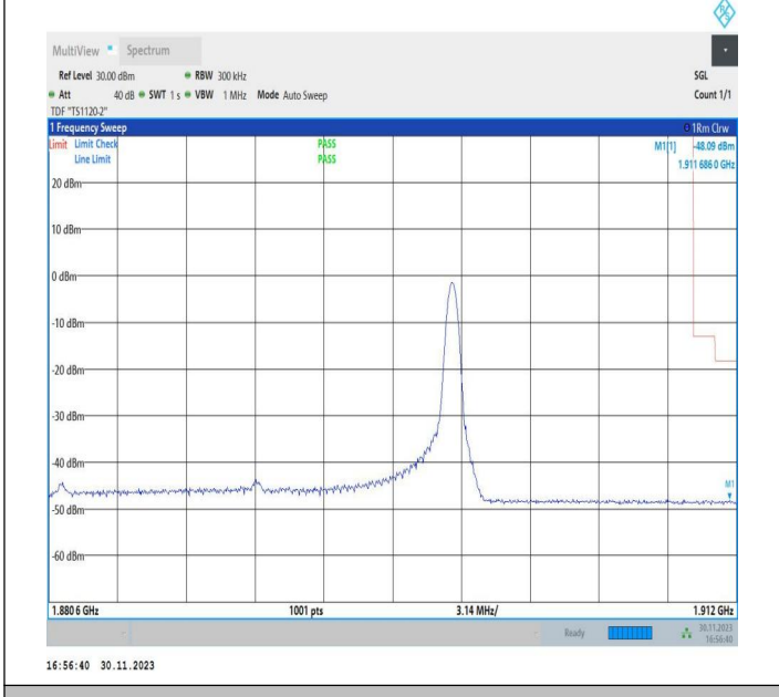
20MHz-10MHz_QPSK@QPSK-QPSK@QPSK_19001-19145_1RB#99@100RB#0-0RB#0@50RB#0
