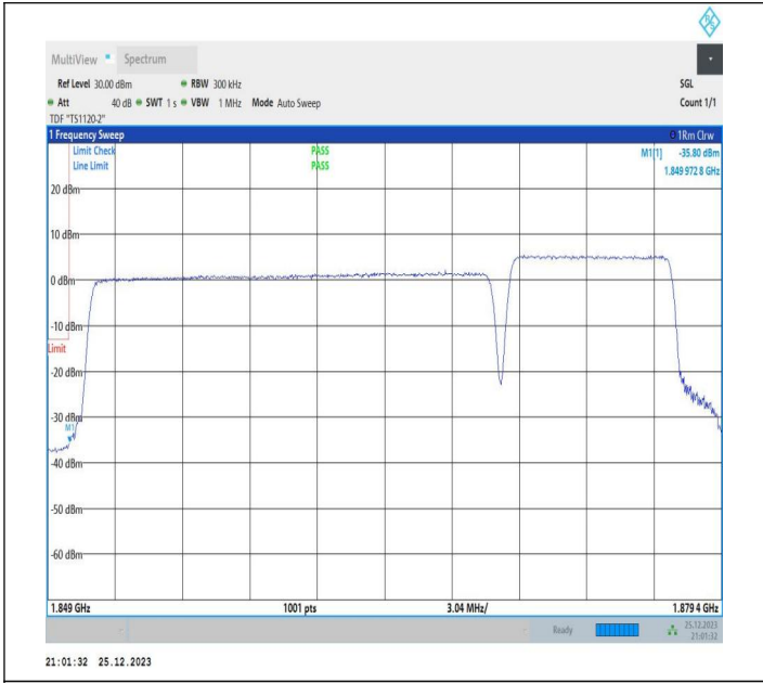
20MHz-10MHz_64QAM@64QAM-64QAM_18700-18844_100RB#0@100RB#0-40RB#0@50RB#0
