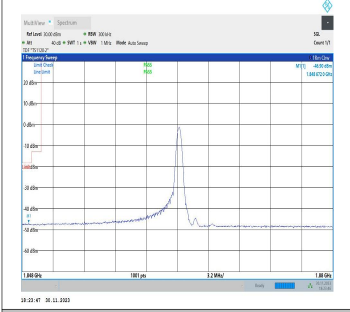
15MHz-15MHz_QPSK@QPSK-QPSK@QPSK_18675-18825_1RB#74@75RB#0-0RB#0@75RB#0
