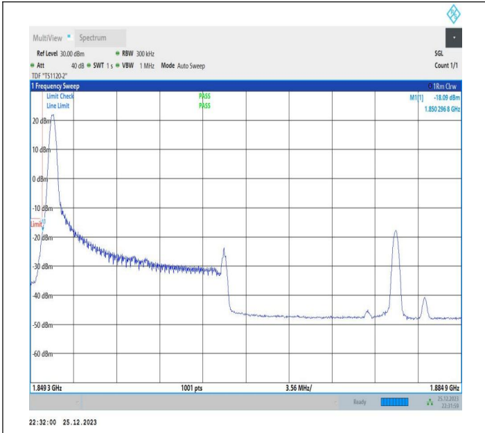
15MHz-20MHz_64QAM@64QAM-64QAM@64QAM_18678-18849_1RB#0@75RB#0-0RB#0@100RB#0
