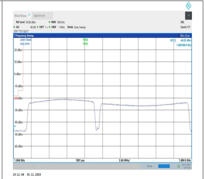
15MHz-20MHz_16QAM@16QAM-16QAM@16QAM_18678-18849_75RB#0@75RB#0-100RB#0@100RB#0
