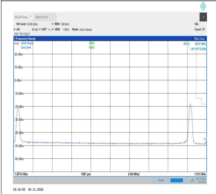
15MHz-20MHz_16QAM@16QAM-16QAM@16QAM_18929-19100_1RB#0@75RB#0-1RB#99@100RB#0
