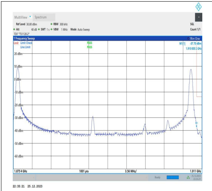
15MHz-20MHz_64QAM@64QAM-64QAM_18929-19100_1RB#0@75RB#0-1RB#99@100RB#0
