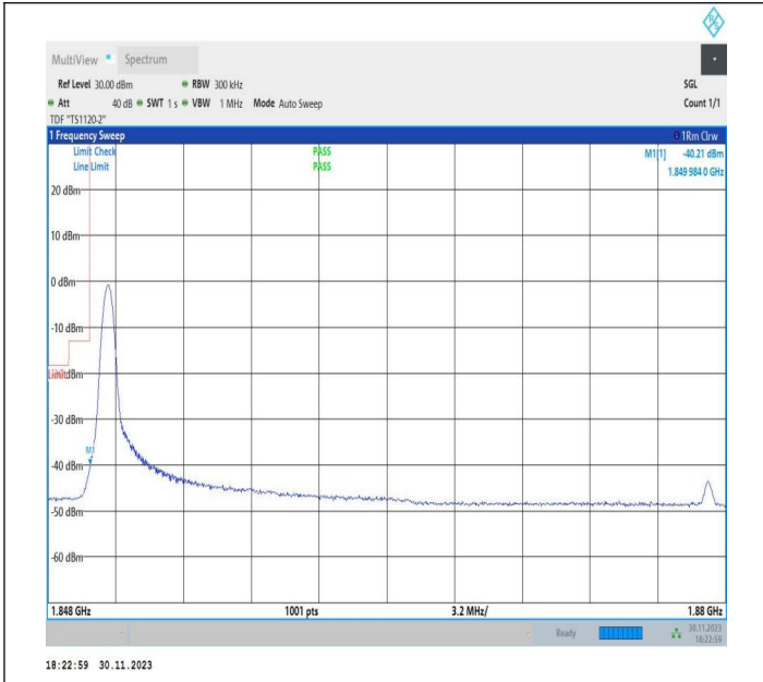
15MHz-15MHz_QPSK@QPSK-QPSK@QPSK_18675-18825_1RB#0@75RB#0-0RB#0@75RB#0
