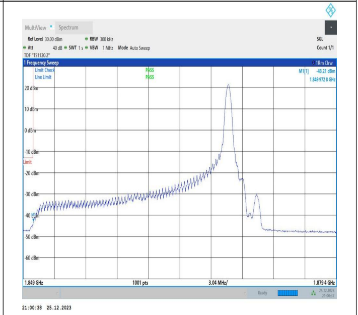
20MHz-10MHz_64QAM@64QAM-64QAM@64QAM_18700-18844_1RB#99@100RB#0-0RB#0@50RB#0
