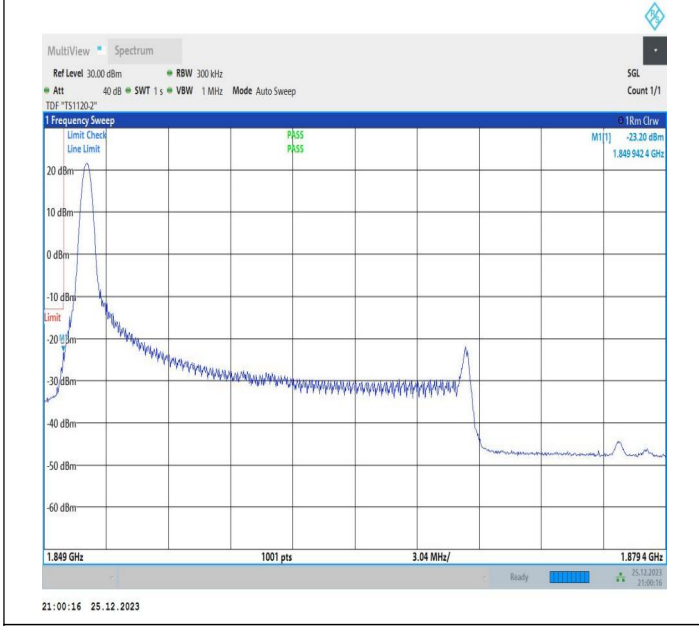
20MHz-10MHz_64QAM@64QAM-64QAM@64QAM_18700-18844_1RB#0@100RB#0-0RB#0@50RB#0
