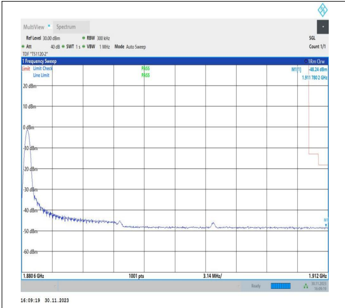
10MHz-20MHz_QPSK@QPSK-QPSK@QPSK_18956-19100_1RB#0@50RB#0-0RB#0@100RB#0
