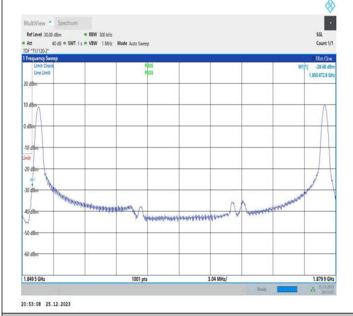
10MHz-20MHz_64QAM@64QAM-64QAM@64QAM_18655-18799_1RB#0@50RB#0-1RB#99@100RB#0
