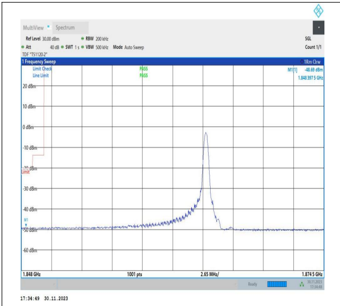
15MHz-10MHz_16QAM@16QAM-16QAM@16QAM_18675-18795_1RB#74@75RB#0-0RB#0@50RB#0
