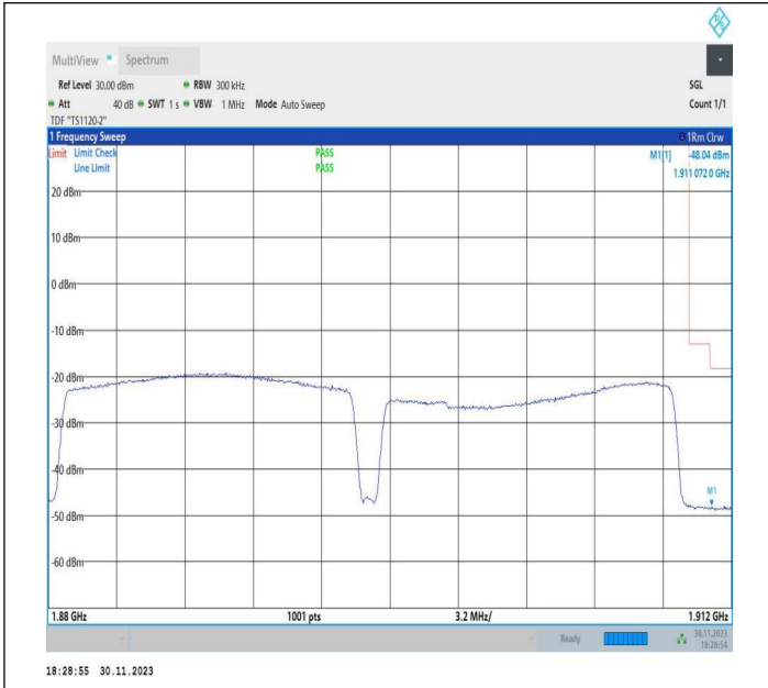
15MHz-15MHz_QPSK@QPSK-QPSK@QPSK_18975-19125_75RB#0@75RB#0-75RB#0@75RB#0
