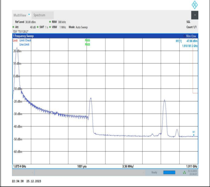
15MHz-20MHz_64QAM@64QAM-64QAM@64QAM_18929-19100_1RB#0@75RB#0-0RB#0@100RB#0
