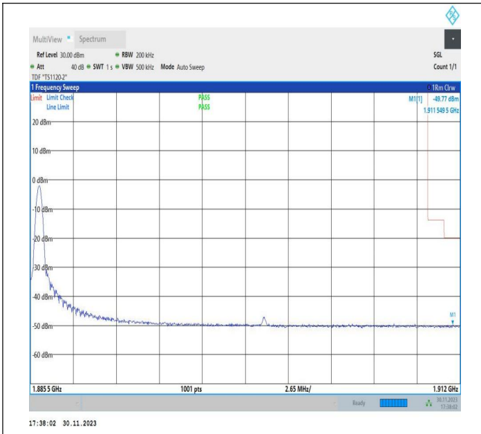
15MHz-10MHz_16QAM@16QAM-16QAM@16QAM_19027-19147_1RB#0@75RB#0-0RB#0@50RB#0
