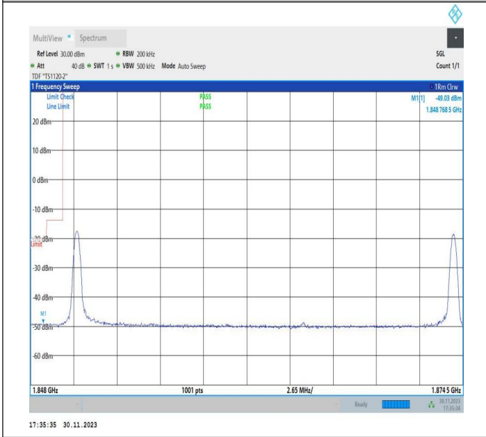
15MHz-10MHz_16QAM@16QAM-16QAM@16QAM_18675-18795_1RB#0@75RB#0-1RB#49@50RB#0
