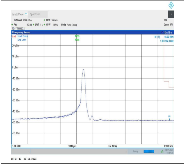
15MHz-15MHz_16QAM@16QAM-16QAM@16QAM_18975-19125_1RB#74@75RB#0-0RB#0@75RB#0
