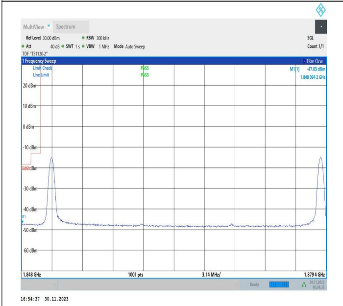
20MHz-10MHz_16QAM@16QAM-16QAM@16QAM_18700-18844_1RB#0@100RB#0-1RB#49@50RB#0
