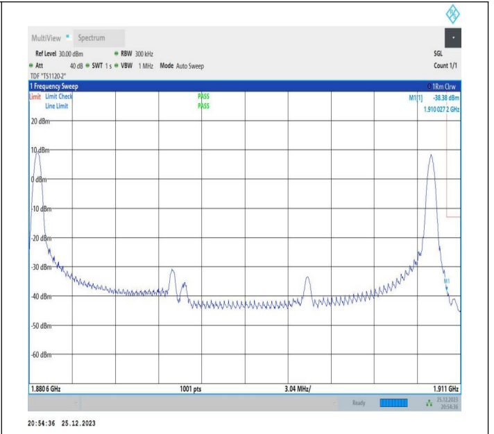
10MHz-20MHz_64QAM@64QAM-64QAM@64QAM_18956-19 100_1RB#0@50RB#0-1RB#99@100RB#0
