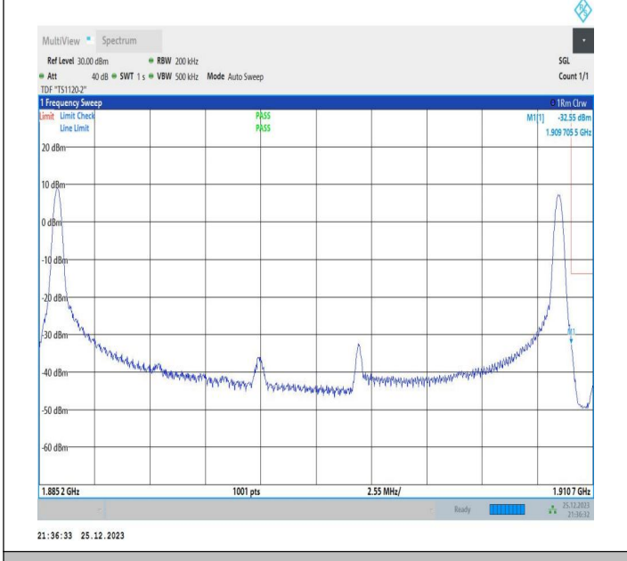
15MHz-10MHz_64QAM@64QAM-64QAM@64QAM_19027-19147_1RB#0@75RB#0-1RB#49@50RB#0
