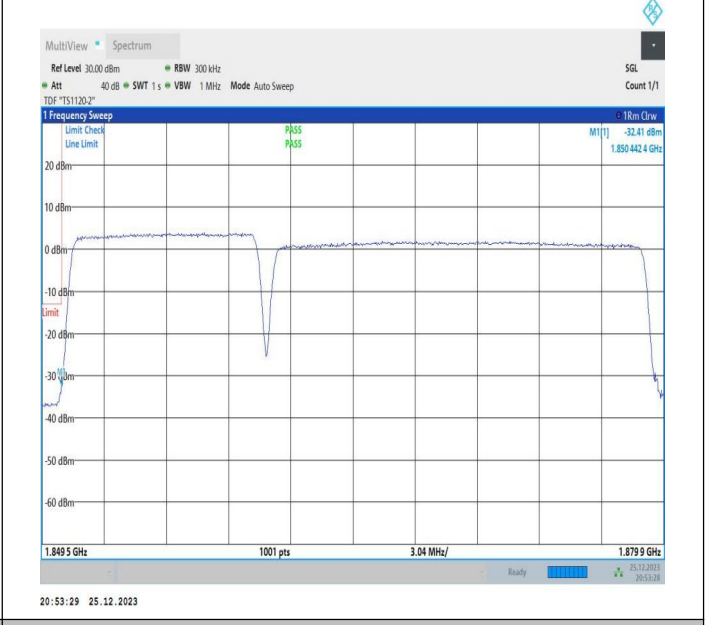
10MHz-20MHz_64QAM@64QAM-64QAM@64QAM_18655-18799_50RB#0@50RB#0-100RB#0@100RB#0
