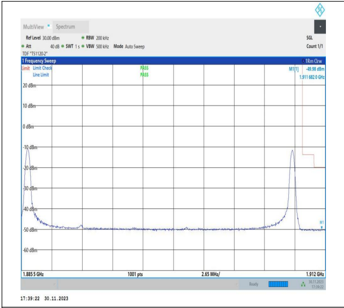
15MHz-10MHz_QPSK@QPSK-QPSK@QPSK_19027-19147_1RB#0@75RB#0-1RB#49@50RB#0
