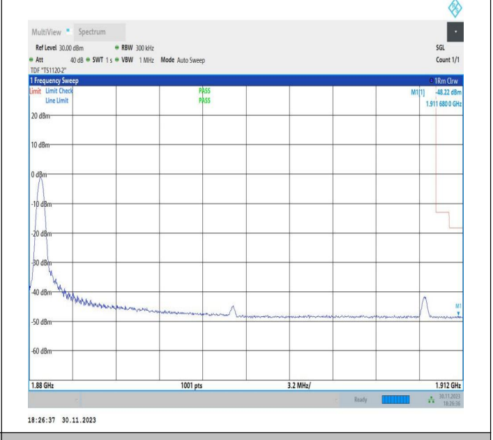
15MHz-15MHz_QPSK@QPSK-QPSK@QPSK_18975-19125_1RB#0@75RB#0-0RB#0@75RB#0
