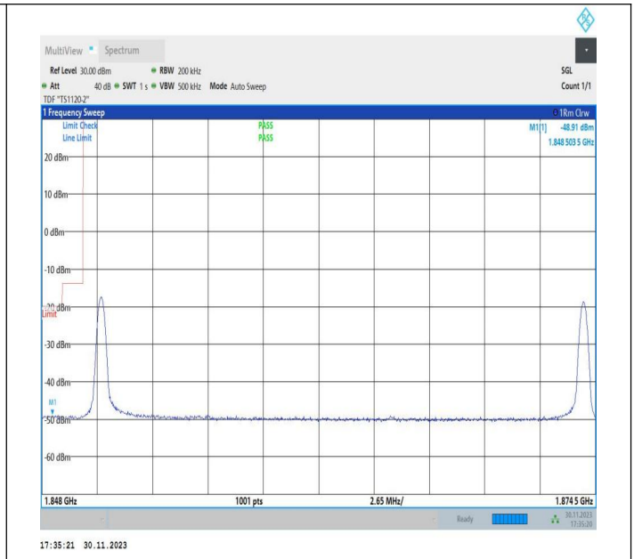
15MHz-10MHz_QPSK@QPSK-QPSK@QPSK_18675-18795_1RB#0@75RB#0-1RB#49@50RB#0
