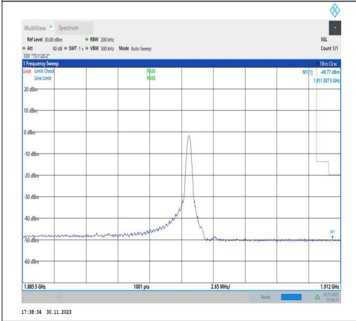
15MHz-10MHz_QPSK@QPSK-QPSK@QPSK_19027-19147_1RB#74@75RB#0-0RB#0@50RB#0
