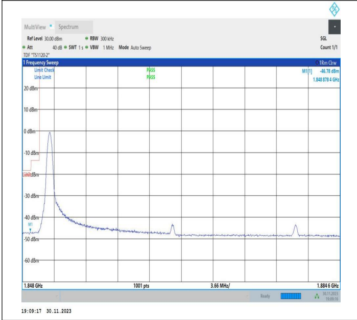
15MHz-20MHz_QPSK@QPSK-QPSK@QPSK_18678-18849_1RB#0@75RB#0-0RB#0@100RB#0
