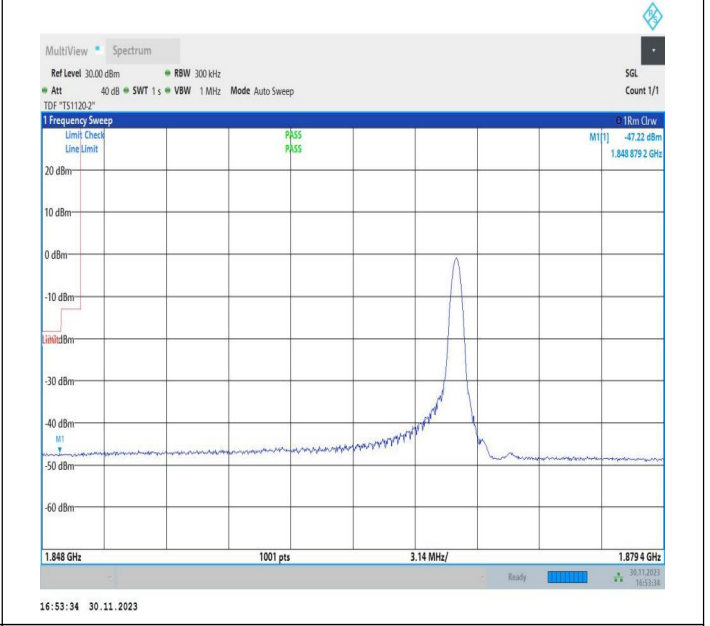
20MHz-10MHz_QPSK@QPSK-QPSK@QPSK_18700-18844_1RB#99@100RB#0-0RB#0@50RB#0
