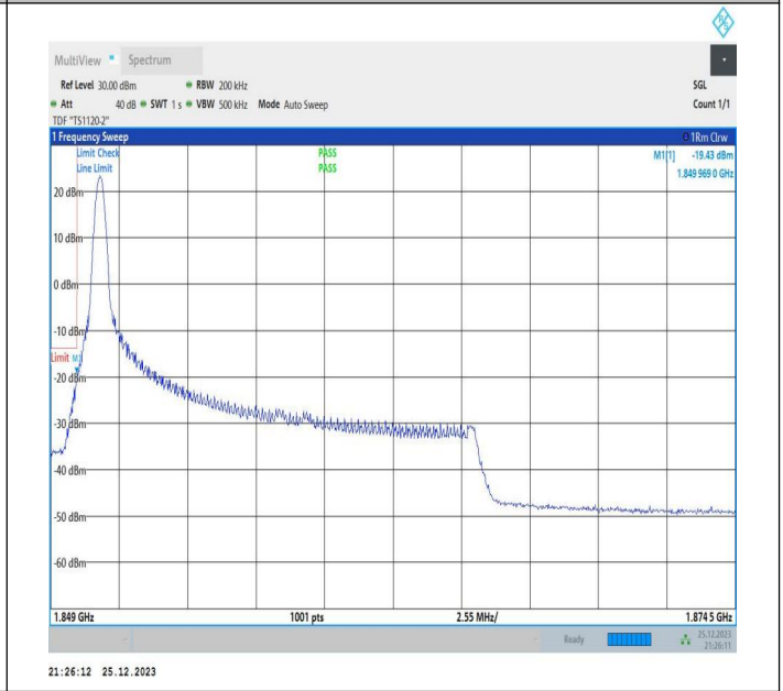
15MHz-10MHz_64QAM@64QAM-64QAM@64QAM_18675-18795_1RB#0@75RB#0-0RB#0@50RB#0
