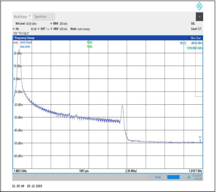
15MHz-10MHz_64QAM@64QAM-64QAM@64QAM_19027-19147_1RB#0@75RB#0-0RB#0@50RB#0
