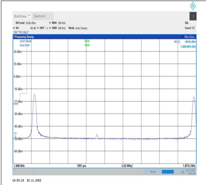
20MHz-5MHz_QPSK@QPSK-QPSK@QPSK_18700-18817_1RB#0@100RB#0-1RB#24@25RB#0
