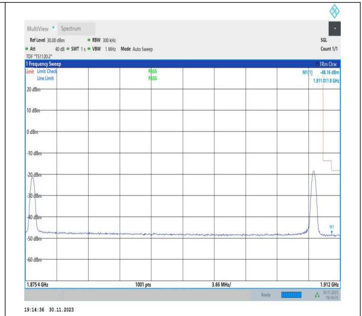
15MHz-20MHz_QPSK@QPSK-QPSK@QPSK_18929-19100_1RB#0@75RB#0-1RB#99@100RB#0
