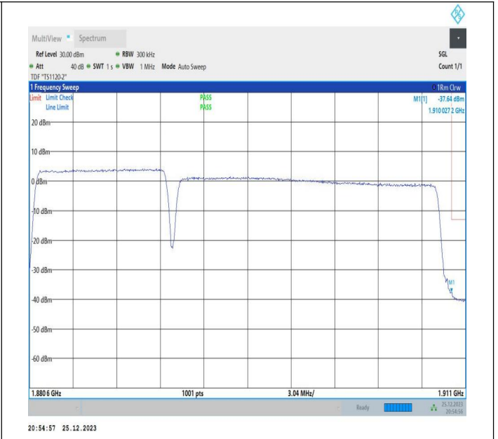
10MHz-20MHz_64QAM@64QAM-64QAM@64QAM_18956-19100_50RB#0@50RB#0-100RB#0@100RB#0
