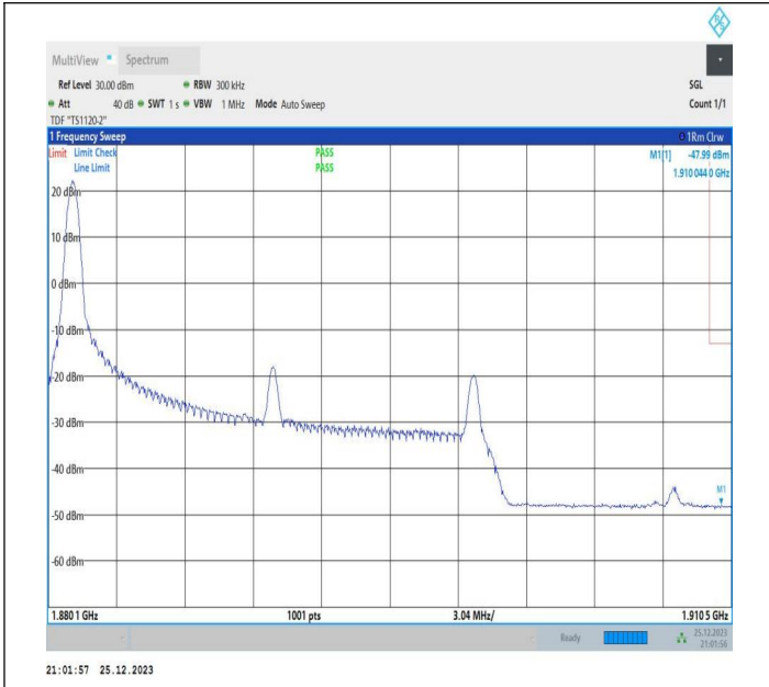
20MHz-10MHz_64QAM@64QAM-64QAM@64QAM_19001-19145_1RB#0@100RB#0-0RB#0@50RB#0
