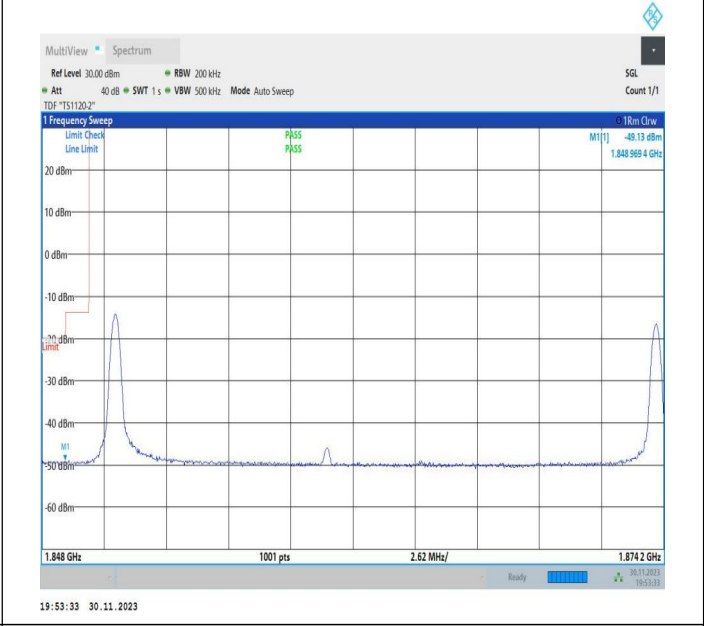
20MHz-5MHz_16QAM@16QAM-16QAM@16QAM_18700-18817_1RB#0@100RB#0-1RB#24@25RB#0
