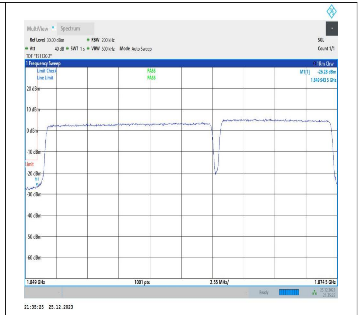
15MHz-10MHz_64QAM@64QAM-64QAM@64QAM_18675-18795_75RB#0@75RB#0-50RB#0@50RB#0
