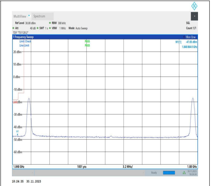
15MHz-15MHz_QPSK@QPSK-QPSK@QPSK_18675-18825_1RB#0@75RB#0-1RB#74@75RB#0
