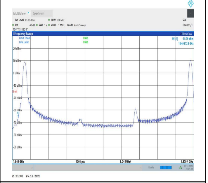
20MHz-10MHz_64QAM@64QAM-64QAM@64QAM_18700-18844_1RB#0@100RB#0-1RB#49@50RB#0
