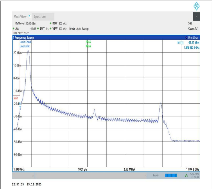
20MHz-5MHz_64QAM@64QAM-64QAM@64QAM_18700-18817_1RB#0@100RB#0-0RB#0@25RB#0
