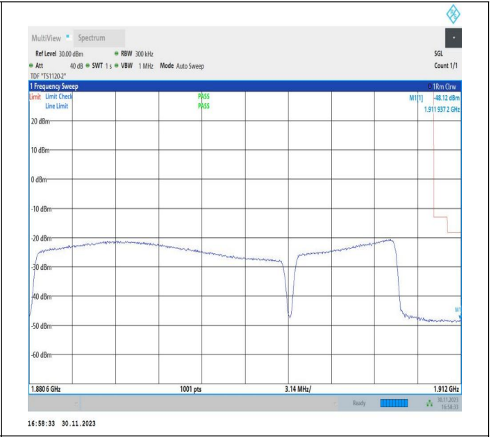
20MHz-10MHz_16QAM@16QAM-16QAM@16QAM_19001-19145_100RB#0@100RB#0-40RB#0@50RB#0
