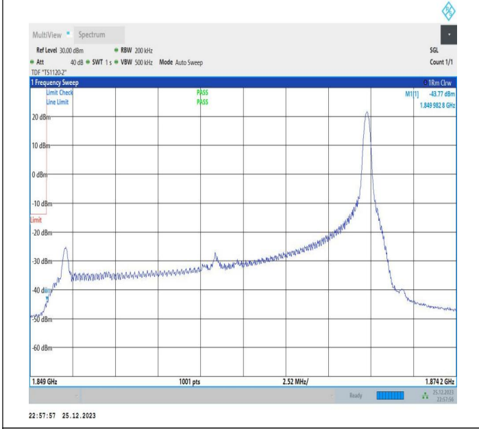
20MHz-5MHz_64QAM@64QAM-64QAM@64QAM_18700-18817_1RB#99@100RB#0-0RB#0@25RB#0
