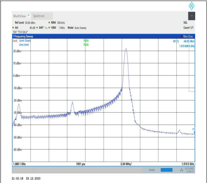
20MHz-10MHz_64QAM@64QAM-64QAM@64QAM_19001-19145_1RB#99@100RB#0-0RB#0@50RB#0
