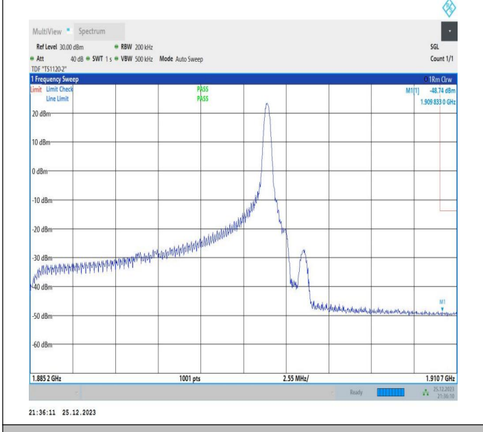
15MHz-10MHz_64QAM@64QAM-64QAM@64QAM_19027-19147_1RB#74@75RB#0-0RB#0@50RB#0
