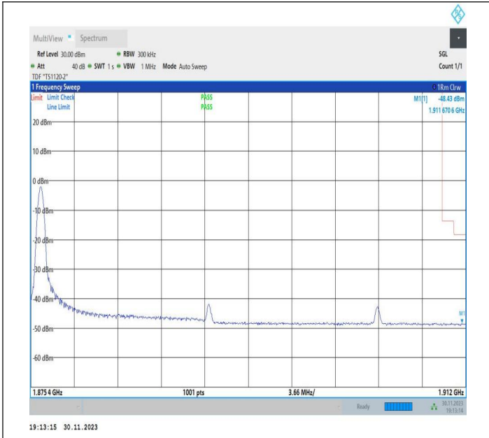
15MHz-20MHz_16QAM@16QAM-16QAM@16QAM_18929-19100_1RB#0@75RB#0-0RB#0@100RB#0
