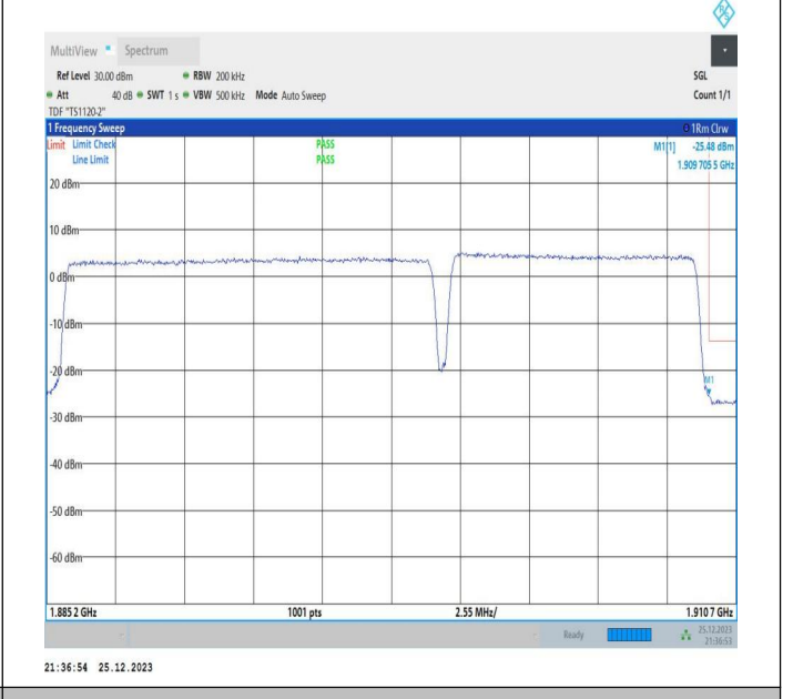
15MHz-10MHz_64QAM@64QAM-64QAM@64QAM_19027-19147_75RB#0@75RB#0-50RB#0@50RB#0
