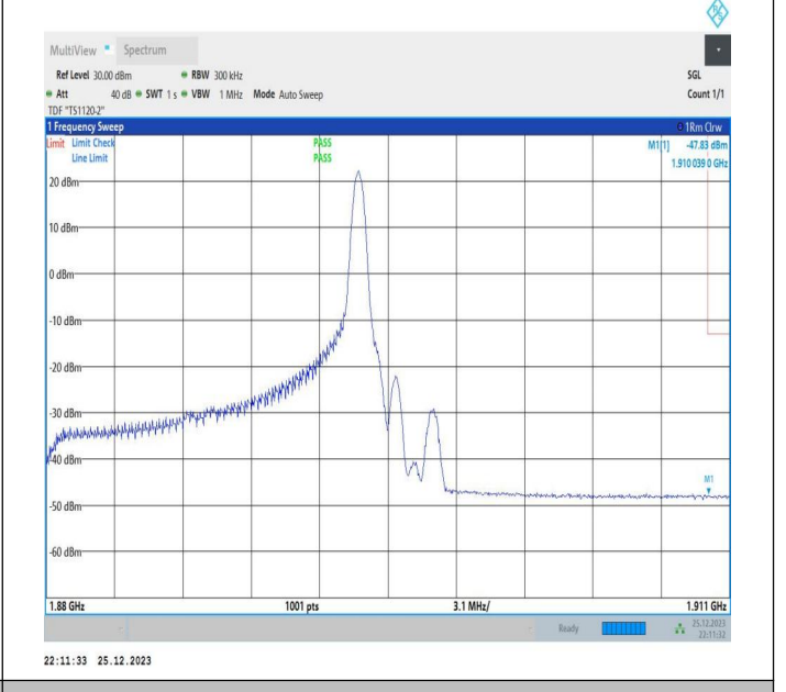
15MHz-15MHz_64QAM@64QAM-64QAM@64QAM_18975-19125_1RB#74@75RB#0-0RB#0@75RB#0
