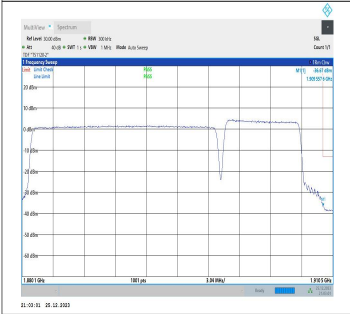
20MHz-10MHz_64QAM@64QAM-64QAM@64QAM_19001-19145_100RB#0@100RB#0-40RB#0@50RB#0
