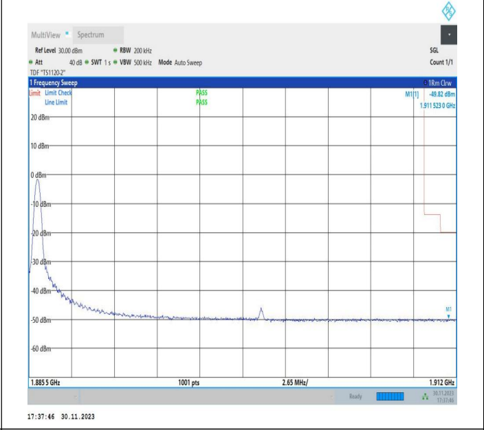
15MHz-10MHz_QPSK@QPSK-QPSK@QPSK_19027-19147_1RB#0@75RB#0-0RB#0@50RB#0
