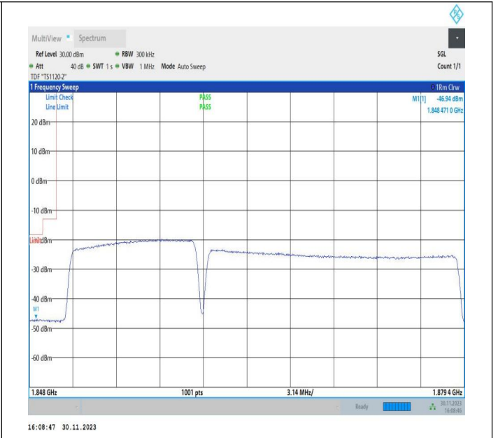
10MHz-20MHz_16QAM@16QAM-16QAM@16QAM_18655-18799_50RB#0@50RB#0-100RB#0@100RB#0
