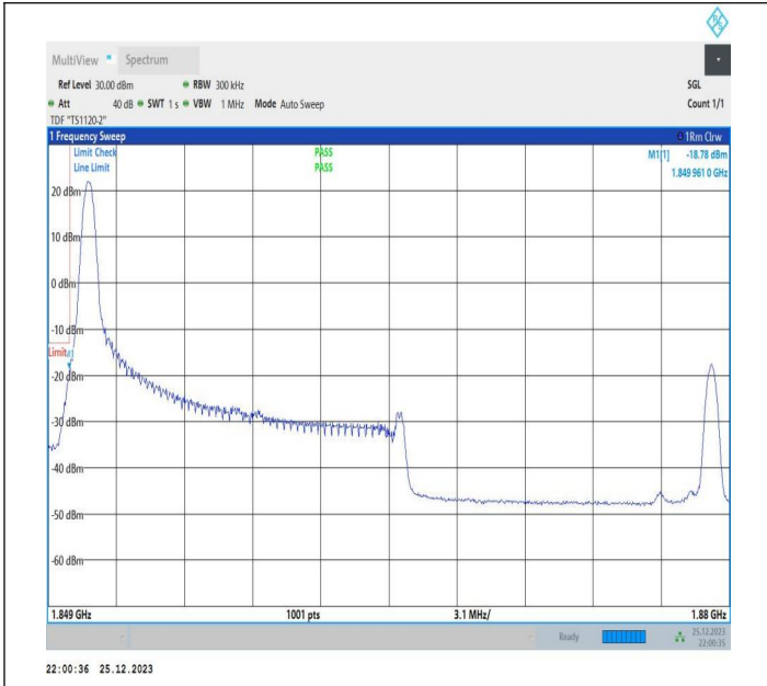
15MHz-15MHz_64QAM@64QAM-64QAM_18675-18825_1RB#0@75RB#0-0RB#0@75RB#0
