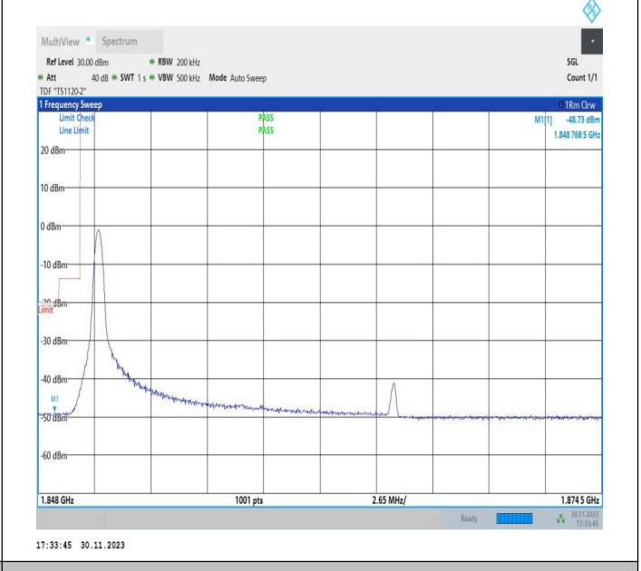
15MHz-10MHz_QPSK@QPSK-QPSK@QPSK_18675-18795_1RB#0@75RB#0-0RB#0@50RB#0
