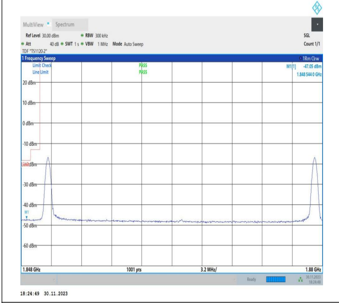
15MHz-15MHz_16QAM@16QAM-16QAM@16QAM_18675-18825_1RB#0@75RB#0-1RB#74@75RB#0
