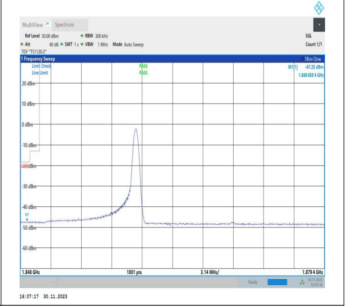
10MHz-20MHz_16QAM@16QAM-16QAM@16QAM_18655-18799_1RB#49@50RB#0-0RB#0@100RB#0
