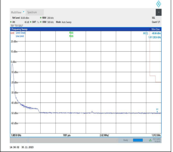
5MHz-20MHz_QPSK@QPSK-QPSK@QPSK_18983-19100_1RB#0@25RB#0-0RB#0@100RB#0
