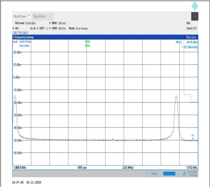
5MHz-20MHz_QPSK@QPSK-QPSK@QPSK_18983-19100_1RB#0@25RB#0-1RB#99@100RB#0
