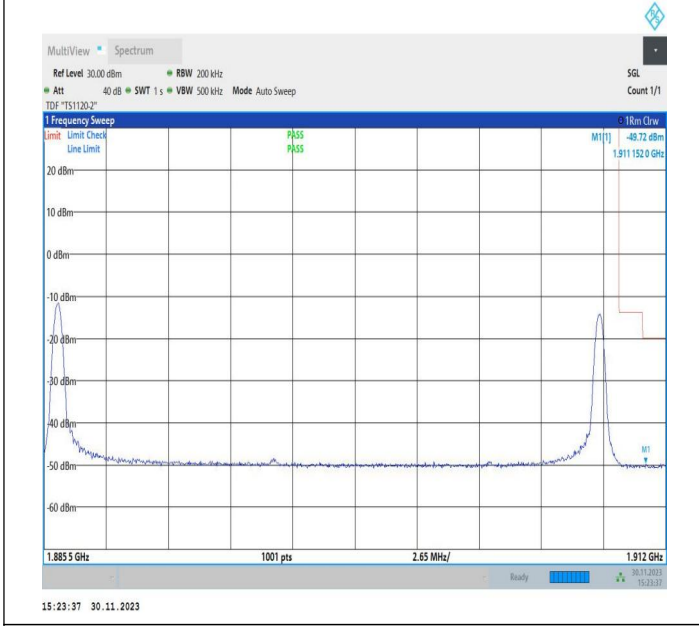
10MHz-15MHz_16QAM@16QAM-16QAM@16QAM_19005-19125_1RB#0@50RB#0-1RB#74@75RB#0
