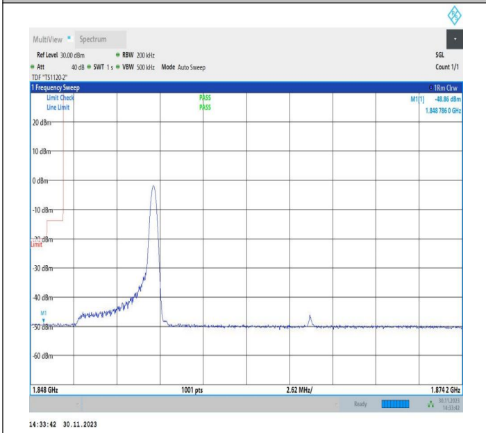
5MHz-20MHz_QPSK@QPSK-QPSK@QPSK_18633-18750_1 RB#24@25RB#0-0RB#0@100RB#0
