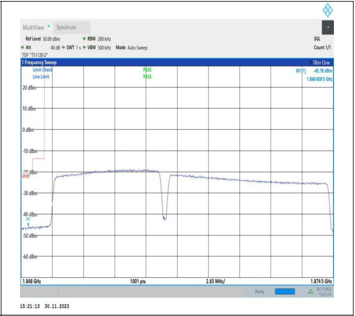
10MHz-15MHz_16QAM@16QAM-16QAM@16QAM_18653-18773_50RB#0@50RB#0-75RB#0@75RB#0
