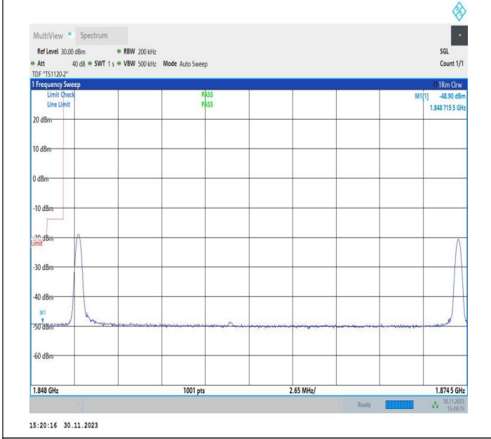
10MHz-15MHz_QPSK@QPSK-QPSK@QPSK_18653-18773_1RB#0@50RB#0-1RB#74@75RB#0
