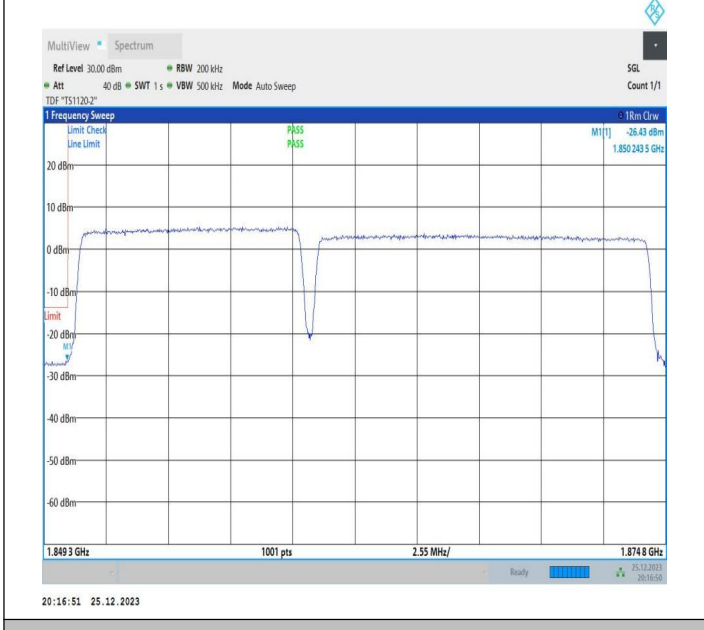
10MHz-15MHz_64QAM@64QAM-64QAM@64QAM_18653-18773_50RB#0@50RB#0-75RB#0@75RB#0
