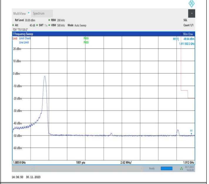
5MHz-20MHz_QPSK@QPSK-QPSK@QPSK_18983-19100_1RB#24@25RB#0-0RB#0@100RB#0
