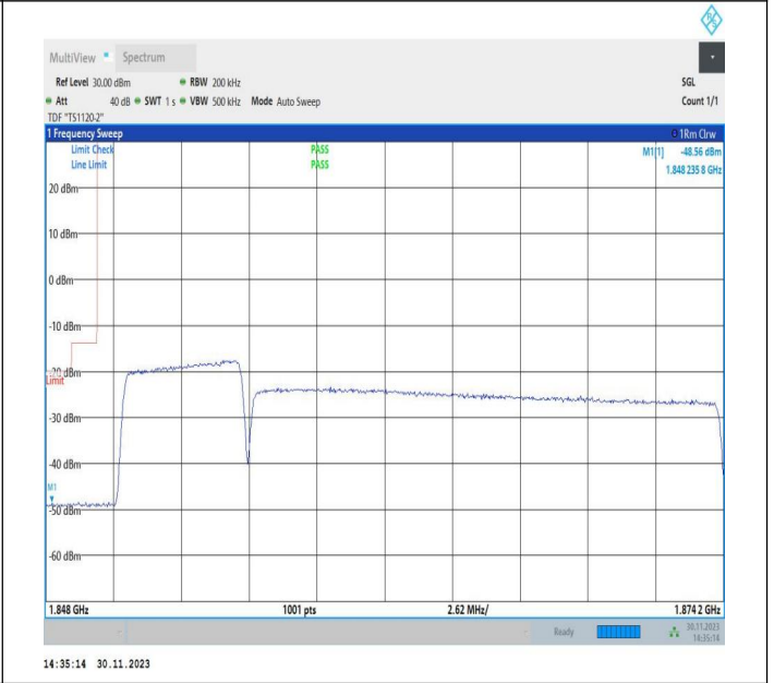
5MHz-20MHz_QPSK@QPSK-QPSK@QPSK_18633-18750_25RB#0@25RB#0-100RB#0@100RB#0
