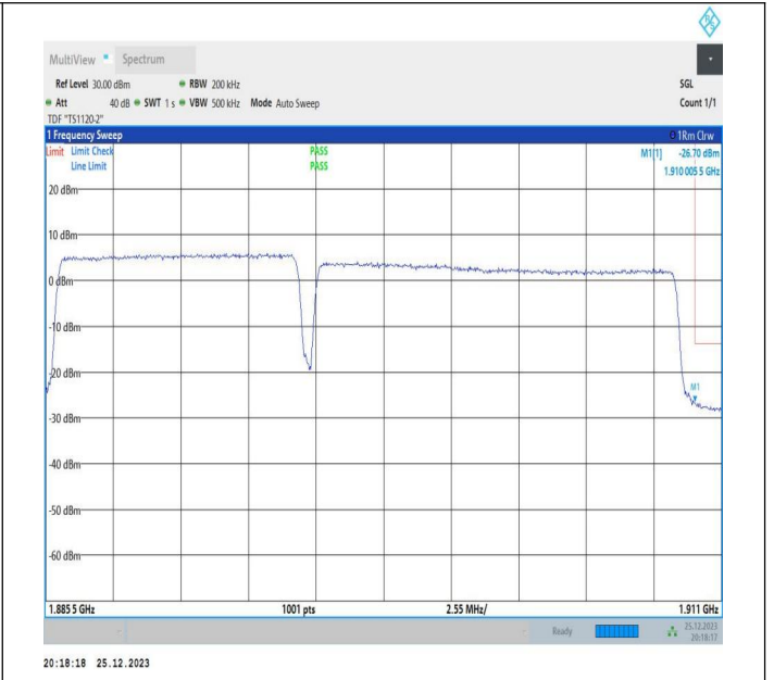
10MHz-15MHz_64QAM@64QAM-64QAM@64QAM_19005-19111_125_50RB#0@50RB#0-75RB#0@75RB#0
