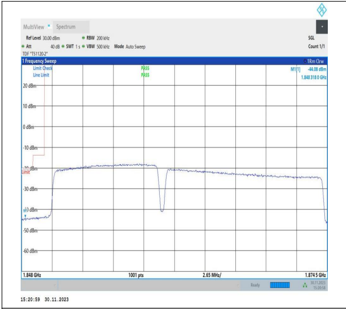
10MHz-15MHz_QPSK@QPSK-QPSK@QPSK_18653-18773_50RB#0@50RB#0-75RB#0@75RB#0
