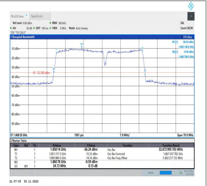
2-2-20MHz-15MHz-16QAM-16QAM-18700-18871-100RB#0-7 5RB#0-PASS
