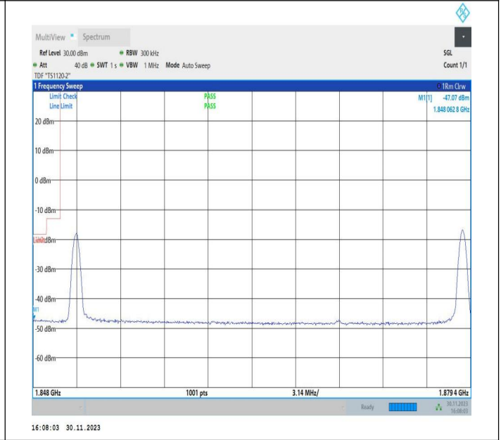
10MHz-20MHz_16QAM@16QAM-16QAM@16QAM_18655-18799_1RB#0@50RB#0-1RB#99@100RB#0
