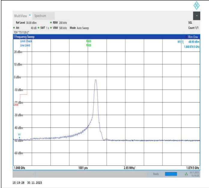
10MHz-15MHz_QPSK@QPSK-QPSK@QPSK_18653-18773_1RB#49@50RB#0-0RB#0@75RB#0
