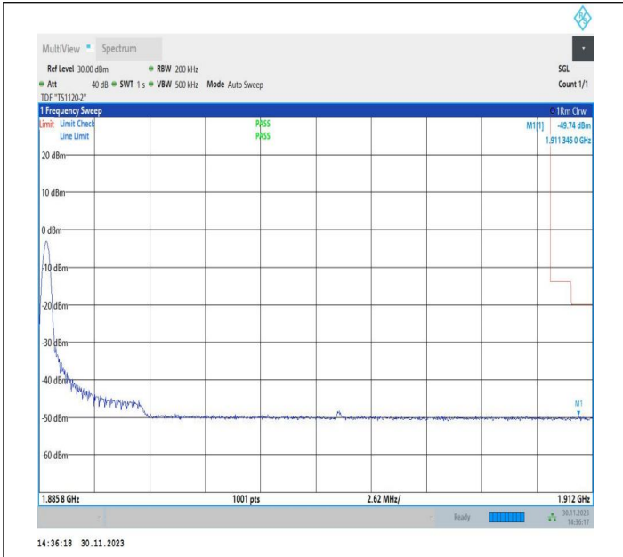
5MHz-20MHz_16QAM@16QAM-16QAM@16QAM_18983-19100_1RB#0@25RB#0-0RB#0@100RB#0
