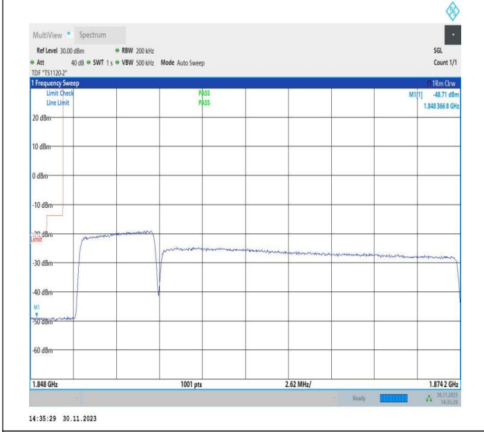
5MHz-20MHz_16QAM@16QAM-16QAM@16QAM_18633-18750_25RB#0@25RB#0-100RB#0@100RB#0
