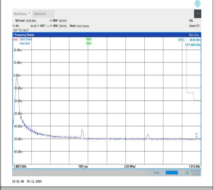
10MHz-15MHz_QPSK@QPSK-QPSK@QPSK_19005-19125_1RB#0@50RB#0-0RB#0@75RB#0
