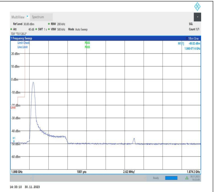
5MHz-20MHz_16QAM@16QAM-16QAM@16QAM_18633-187 50_1RB#0@25RB#0-0RB#0@100RB#0
