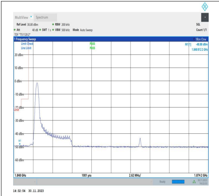
5MHz-20MHz_QPSK@QPSK-QPSK@QPSK_18633-18750_1 RB#0@25RB#0-0RB#0@100RB#0
