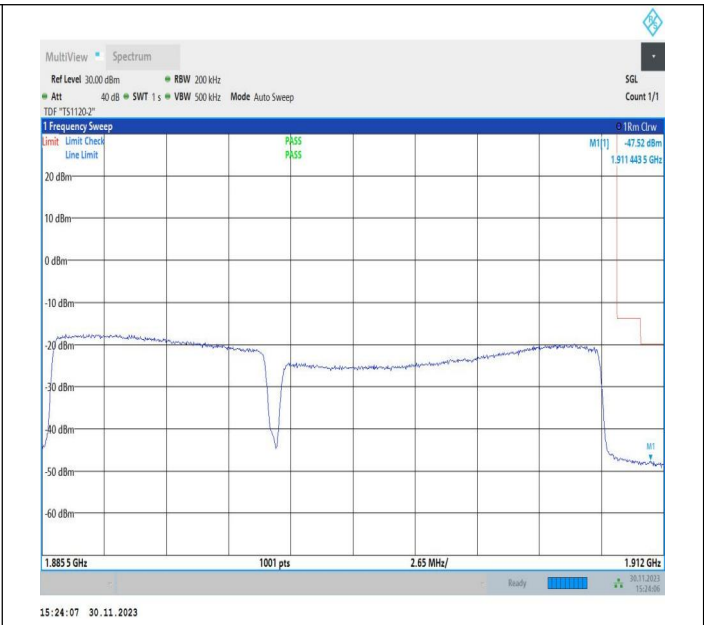
10MHz-15MHz_QPSK@QPSK-QPSK@QPSK_19005-19125_50RB#0@50RB#0-75RB#0@75RB#0
