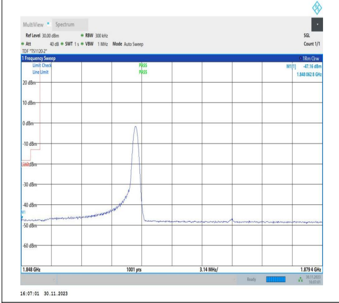
10MHz-20MHz_QPSK@QPSK-QPSK@QPSK_18655-18799_1RB#49@50RB#0-0RB#0@100RB#0
