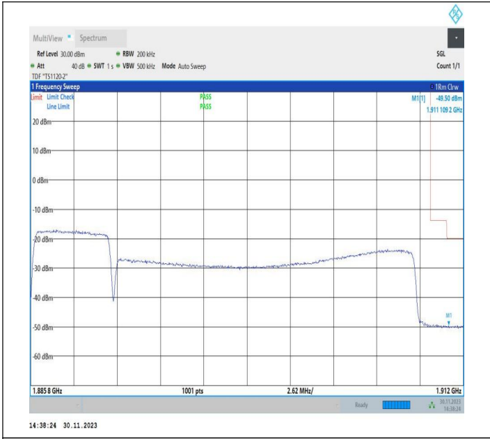
5MHz-20MHz_QPSK@QPSK-QPSK@QPSK_18983-19100_2 5RB#0@25RB#0-100RB#0@100RB#0
