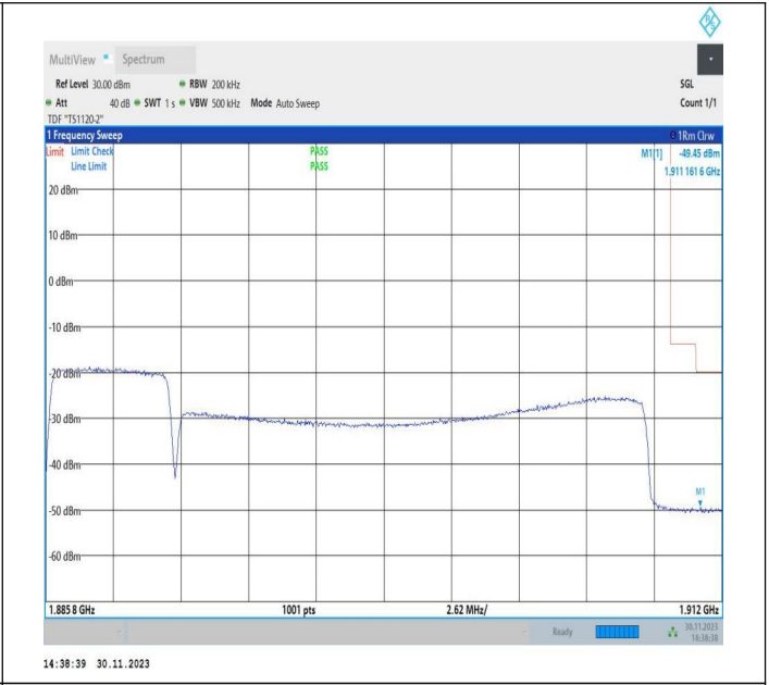
5MHz-20MHz_16QAM@16QAM-16QAM@16QAM_18983-19100_25RB#0@25RB#0-100RB#0@100RB#0
