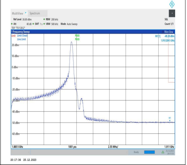
10MHz-15MHz_64QAM@64QAM-64QAM@64QAM_19005-19125_1RB#49@50RB#0-0RB#0@75RB#0
