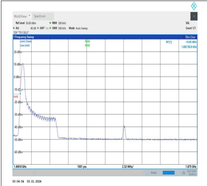
5MHz-20MHz_64QAM@64QAM-64QAM_18633-18750_1RB#0@25RB#0-0RB#0@100RB#0
