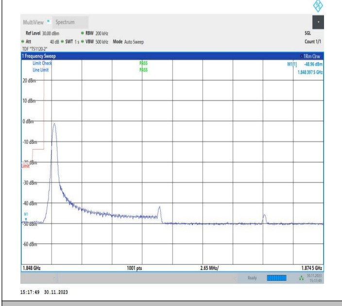
10MHz-15MHz_QPSK@QPSK-QPSK@QPSK_18653-18773_1RB#0@50RB#0-0RB#0@75RB#0
