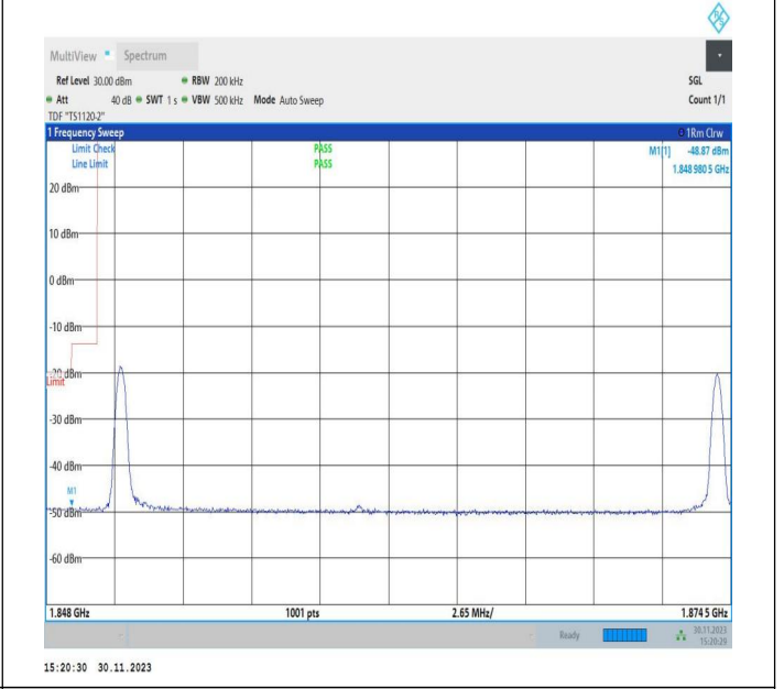
10MHz-15MHz_16QAM@16QAM-16QAM@16QAM_18653-18773_1RB#0@50RB#0-1RB#74@75RB#0
