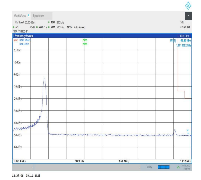
5MHz-20MHz_16QAM@16QAM-16QAM@16QAM_18983-19100_1RB#24@25RB#0-0RB#0@100RB#0
