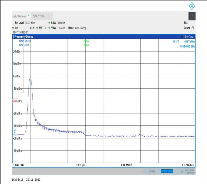
10MHz-20MHz_QPSK@QPSK-QPSK@QPSK_18655-18799_1RB#0@50RB#0-0RB#0@100RB#0
