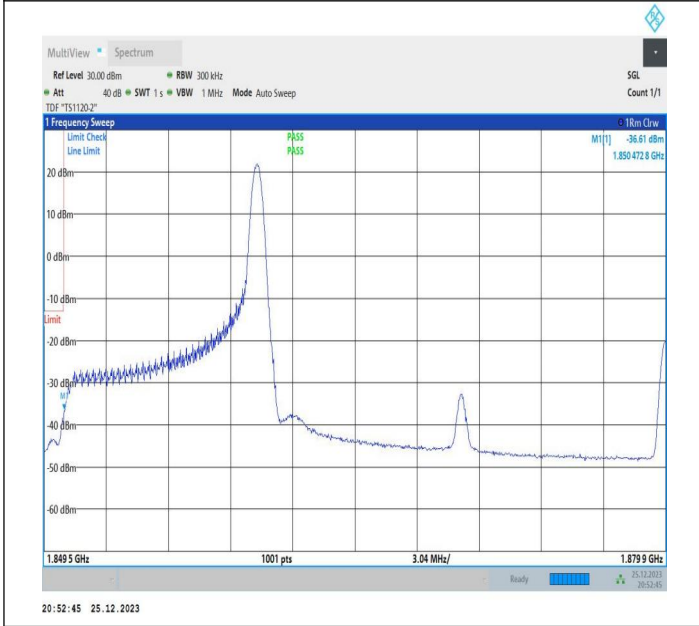
10MHz-20MHz_64QAM@64QAM-64QAM@64QAM_18655-18799_1RB#49@50RB#0-0RB#0@100RB#0
