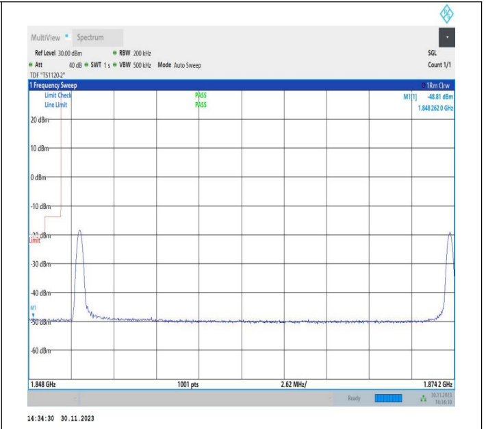
5MHz-20MHz_QPSK@QPSK-QPSK@QPSK_18633-18750_1RB#0@25RB#0-1RB#99@100RB#0
