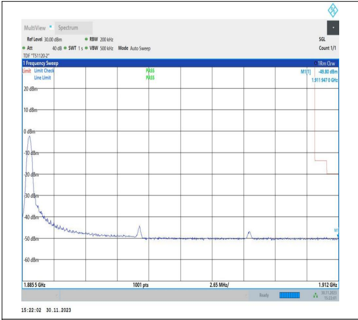
10MHz-15MHz_16QAM@16QAM-16QAM@16QAM_19005-19125_1RB#0@50RB#0-0RB#0@75RB#0
