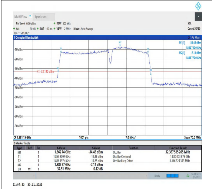
2-2-20MHz-15MHz-QPSK-QPSK-18826-18997-100RB#0-75R B#0-PASS
