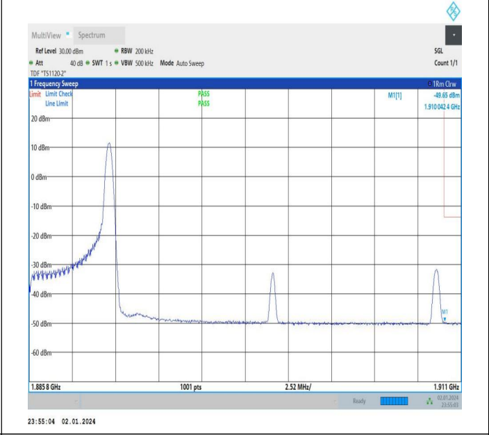
5MHz-20MHz_64QAM@64QAM-64QAM@64QAM_18983-19100_1RB#24@25RB#0-0RB#0@100RB#0
