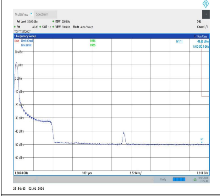
5MHz-20MHz_64QAM@64QAM-64QAM@64QAM_18983-19100_1RB#0@25RB#0-0RB#0@100RB#0
