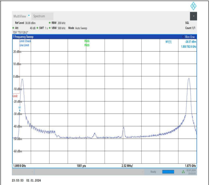
5MHz-20MHz_64QAM@64QAM-64QAM@64QAM_18633-18750_1RB#0@25RB#0-1RB#99@100RB#0
