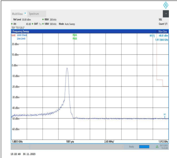
10MHz-15MHz_16QAM@16QAM-16QAM@16QAM_19005-19125_1RB#49@50RB#0-0RB#0@75RB#0
