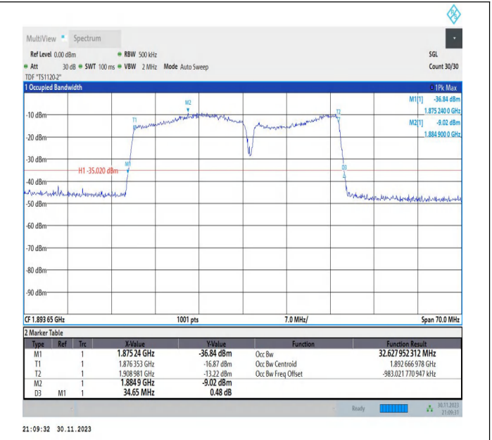
2-2-20MHz-15MHz-16QAM-16QAM-18951-19122-100RB#0-7 5RB#0-PASS
