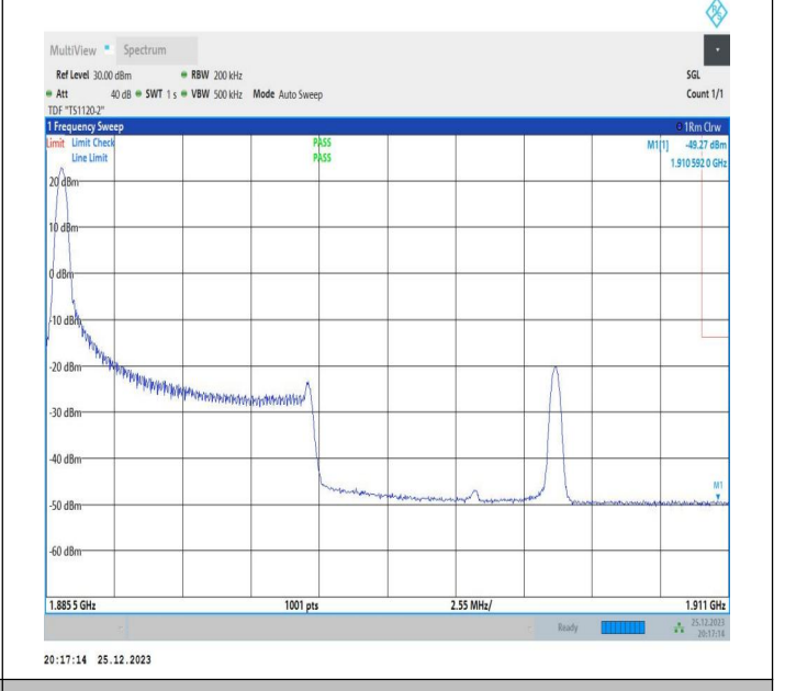
10MHz-15MHz_64QAM@64QAM-64QAM@64QAM_19005-19125_1RB#0@50RB#0-0RB#0@75RB#0
