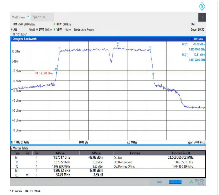
2-2-20MHz-15MHz-64QAM-64QAM-18951-19122-100RB#0-7 5RB#0-PASS
