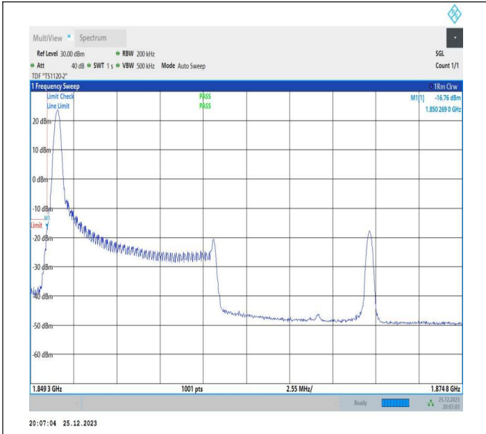
10MHz-15MHz_64QAM@64QAM-64QAM@64QAM_18653-18773_1RB#0@50RB#0-0RB#0@75RB#0
