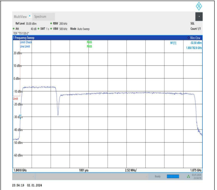
5MHz-20MHz_64QAM@64QAM-64QAM@64QAM_18633-18750_50_25RB#0@25RB#0-100RB#0@100RB#0
