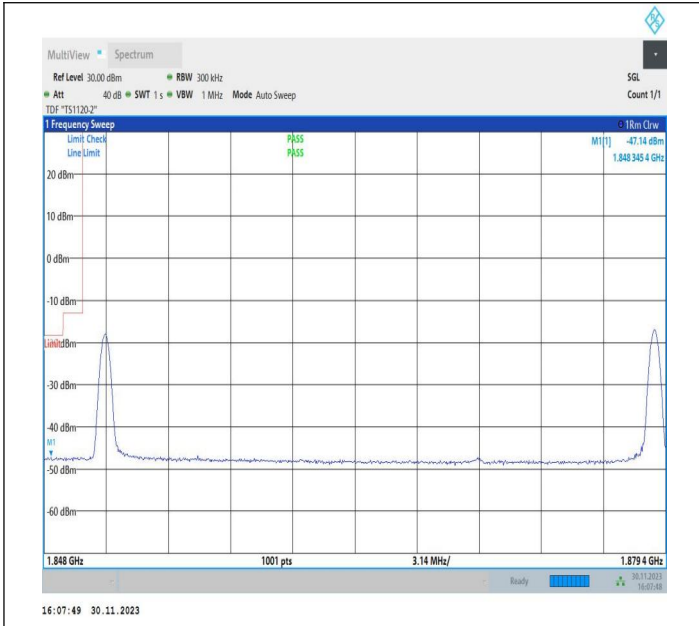
10MHz-20MHz_QPSK@QPSK-QPSK@QPSK_18655-18799_1RB#0@50RB#0-1RB#99@100RB#0
