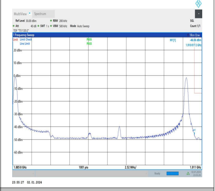
5MHz-20MHz_64QAM@64QAM-64QAM@64QAM_18983-19100_1RB#0@25RB#0-1RB#99@100RB#0
