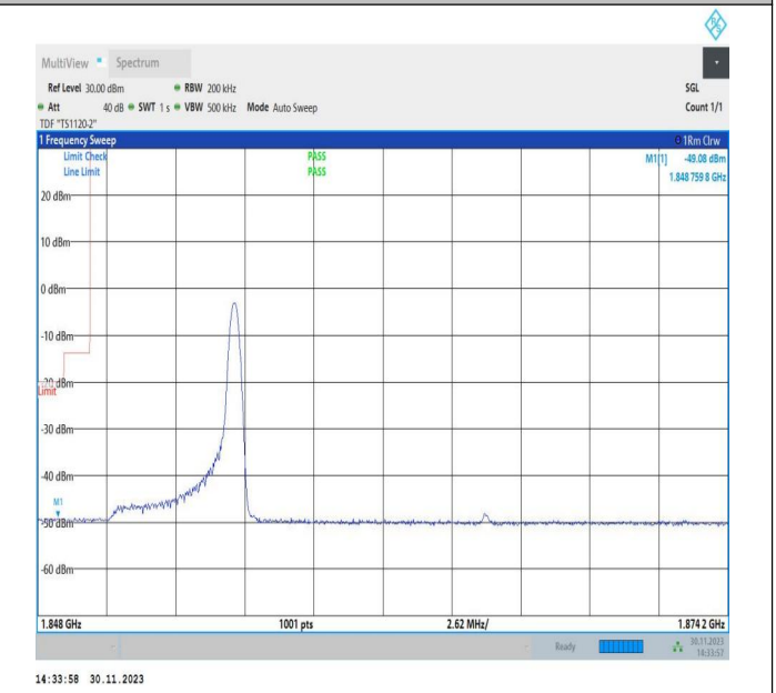
5MHz-20MHz_16QAM@16QAM-16QAM@16QAM_18633-187 50_1RB#24@25RB#0-0RB#0@100RB#0
