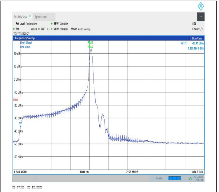
10MHz-15MHz_64QAM@64QAM-64QAM@64QAM_18653-18773_1RB#49@50RB#0-0RB#0@75RB#0
