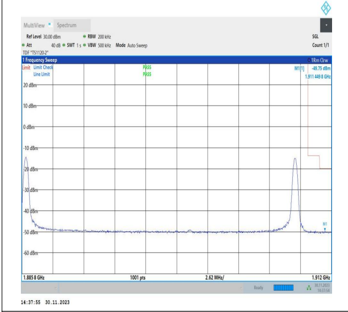
5MHz-20MHz_16QAM@16QAM-16QAM@16QAM_18983-19100_1RB#0@25RB#0-1RB#99@100RB#0
