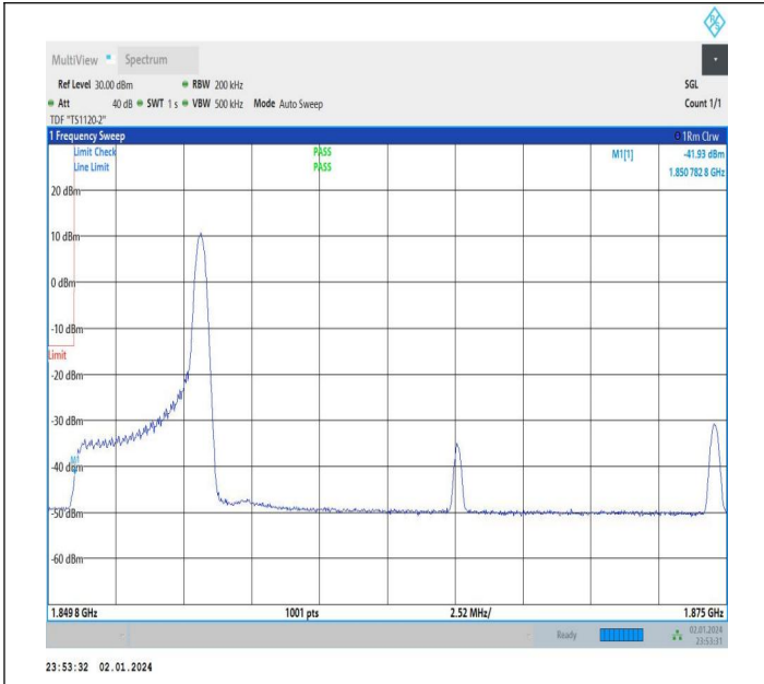
5MHz-20MHz_64QAM@64QAM-64QAM@64QAM_18633-18750_1RB#24@25RB#0-0RB#0@100RB#0
