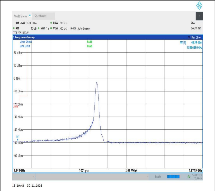
10MHz-15MHz_16QAM@16QAM-16QAM@16QAM_18653-18773_1RB#49@50RB#0-0RB#0@75RB#0
