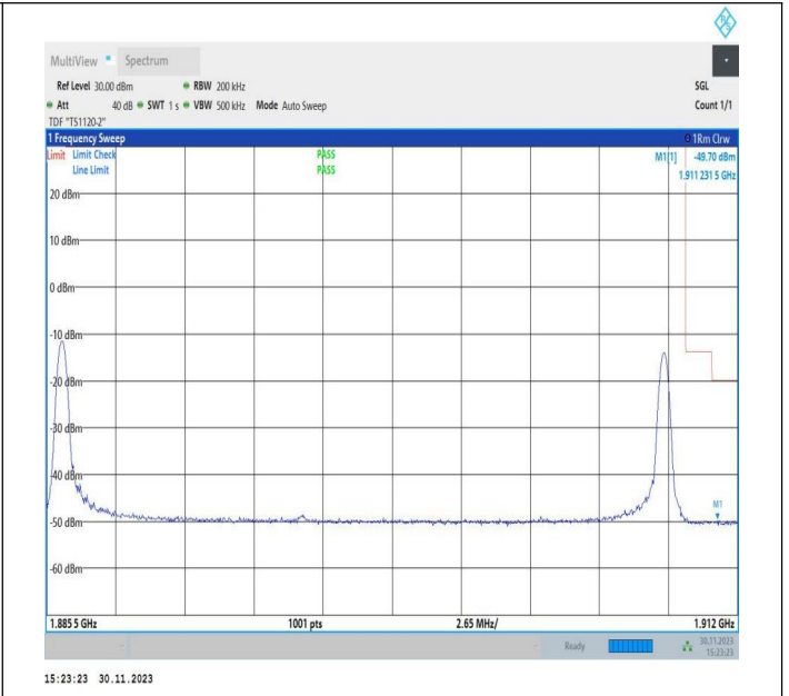
10MHz-15MHz_QPSK@QPSK-QPSK@QPSK_19005-19125_1RB#0@50RB#0-1RB#74@75RB#0
