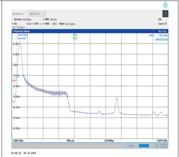
10MHz-20MHz_64QAM@64QAM-64QAM@64QAM_18655-18799_1RB#0@50RB#0-0RB#0@100RB#0
