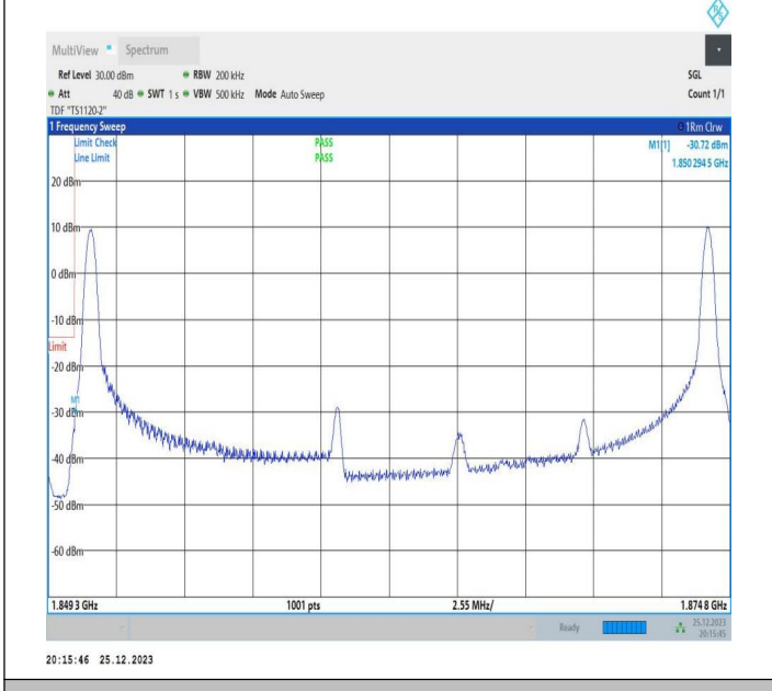
10MHz-15MHz_64QAM@64QAM-64QAM@64QAM_18653-18773_1RB#0@50RB#0-1RB#74@75RB#0
