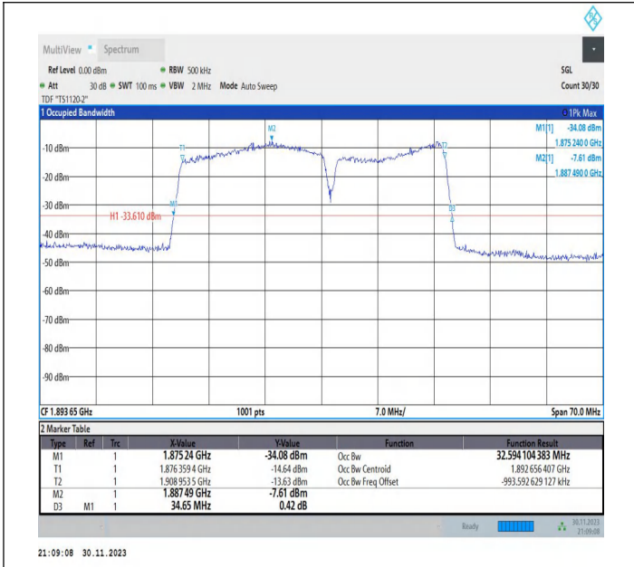
2-2-20MHz-15MHz-QPSK-QPSK-18951-19122-100RB#0-75R B#0-PASS
