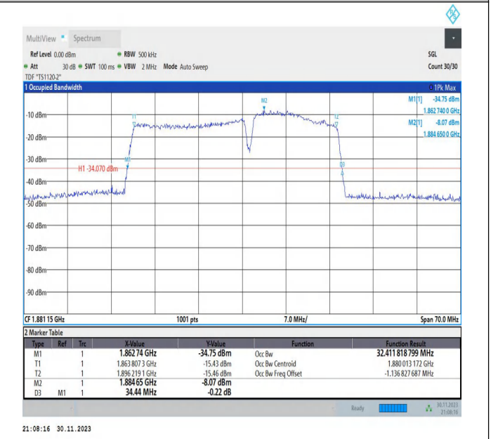
2-2-20MHz-15MHz-16QAM-16QAM-18826-18997-100RB#0-7 5RB#0-PASS
