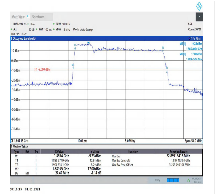
2-2-5MHz-20MHz-64QAM-64QAM-18983-19100-25RB#0-100 RB#0-PASS
