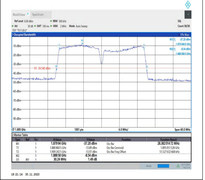
2-2-15MHz-15MHz-16QAM-16QAM-18975-19125-75RB#0-75 RB#0-PASS
