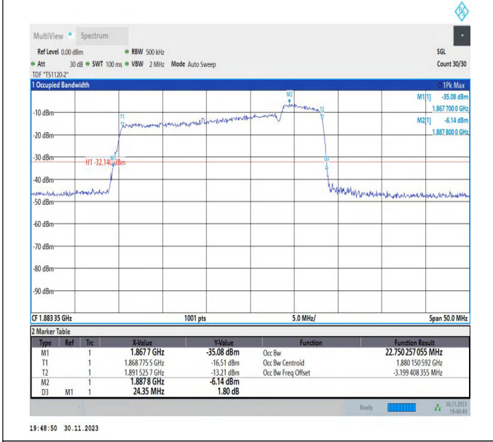
2-2-20MHz-5MHz-16QAM-16QAM-18875-18992-100RB#0-25 RB#0-PASS
