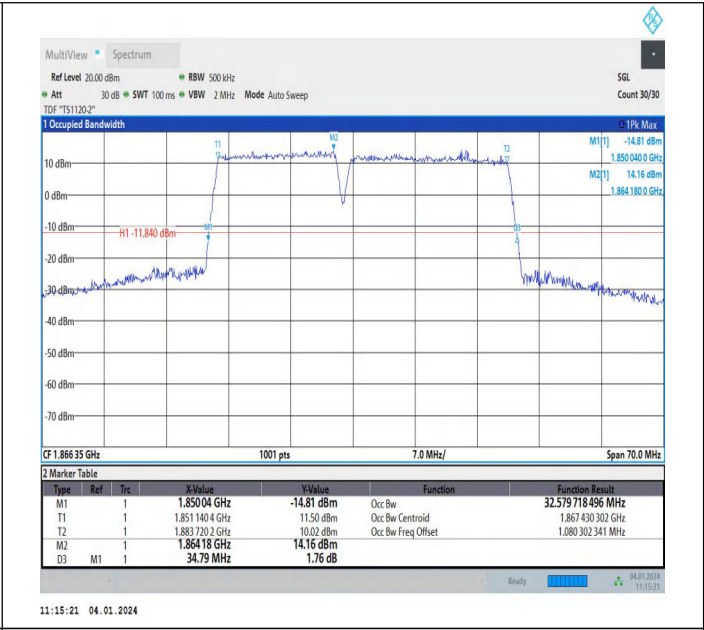
2-2-15MHz-20MHz-64QAM-64QAM-18678-18849-75RB#0-10 ORB#0-PASS
