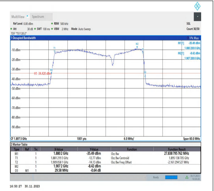
2-2-20MHz-10MHz-16QAM-16QAM-19001-19145-100RB#0-5 ORB#0-PASS
