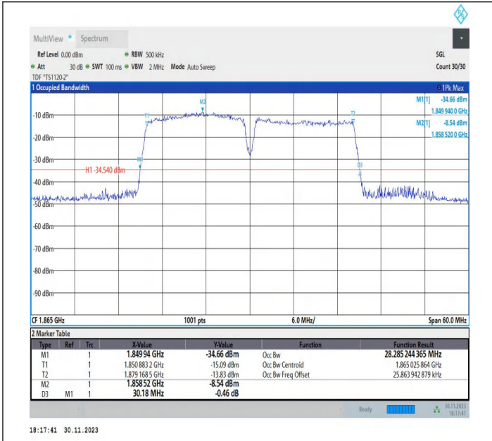
2-2-15MHz-15MHz-16QAM-16QAM-18675-18825-75RB#0-75 RB#0-PASS
