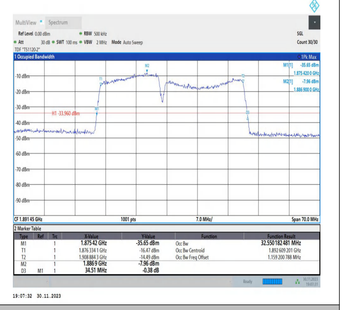
2-2-15MHz-20MHz-16QAM-16QAM-18929-19100-75RB#0-10 ORB#0-PASS
