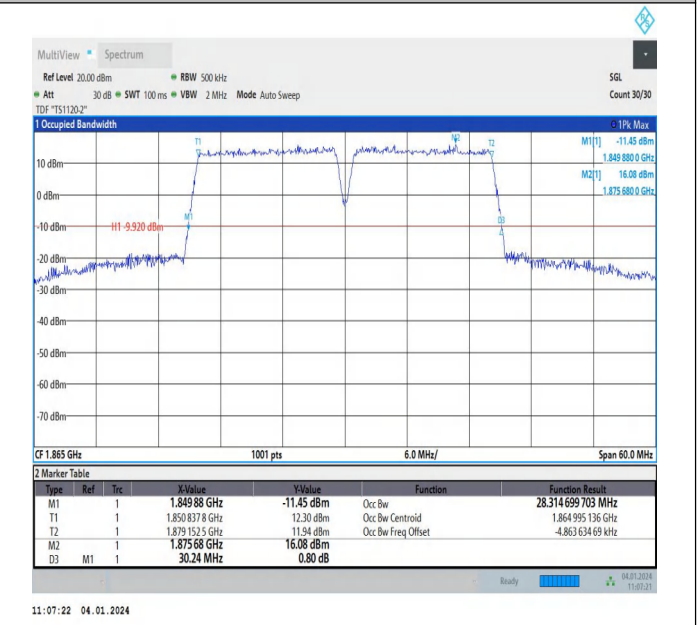
2-2-15MHz-15MHz-64QAM-64QAM-18675-18825-75RB#0-75 RB#0-PASS
