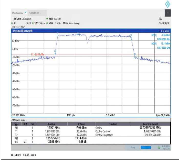
2-2-10MHz-15MHz-64QAM-64QAM-18653-18773-50RB#0-75 RB#0-PASS
