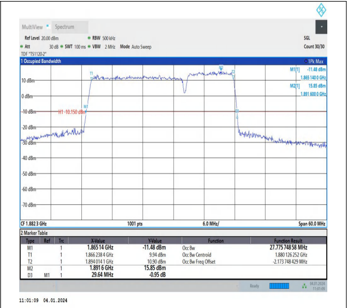
2-2-20MHz-10MHz-64QAM-64QAM-18851-18995-100RB#0-5 ORB#0-PASS
