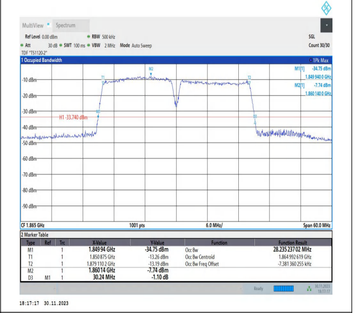
2-2-15MHz-15MHz-QPSK-QPSK-18675-18825-75RB#0-75RB #0-PASS
