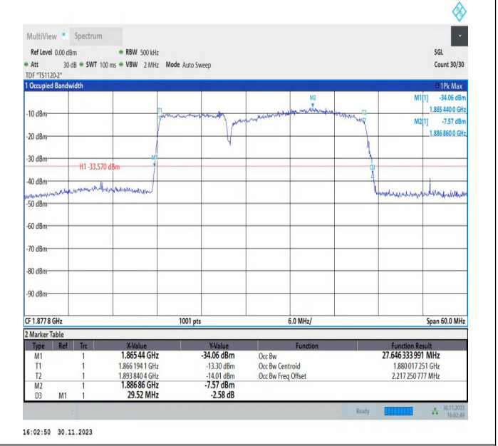
2-2-10MHz-20MHz-QPSK-QPSK-18806-18950-50RB#0-100R B#0-PASS
