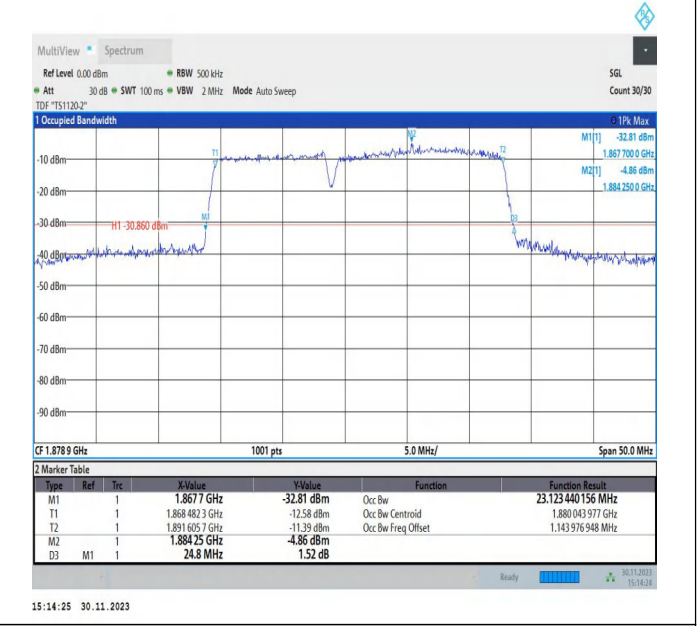
2-2-10MHz-15MHz-16QAM-16QAM-18829-18949-50RB#0-75 RB#0-PASS
