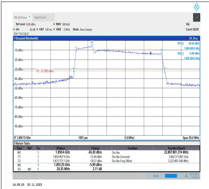
2-2-5MHz-20MHz-QPSK-QPSK-18633-18750-25RB#0-100RB #0-PASS
