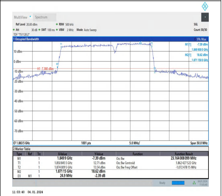
2-2-15MHz-10MHz-64QAM-64QAM-18675-18795-75RB#0-50 RB#0-PASS
