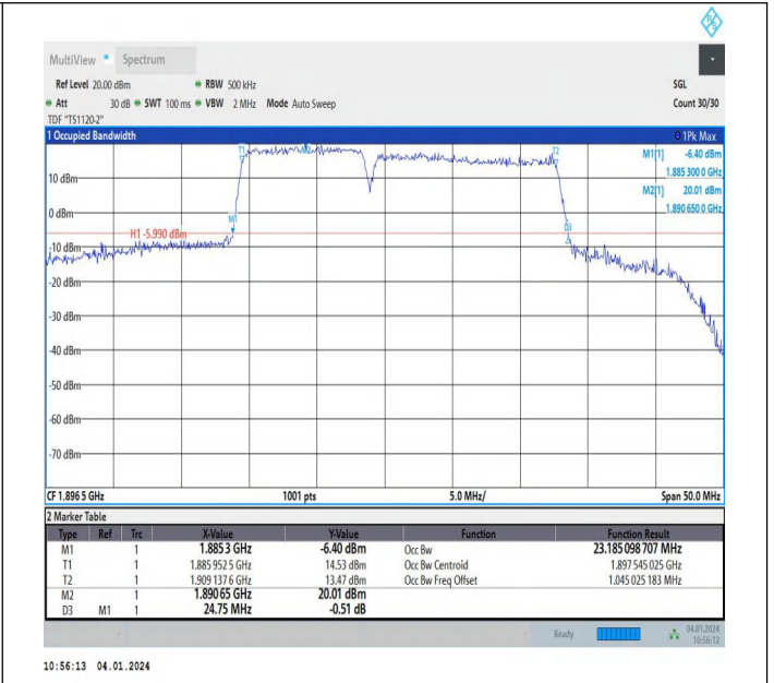
2-2-10MHz-15MHz-64QAM-64QAM-19005-19125-50RB#0-75 RB#0-PASS
