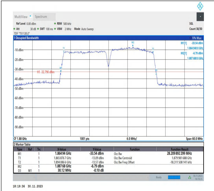
2-2-15MHz-15MHz-QPSK-QPSK-18825-18975-75RB#0-75RB #0-PASS
