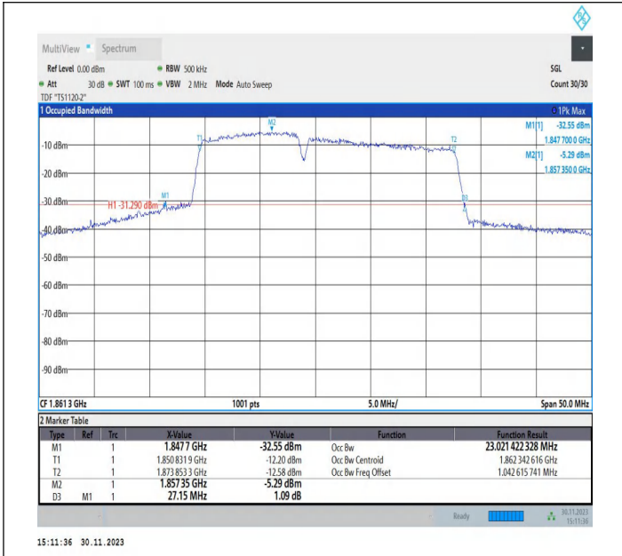
2-2-10MHz-15MHz-QPSK-QPSK-18653-18773-50RB#0-75RB #0-PASS
