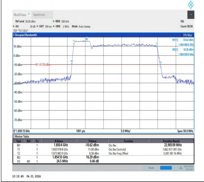
2-2-5MHz-20MHz-64QAM-64QAM-18633-18750-25RB#0-100RB#0-PASS
