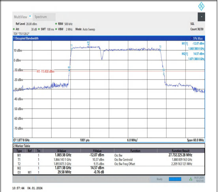
2-2-10MHz-20MHz-64QAM-64QAM-18806-18950-50RB#0-10 ORB#0-PASS
