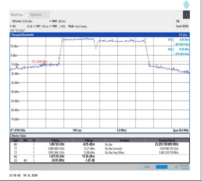
2-2-10MHz-15MHz-64QAM-64QAM-18829-18949-50RB#0-75 RB#0-PASS
