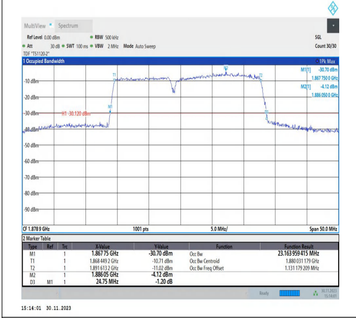
2-2-10MHz-15MHz-QPSK-QPSK-18829-18949-50RB#0-75RB #0-PASS
