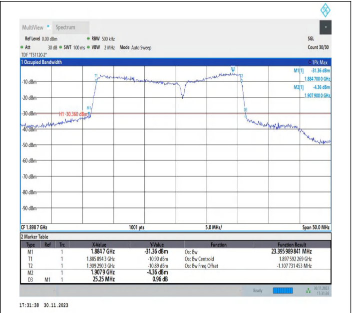
2-2-15MHz-10MHz-QPSK-QPSK-19027-19147-75RB#0-50RB #0-PASS
