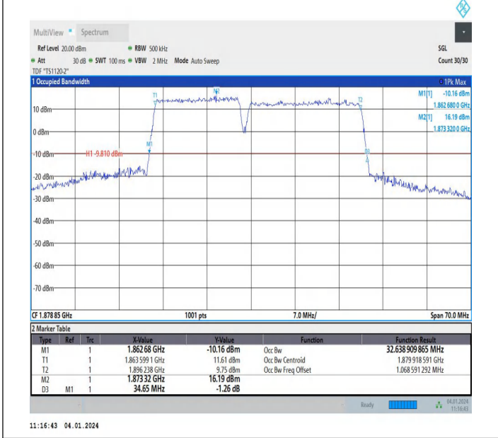
2-2-15MHz-20MHz-64QAM-64QAM-18803-18974-75RB#0-10 ORB#0-PASS
