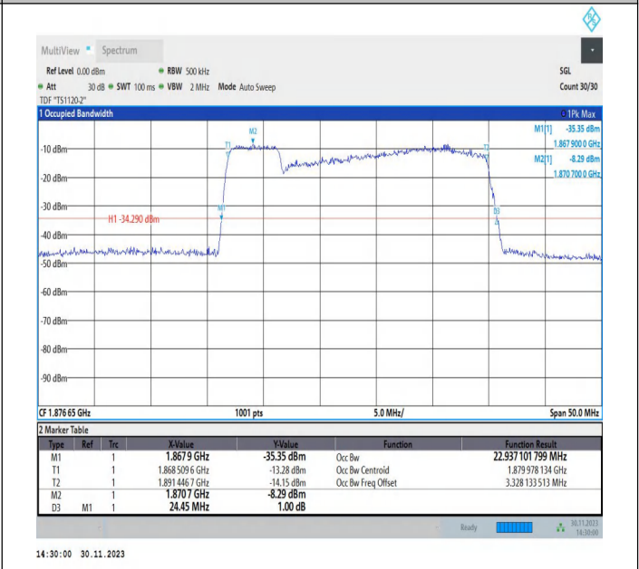
2-2-5MHz-20MHz-16QAM-16QAM-18808-18925-25RB#0-100RB#0-PASS
