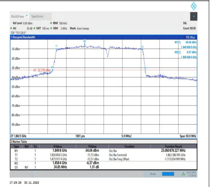
2-2-15MHz-10MHz-16QAM-16QAM-18675-18795-75RB#0-50 RB#0-PASS
