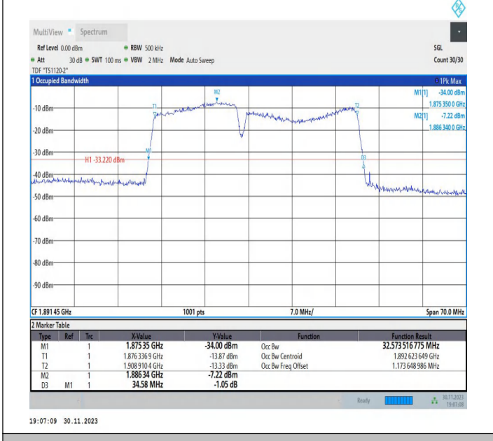
2-2-15MHz-20MHz-QPSK-QPSK-18929-19100-75RB#0-100R B#0-PASS
