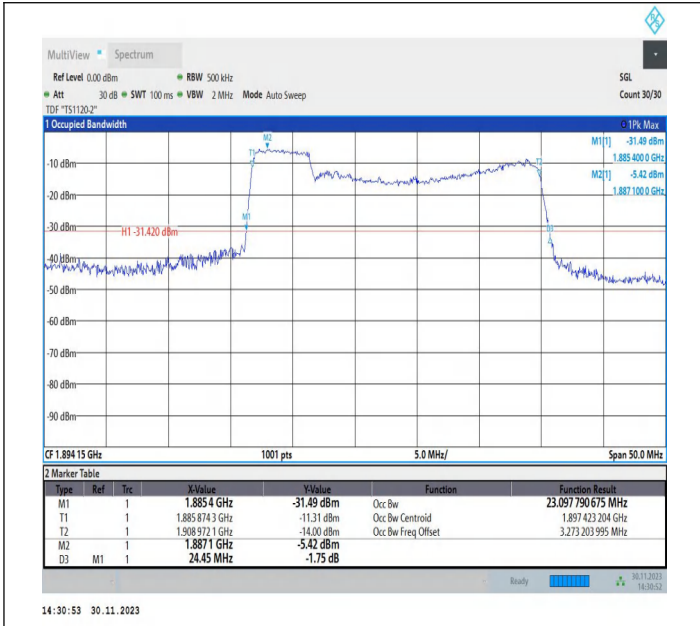
2-2-5MHz-20MHz-QPSK-QPSK-18983-19100-25RB#0-100RB #0-PASS
