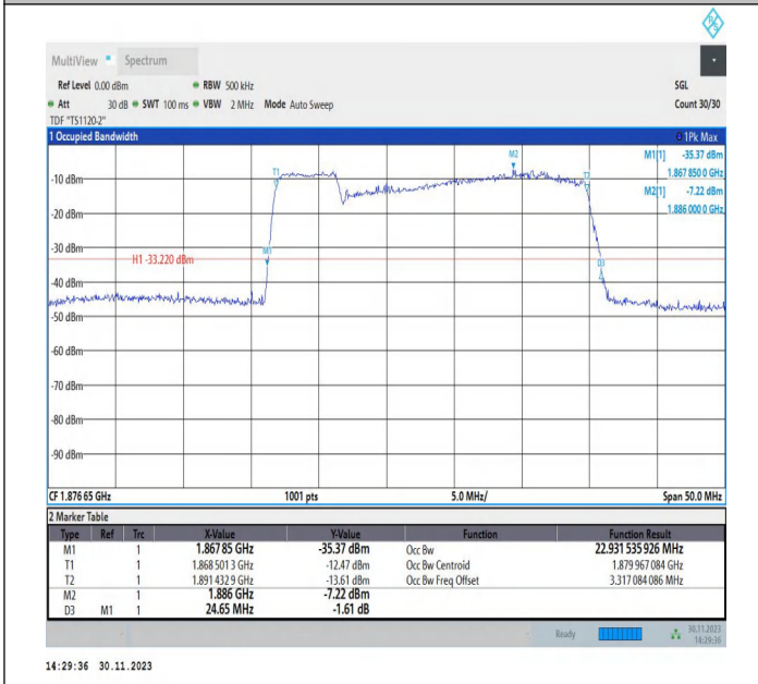
2-2-5MHz-20MHz-QPSK-QPSK-18808-18925-25RB#0-100RB #0-PASS
