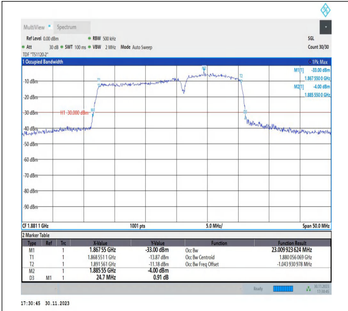
2-2-15MHz-10MHz-16QAM-16QAM-18851-18971-75RB#0-50 RB#0-PASS
