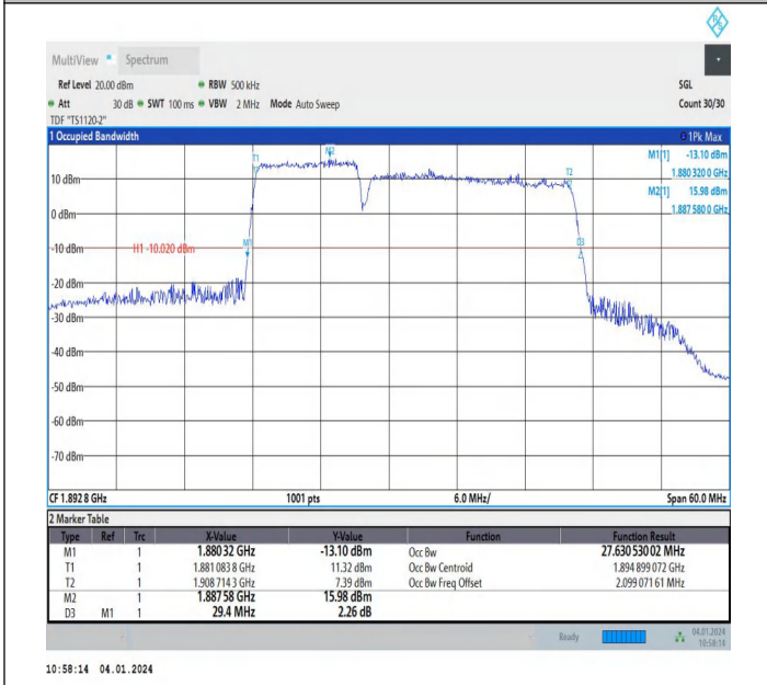
2-2-10MHz-20MHz-64QAM-64QAM-18956-19100-50RB#0-10 ORB#0-PASS
