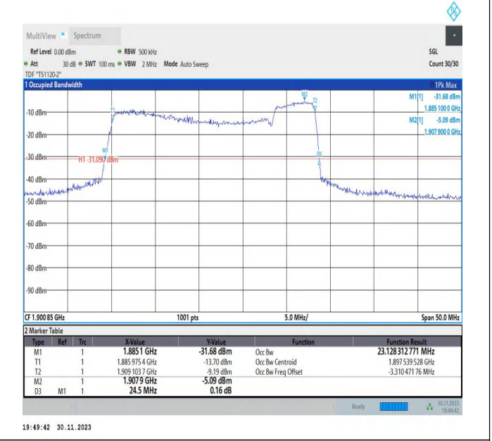
2-2-20MHz-5MHz-QPSK-QPSK-19050-19167-100RB#0-25RB #0-PASS
