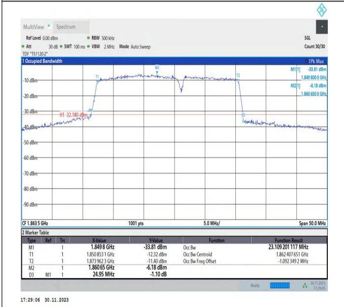
2-2-15MHz-10MHz-QPSK-QPSK-18675-18795-75RB#0-50RB #0-PASS
