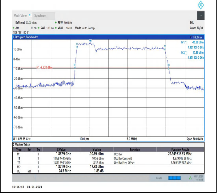
2-2-5MHz-20MHz-64QAM-64QAM-18808-18925-25RB#0-100RB#0-PASS
