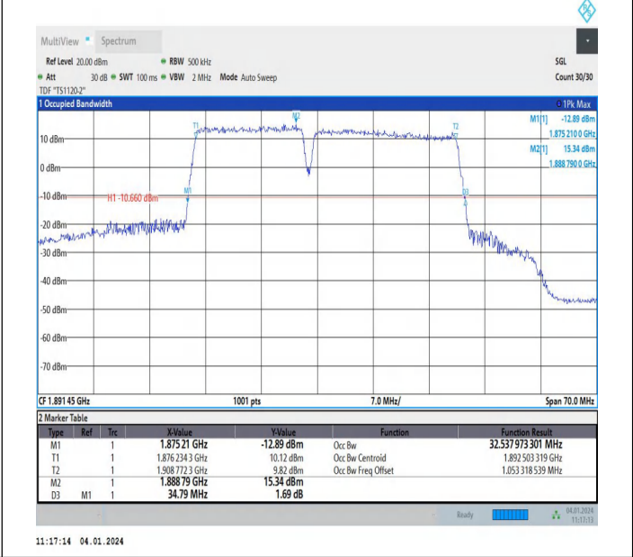
2-2-15MHz-20MHz-64QAM-64QAM-18929-19100-75RB#0-10 ORB#0-PASS
