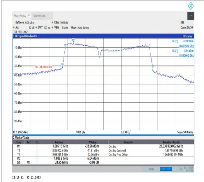
2-2-10MHz-15MHz-16QAM-16QAM-19005-19125-50RB#0-75 RB#0-PASS
