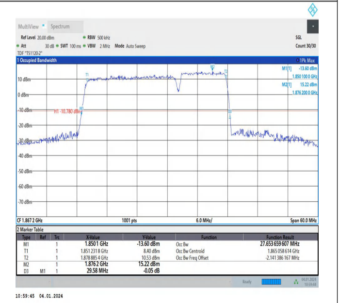
2-2-20MHz-10MHz-64QAM-64QAM-18700-18844-100RB#0-5 ORB#0-PASS
