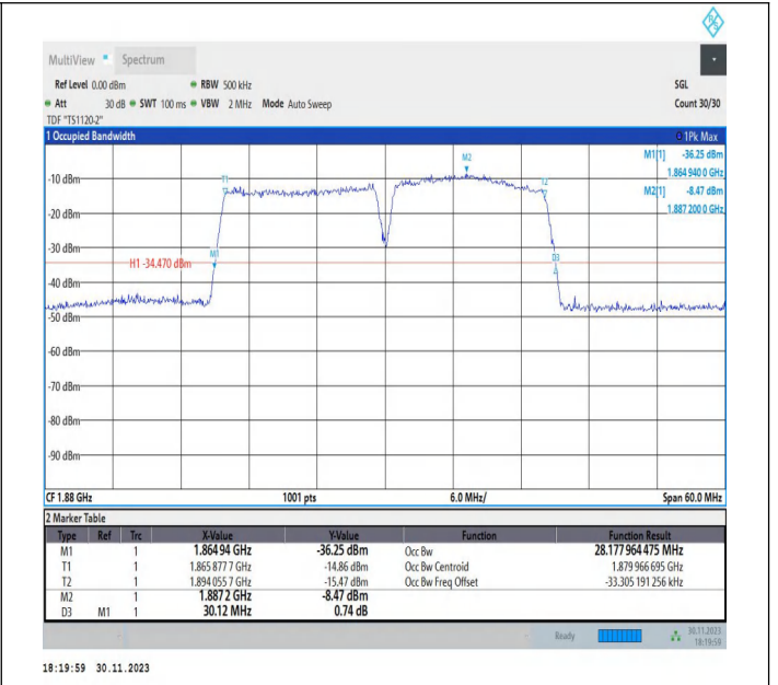
2-2-15MHz-15MHz-16QAM-16QAM-18825-18975-75RB#0-75 RB#0-PASS
