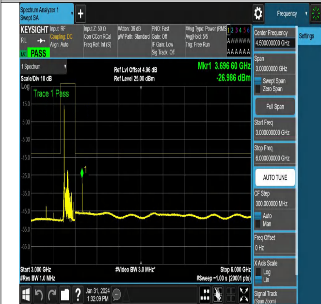
NTNV_N78-3450-3550_PC2_30_100_M_TID17_NS_01_3000_6000_#1
