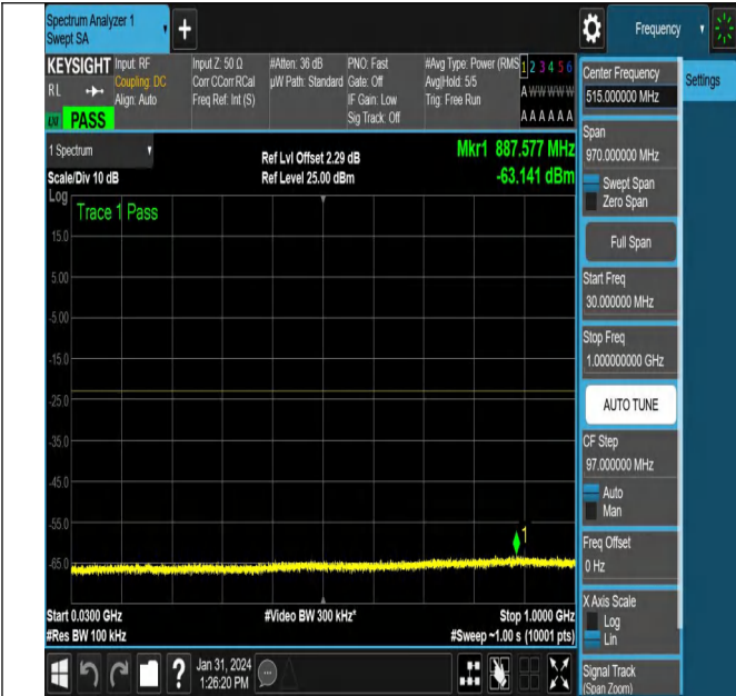
NTNV_N78-3450-3550_PC2_30_100_M_TID2_NS_01_30_10_00_#1
