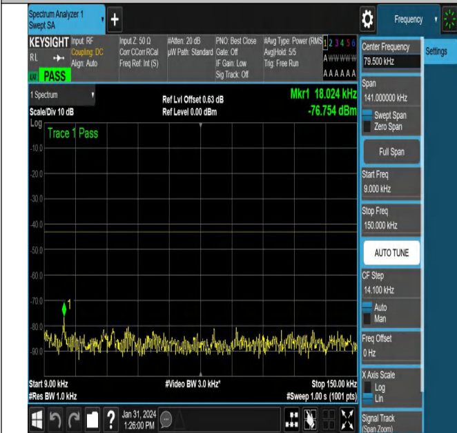
NTVN_N78-3450-3550_PC2_30_100_M_TID2_NS_01_0.009_0.15_#1
