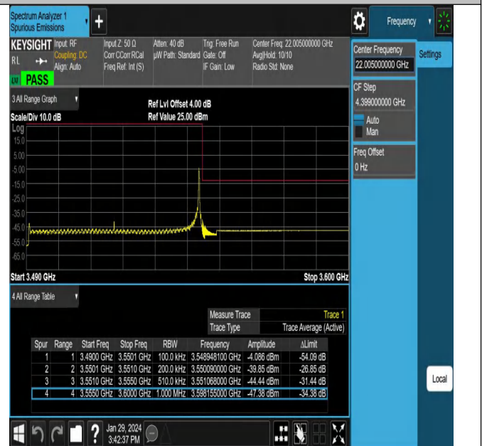
NTNV_N78-3450-3550_PC2_30_60_H_TID27_#1
