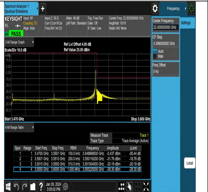
NTNV_N78-3450-3550_PC2_30_80_H_TID9_#1
