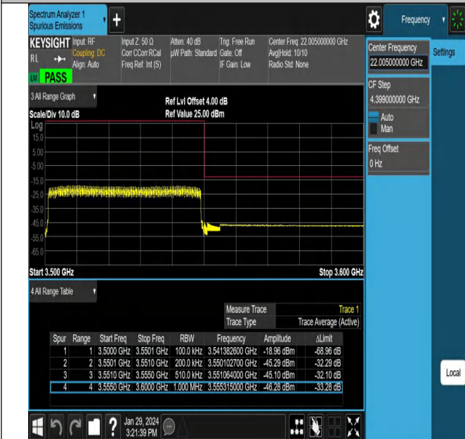
NTNV_N78-3450-3550_PC2_30_50_H_TID19_#1
