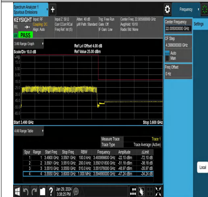
NTNV_N78-3450-3550_PC2_30_60_H_TID13_#1
