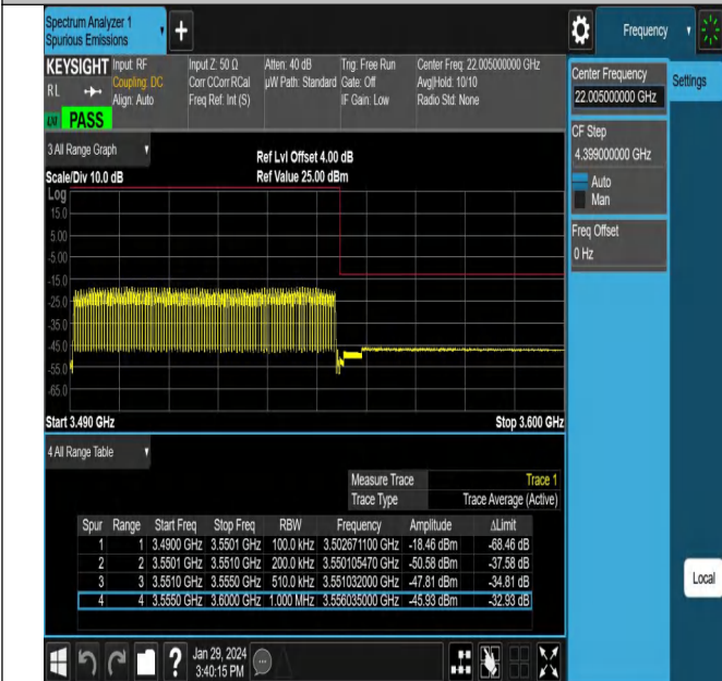
NTNV_N78-3450-3550_PC2_30_60_H_TID19_#1
