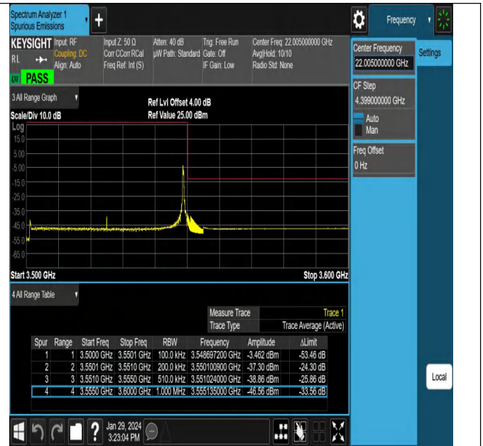
NTNV_N78-3450-3550_PC2_30_50_H_TID24_#1
