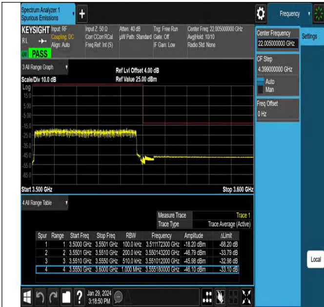
NTNV_N78-3450-3550_PC2_30_50_H_TID10_#1
