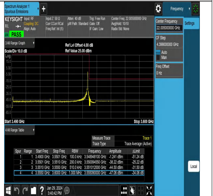
NTNV_N78-3450-3550_PC2_30_60_H_TID21_#1
