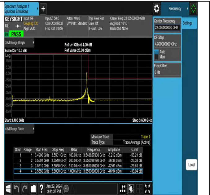
NTNV_N78-3450-3550_PC2_30_60_H_TID24_#1
