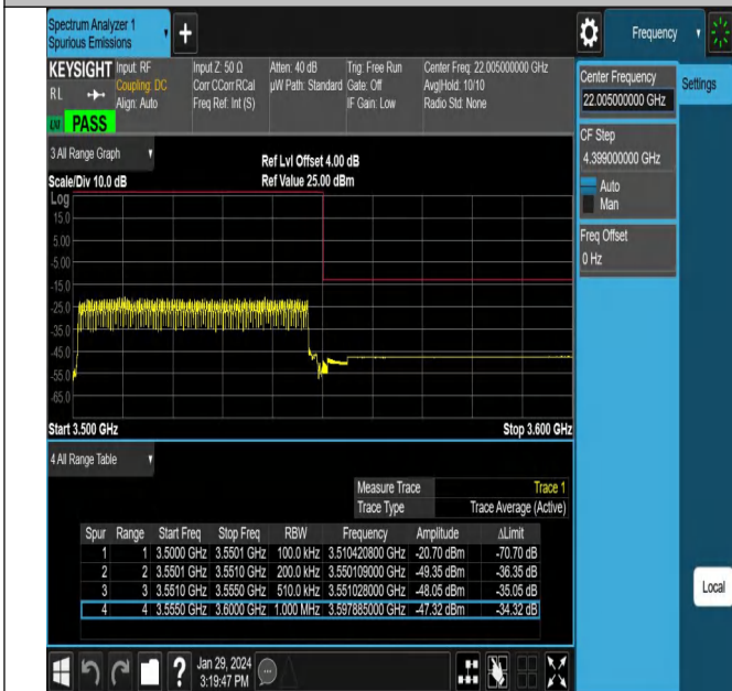
NTNV_N78-3450-3550_PC2_30_50_H_TID13_#1
