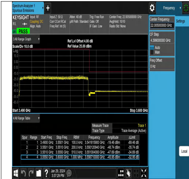
NTNV_N78-3450-3550_PC2_30_60_H_TID10_#1
