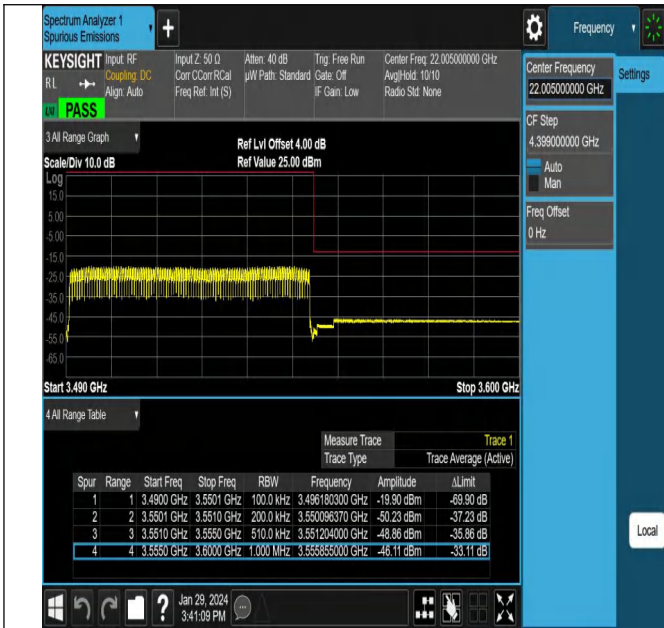
NTNV_N78-3450-3550_PC2_30_60_H_TID22_#1
