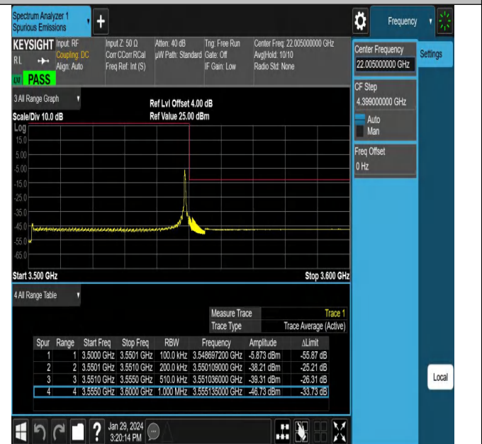
NTNV_N78-3450-3550_PC2_30_50_H_TID15_#1
