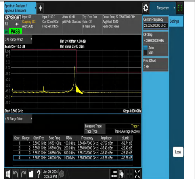
NTNV_N78-3450-3550_PC2_30_50_H_TID21_#1
