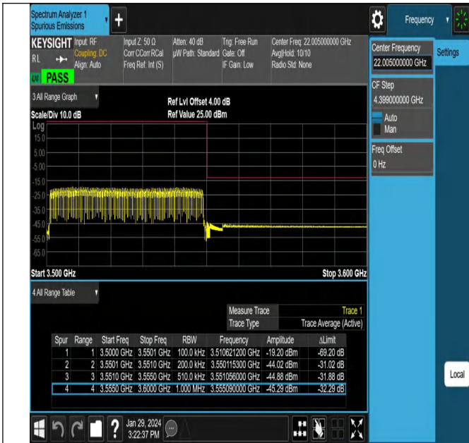
NTNV_N78-3450-3550_PC2_30_50_H_TID22_#1
