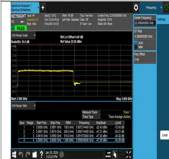
NTNV_N78-3450-3550_PC2_30_50_H_TID25_#1
