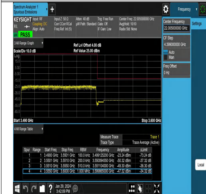
NTNV_N78-3450-3550_PC2_30_60_H_TID25_#1
