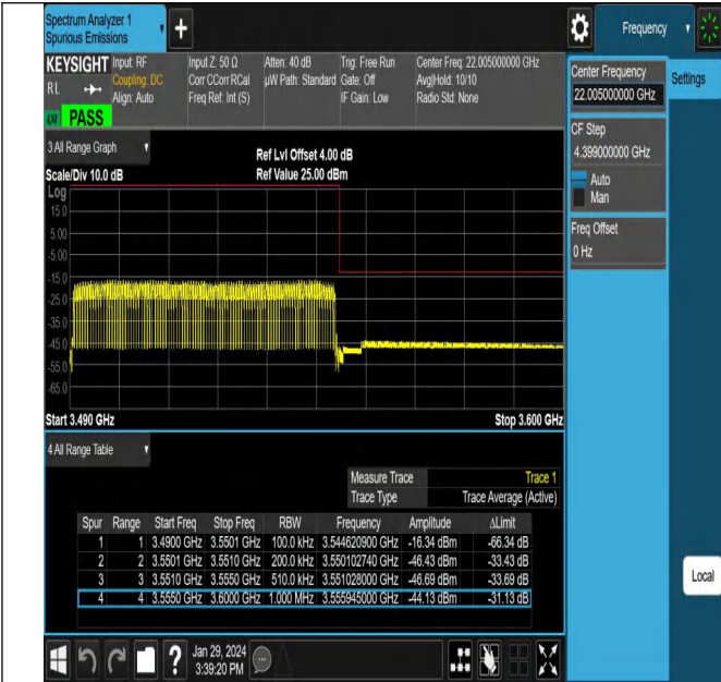
NTNV_N78-3450-3550_PC2_30_60_H_TID16_#1
