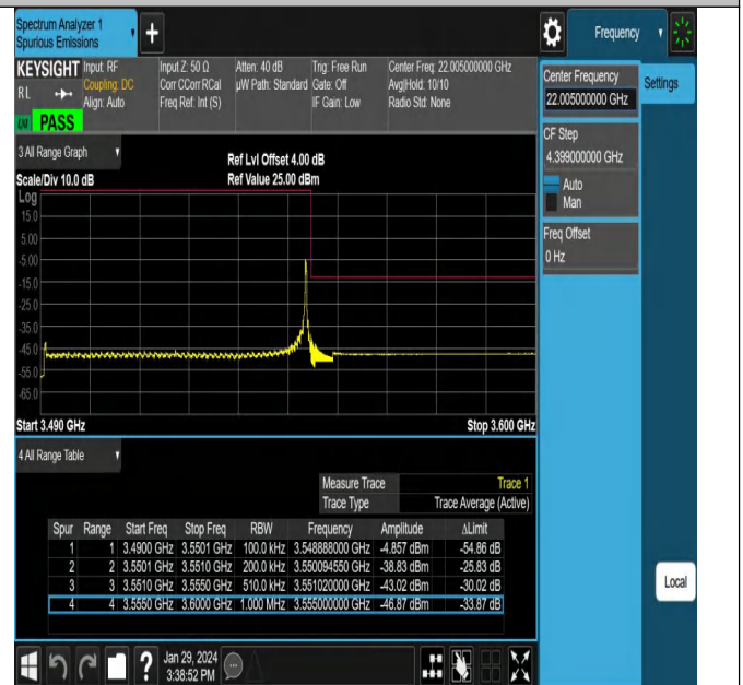
NTNV_N78-3450-3550_PC2_30_60_H_TID15_#1
