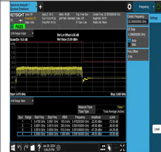
NTNV_N78-3450-3550_PC2_30_80_H_TID13_#1
