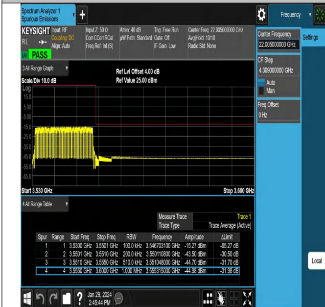
NTNV_N78-3450-3550_PC2_30_20_H_TID19_#1
