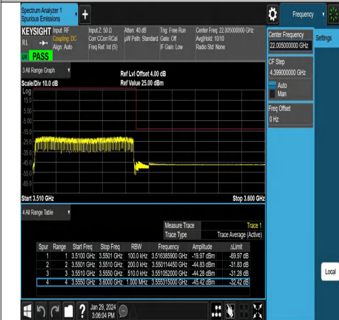
NTNV_N78-3450-3550_PC2_30_40_H_TID25_#1
