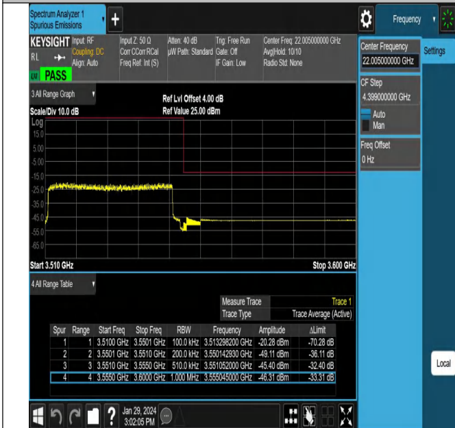
NTNV_N78-3450-3550_PC2_30_40_H_TID13_#1
