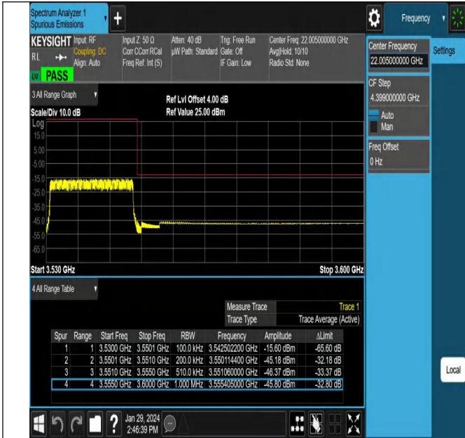
NTNV_N78-3450-3550_PC2_30_20_H_TID22_#1
