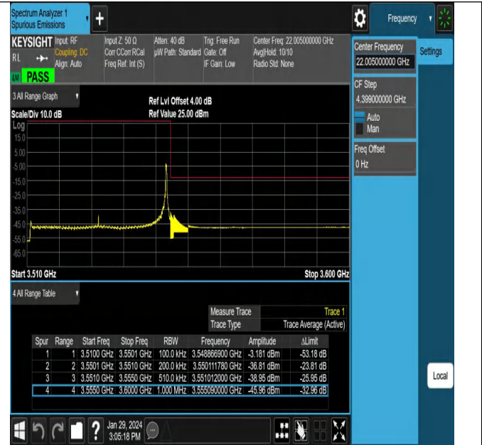
NTNV_N78-3450-3550_PC2_30_40_H_TID24_#1
