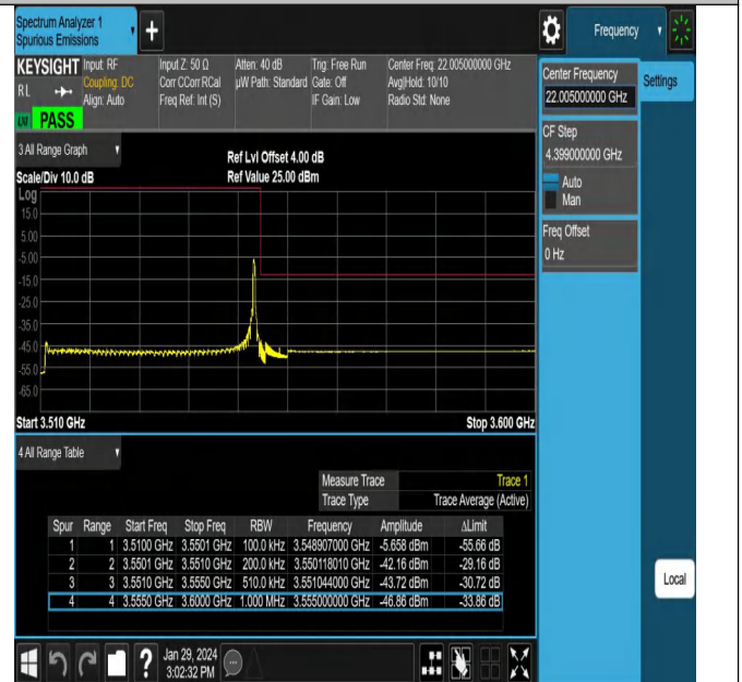
NTNV_N78-3450-3550_PC2_30_40_H_TID15_#1
