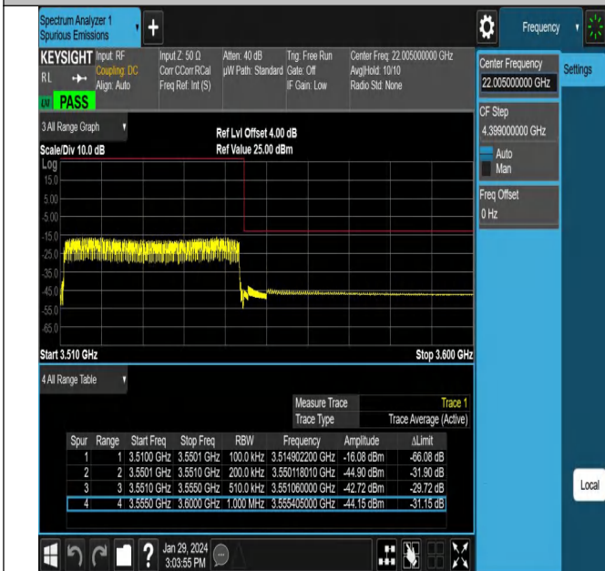
NTNV_N78-3450-3550_PC2_30_40_H_TID19_#1
