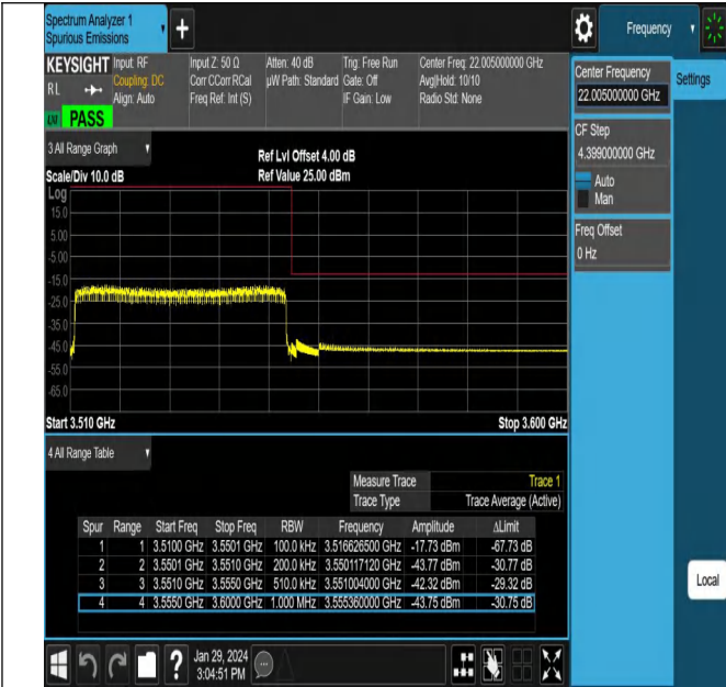
NTNV_N78-3450-3550_PC2_30_40_H_TID22_#1
