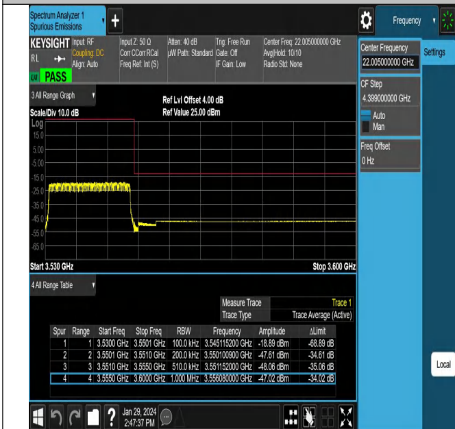
NTNV_N78-3450-3550_PC2_30_20_H_TID25_#1
