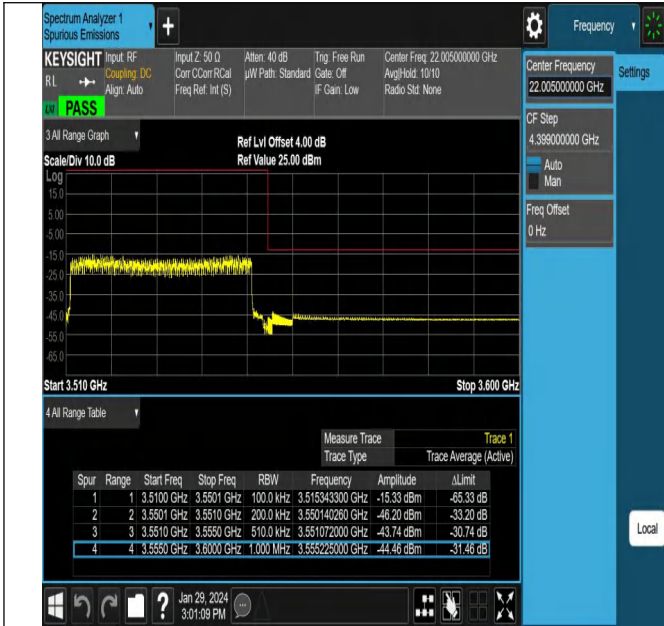
NTNV_N78-3450-3550_PC2_30_40_H_TID10_#1
