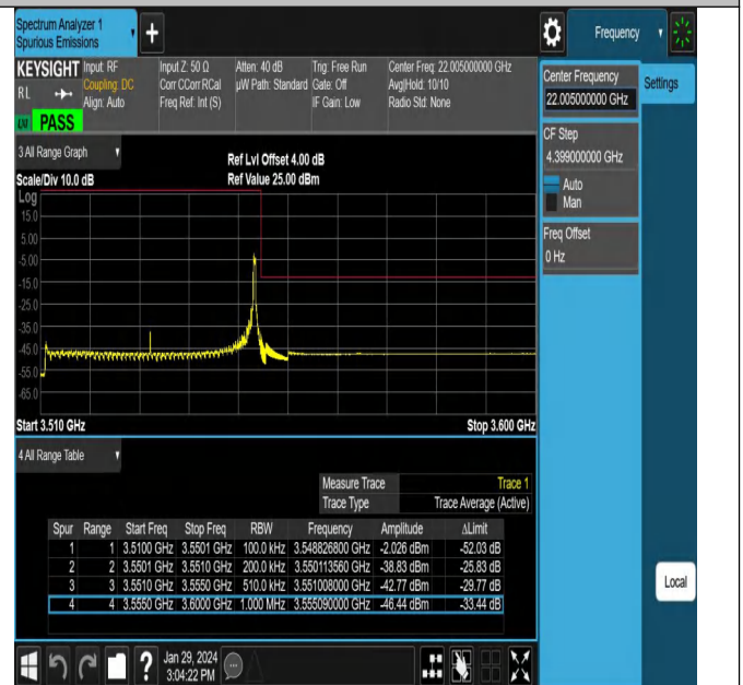
NTNV_N78-3450-3550_PC2_30_40_H_TID21_#1
