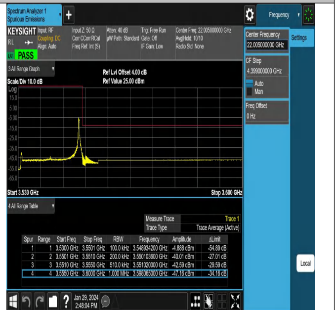
NTNV_N78-3450-3550_PC2_30_20_H_TID27_#1
