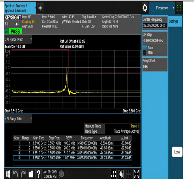
NTNV_N78-3450-3550_PC2_30_40_H_TID27_#1
