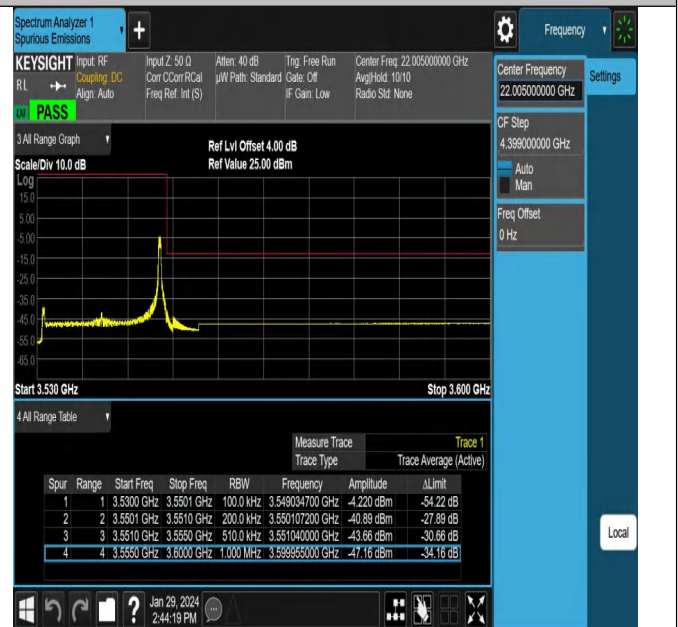
NTNV_N78-3450-3550_PC2_30_20_H_TID15_#1
