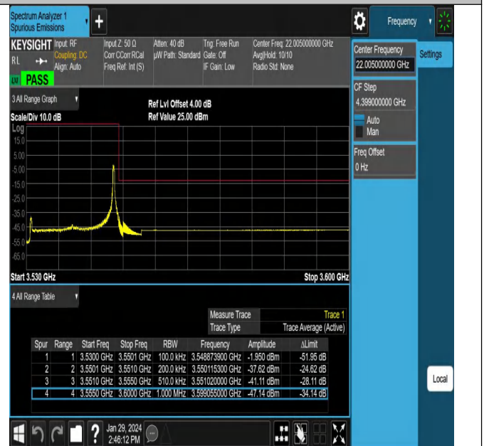
NTNV_N78-3450-3550_PC2_30_20_H_TID21_#1
