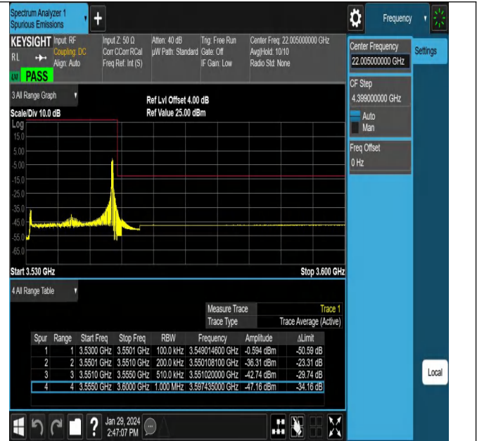
NTNV_N78-3450-3550_PC2_30_20_H_TID24_#1
