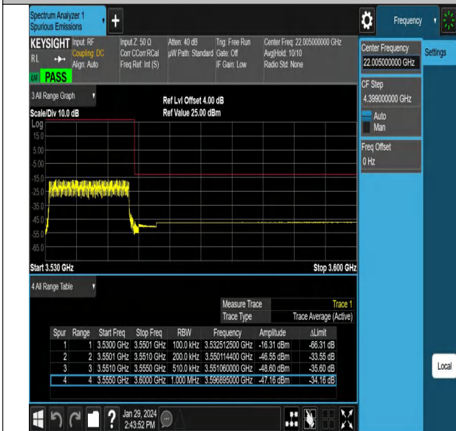
NTNV_N78-3450-3550_PC2_30_20_H_TID13_#1
