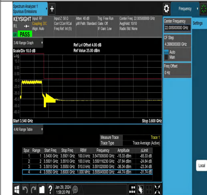
NTNV_N78-3450-3550_PC2_30_10_H_TID13_#1
