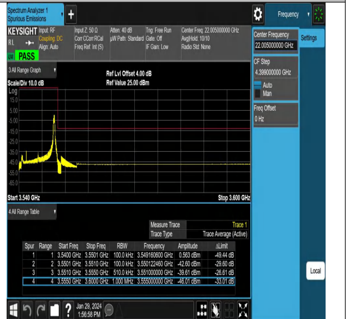
NTNV_N78-3450-3550_PC2_30_10_H_TID9_#1
