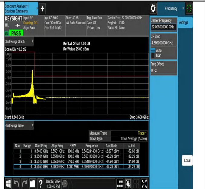
NTNV_N78-3450-3550_PC2_30_10_H_TID15_#1
