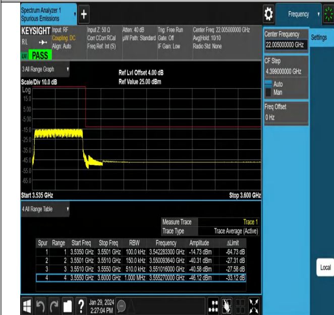
NTNV_N78-3450-3550_PC2_30_15_H_TID19_#1
