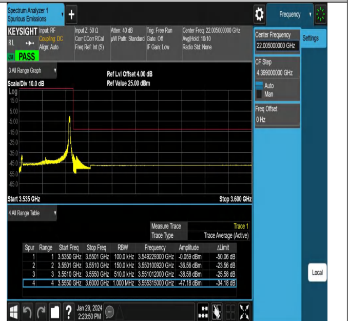
NTNV_N78-3450-3550_PC2_30_15_H_TID9_#1
