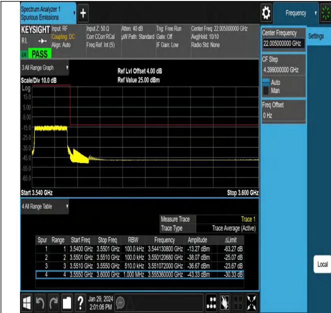
NTNV_N78-3450-3550_PC2_30_10_H_TID22_#1
