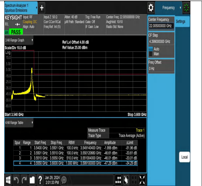
NTNV_N78-3450-3550_PC2_30_10_H_TID24_#1
