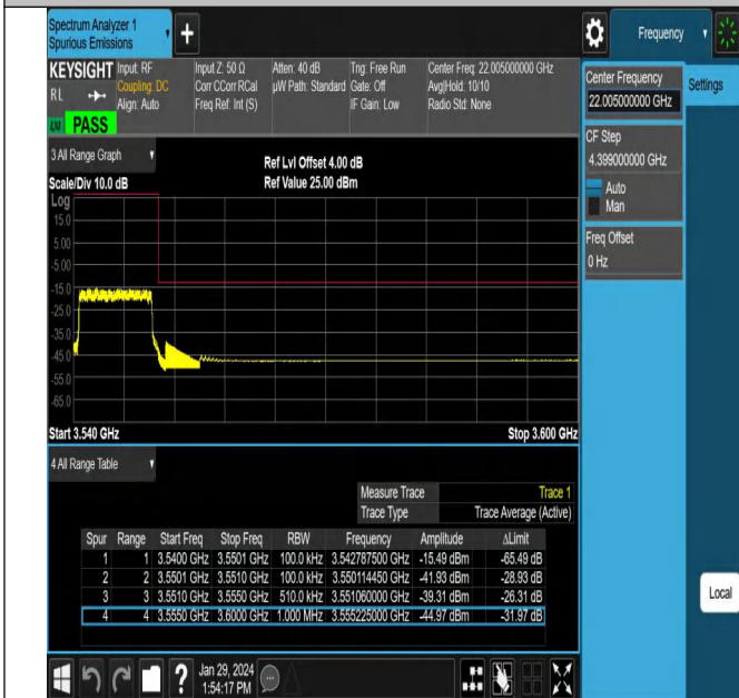
NTNV_N78-3450-3550_PC2_30_10_H_TID1_#1
