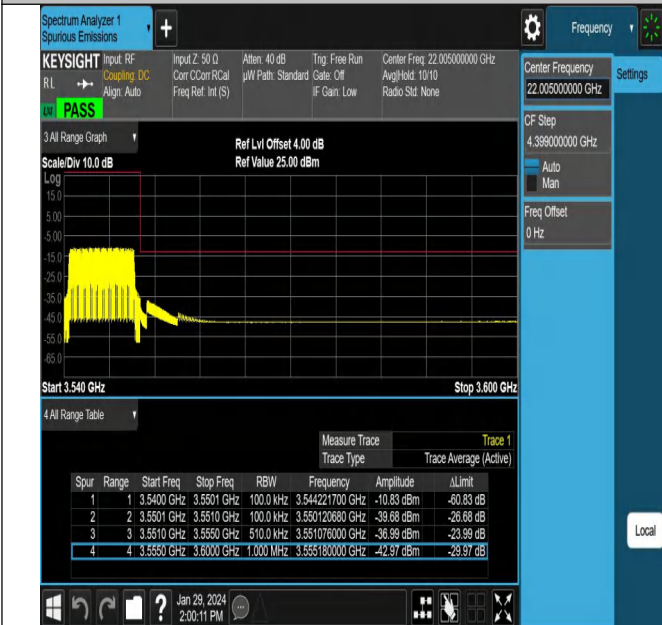
NTNV_N78-3450-3550_PC2_30_10_H_TID19_#1
