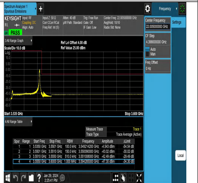
NTNV_N78-3450-3550_PC2_30_15_H_TID15_#1
