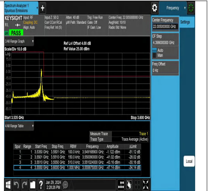
NTNV_N78-3450-3550_PC2_30_15_H_TID24_#1
