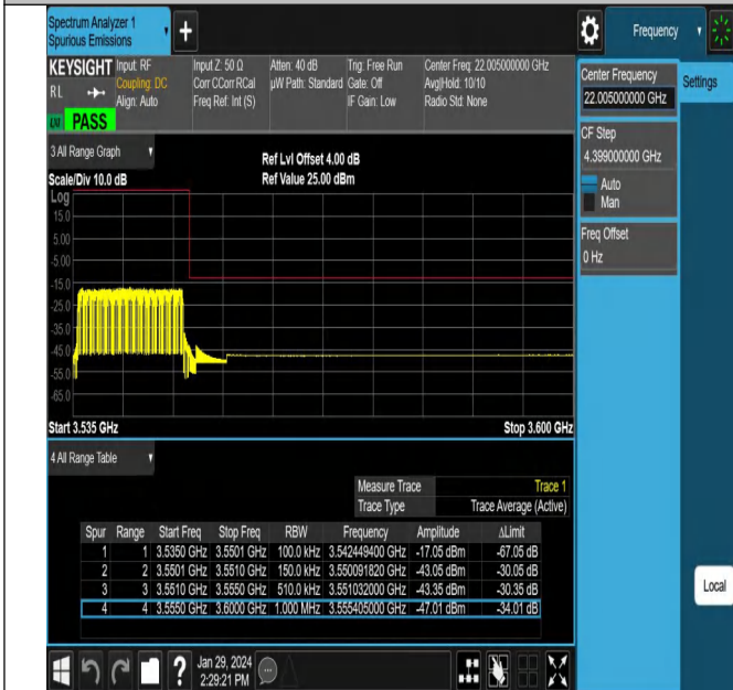
NTNV_N78-3450-3550_PC2_30_15_H_TID25_#1
