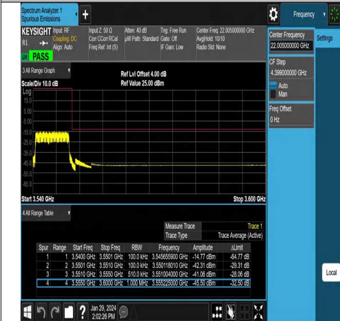
NTNV_N78-3450-3550_PC2_30_10_H_TID25_#1
