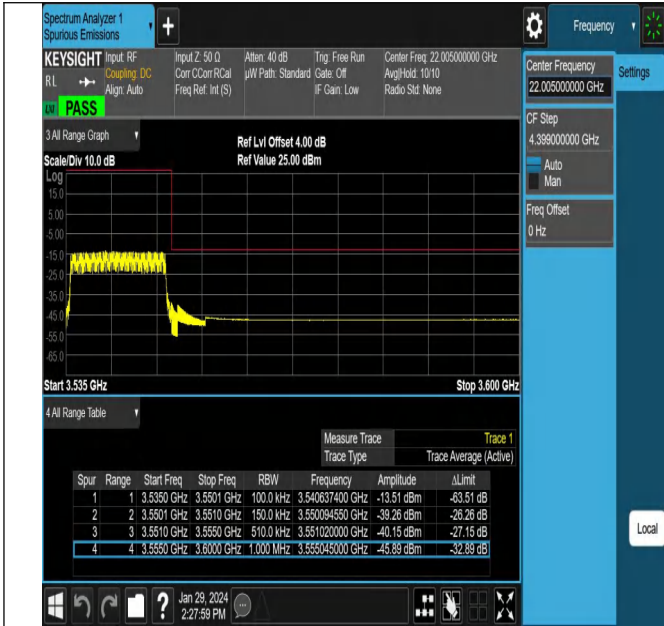
NTNV_N78-3450-3550_PC2_30_15_H_TID22_#1
