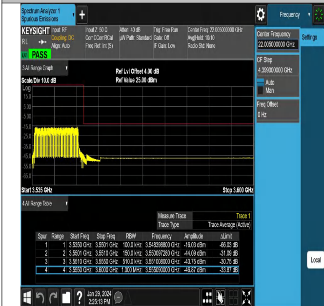
NTNV_N78-3450-3550_PC2_30_15_H_TID13_#1
