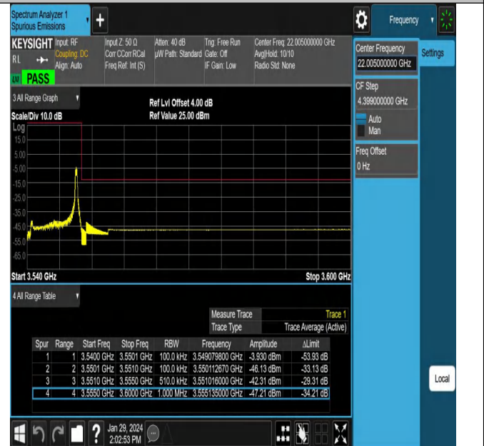
NTNV_N78-3450-3550_PC2_30_10_H_TID27_#1
