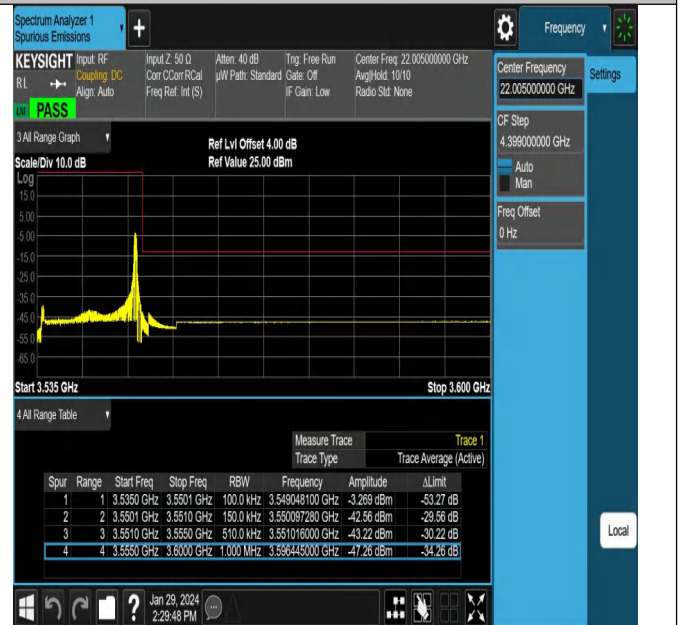
NTNV_N78-3450-3550_PC2_30_15_H_TID27_#1
