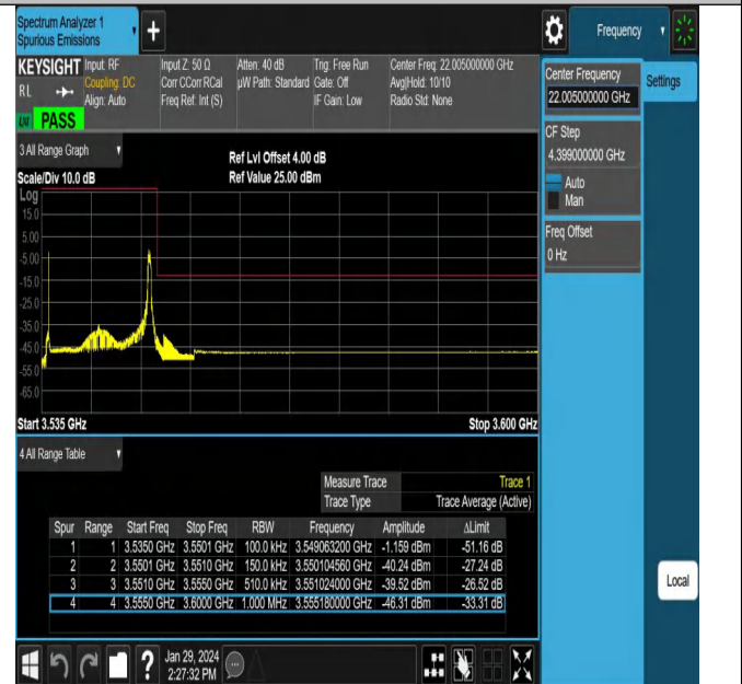
NTNV_N78-3450-3550_PC2_30_15_H_TID21_#1
