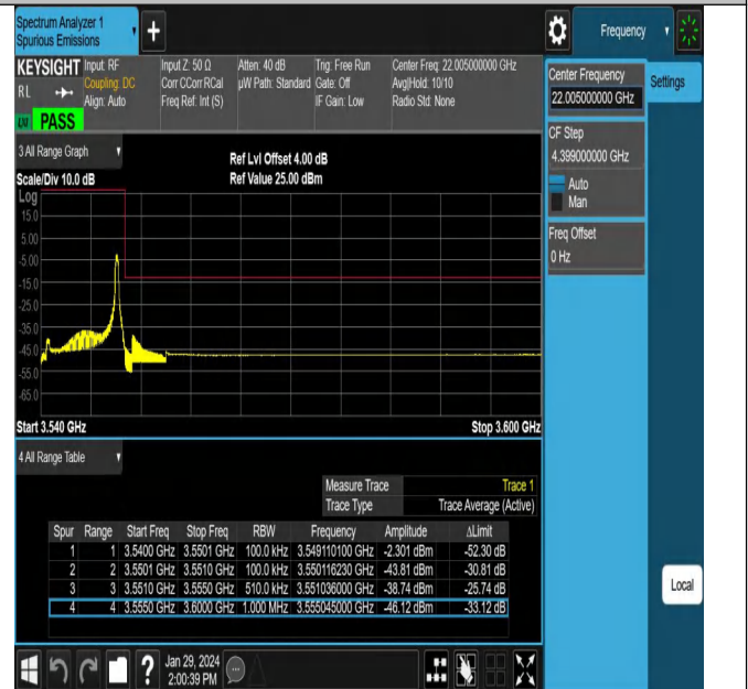
NTNV_N78-3450-3550_PC2_30_10_H_TID21_#1
