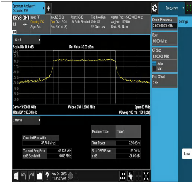
NTV_N78-3450-3550_PC2_30_40_M_TID9_Ant1#1
