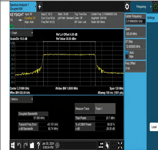
NTV_N78-3450-3550_PC_30_60_H_TID4_Ant1#1
