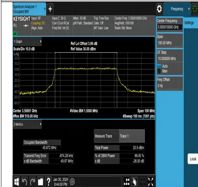
NTV_N78-3450-3550_PC2_30_50_M_TID4_Ant1#1
