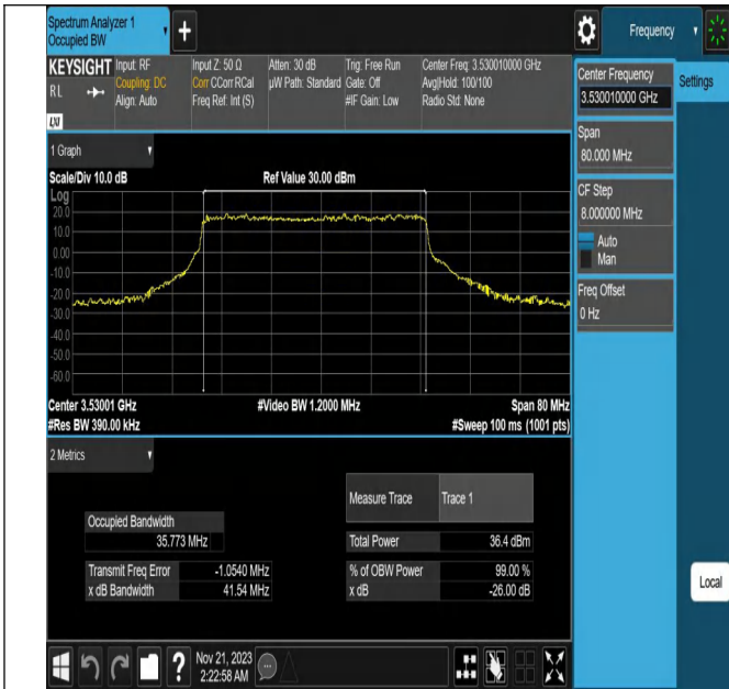
NTV_N78-3450-3550_PC_30_40_H_TID4_Ant1#1
