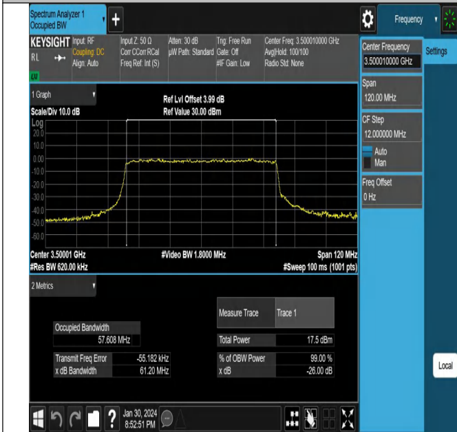
NTV_N78-3450-3550_PC_30_60_M_TID1_Ant1#1
