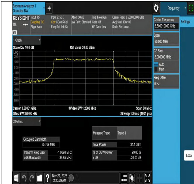
NTV_N78-3450-3550_PC2_30_40_M_TID5_Ant1#1
