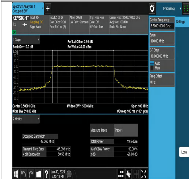
NTV_N78-3450-3550_PC2_30_50_M_TID8_Ant1#1
