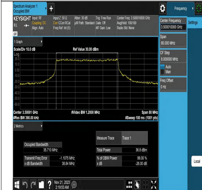
NTV_N78-3450-3550_PC2_30_40_M_TID3_Ant1#1
