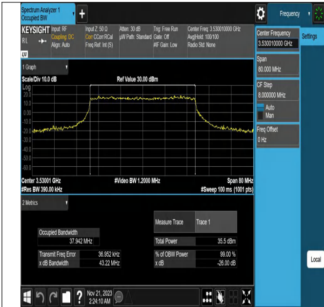
NTV_N78-3450-3550_PC2_30_40_H_TID8_Ant1#1
