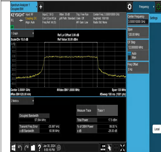
NTV_N78-3450-3550_PC2_30_60_M_TID9_Ant1#1
