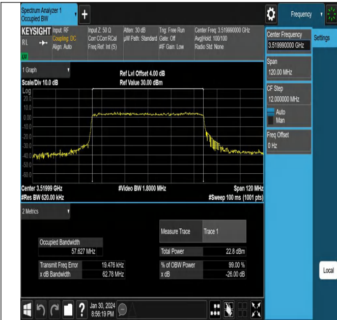
NTV_N78-3450-3550_PC_30_60_H_TID2_Ant1#1
