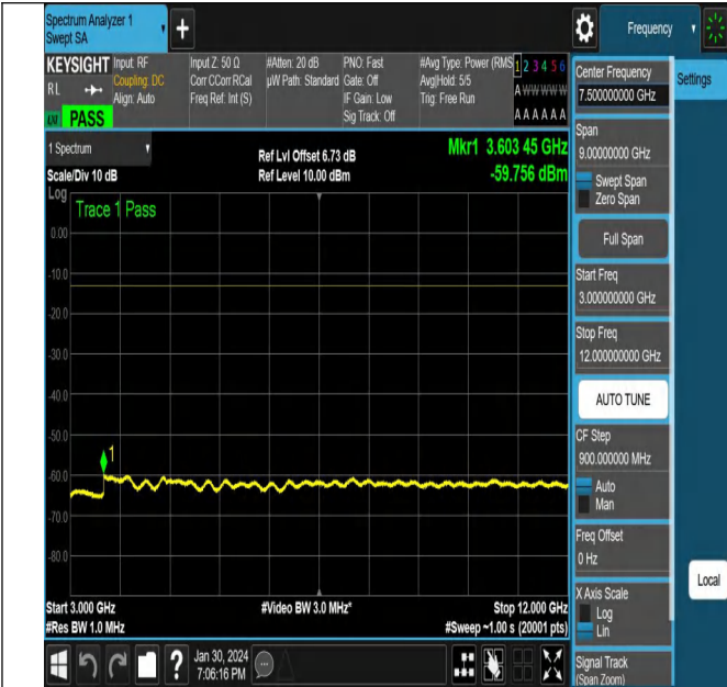
NTNV_N71_PC3_15_20_M_TID17_NS_01_3000_12000_#1
