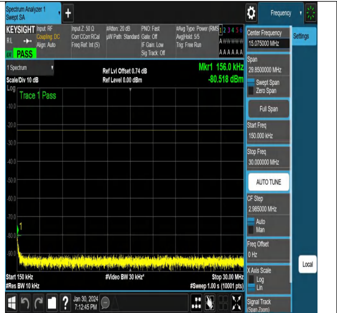
NTNV_N71_PC3_15_20_H_TID17_NS_01_0.15_30_#1
