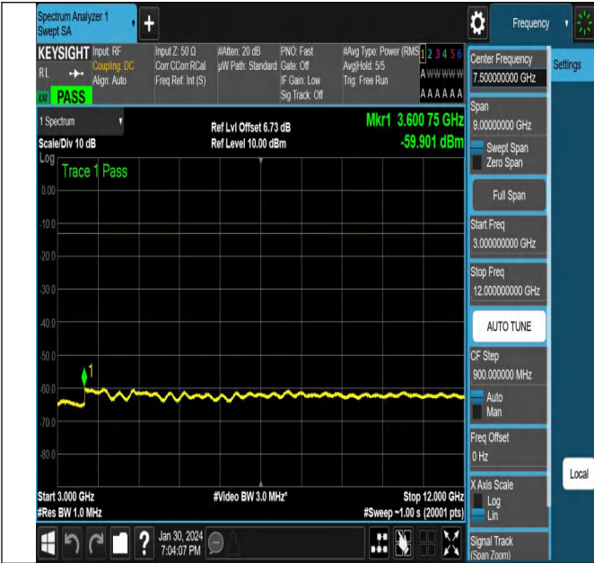
NTNV_N71_PC3_15_20_M_TID5_NS_01_3000_12000_#1
