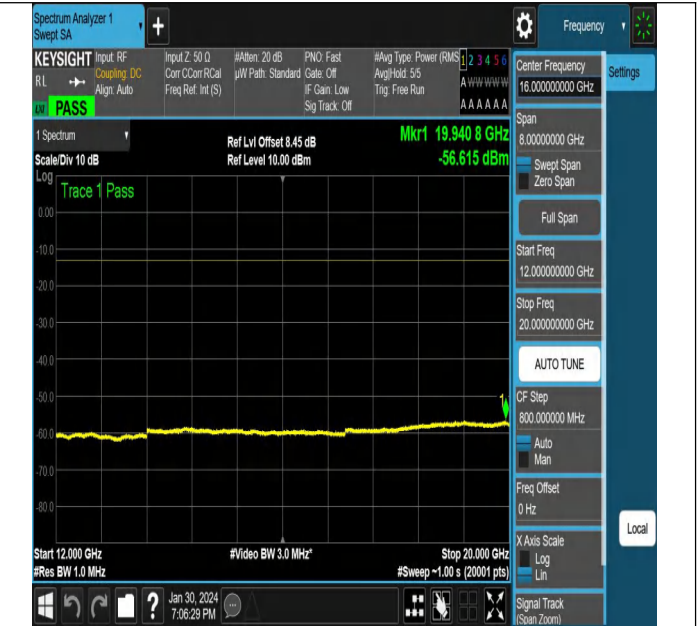
NTNV_N71_PC3_15_20_M_TID17_NS_01_12000_20000_#1
