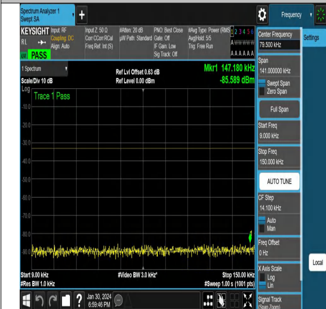
NTNV_N71_PC3_15_20_L_TID18_NS_01_0.009_0.15_#1
