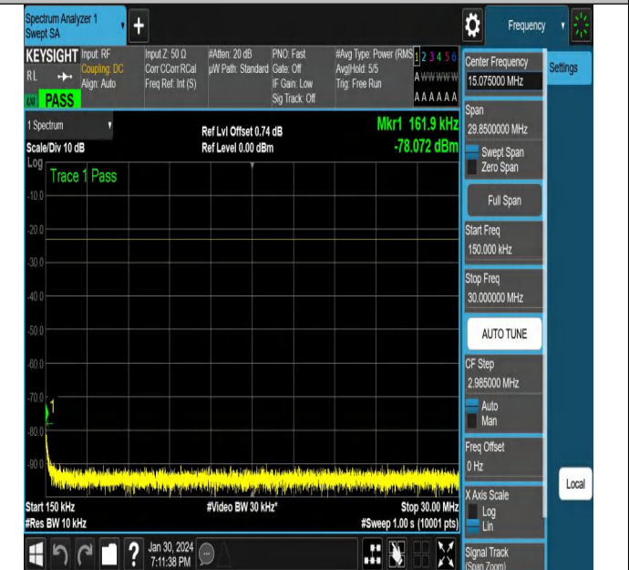
NTNV_N71_PC3_15_20_H_TID6_NS_01_0.15_30_#1
