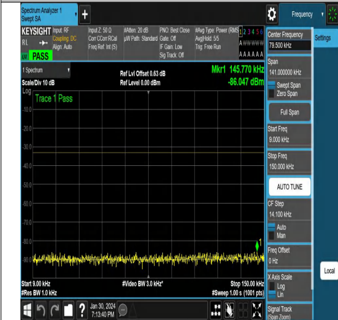
NTNV_N71_PC3_15_20_H_TID18_NS_01_0.009_0.15_#1
