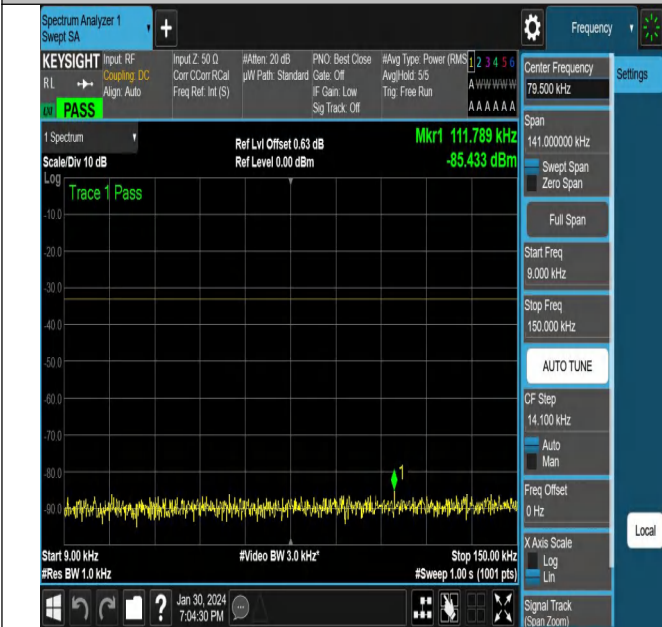
NTNV_N71_PC3_15_20_M_TID6_NS_01_0.009_0.15_#1
