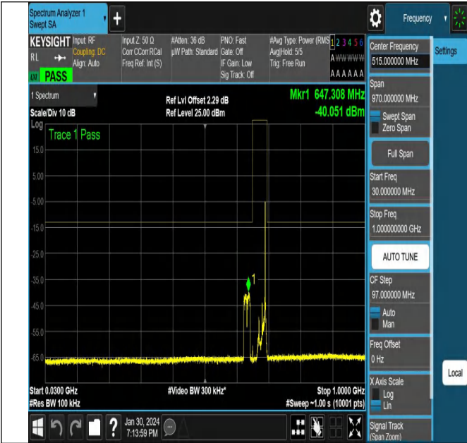
NTNV_N71_PC3_15_20_H_TID18_NS_01_30_1000_#1
