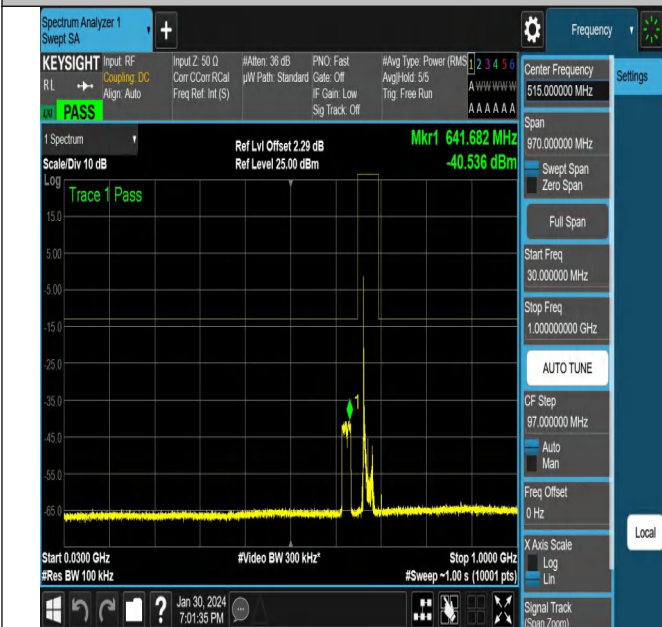
NTNV_N71_PC3_15_20_M_TID2_NS_01_30_1000_#1
