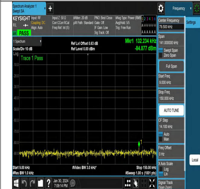
NTNV_N71_PC3_15_20_H_TID3_NS_01_0.009_0.15_#1
