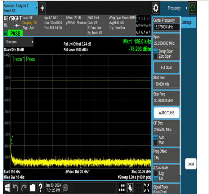
NTNV_N71_PC3_15_20_M_TID2_NS_01_0.15_30_#1
