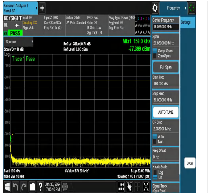
NTNV_N71_PC3_15_20_M_TID17_NS_01_0.15_30_#1
