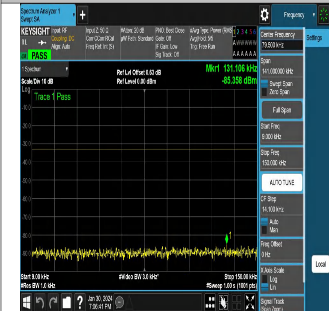
NTNV_N71_PC3_15_20_M_TID18_NS_01_0.009_0.15_#1
