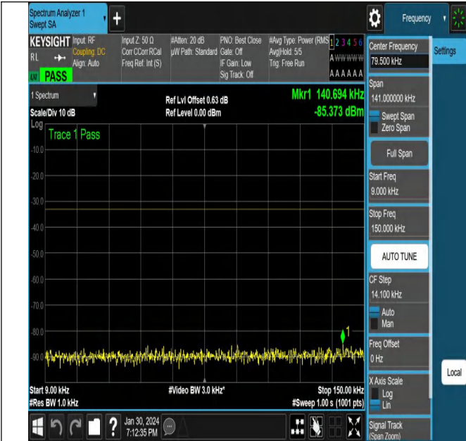
NTNV_N71_PC3_15_20_H_TID17_NS_01_0.009_0.15_#1
