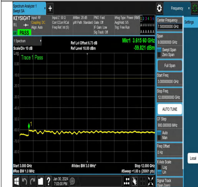
NTNV_N71_PC3_15_20_M_TID3_NS_01_3000_12000_#1
