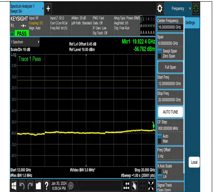
NTNV_N71_PC3_15_20_L_TID17_NS_01_12000_20000_#1
