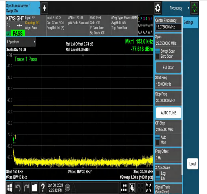
NTNV_N38_PC3_30_15_M_TID4_NS_01_0.15_30_#1
