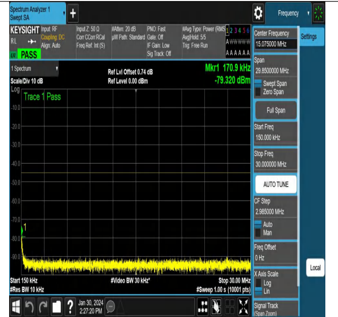
NTNV_N38_PC3_30_15_M_TID6_NS_01_0.15_30_#1
