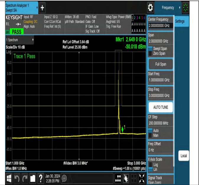
NTNV_N38_PC3_30_15_M_TID5_NS_01_1000_3000_#1
