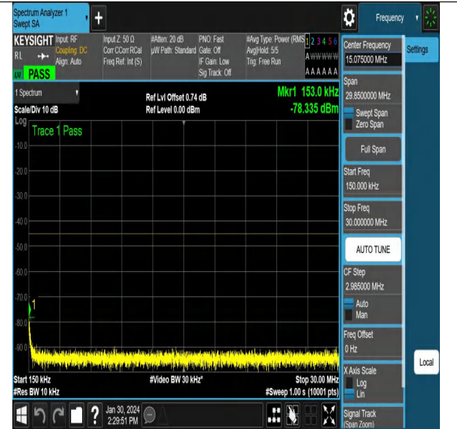
NTNV_N38_PC3_30_15_H_TID2_NS_01_0.15_30_#1
