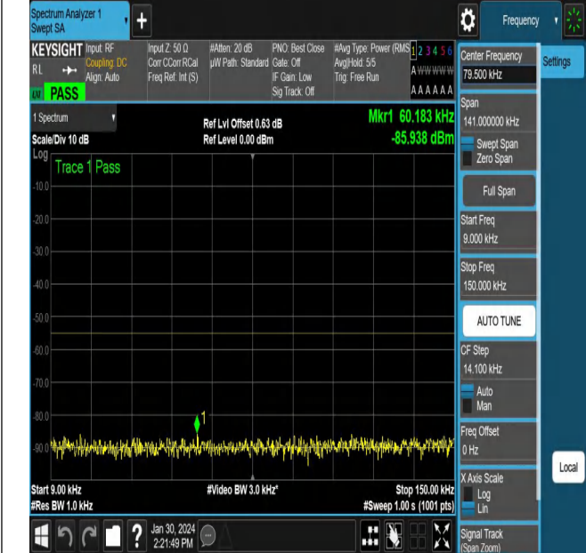
NTNV_N38_PC3_30_15_M_TID1_NS_01_0.009_0.15_#1
