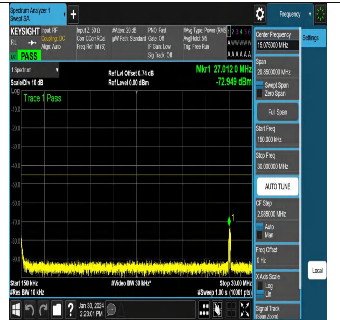
NTNV_N38_PC3_30_15_M_TID2_NS_01_0.15_30_#1
