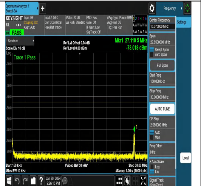
NTNV_N38_PC3_30_15_M_TID5_NS_01_0.15_30_#1
