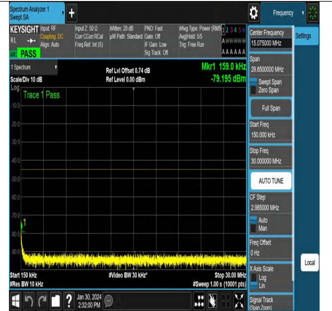
NTNV_N38_PC3_30_15_H_TID4_NS_01_0.15_30_#1
