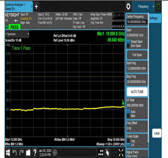
NTNV_N38_PC3_30_15_M_TID1_NS_01_12000_20000_#1
