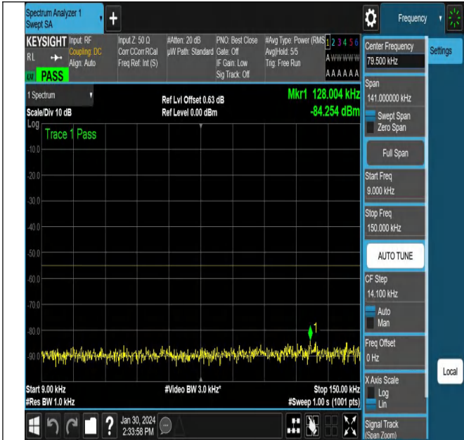
NTNV_N38_PC3_30_15_H_TID6_NS_01_0.009_0.15_#1
