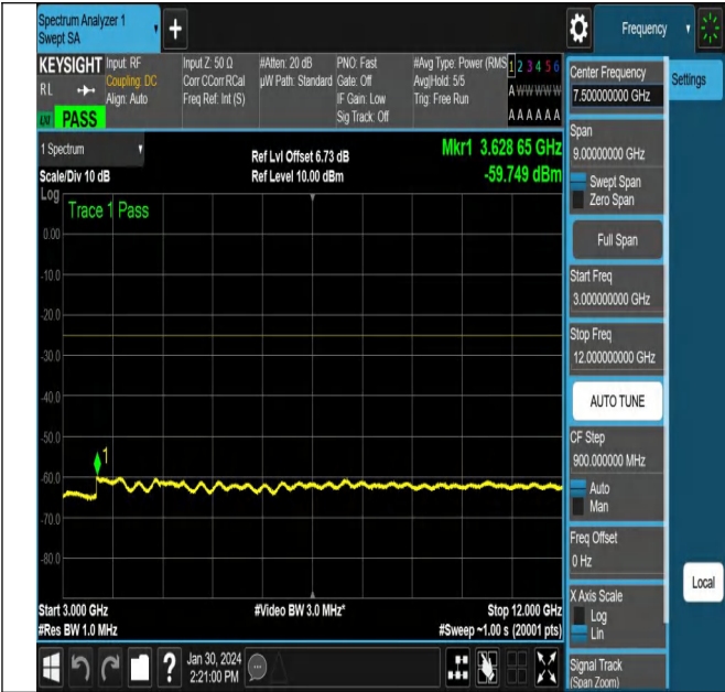
NTNV_N38_PC3_30_15_L_TID6_NS_01_3000_12000_#1
