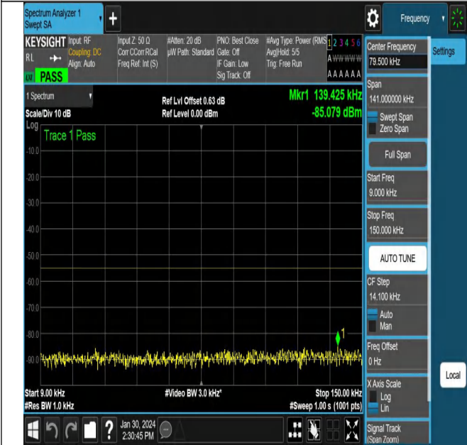
NTNV_N38_PC3_30_15_H_TID3_NS_01_0.009_0.15_#1
