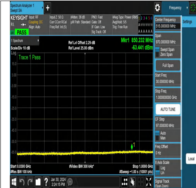
NTNV_N38_PC3_30_15_M_TID3_NS_01_30_1000_#1
