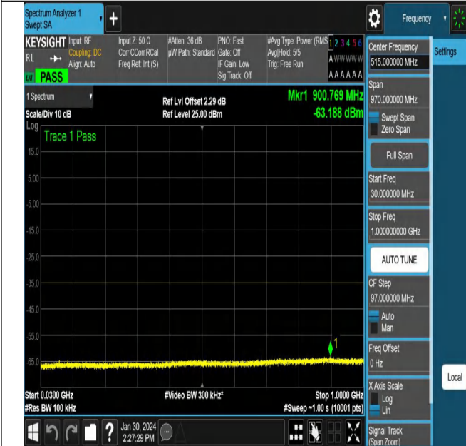
NTNV_N38_PC3_30_15_M_TID6_NS_01_30_1000_#1
