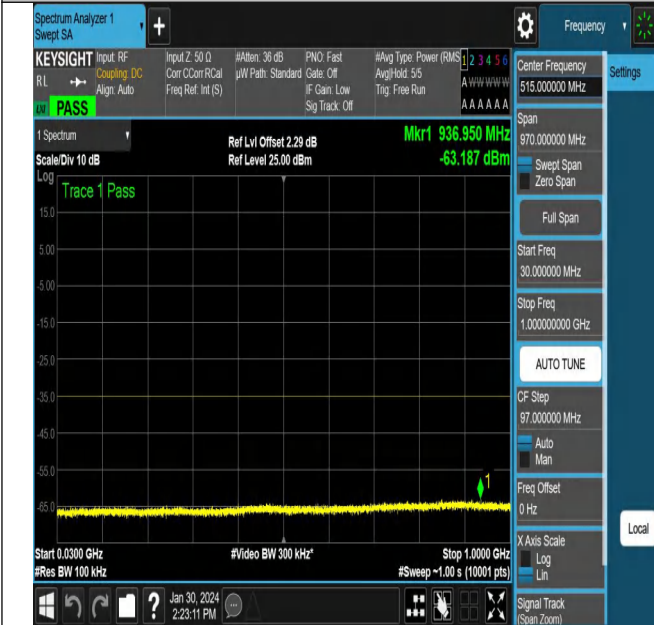
NTNV_N38_PC3_30_15_M_TID2_NS_01_30_1000_#1
