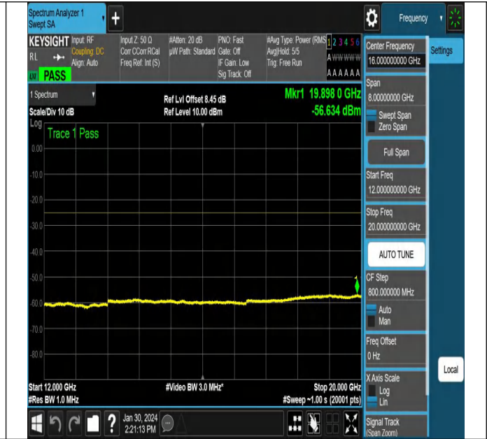
NTNV_N38_PC3_30_15_L_TID6_NS_01_12000_20000_#1
