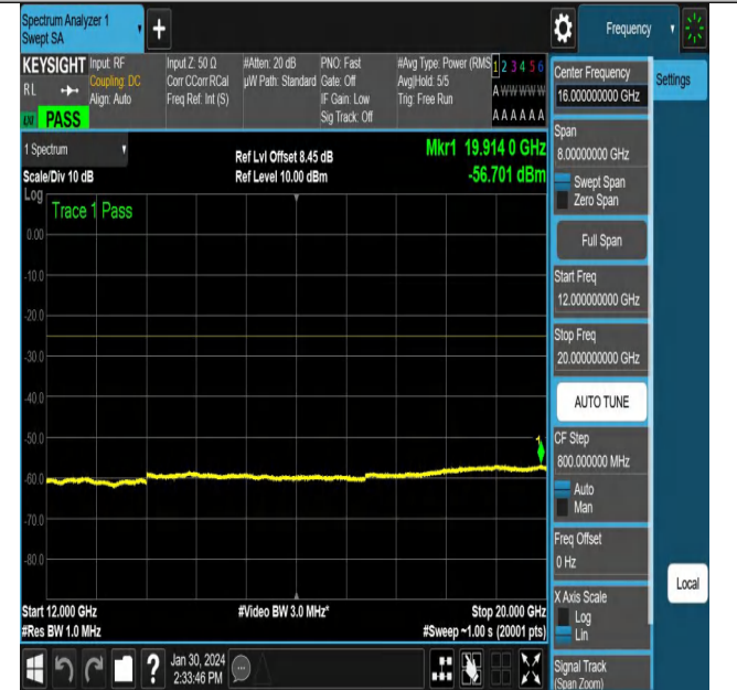
NTNV_N38_PC3_30_15_H_TID5_NS_01_12000_20000_#1
