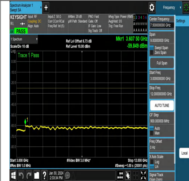
NTNV_N38_PC3_30_15_H_TID5_NS_01_3000_12000_#1
