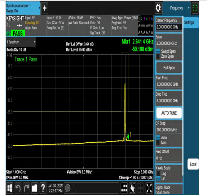
NTNV_N38_PC3_30_15_M_TID1_NS_01_1000_3000_#1
