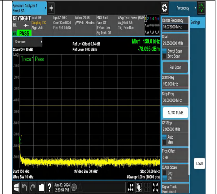
NTNV_N38_PC3_30_15_H_TID3_NS_01_0.15_30_#1
