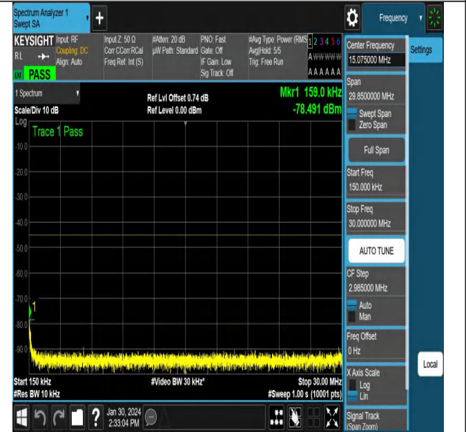
NTNV_N38_PC3_30_15_H_TID5_NS_01_0.15_30_#1
