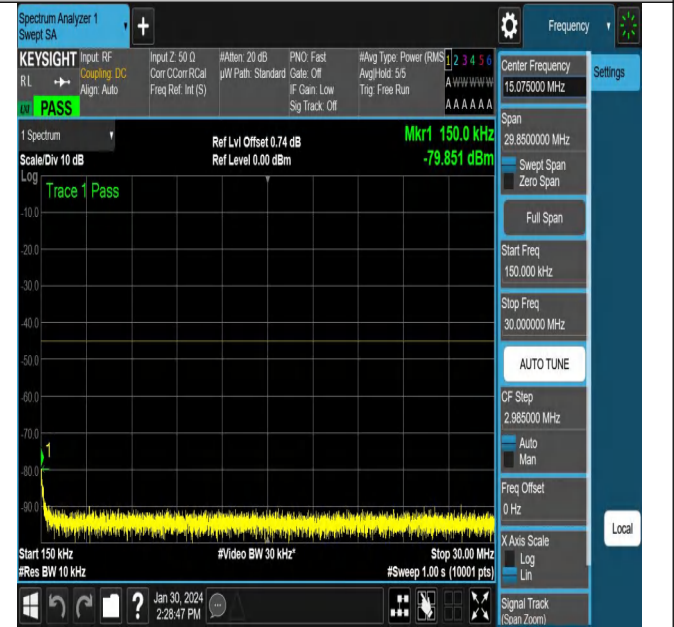
NTNV_N38_PC3_30_15_H_TID1_NS_01_0.15_30_#1
