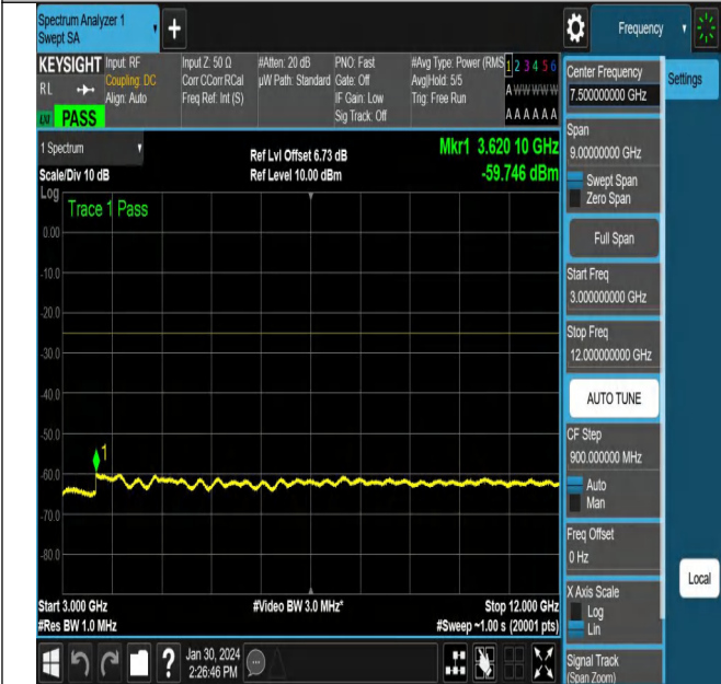
NTNV_N38_PC3_30_15_M_TID5_NS_01_3000_12000_#1
