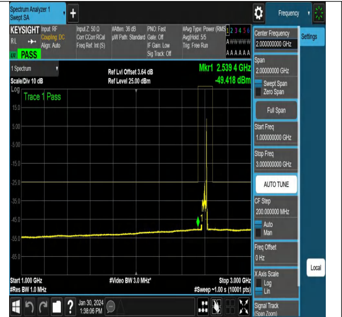
NTNV_N38_PC3_30_40_M_TID3_NS_01_1000_3000_#1
