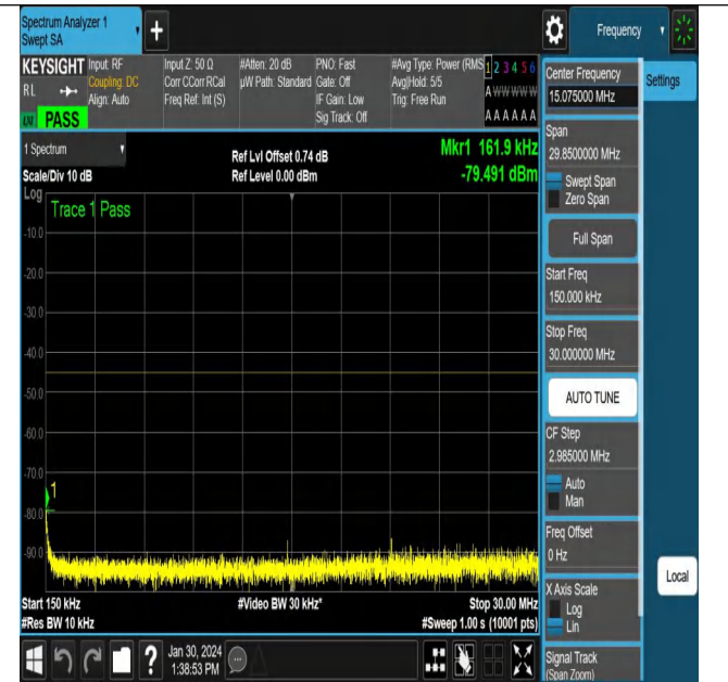
NTNV_N38_PC3_30_40_M_TID4_NS_01_0.15_30_#1
