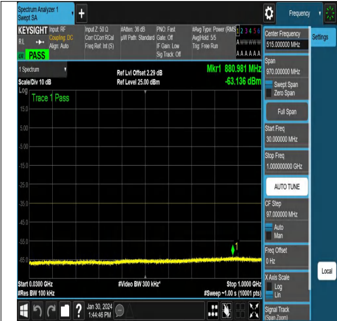
NTNV_N38_PC3_30_40_H_TID3_NS_01_30_1000_#1
