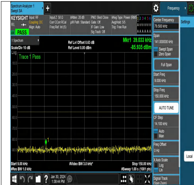
NTNV_N38_PC3_30_40_M_TID4_NS_01_0.009_0.15_#1
