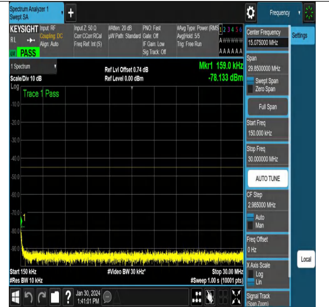
NTNV_N38_PC3_30_40_M_TID6_NS_01_0.15_30_#1
