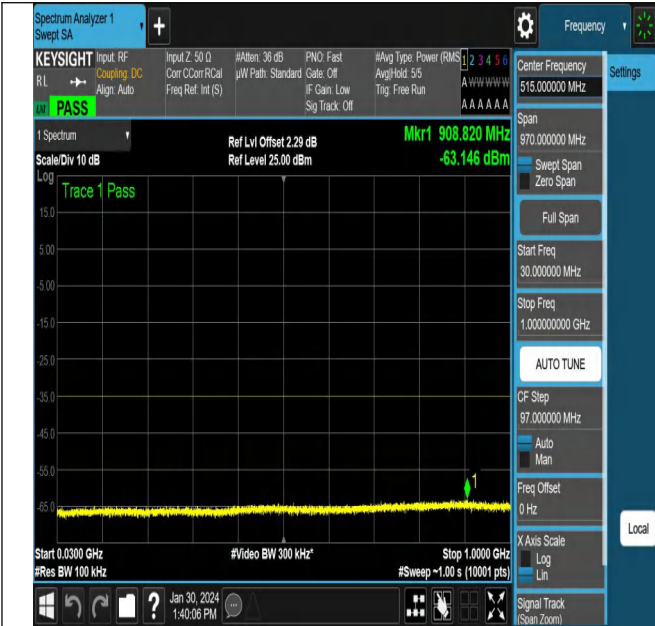
NTNV_N38_PC3_30_40_M_TID5_NS_01_30_1000_#1
