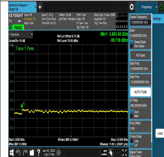
NTNV_N38_PC3_30_40_M_TID3_NS_01_3000_12000_#1
