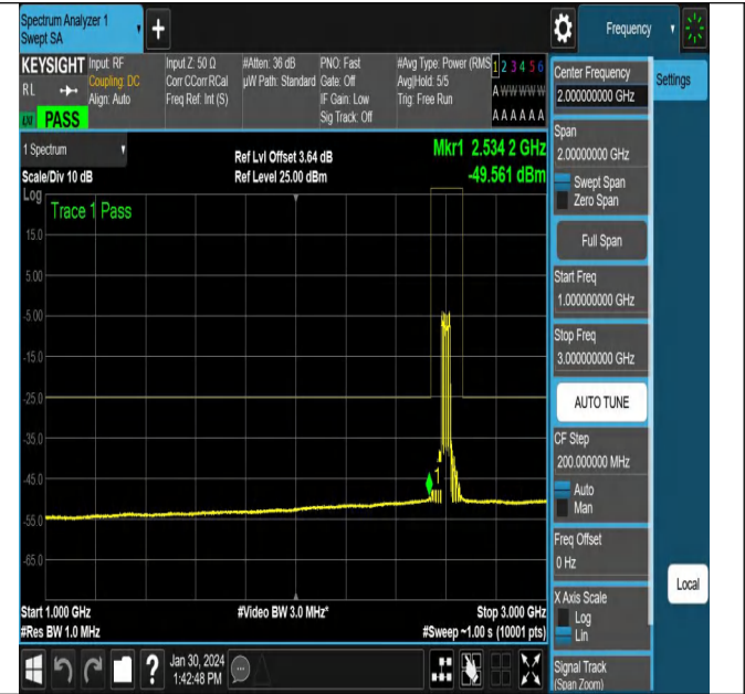
NTNV_N38_PC3_30_40_H_TID1_NS_01_1000_3000_#1
