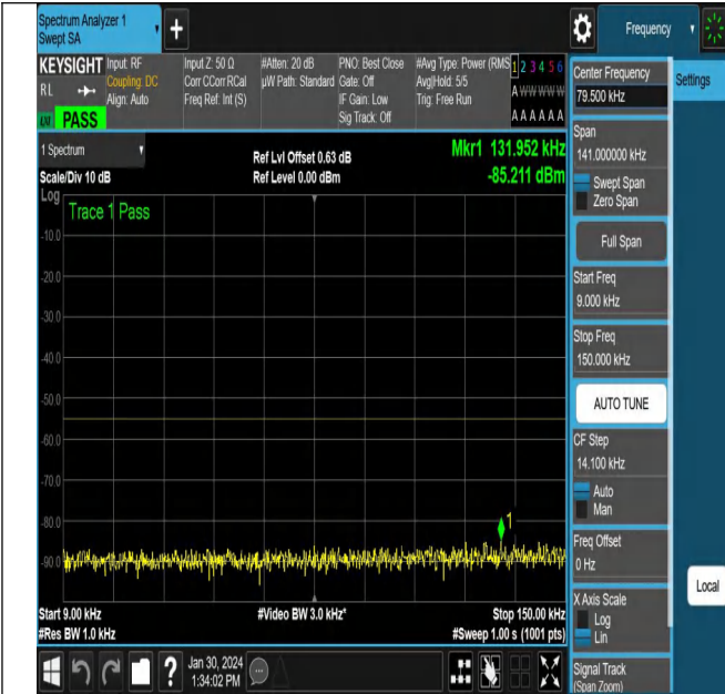
NTNV_N38_PC3_30_40_L_TID5_NS_01_0.009_0.15_#1
