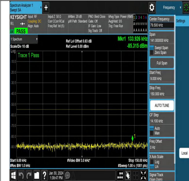
NTNV_N38_PC3_30_40_M_TID5_NS_01_0.009_0.15_#1
