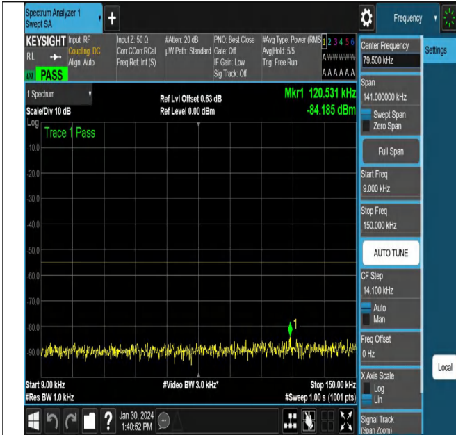
NTNV_N38_PC3_30_40_M_TID6_NS_01_0.009_0.15_#1
