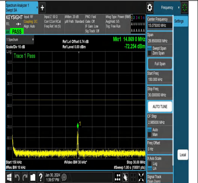
NTNV_N38_PC3_30_40_M_TID5_NS_01_0.15_30_#1
