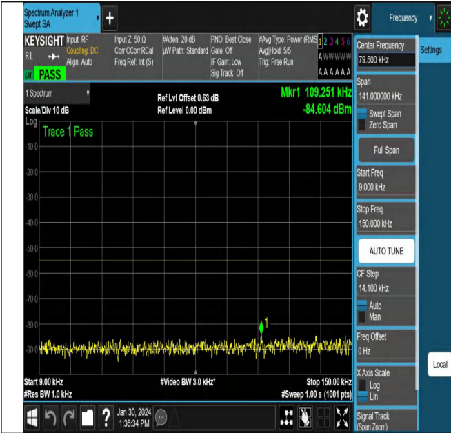
NTNV_N38_PC3_30_40_M_TID2_NS_01_0.009_0.15_#1
