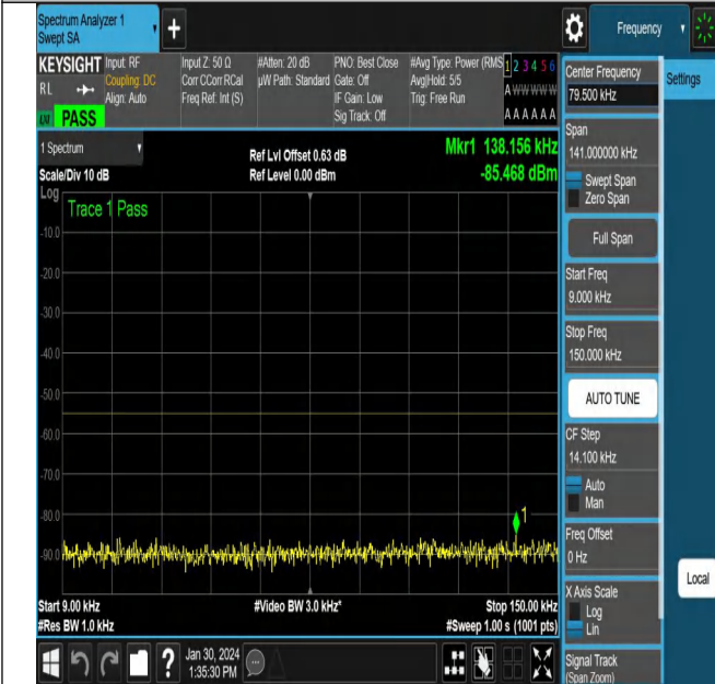
NTNV_N38_PC3_30_40_M_TID1_NS_01_0.009_0.15_#1
