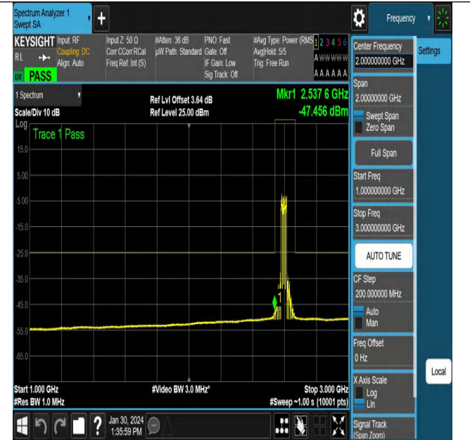
NTNV_N38_PC3_30_40_M_TID1_NS_01_1000_3000_#1
