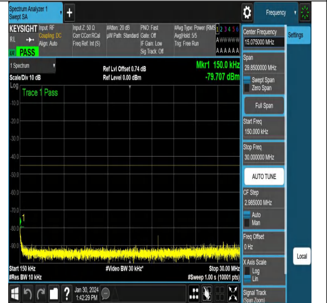
NTNV_N38_PC3_30_40_H_TID1_NS_01_0.15_30_#1
