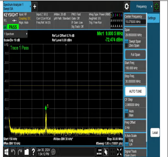
NTNV_N38_PC3_30_40_L_TID5_NS_01_0.15_30_#1
