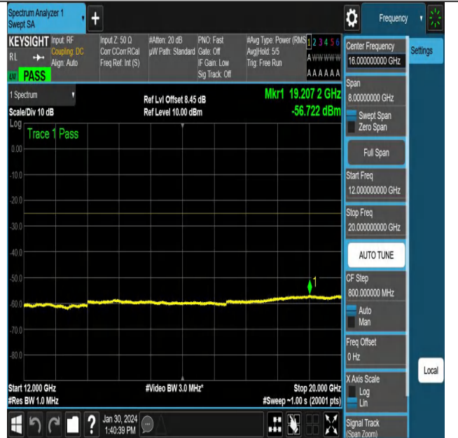
NTNV_N38_PC3_30_40_M_TID5_NS_01_12000_20000_#1
