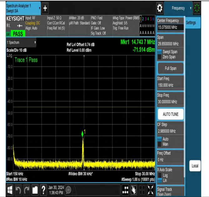
NTNV_N38_PC3_30_40_M_TID2_NS_01_0.15_30_#1
