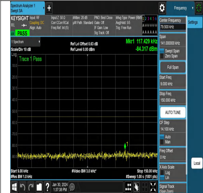
NTNV_N38_PC3_30_40_M_TID3_NS_01_0.009_0.15_#1
