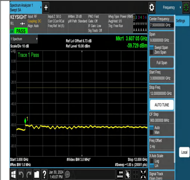
NTNV_N38_PC3_30_40_H_TID3_NS_01_3000_12000_#1
