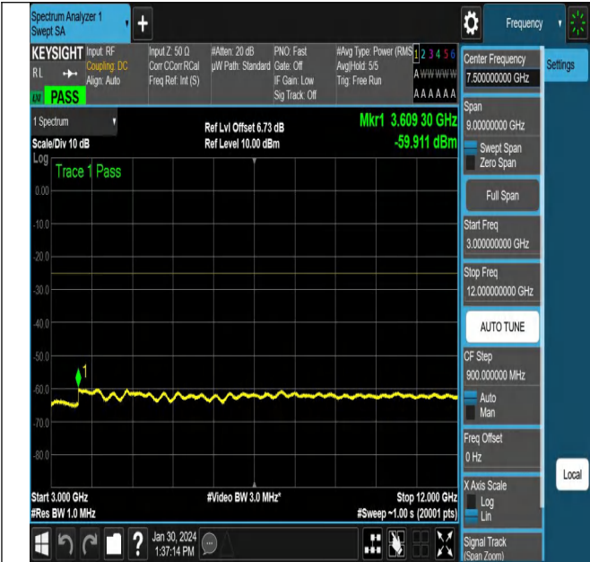
NTNV_N38_PC3_30_40_M_TID2_NS_01_3000_12000_#1
