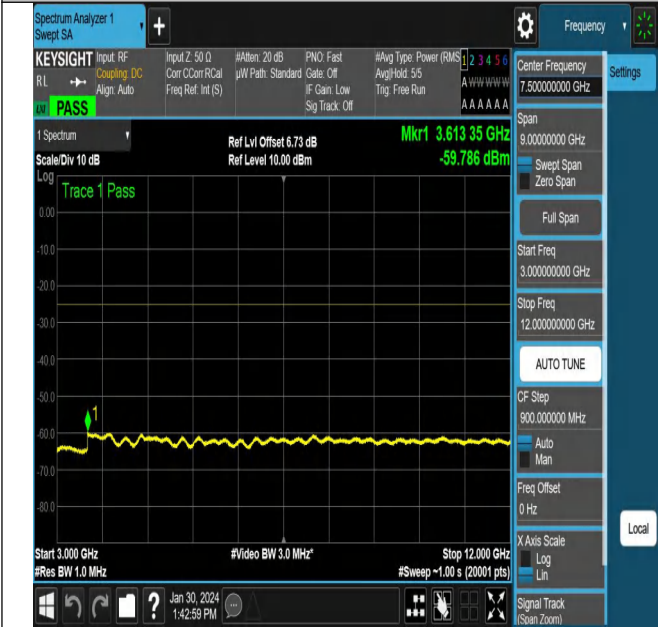
NTNV_N38_PC3_30_40_H_TID1_NS_01_3000_12000_#1
