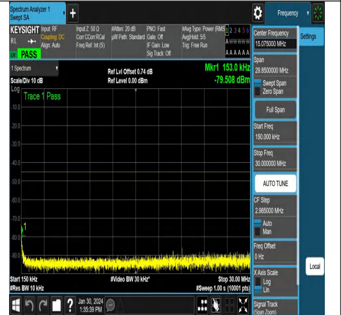
NTNV_N38_PC3_30_40_M_TID1_NS_01_0.15_30_#1
