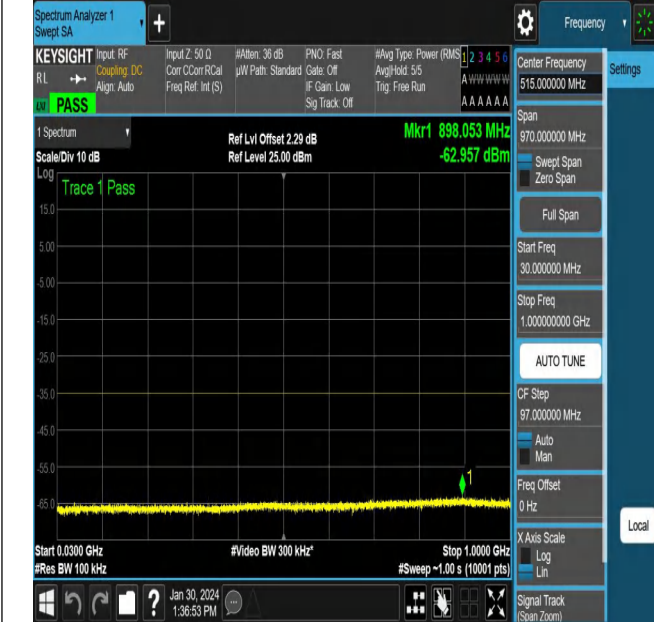
NTNV_N38_PC3_30_40_M_TID2_NS_01_30_1000_#1
