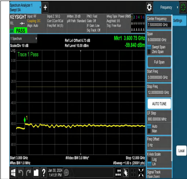
NTNV_N38_PC3_30_40_M_TID6_NS_01_3000_12000_#1
