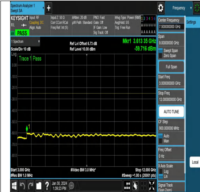
NTNV_N38_PC3_30_40_M_TID4_NS_01_3000_12000_#1
