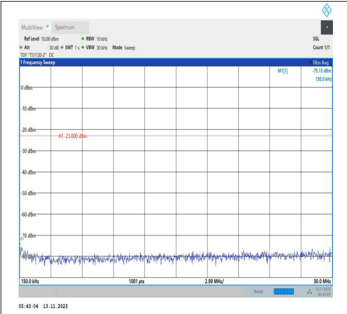
Band71_20MHz_16QAM_133372_1RB#0_0.15~30_0.15~30
