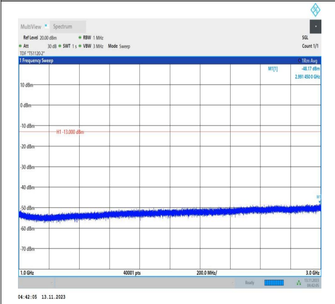
Band71_10MHz_16QAM_133422_1RB#0_1000~3000_1000~3000
