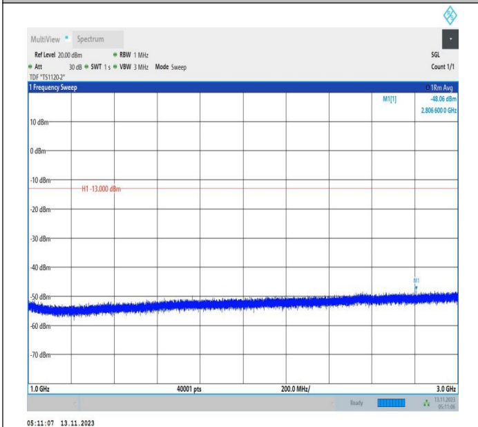
Band71_15MHz_16QAM_133297_1RB#0_1000~3000_1000~3000
