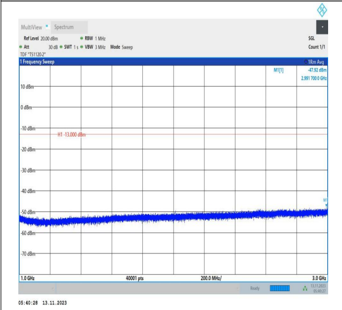
Band71_20MHz_16QAM_133222_1RB#0_1000~3000_1000~3000
