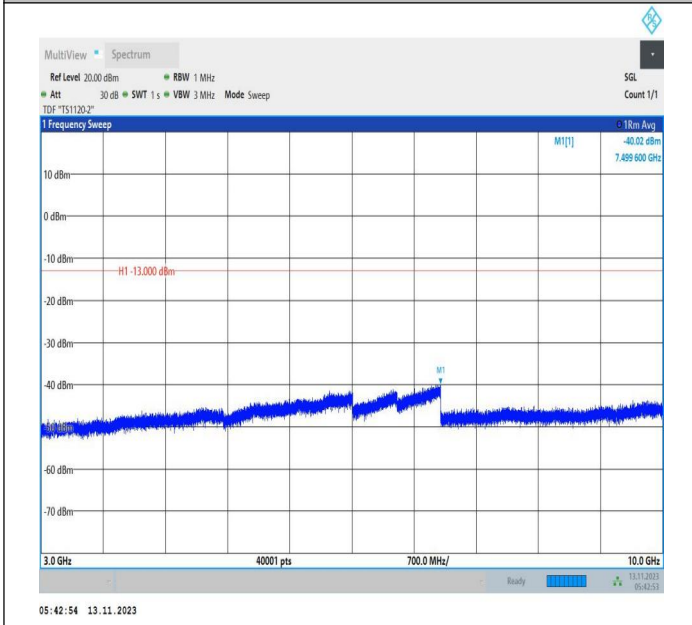
Band71_20MHz_QPSK_133372_1RB#0_3000~10000_3000~10000
