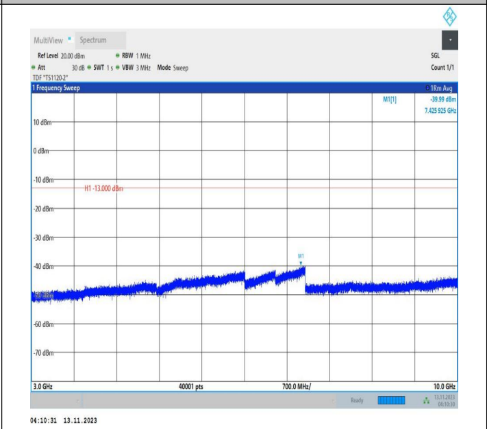
Band71_5MHz_16QAM_133297_1RB#0_3000~10000_3000~10000
