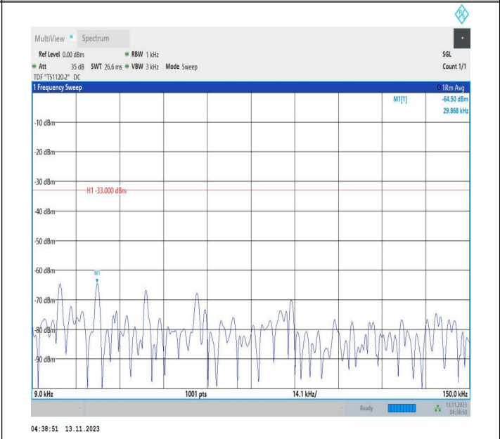
Band71_10MHz_16QAM_133172_1RB#0_0.009~0.15_0.009~0.15
