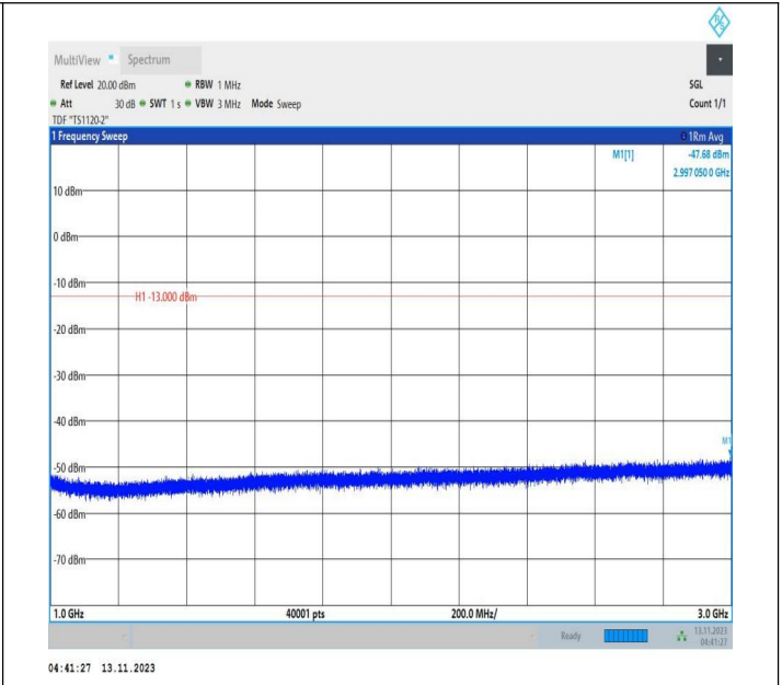
Band71_10MHz_QPSK_133422_1RB#0_1000~3000_1000~3000 00
