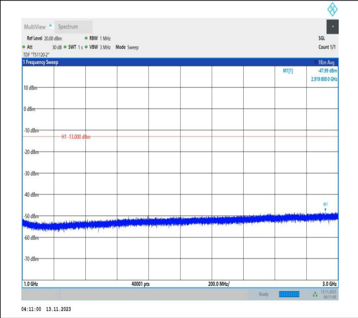
Band71_5MHz_QPSK_133447_1RB#0_1000~3000_1000~3000 0
