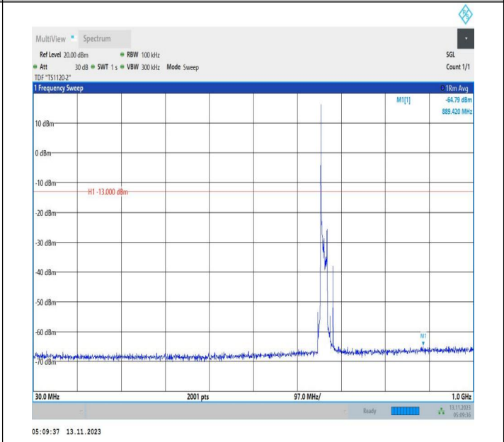
Band71_15MHz_16QAM_133197_1RB#0_30~1000_30~1000
