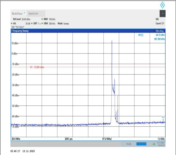
Band71_20MHz_16QAM_133222_1RB#0_30~1000_30~1000
