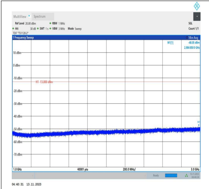
Band71_10MHz_16QAM_133297_1RB#0_1000~3000_1000~3000
