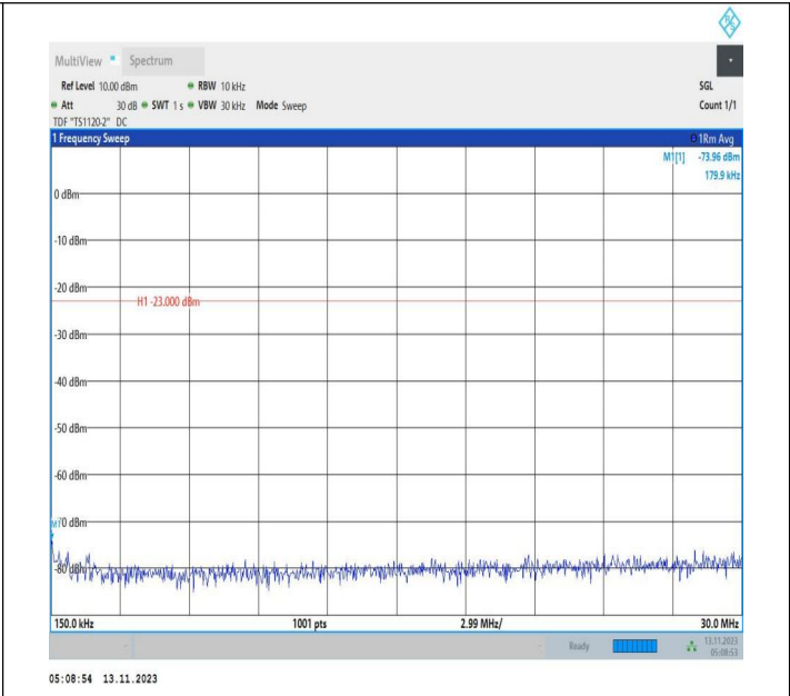
Band71_15MHz_QPSK_133197_1RB#0_0.15~30_0.15~30
