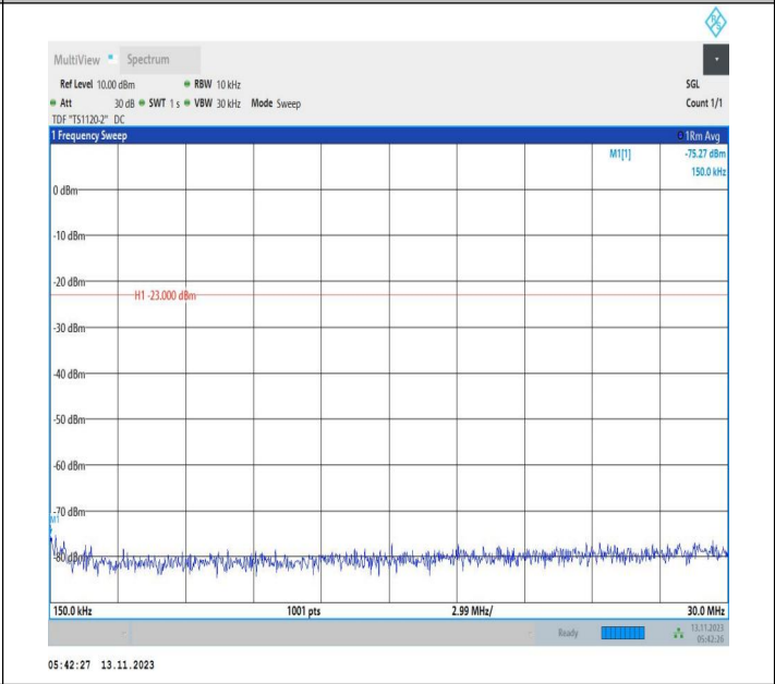
Band71_20MHz_QPSK_133372_1RB#0_0.15~30_0.15~30
