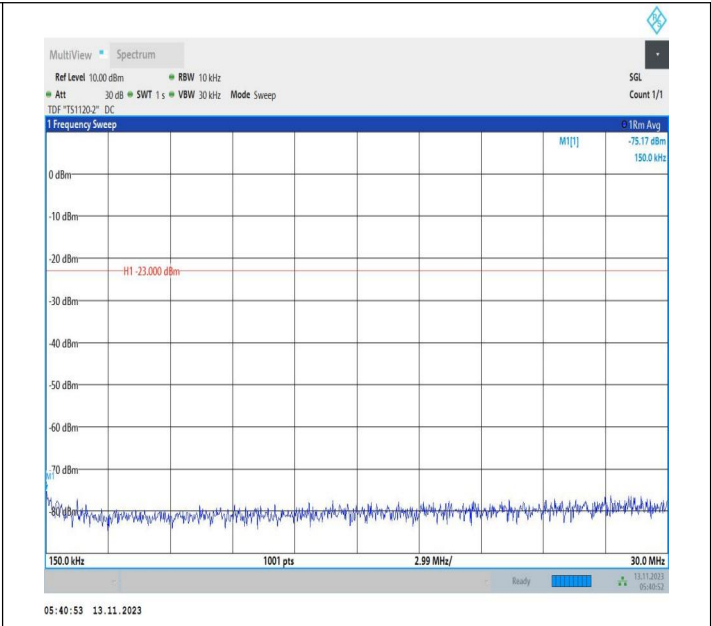
Band71_20MHz_QPSK_133322_1RB#0_0.15~30_0.15~30
