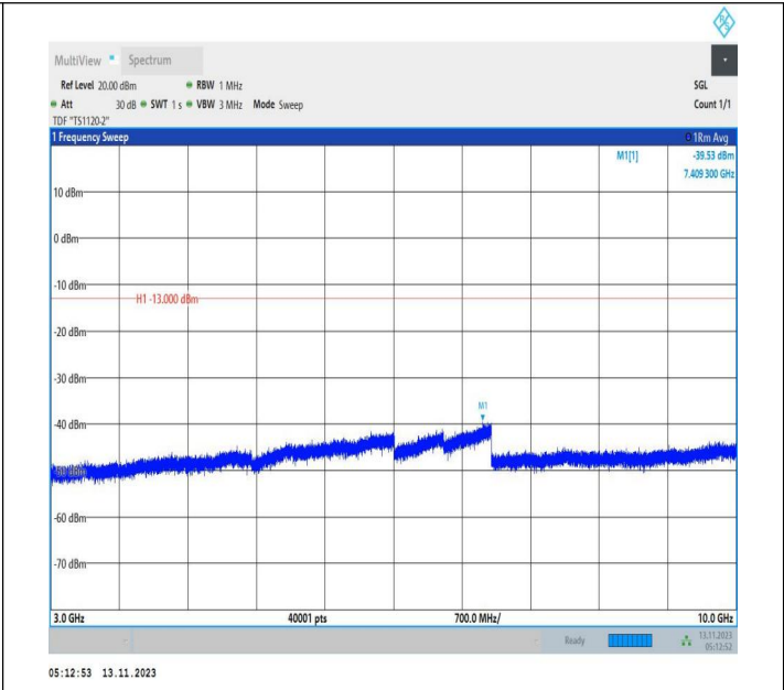
Band71_15MHz_16QAM_133397_1RB#0_3000~10000_3000~10000
