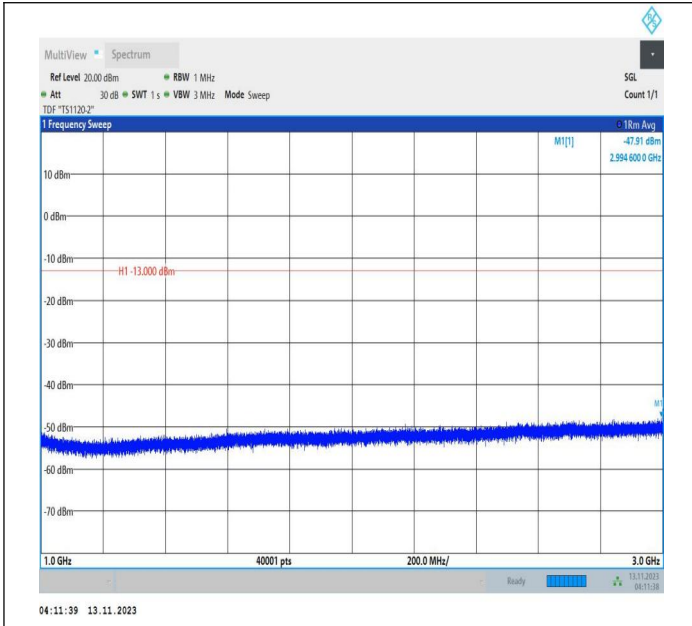
Band71_5MHz_16QAM_133447_1RB#0_1000~3000_1000~3000
