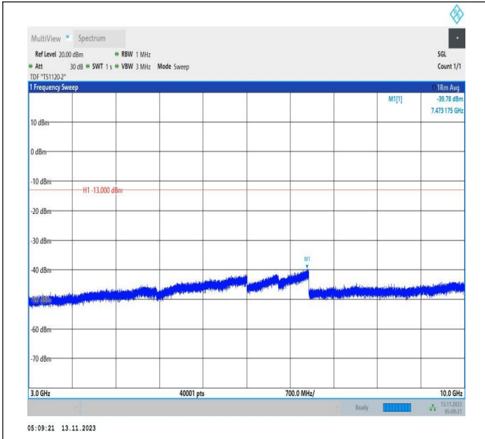
Band71_15MHz_QPSK_133197_1RB#0_3000~10000_3000~10000
