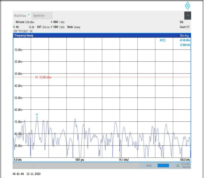
Band71_10MHz_16QAM_133422_1RB#0_0.009~0.15_0.009~0.15
