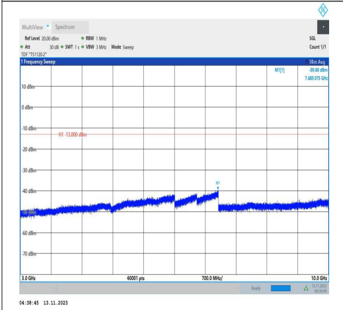
Band71_10MHz_QPSK_133172_1RB#0_3000~10000_3000~10000
