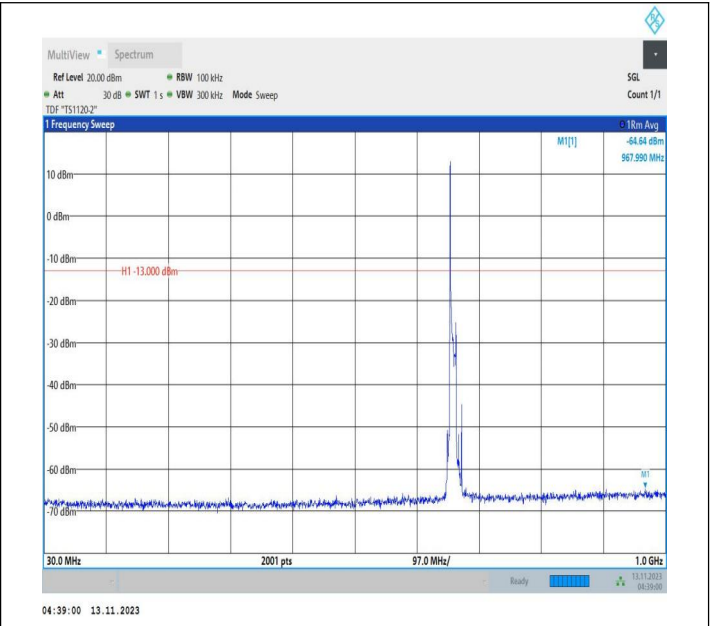
Band71_10MHz_16QAM_133172_1RB#0_30~1000_30~1000
