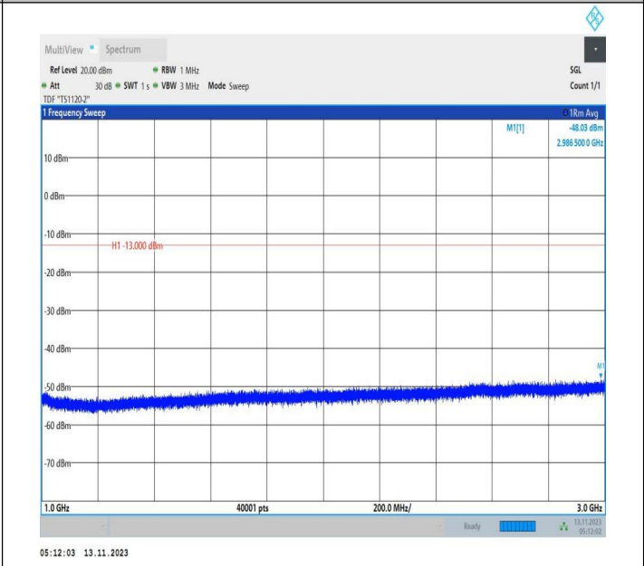
Band71_15MHz_QPSK_133397_1RB#0_1000~3000_1000~3000
