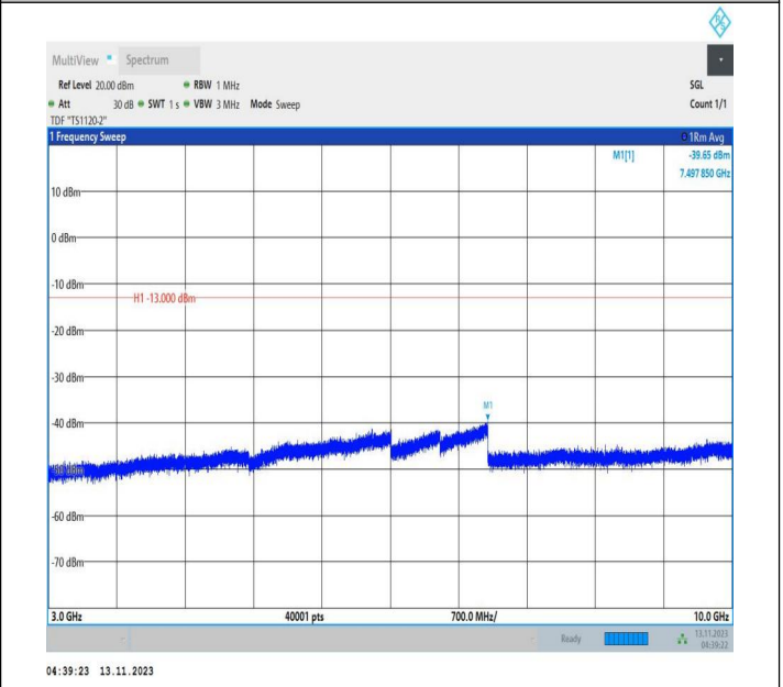
Band71_10MHz_16QAM_133172_1RB#0_3000~10000_3000~10000
