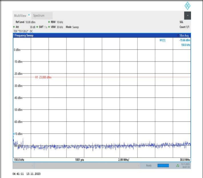
Band71_10MHz_QPSK_133422_1RB#0_0.15~30_0.15~30
