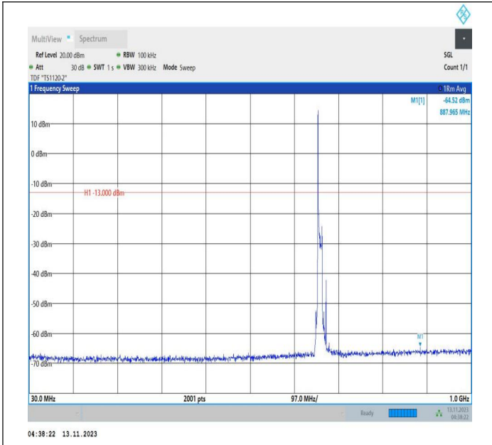
Band71_10MHz_QPSK_133172_1RB#0_30~1000_30~1000
