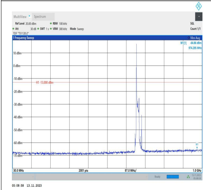
Band71_15MHz_QPSK_133197_1RB#0_30~1000_30~1000
