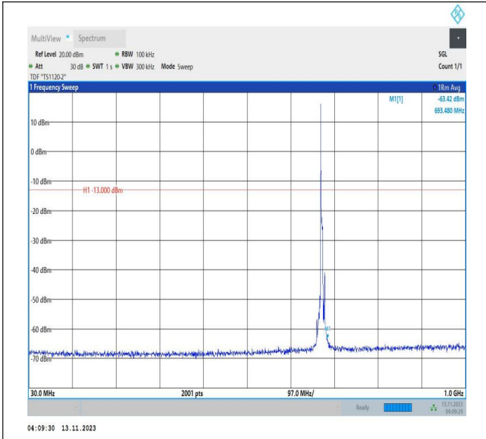
Band71_5MHz_QPSK_133297_1RB#0_30~1000_30~1000
