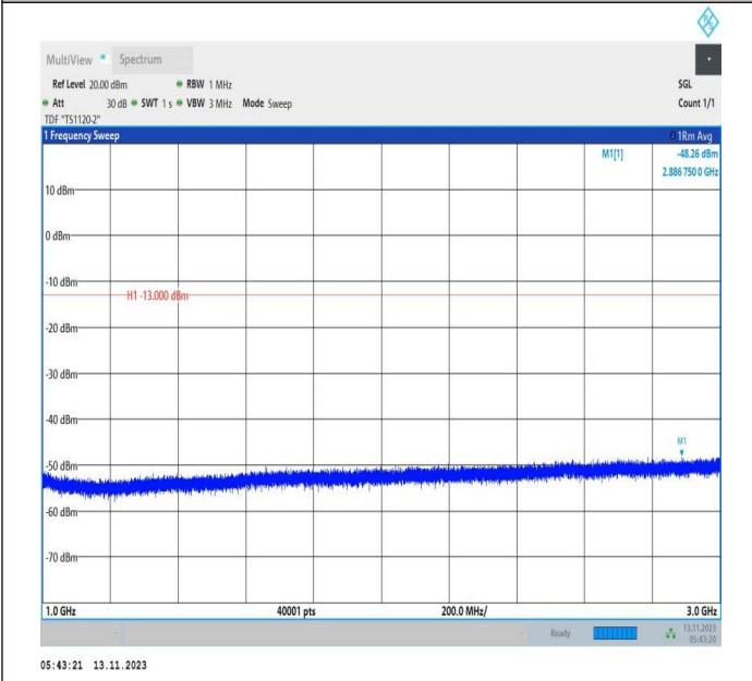
Band71_20MHz_16QAM_133372_1RB#0_1000~3000_1000~3000
