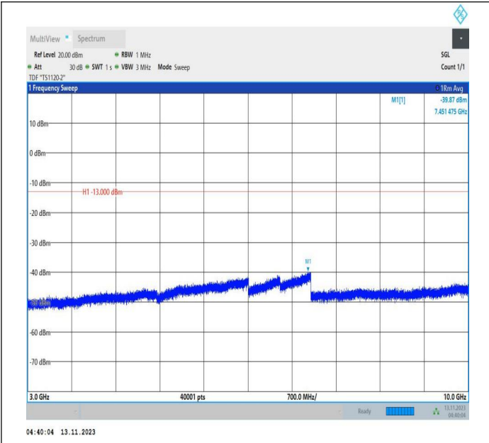
Band71_10MHz_QPSK_133297_1RB#0_3000~10000_3000~10000
