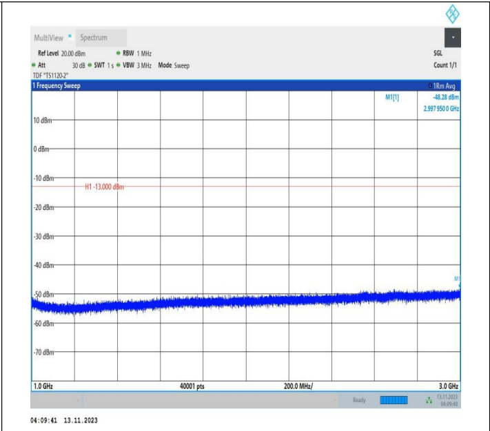
Band71_5MHz_QPSK_133297_1RB#0_1000~3000_1000~300 0
