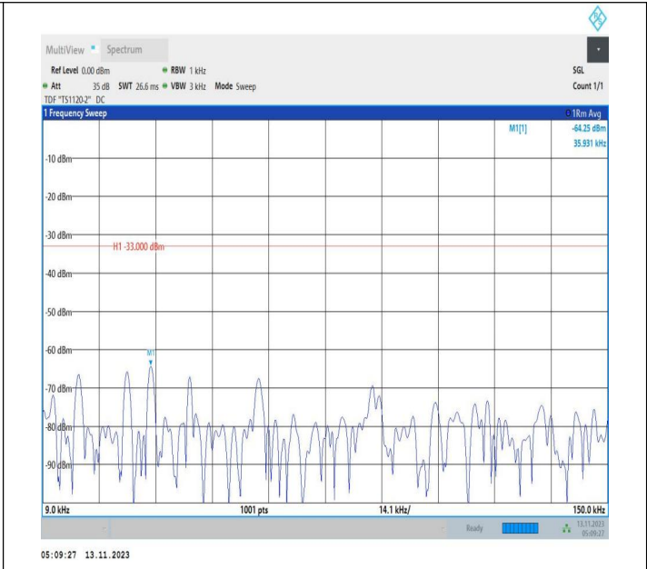
Band71_15MHz_16QAM_133197_1RB#0_0.009~0.15_0.009~0.15
