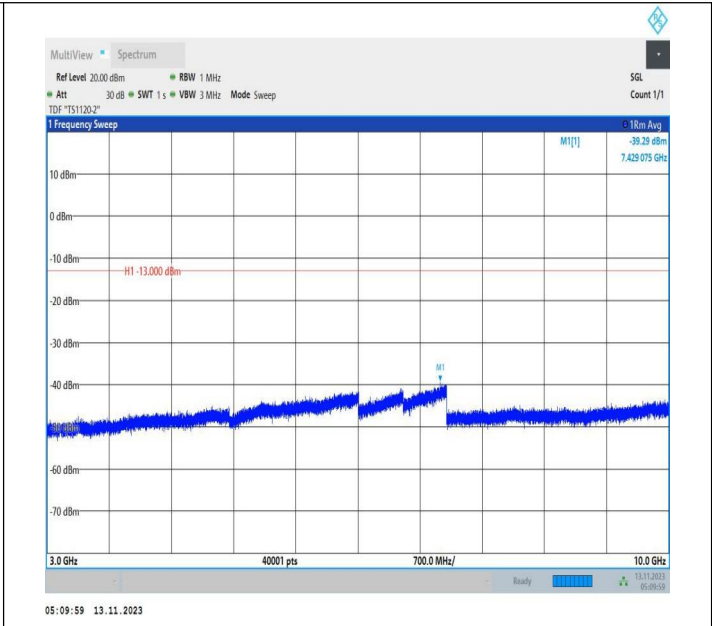
Band71_15MHz_16QAM_133197_1RB#0_3000~10000_3000~10000
