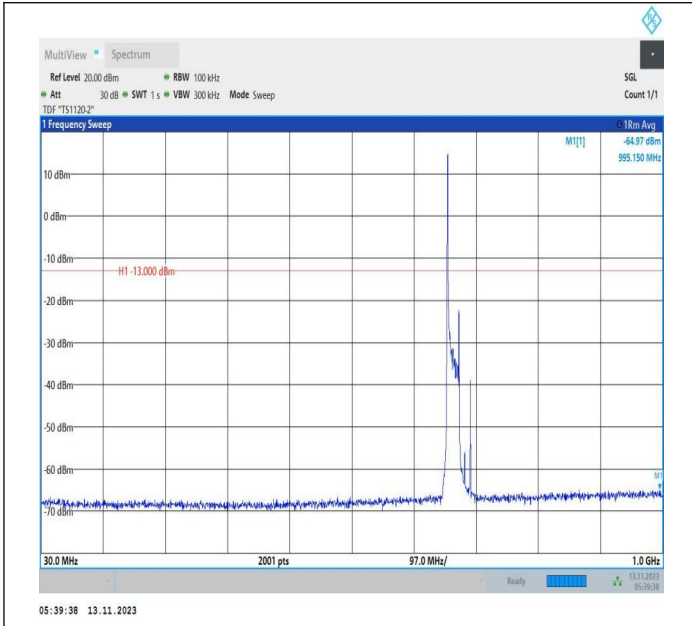
Band71_20MHz_QPSK_133222_1RB#0_30~1000_30~1000
