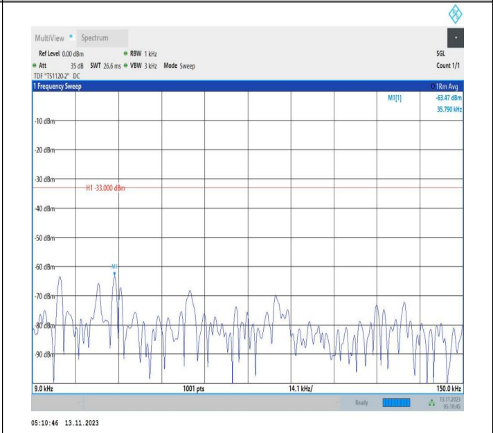
Band71_15MHz_16QAM_133297_1RB#0_0.009~0.15_0.009~0.15
