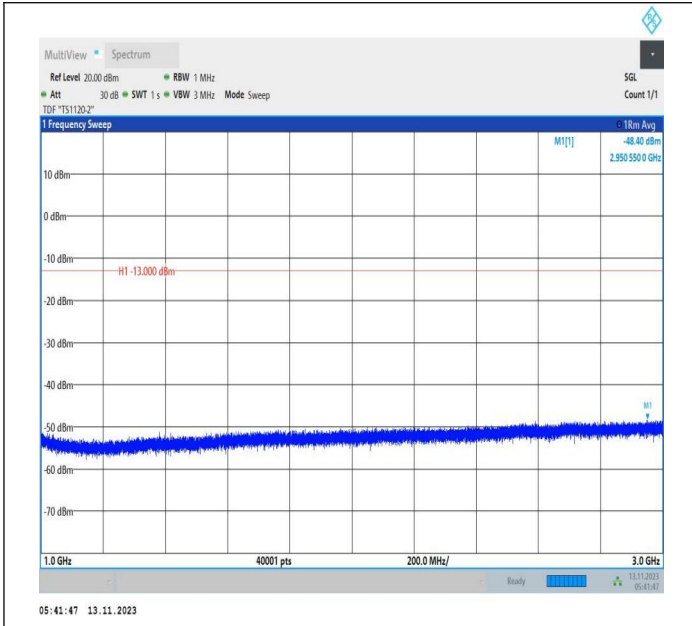
Band71_20MHz_16QAM_133322_1RB#0_1000~3000_1000~3000
