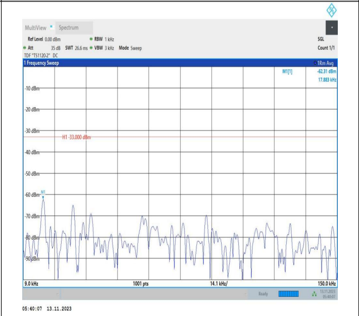
Band71_20MHz_16QAM_133222_1RB#0_0.009~0.15_0.009~0.15
