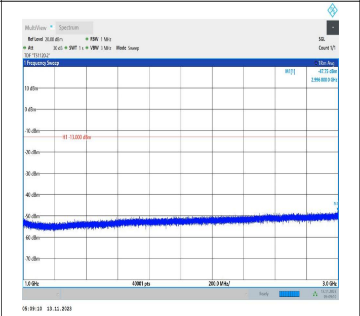
Band71_15MHz_QPSK_133197_1RB#0_1000~3000_1000~3000
