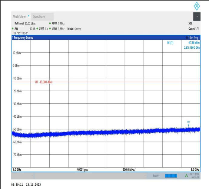
Band71_10MHz_16QAM_133172_1RB#0_1000~3000_1000~3000
