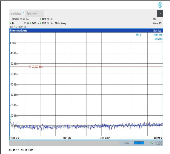
Band71_20MHz_16QAM_133222_1RB#0_0.15~30_0.15~30
