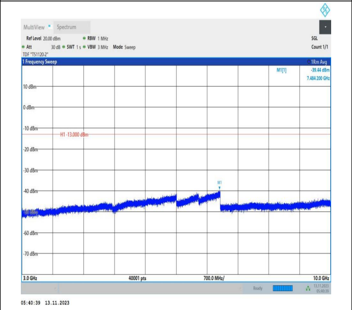
Band71_20MHz_16QAM_133222_1RB#0_3000~10000_3000~10000
