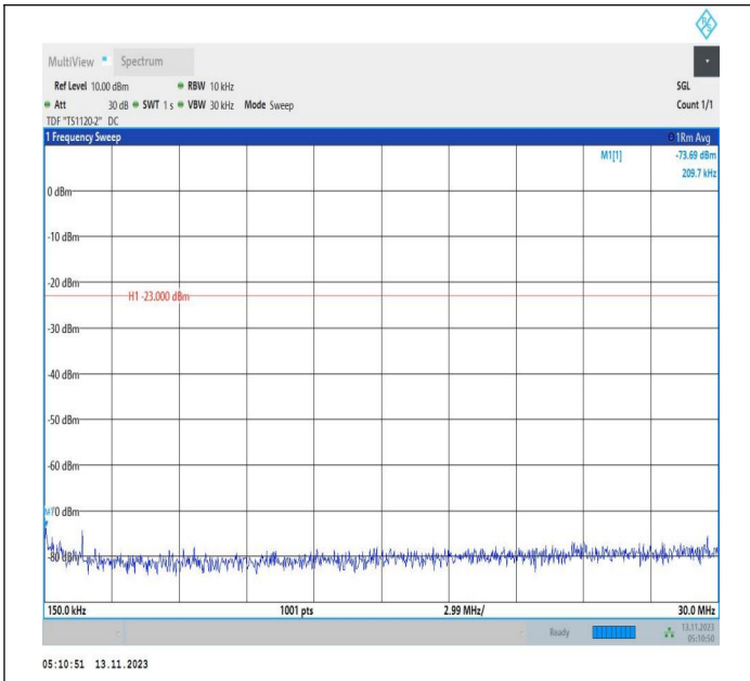
Band71_15MHz_16QAM_133297_1RB#0_0.15~30_0.15~30
