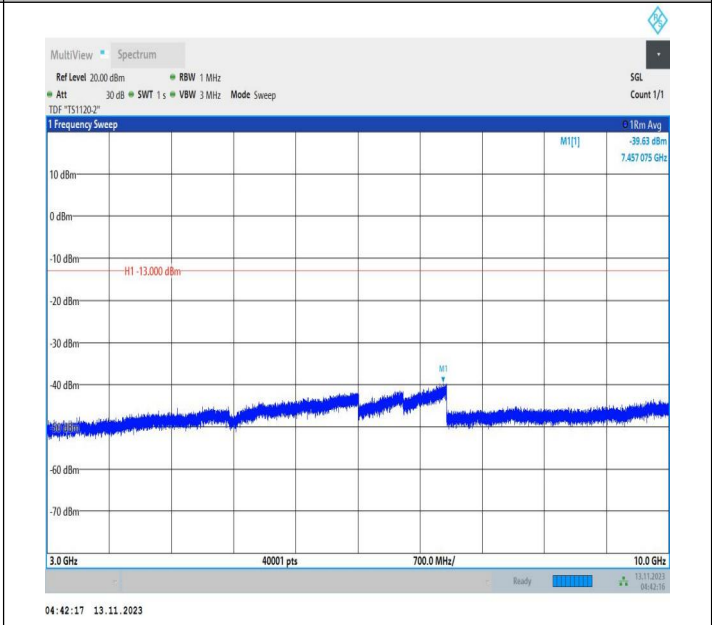
Band71_10MHz_16QAM_133422_1RB#0_3000~10000_3000~10000
