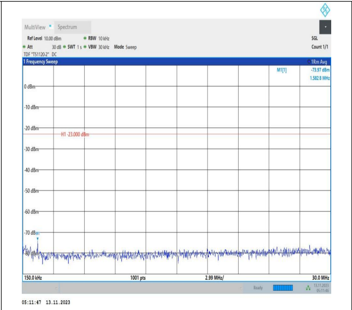
Band71_15MHz_QPSK_133397_1RB#0_0.15~30_0.15~30
