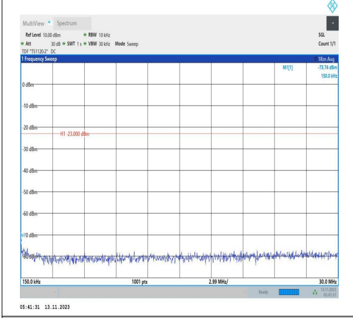
Band71_20MHz_16QAM_133322_1RB#0_0.15~30_0.15~30
