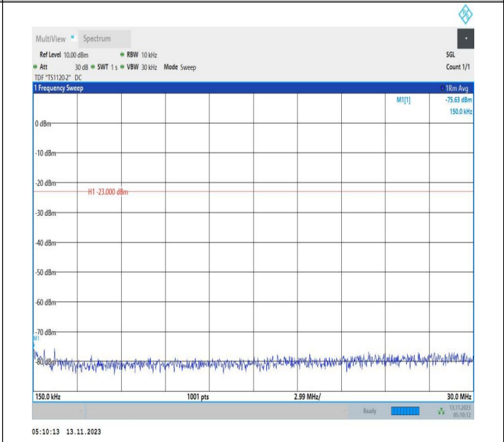
Band71_15MHz_QPSK_133297_1RB#0_0.15~30_0.15~30
