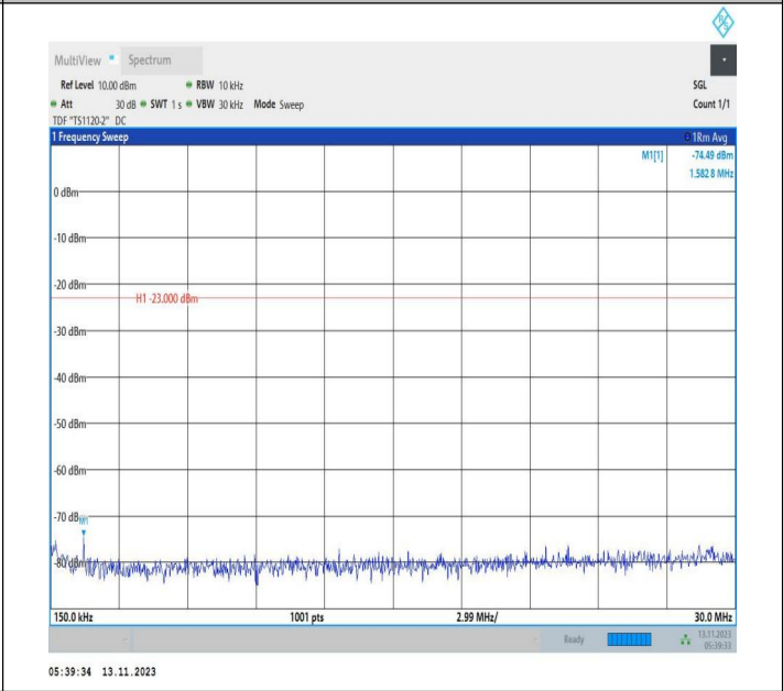
Band71_20MHz_QPSK_133222_1RB#0_0.15~30_0.15~30
