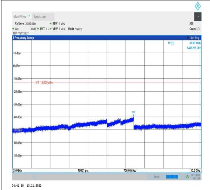
Band71_10MHz_QPSK_133422_1RB#0_3000~10000_3000~10000
