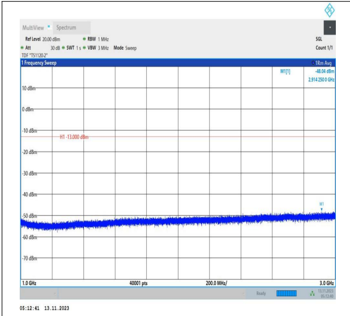
Band71_15MHz_16QAM_133397_1RB#0_1000~3000_1000~3000
