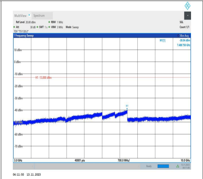
Band71_5MHz_16QAM_133447_1RB#0_3000~10000_3000~10000
