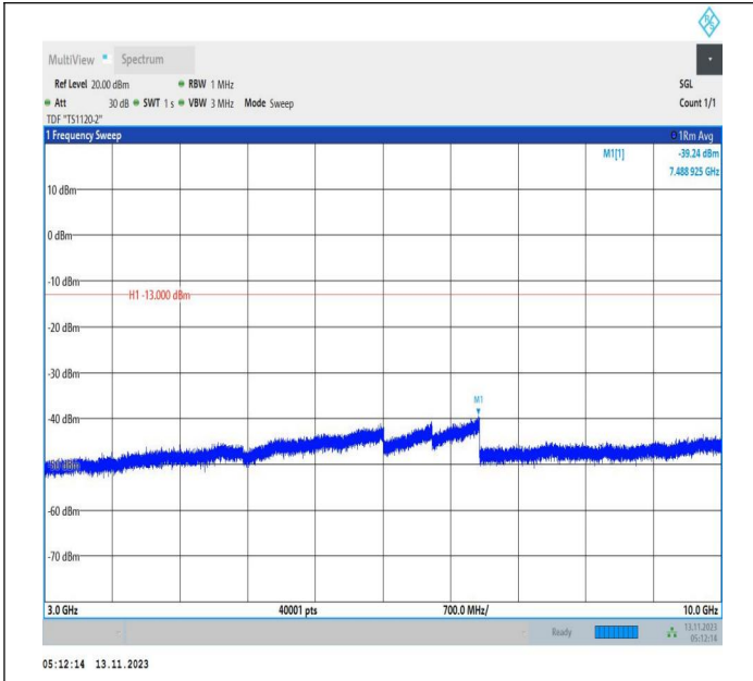
Band71_15MHz_QPSK_133397_1RB#0_3000~10000_3000~10000
