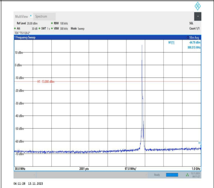
Band71_5MHz_16QAM_133447_1RB#0_30~1000_30~1000
