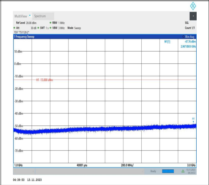
Band71_10MHz_QPSK_133297_1RB#0_1000~3000_1000~3000
