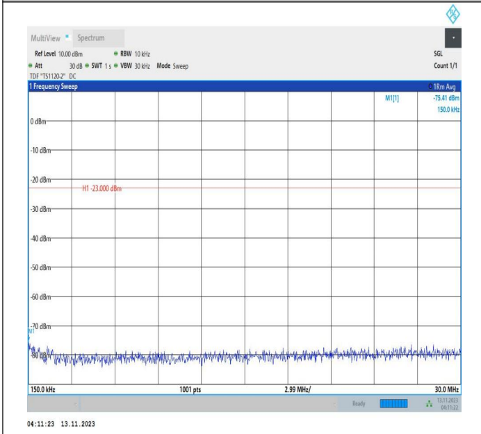
Band71_5MHz_16QAM_133447_1RB#0_0.15~30_0.15~30
