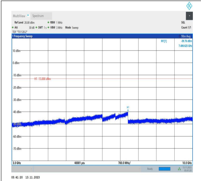
Band71_20MHz_QPSK_133322_1RB#0_3000~10000_3000~10000
