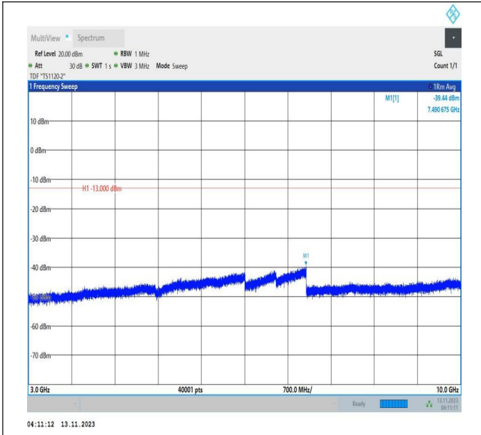
Band71_5MHz_QPSK_133447_1RB#0_3000~10000_3000~10000
