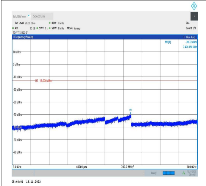
Band71_20MHz_QPSK_133222_1RB#0_3000~10000_3000~10000
