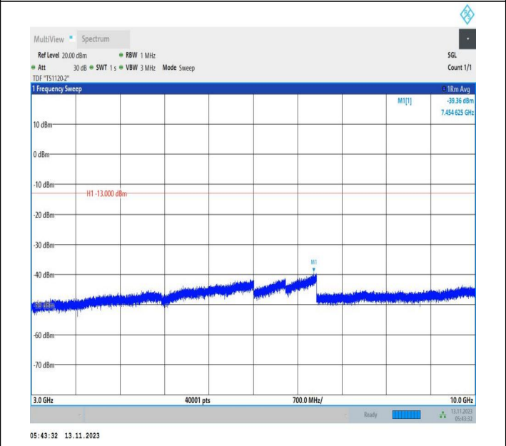
Band71_20MHz_16QAM_133372_1RB#0_3000~10000_3000~10000
