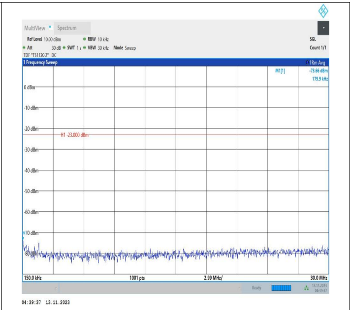
Band71_10MHz_QPSK_133297_1RB#0_0.15~30_0.15~30
