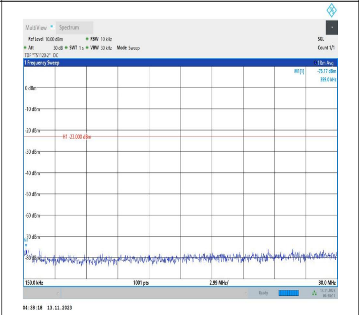
Band71_10MHz_QPSK_133172_1RB#0_0.15~30_0.15~30
