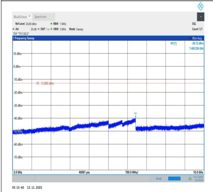
Band71_15MHz_QPSK_133297_1RB#0_3000~10000_3000~10000
