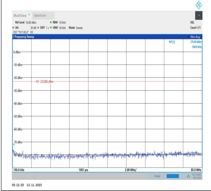
Band71_15MHz_16QAM_133397_1RB#0_0.15~30_0.15~30
