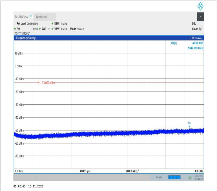
Band71_20MHz_QPSK_133372_1RB#0_1000~3000_1000~3000 00
