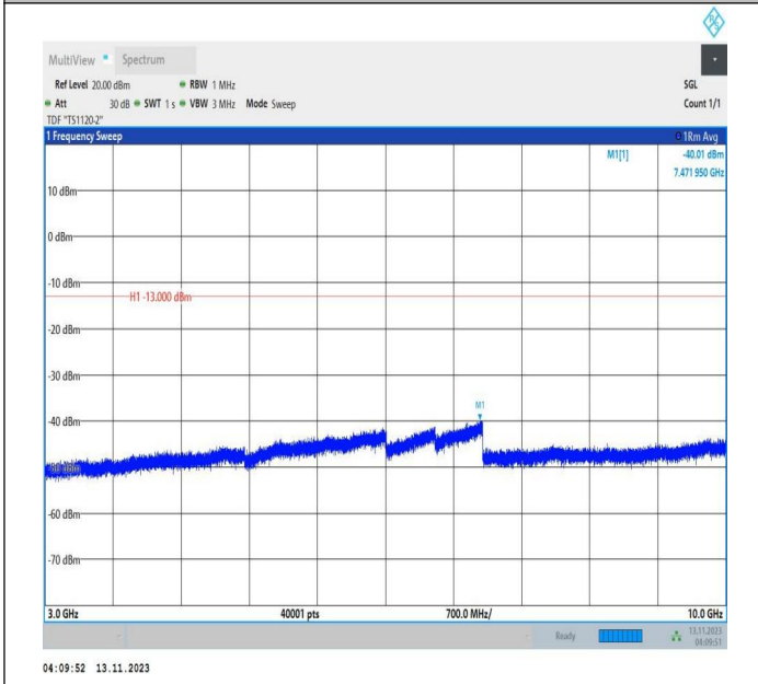
Band71_5MHz_QPSK_133297_1RB#0_3000~10000_3000~1 0000
