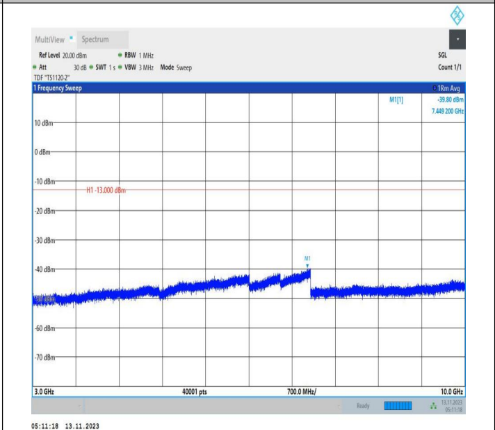
Band71_15MHz_16QAM_133297_1RB#0_3000~10000_3000~10000
