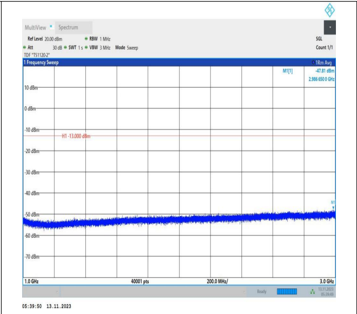
Band71_20MHz_QPSK_133222_1RB#0_1000~3000_1000~3000
