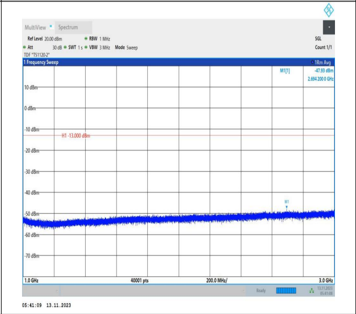
Band71_20MHz_QPSK_133322_1RB#0_1000~3000_1000~3000
