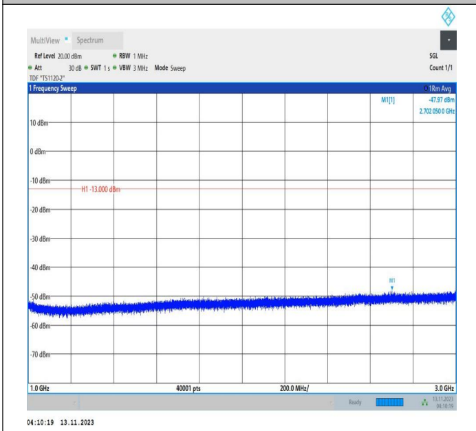
Band71_5MHz_16QAM_133297_1RB#0_1000~3000_1000~3000
