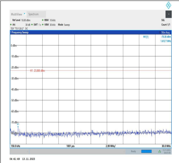
Band71_10MHz_16QAM_133422_1RB#0_0.15~30_0.15~30
