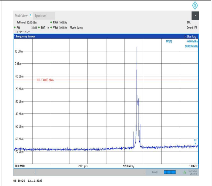
Band71_10MHz_16QAM_133297_1RB#0_30~1000_30~1000
