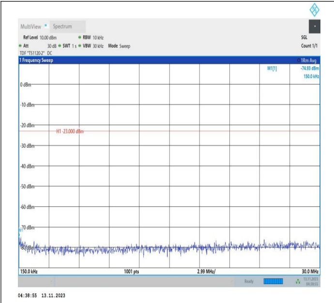
Band71_10MHz_16QAM_133172_1RB#0_0.15~30_0.15~30
