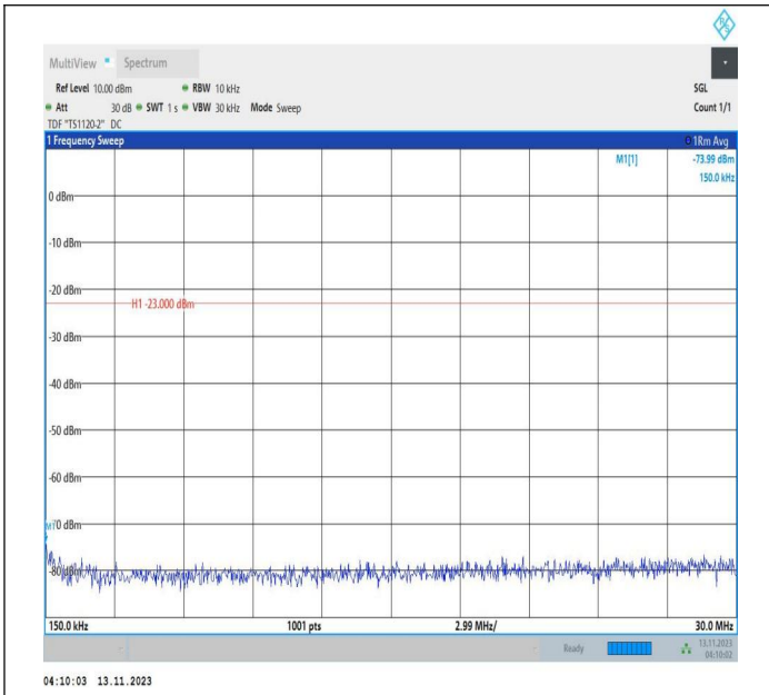
Band71_5MHz_16QAM_133297_1RB#0_0.15~30_0.15~30
