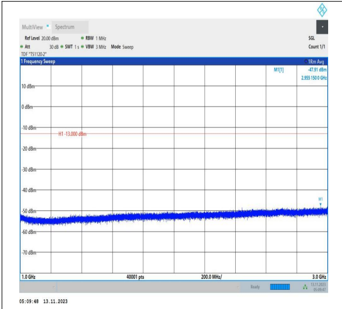
Band71_15MHz_16QAM_133197_1RB#0_1000~3000_1000~3000
