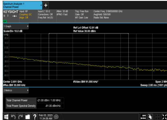
N41(100M)_DFT-s-OFDM_BPSK_Edge_1RB_Right_High_CH_CHP_PA
