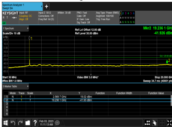
N41(50M)_DFT-s-OFDM_QPSK_Edge_1RB_Left_Mid_CH
