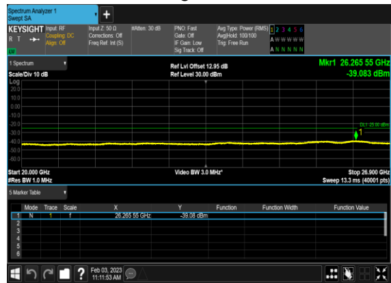
N41(50M)_DFT-s-OFDM_QPSK_Edge_1RB_Left_Mid_CH
