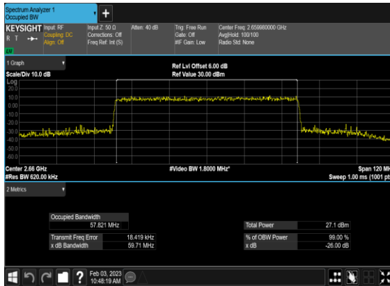
N41(60M)_CP-OFDM_64 QAM_Outer_Full_High_CH
