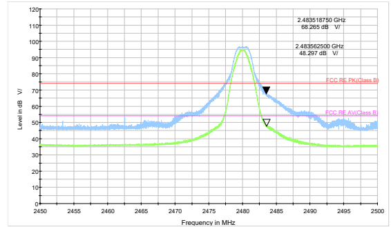
Bluetooth LE (2M) Channel 39 Peak+Average
