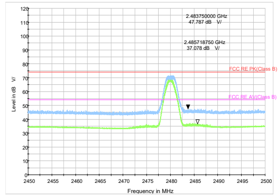
Bluetooth LE (2M) Channel 39 Peak+Average
