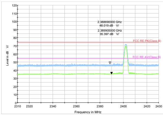
Bluetooth LE (2M) Channel 0 Peak+ Average
