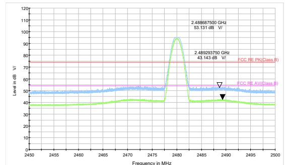
Bluetooth LE (1M) Channel 39 Peak+Average
