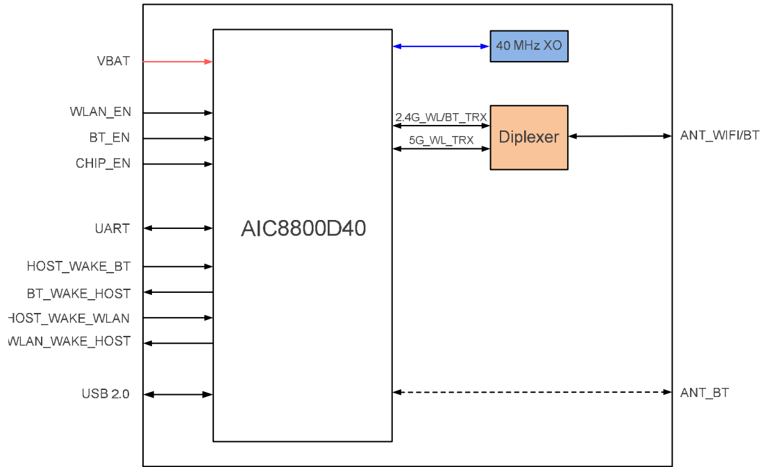
Figure 1: Functional Diagram
