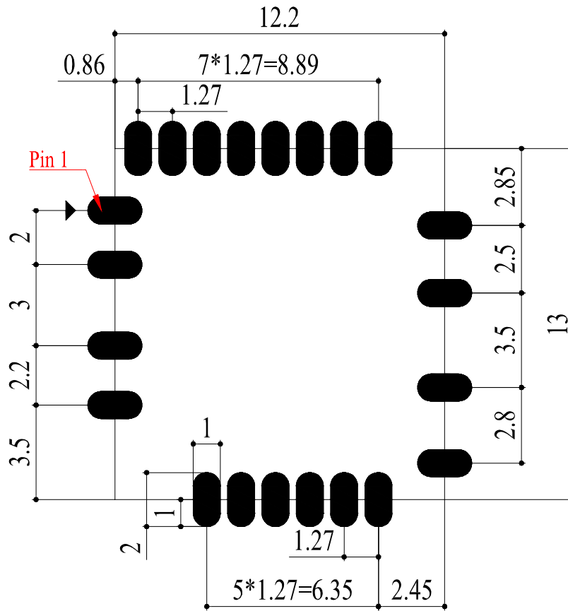
Figure 19: Recommended Footprint
