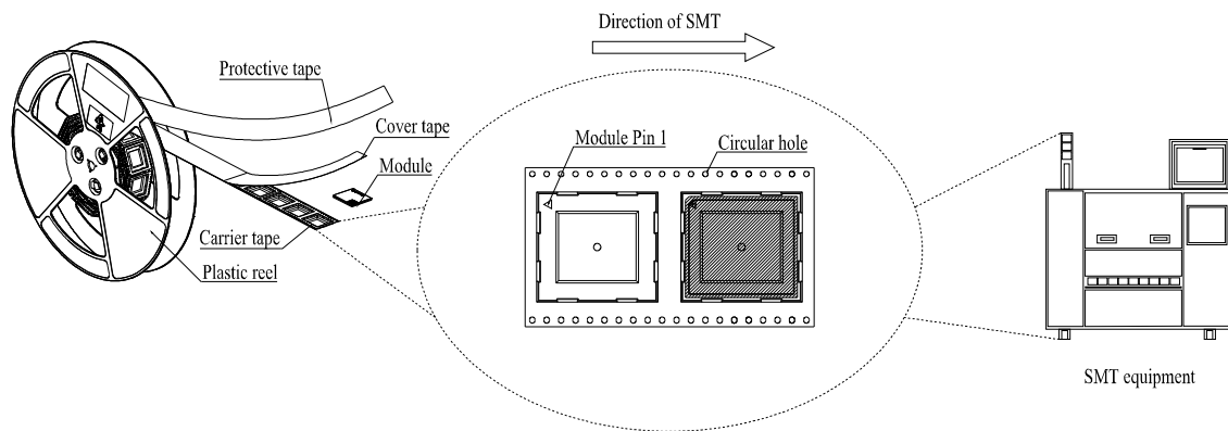
Figure 24: Mounting Direction
