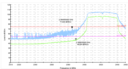
802.11n HT40-Channel 3 Peak+ Average
