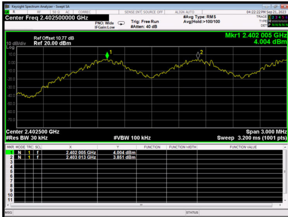
CFS 1-DH5 2402MHz
