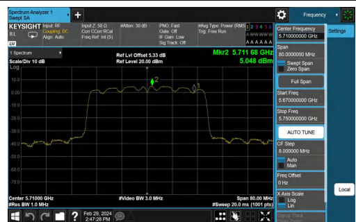
11N40SISO-Ant2-5710_UNII-3-PASS
