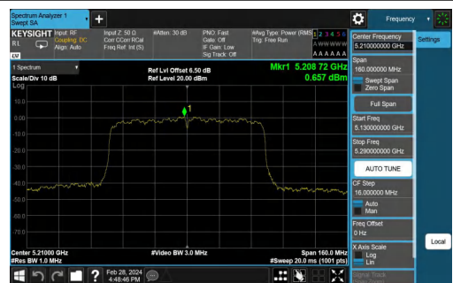
11AC80MIMO-Ant2-5210-PASS
