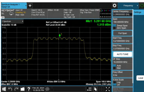
11AC80MIMO-Ant1-5290-PASS
