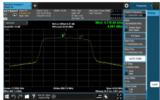
11A-CDD-Ant2-5720_UNII-3-PASS
