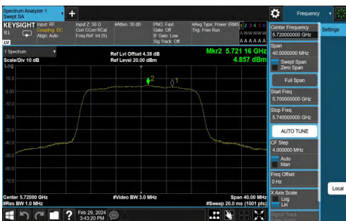
11N20MIMO-Ant1-5720_UNII-3-PASS
