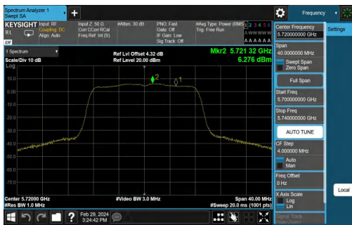
11A-CDD-Ant1-5720_UNII-3-PASS
