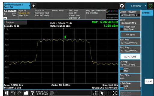
11AC80MIMO-Ant2-5290-PASS
