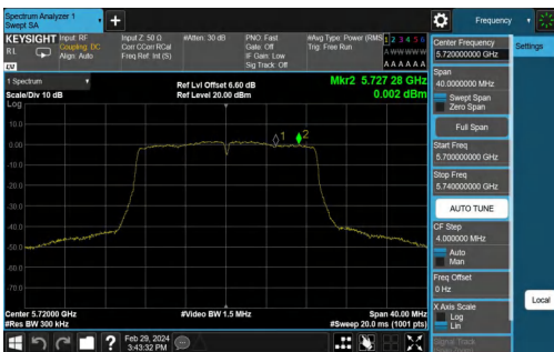
11N40SISO-Ant1-5510-PASS
