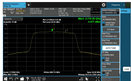
11N20MIMO-Ant2-5720_UNII-3-PASS
