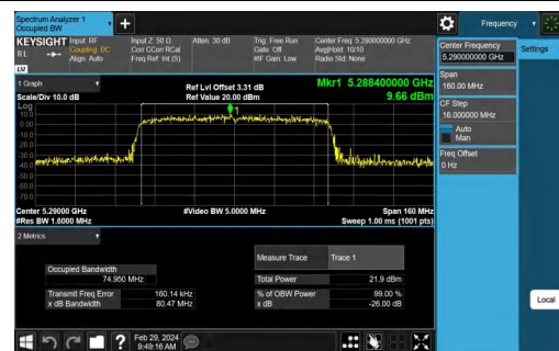
11AC80MIMO-Ant2-5290
