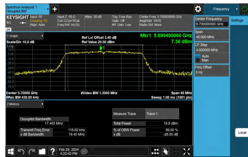
11AC20MIMO-Ant2-5700
