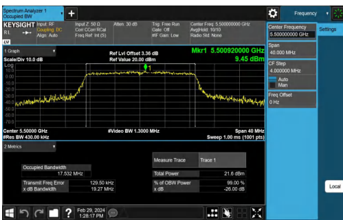
11AC20SISO-Ant1-5580
