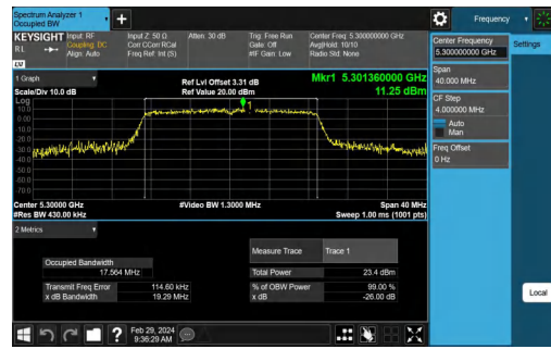
11AC20SISO-Ant2-5320
