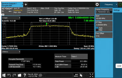
11AC20MIMO-Ant1-5700
