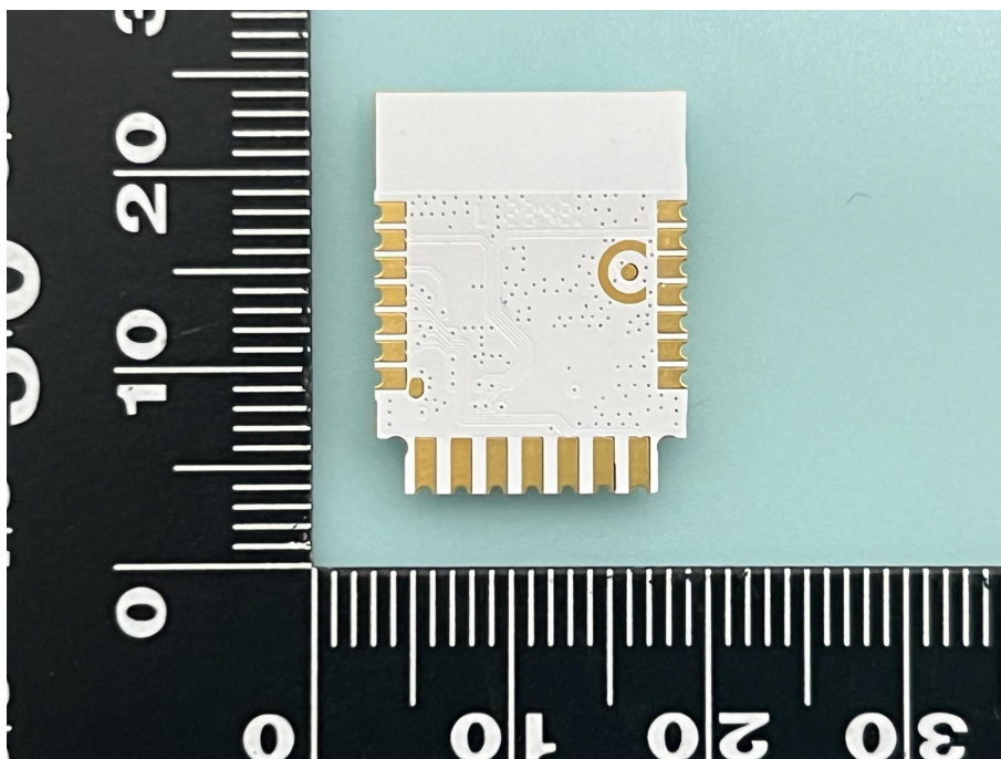
FCM740D_Bottom
