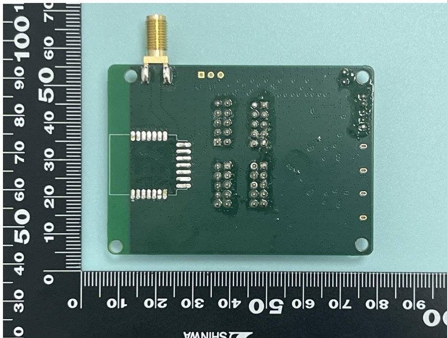
FCM740D + EVB_Bottom
