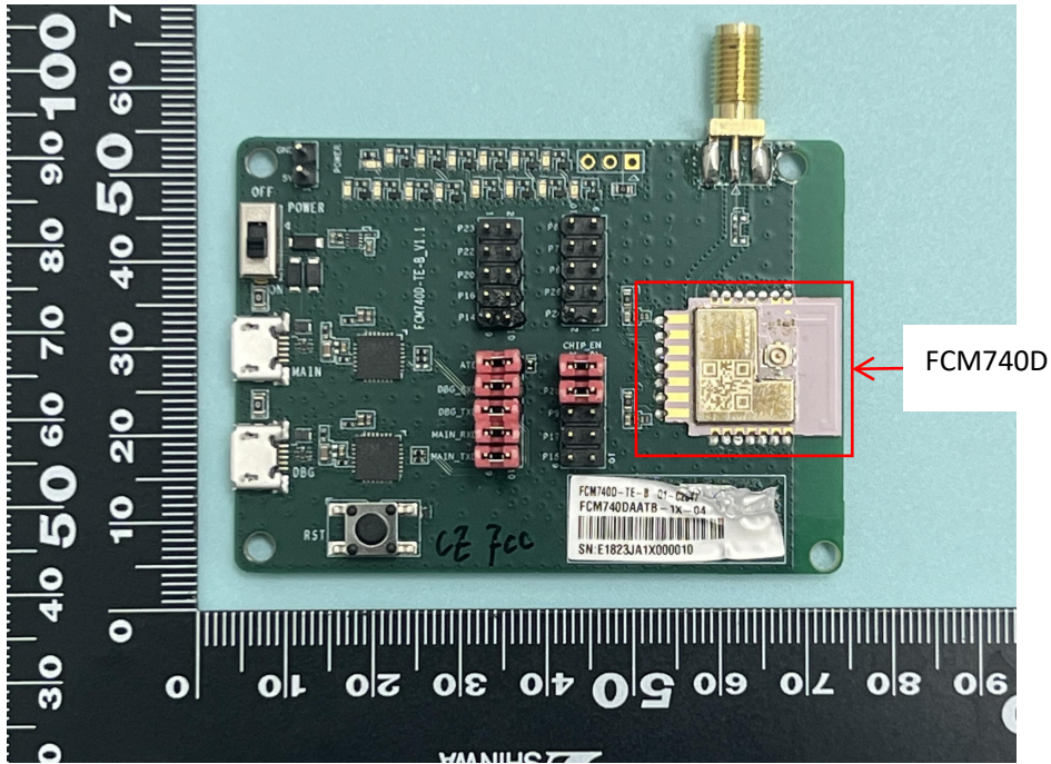
FCM740D + EVB_Top
