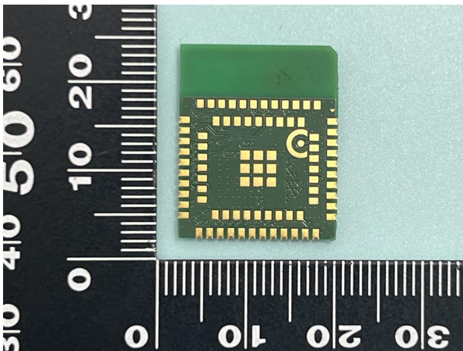
FCM561D-P_Bottom
