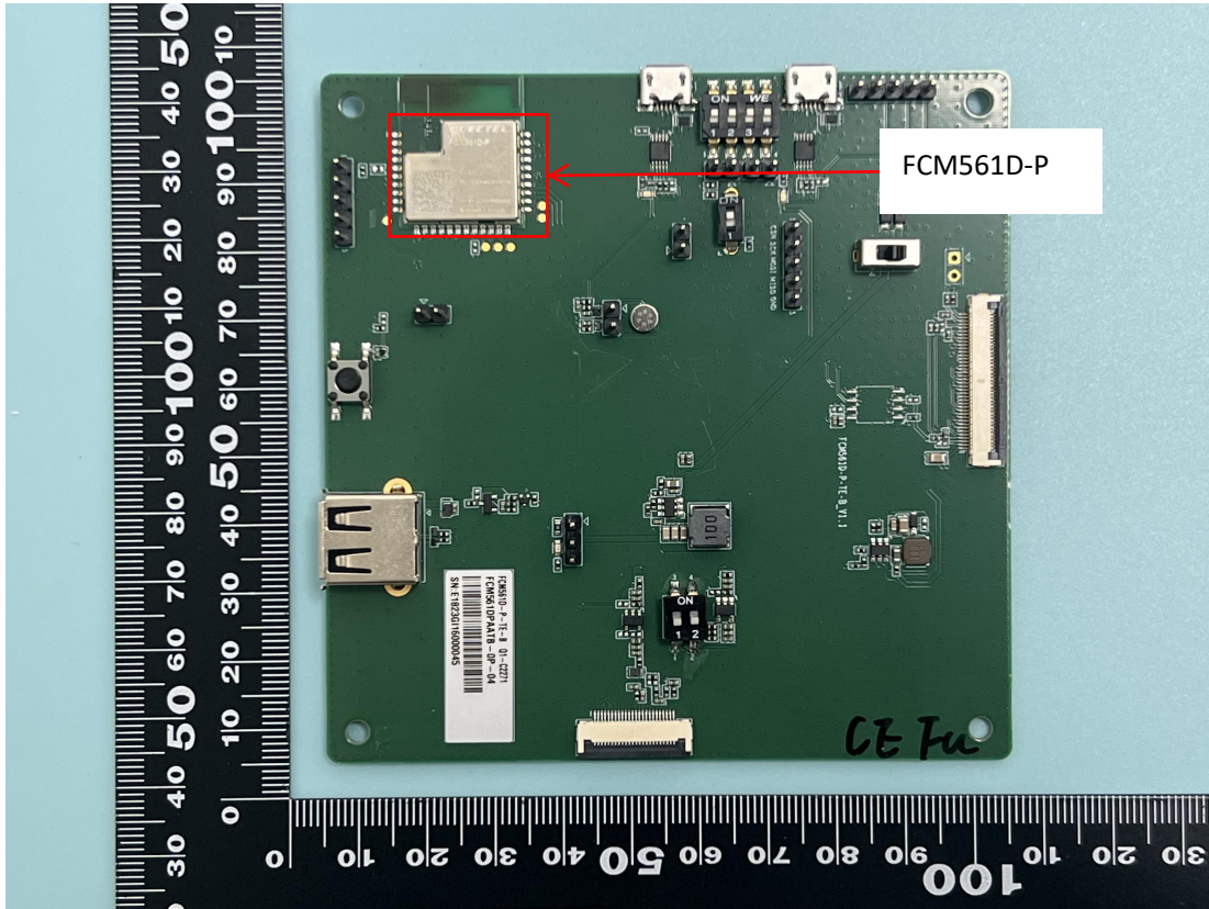
FCM561D-P + EVB_Top
