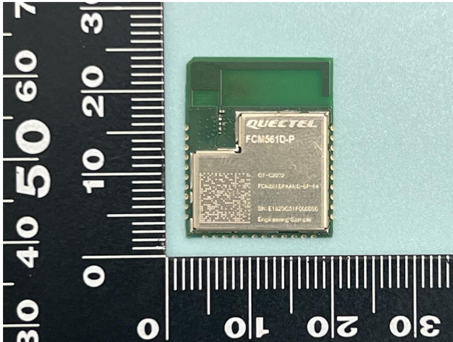
FCM561D-P_Top
