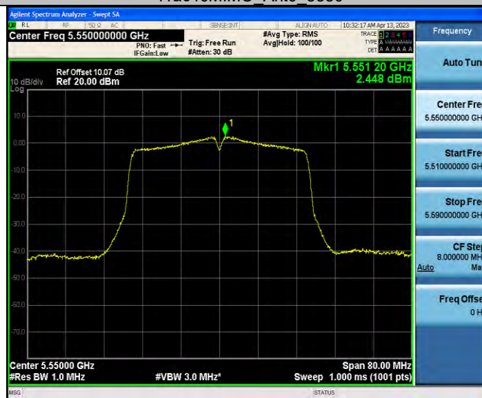
11ac40MIMO Ant0 5550
