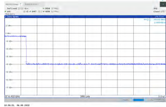
802.11 ax (HE20) /6455MHz Transmission when the interferer is Minimal Operation
