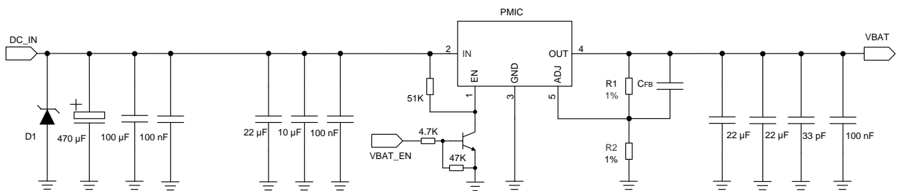
Figure 2: Reference Design of Power Input
