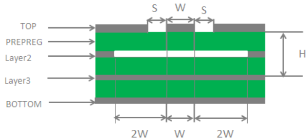
Figure 23: Coplanar Waveguide Design on a 4-layer PCB (Layer 3 as Reference Ground)
