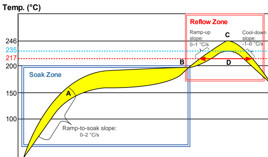
Figure 32: Recommended Reflow Soldering Thermal Profile
