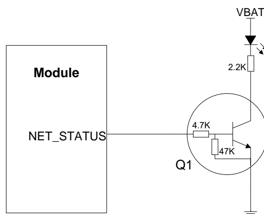
Figure 16: Reference Design of Network Status Indication
