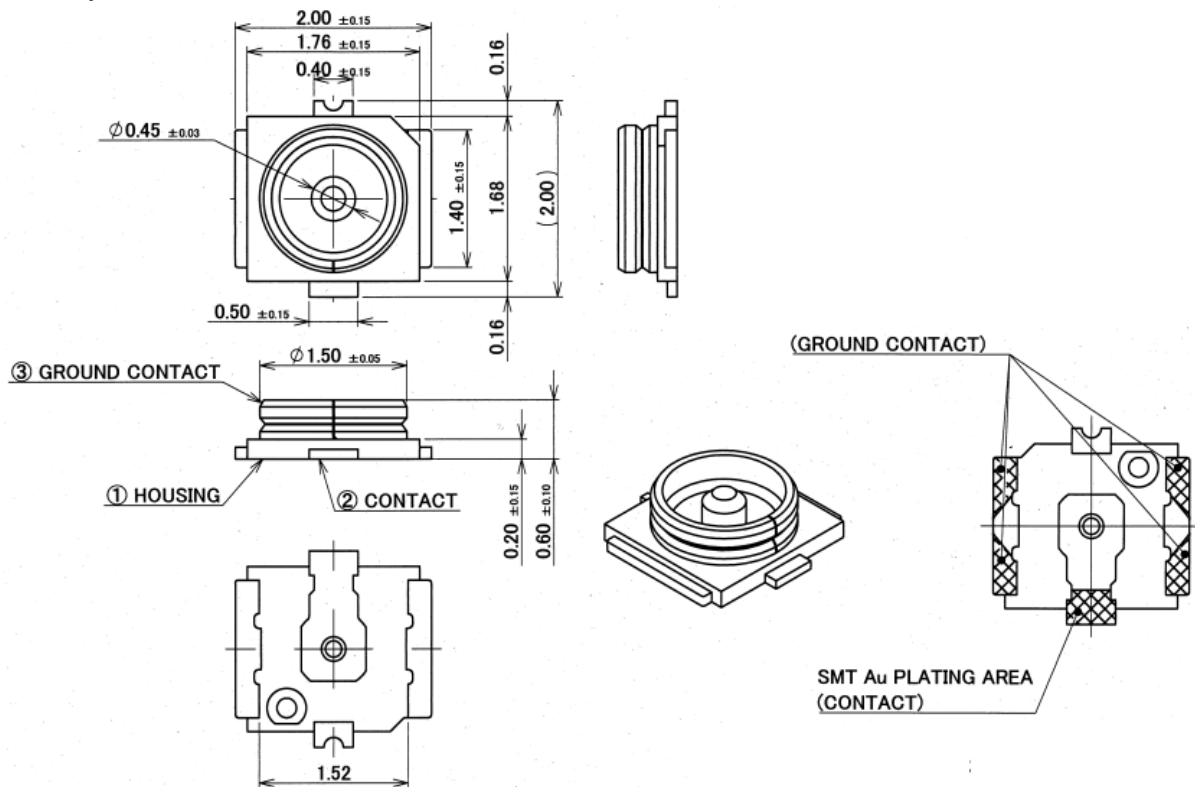
Figure 25: Dimensions of the Receptacle (Unit: mm)
