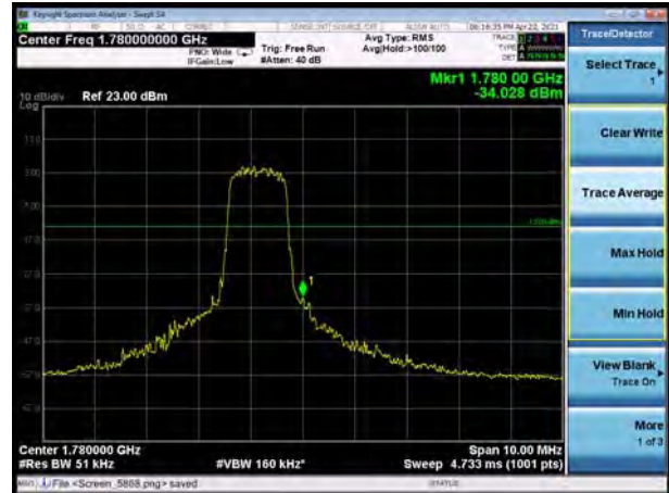
LTE eMTC Band 66 QPSK 5MHz CH-High, 1 RB
