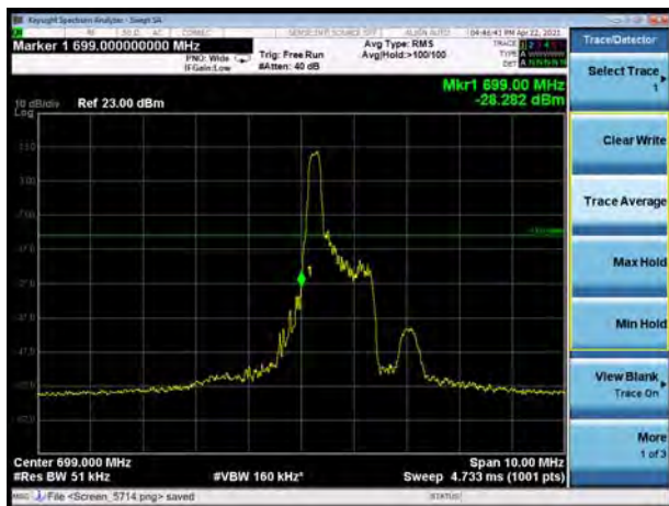
LTE eMTC Band 12 16QAM 1.4MHz CH-Low, 1 RB
