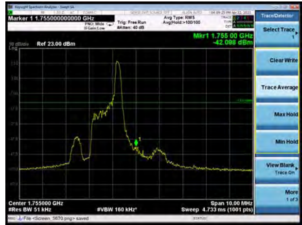
LTE eMTC Band 4 16QAM 10MHz CH-High, 100%RB
