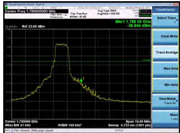
LTE eMTC Band 66 16QAM 20MHz CH-High, 1 RB
