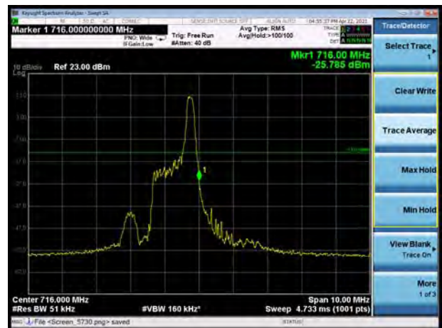
LTE eMTC Band 12 16QAM 1.4MHz CH-High, 1 RB
