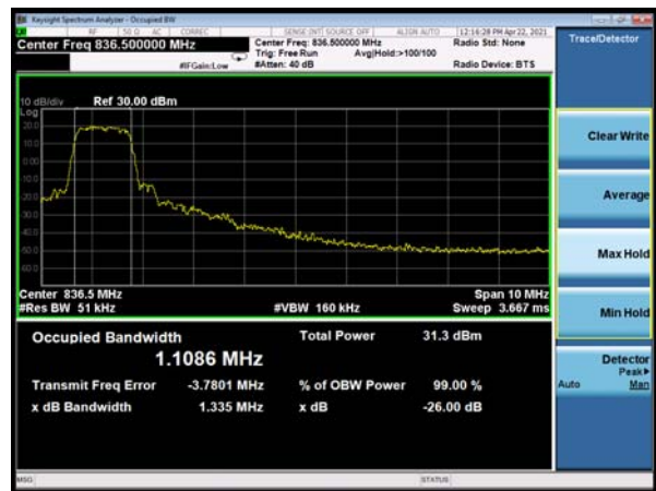
LTE eMTC Band 5 QPSK 10MHz CH-Middle
