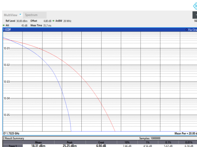
Band4-20MHz-QPSK-20175-100RB#0
