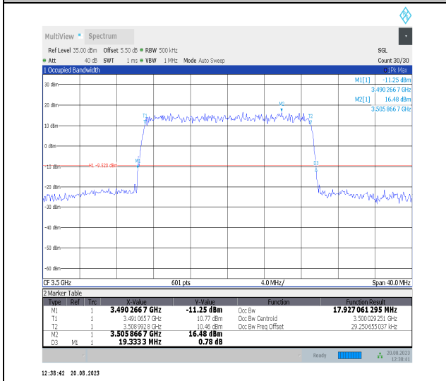
Band42-20MHz-QPSK-42590-100RB#0-PASS
