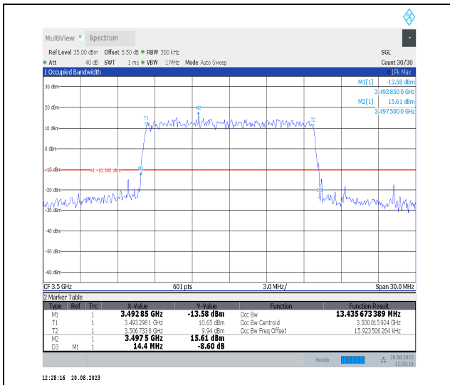
Band42-15MHz-QPSK-42590-75RB#0-PASS
