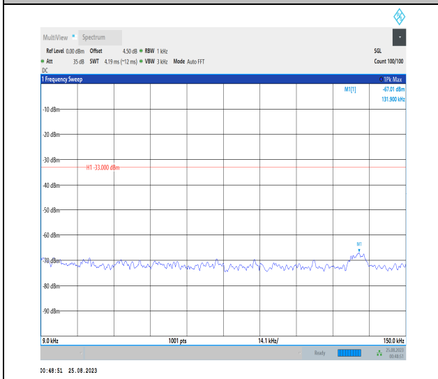
Band42_20MHz_QPSK_42990_1RB#0_0.009~0.15_0.009~0.15
