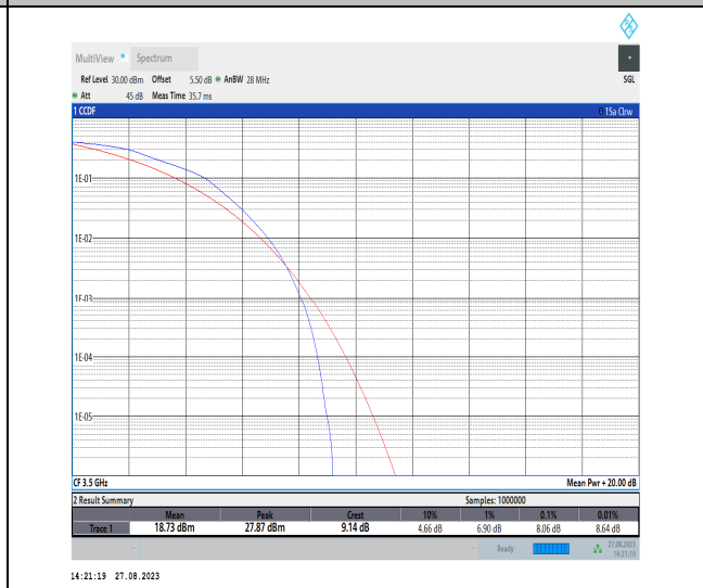
Band42-20MHz-16QAM-42590-100RB#0-PASS
