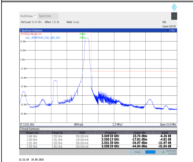
Band42_10MHz_QPSK_43040_1RB#49
