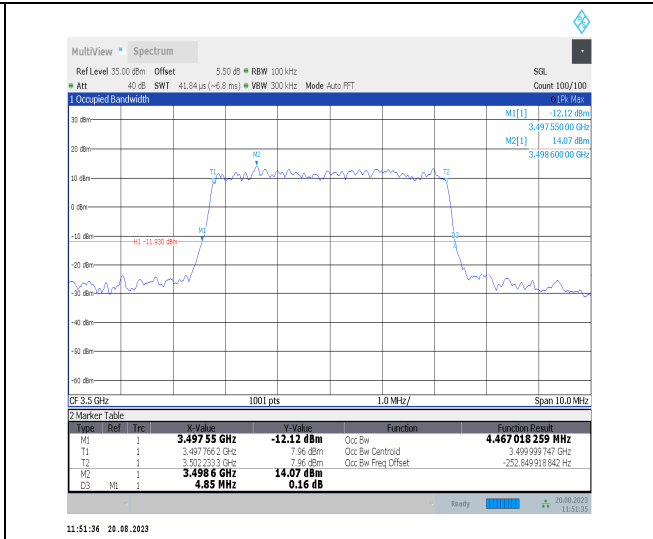
Band42-5MHz-16QAM-42590-25RB#0-PASS
