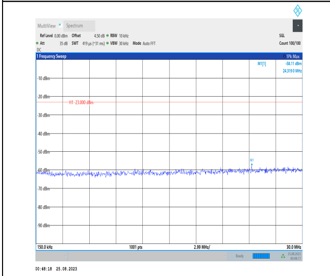
Band42_20MHz_QPSK_42590_1RB#0_0.15~30_0.15~30
