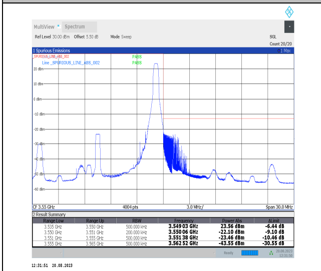
Band42_15MHz_QPSK_43015_1RB#74
