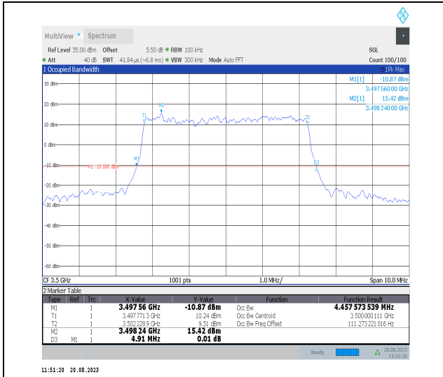
Band42-5MHz-QPSK-42590-25RB#0-PASS
