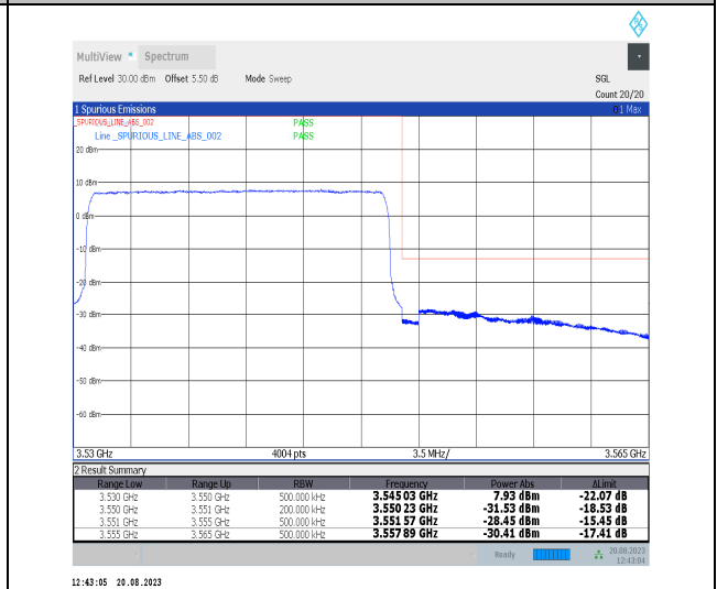
Band42_20MHz_QPSK_42990_100RB#0
