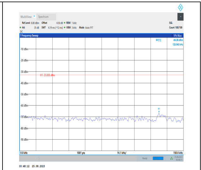
Band42_20MHz_QPSK_42590_1RB#0_0.009~0.15_0.09~0.15
