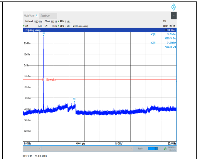
Band42_20MHz_QPSK_42990_1RB#0_1000~20000_1000~20000
