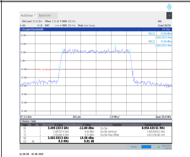
Band42-10MHz-16QAM-42590-50RB#0-PASS
