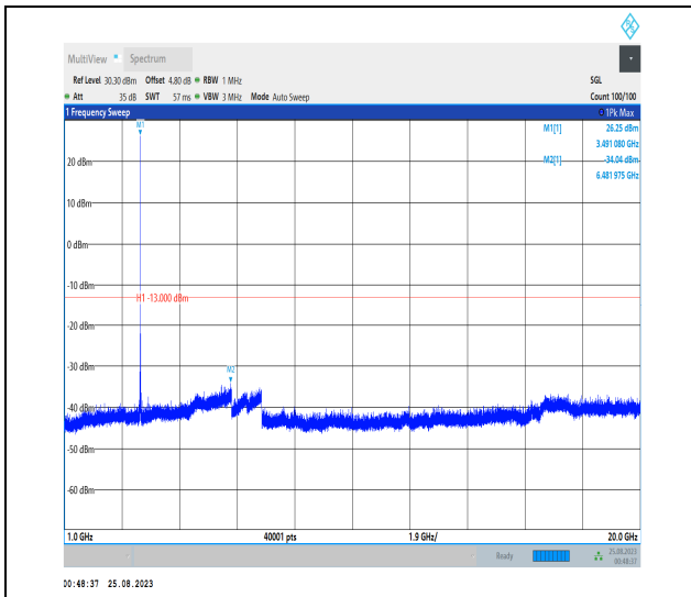
Band42_20MHz_QPSK_42590_1RB#0_1000~20000_1000~20000
