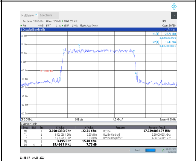
Band42-20MHz-16QAM-42590-100RB#0-PASS
