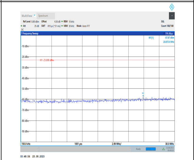
Band42_20MHz_QPSK_42990_1RB#0_0.15~30_0.15~30
