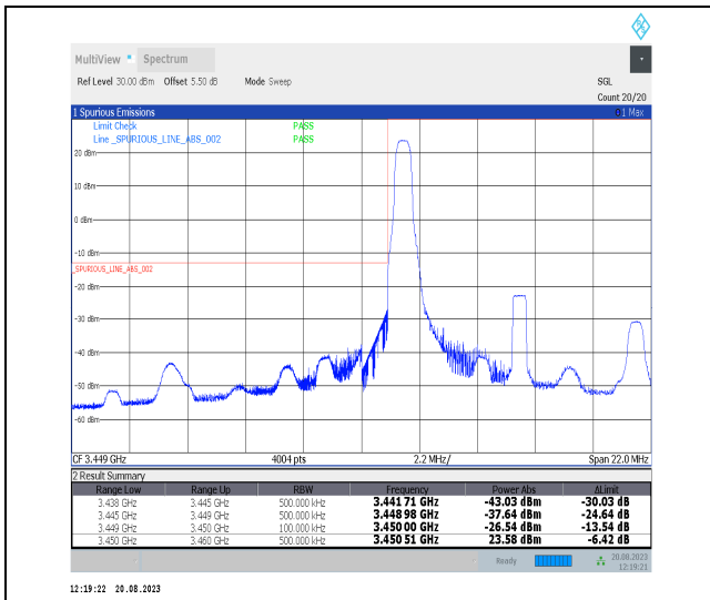
Band42_10MHz_QPSK_42140_1RB#0
