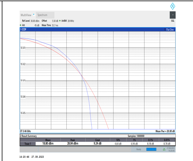
Band42-20MHz-16QAM-42190-100RB#0-PASS
