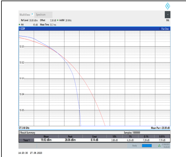
Band42-20MHz-QPSK-42190-100RB#0-PASS
