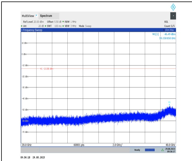
Band42_20MHz_QPSK_42190_1RB#0_20000~40000_20 000~40000
