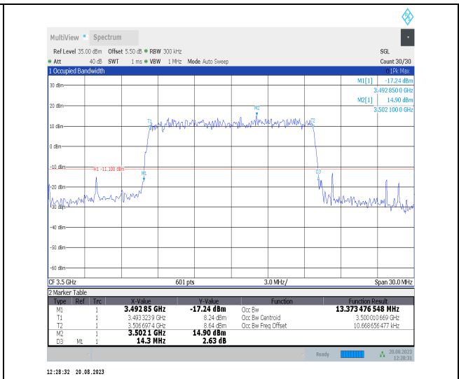
Band42-15MHz-16QAM-42590-75RB#0-PASS
