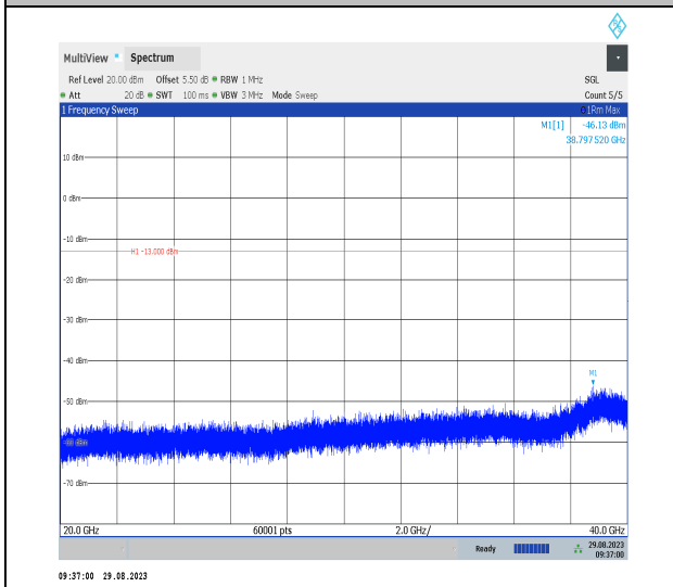
Band42_20MHz_QPSK_42990_1RB#0_20000~40000_20000~40000
