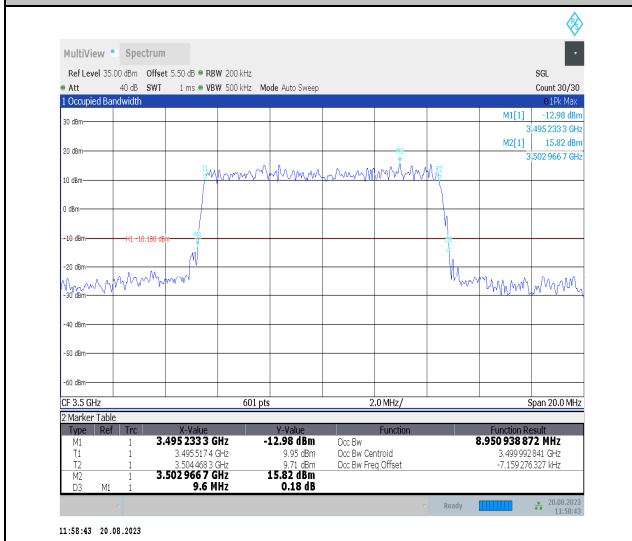
Band42-10MHz-QPSK-42590-50RB#0-PASS
