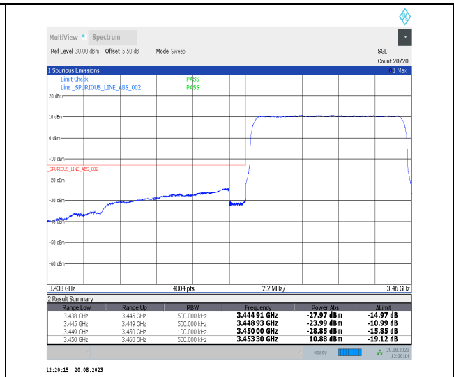
Band42_10MHz_QPSK_42140_50RB#0
