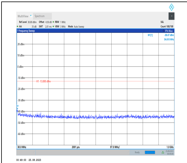
Band42_20MHz_QPSK_42990_1RB#0_30~1000_30~1000
