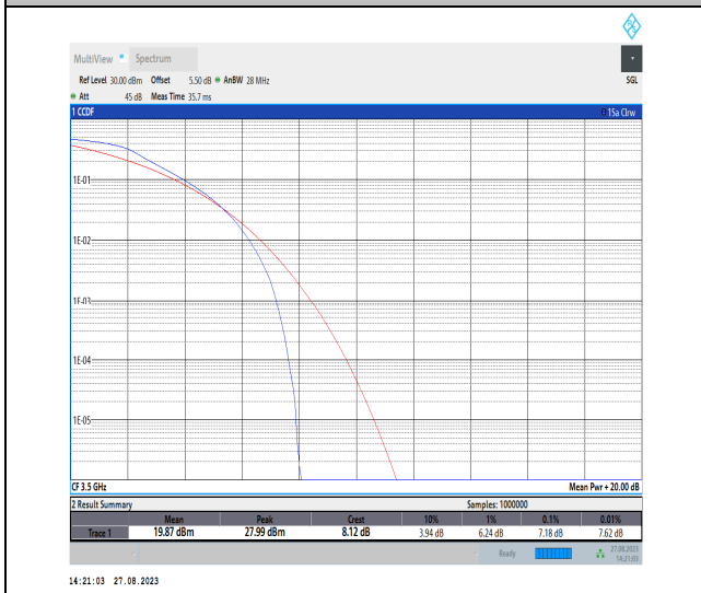
Band42-20MHz-QPSK-42590-100RB#0-PASS
