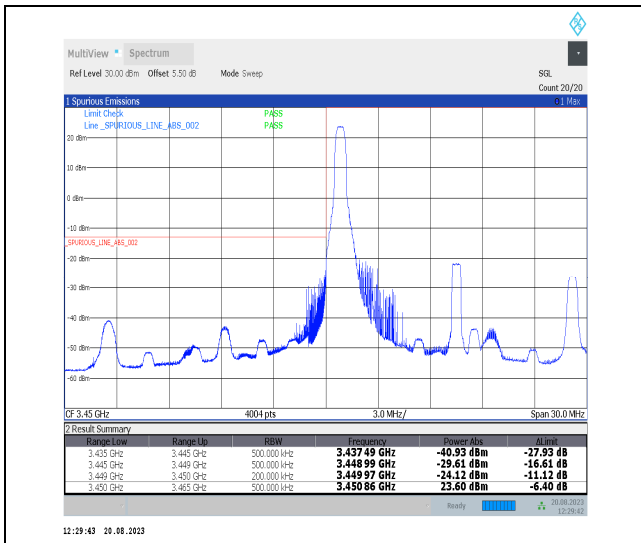
Band42_15MHz_QPSK_42165_1RB#0
