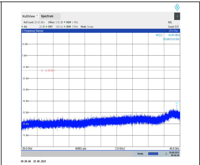
Band42_20MHz_QPSK_42590_1RB#0_20000~40000_20000~40000
