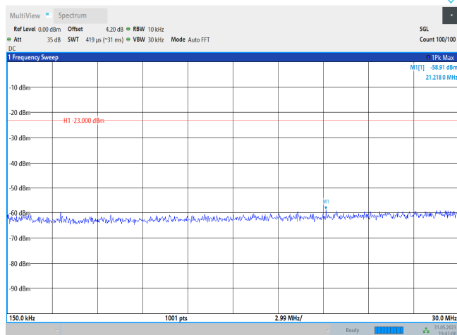
Band26-15MHz-QPSK-26865-1RB#0-Range2:0.15~30MHz
