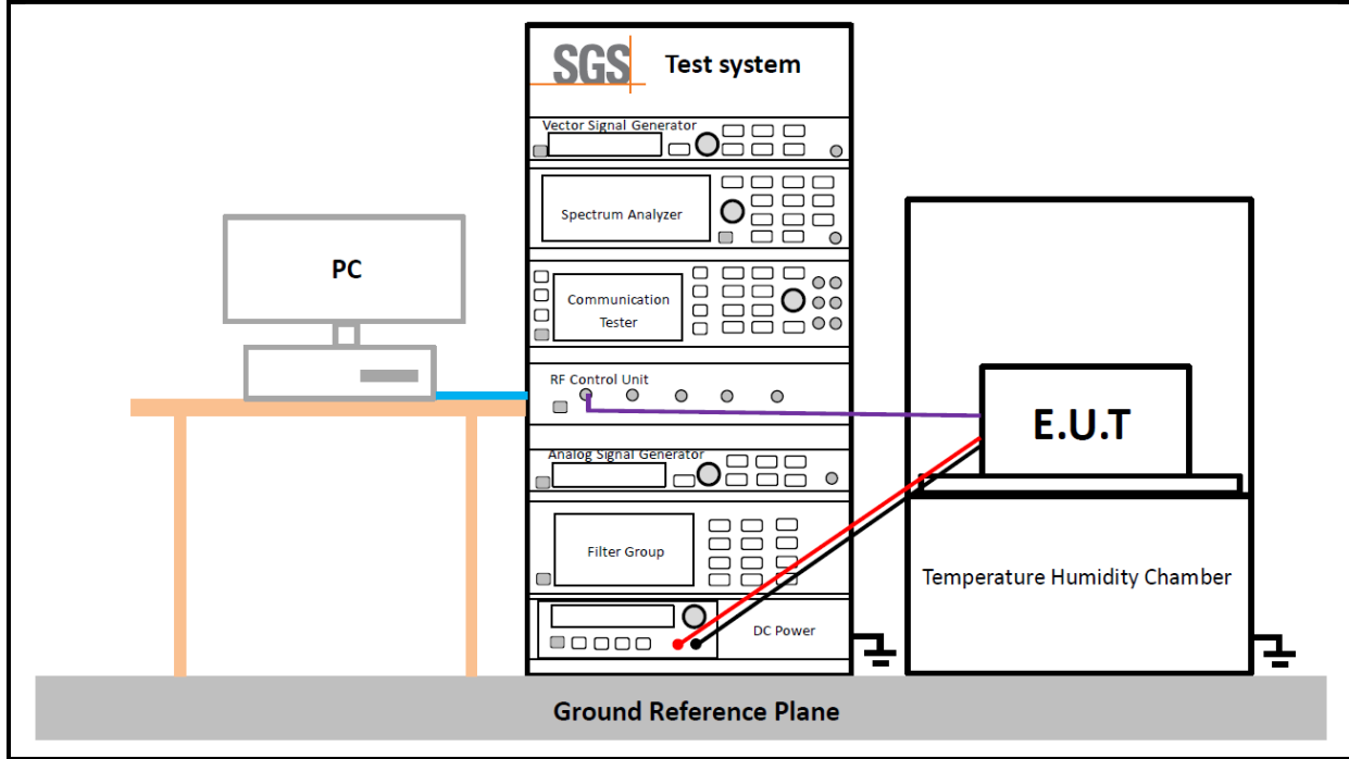
Figure 3. above 1GHz
