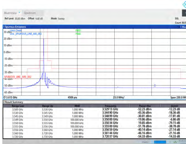
Band48-5MHz-QPSK-55265-1RB#0
