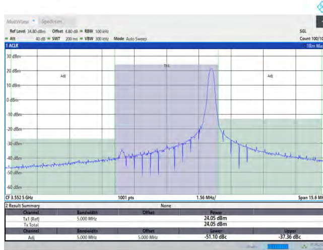
Band48-5MHz-QPSK-55265-1RB#24
