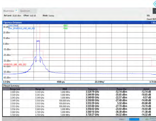
Band48-5MHz-QPSK-55265-25RB#0
