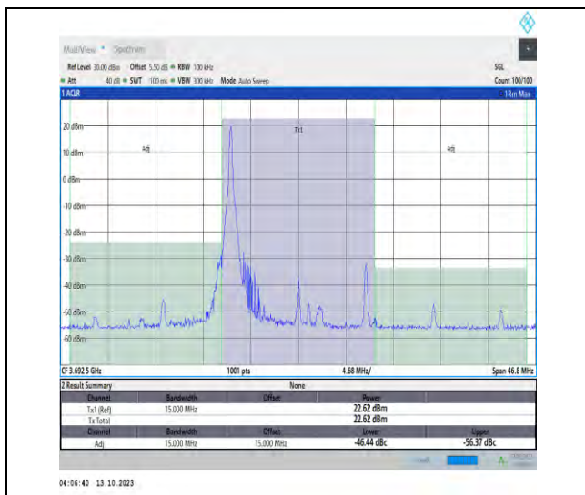
43(3600-3700)-15MHz-QPSK-44515-1RB#0-PASS
