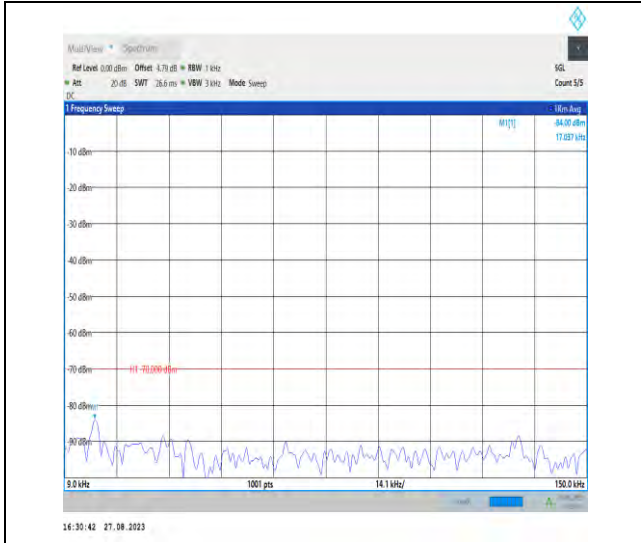
Band43_20MHz_QPSK_44490_1RB#0_0.009~0.15_0.09~0.15
