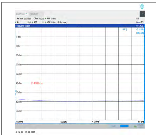
Band43_20MHz_QPSK_44090_1RB#0_30~1000_30~1000
