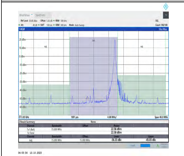
43(3600-3700)-15MHz-QPSK-44090-1RB#74-PASS
