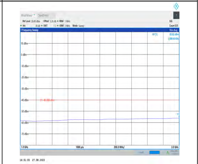
Band43_20MHz_QPSK_44490_1RB#0_1000~3000_1000~3000
