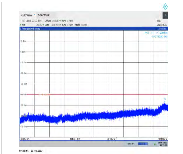
Band43_20MHz_QPSK_43690_1RB#0_6000~40000_600 0~40000
