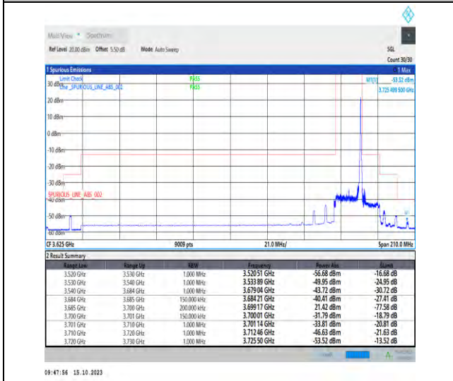
Band43_15MHz_QPSK_44515_1RB#74
