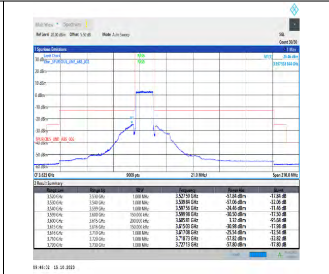
Band43_15MHz_QPSK_43665_75RB#0
