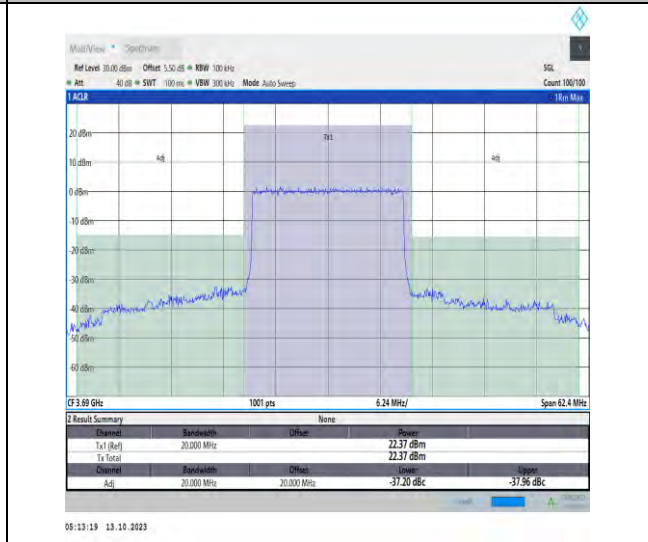
43(3600-3700)-20MHz-QPSK-44490-100RB#0-PASS
