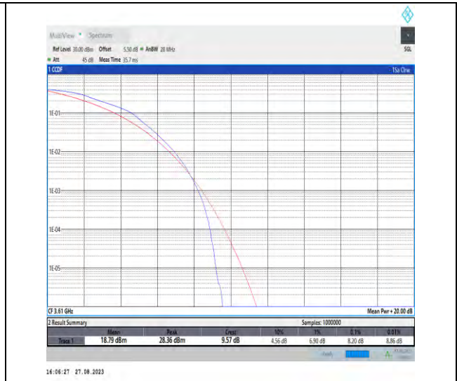
Band43-20MHz-16QAM-43690-100RB#0-PASS
