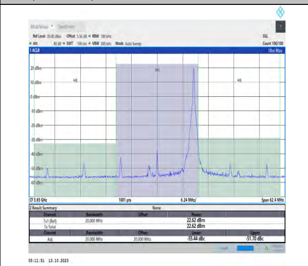
43(3600-3700)-20MHz-QPSK-44090-1RB#99-PASS
