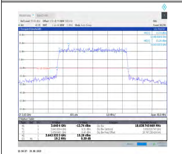
Band43-20MHz-QPSK-44090-100RB#0-PASS
