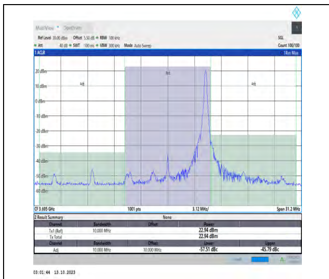
43(3600-3700)-10MHz-QPSK-44540-1RB#49-PASS
