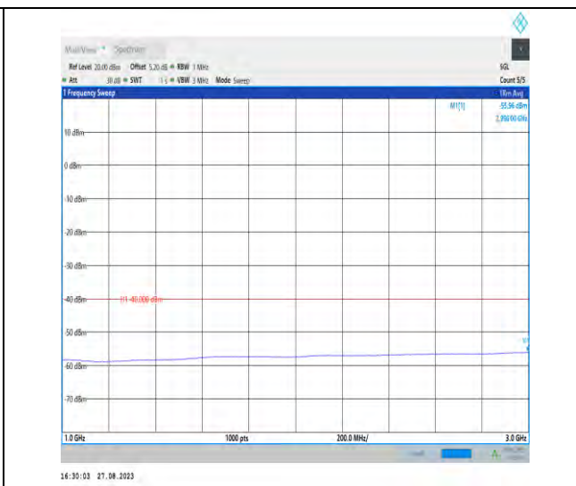
Band43_20MHz_QPSK_44090_1RB#0_1000~3000_1000~3000
