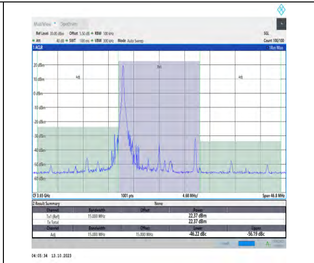
43(3600-3700)-15MHz-QPSK-44090-1RB#0-PASS
