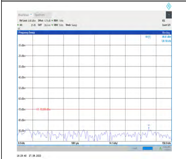
Band43_20MHz_QPSK_44090_1RB#0_0.009~0.15_0.0 09~0.15
