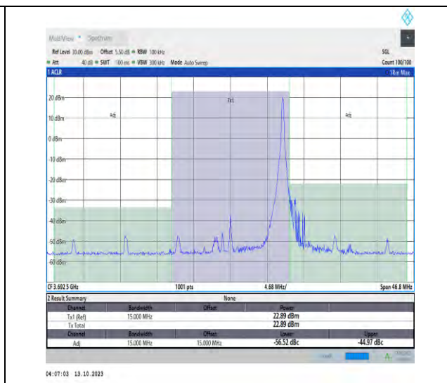
43(3600-3700)-15MHz-QPSK-44515-1RB#74-PASS
