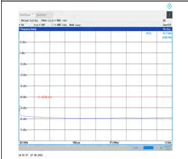
Band43_20MHz_QPSK_44490_1RB#0_30~1000_30~10
