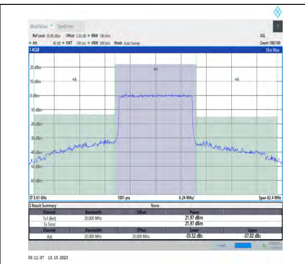
43(3600-3700)-20MHz-QPSK-43690-100RB#0-PASS
