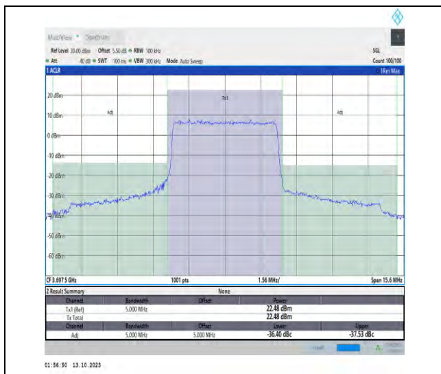
43(3600-3700)-5MHz-QPSK-44565-25RB#0-PASS
