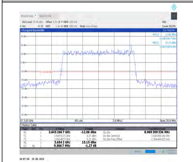
Band43-10MHz-QPSK-44090-50RB#0-PASS
