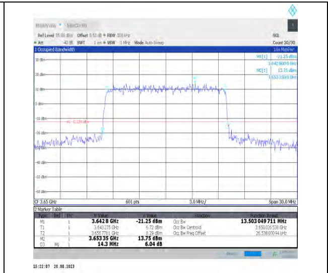
Band43-15MHz-16QAM-44090-75RB#0-PASS
