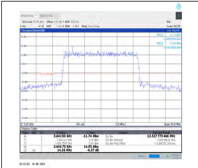
Band43-15MHz-QPSK-44090-75RB#0-PASS
