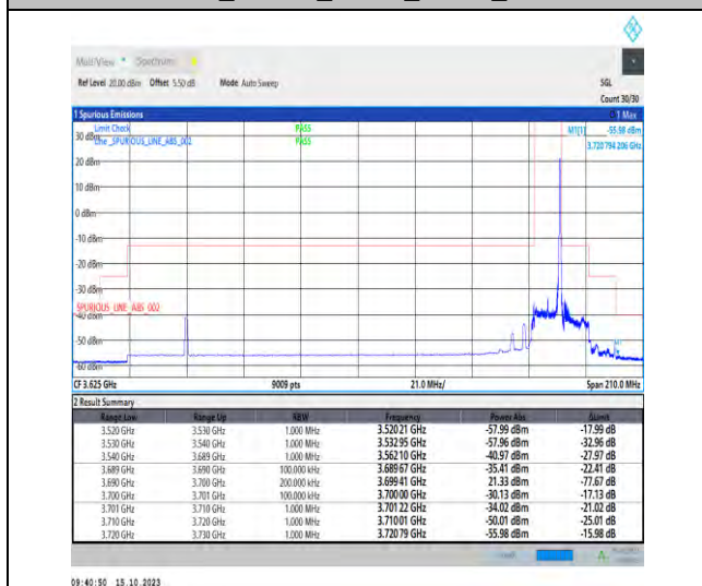
Band43_10MHz_QPSK_44540_1RB#49
