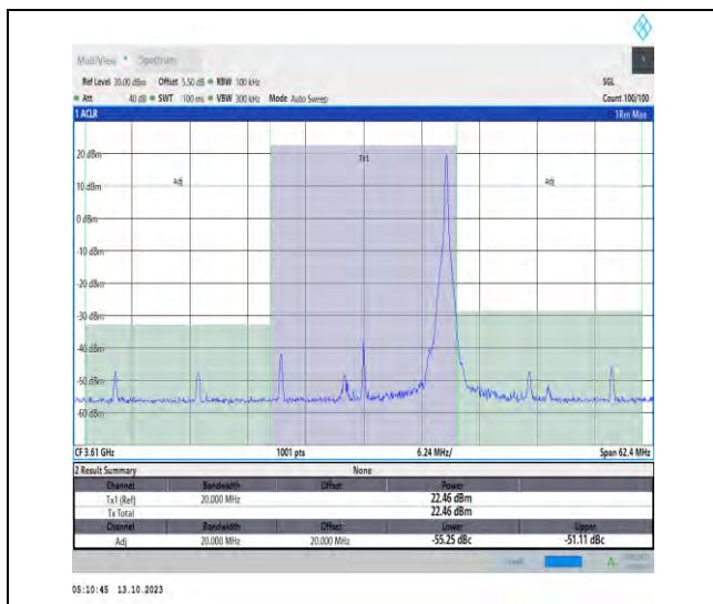
43(3600-3700)-20MHz-QPSK-43690-1RB#99-PASS
