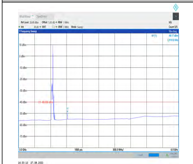
Band43_20MHz_QPSK_44090_1RB#0_3000~6000_3000~6000
