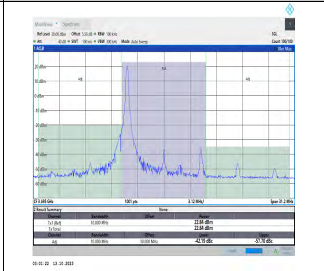
43(3600-3700)-10MHz-QPSK-44540-1RB#0-PASS
