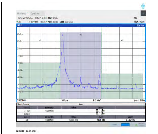
43(3600-3700)-10MHz-QPSK-43640-1RB#0-PASS
