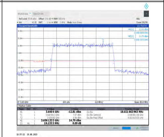
Band43-20MHz-16QAM-44090-100RB#0-PASS
