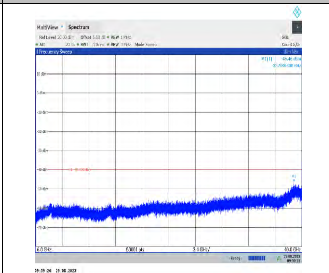
Band43_20MHz_QPSK_44090_1RB#0_6000~40000_6000~40000
