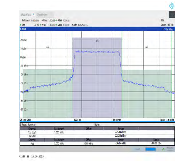
43(3600-3700)-5MHz-QPSK-44090-25RB#0-PASS
