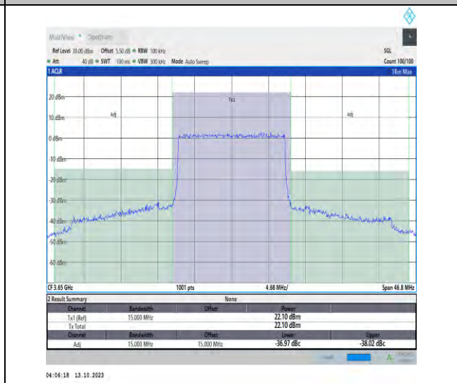
43(3600-3700)-15MHz-QPSK-44090-75RB#0-PASS
