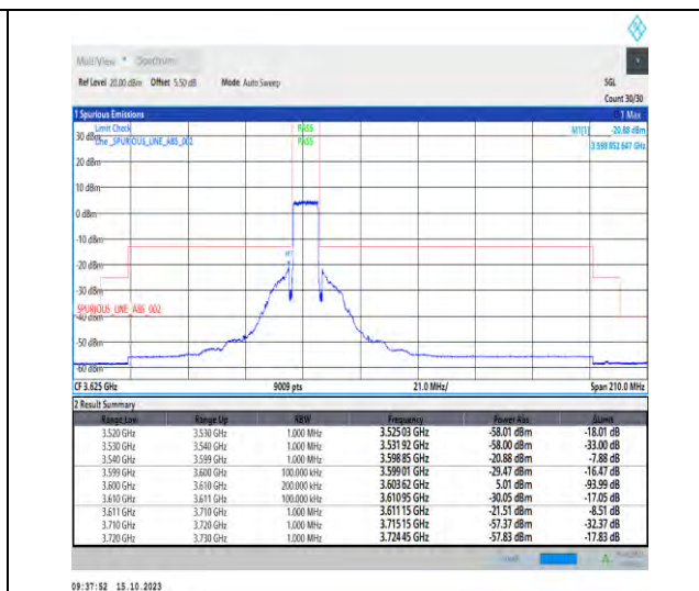
Band43_10MHz_QPSK_43640_50RB#0
