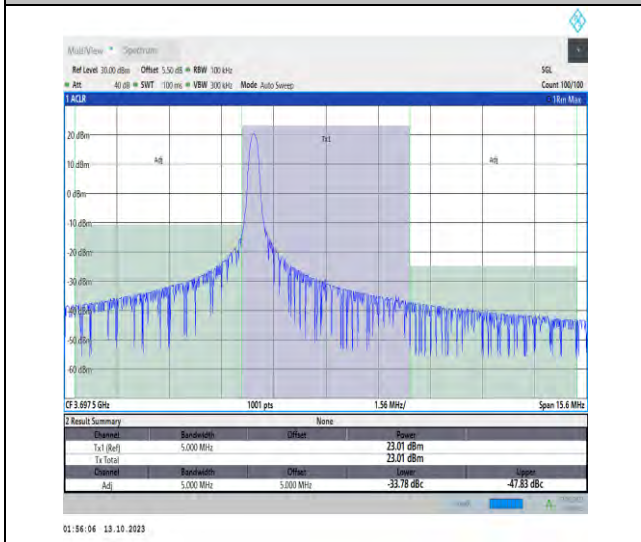
43(3600-3700)-5MHz-QPSK-44565-1RB#0-PASS
