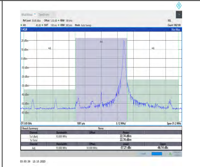
43(3600-3700)-10MHz-QPSK-44090-1RB#49-PASS
