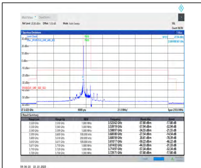
Band43_10MHz_QPSK_43640_1RB#0
