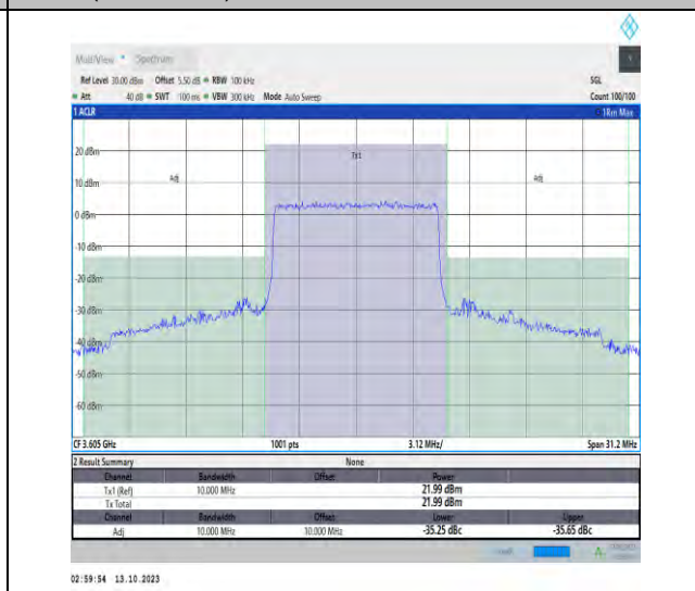
43(3600-3700)-10MHz-QPSK-43640-50RB#0-PASS
