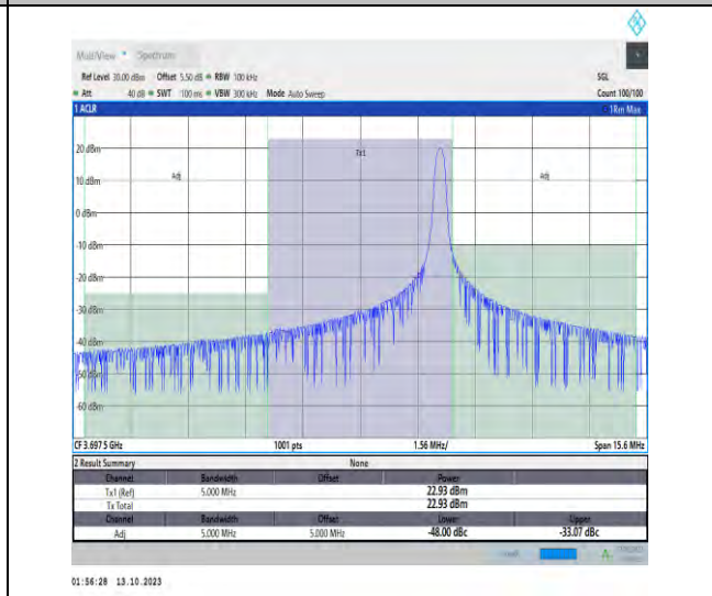
43(3600-3700)-5MHz-QPSK-44565-1RB#24-PASS
