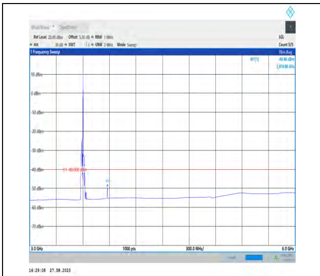
Band43_20MHz_QPSK_43690_1RB#0_3000~6000_30 00~6000
