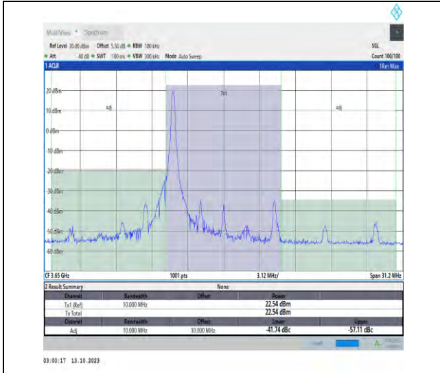
43(3600-3700)-10MHz-QPSK-44090-1RB#0-PASS
