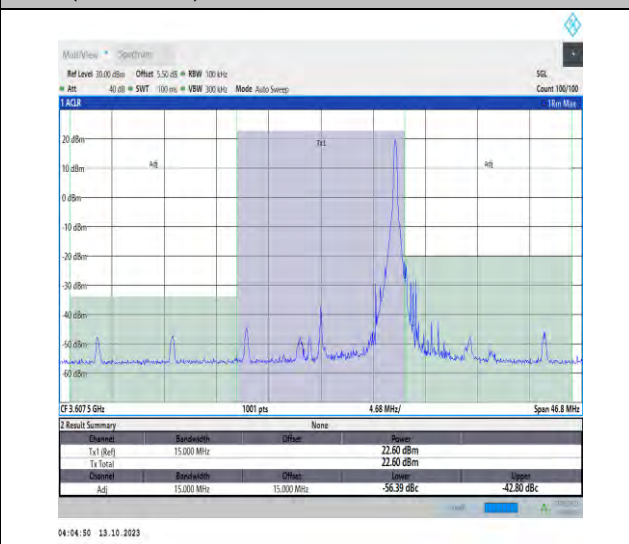
43(3600-3700)-15MHz-QPSK-43665-1RB#74-PASS
