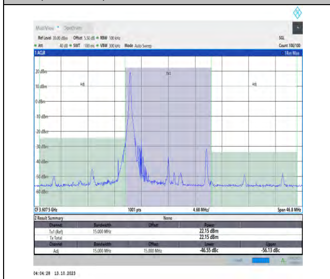
43(3600-3700)-15MHz-QPSK-43665-1RB#0-PASS
