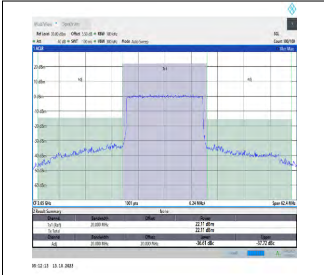
43(3600-3700)-20MHz-QPSK-44090-100RB#0-PASS
