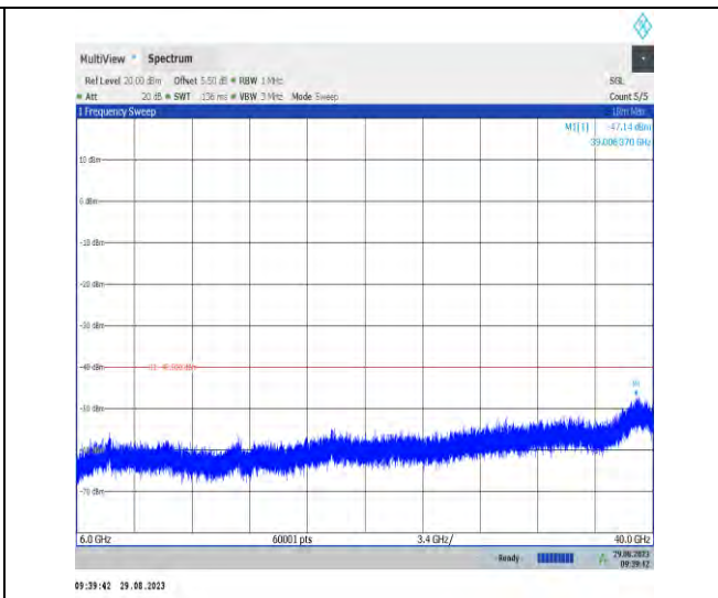
Band43_20MHz_QPSK_44490_1RB#0_6000~40000_600 0~40000
