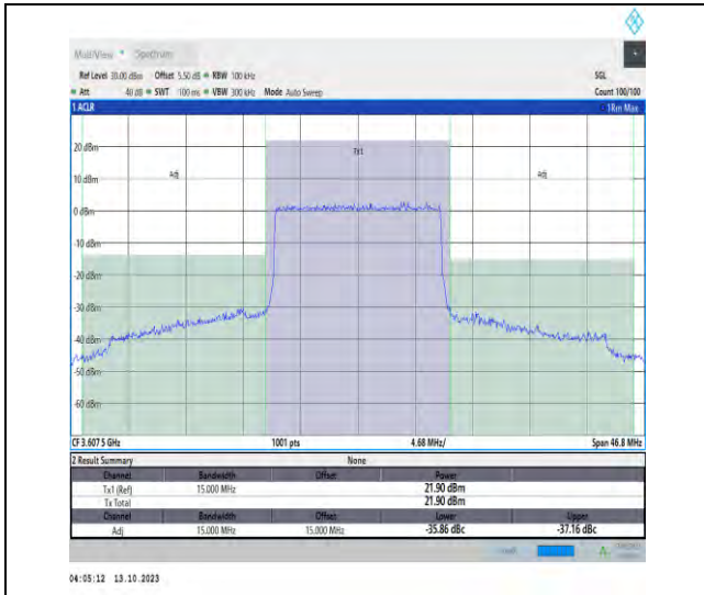
43(3600-3700)-15MHz-QPSK-43665-75RB#0-PASS
