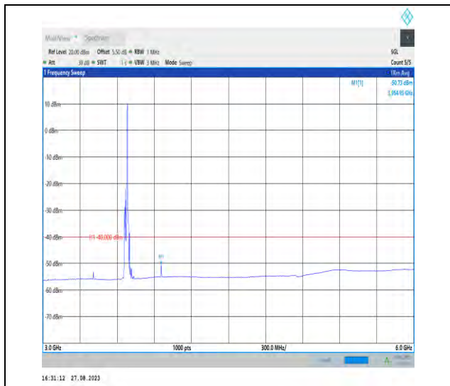
Band43_20MHz_QPSK_44490_1RB#0_3000~6000_30 00~6000
