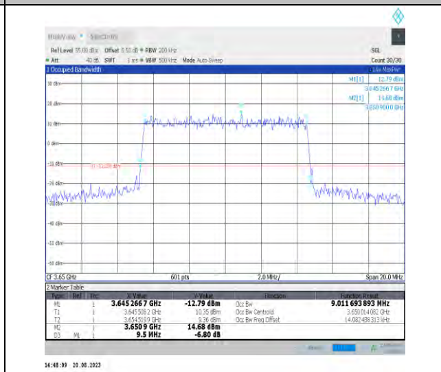
Band43-10MHz-16QAM-44090-50RB#0-PASS
