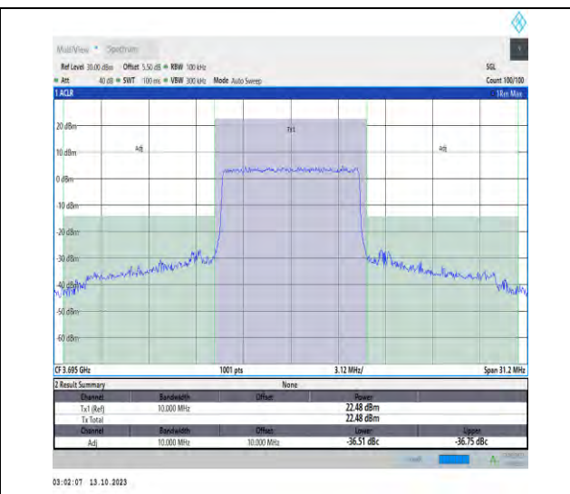
43(3600-3700)-10MHz-QPSK-44540-50RB#0-PASS
