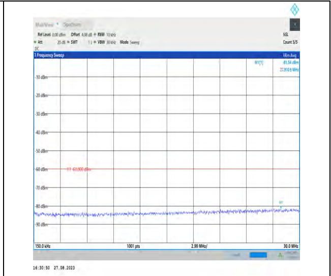
Band43_20MHz_QPSK_44490_1RB#0_0.15~30_0.15~30
