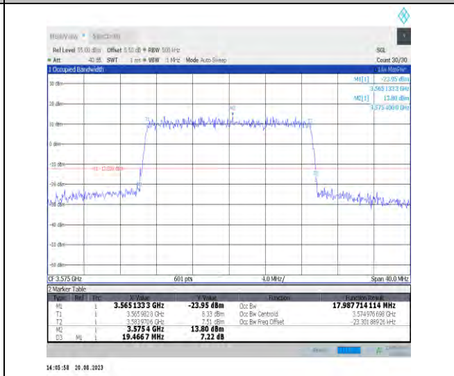
Band42-20MHz-16QAM-43340-100RB#0-PASS
