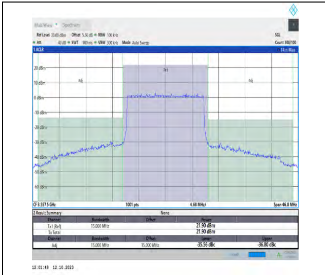
42(3550-3600)-15MHz-QPSK-43165-75RB#0-PASS
