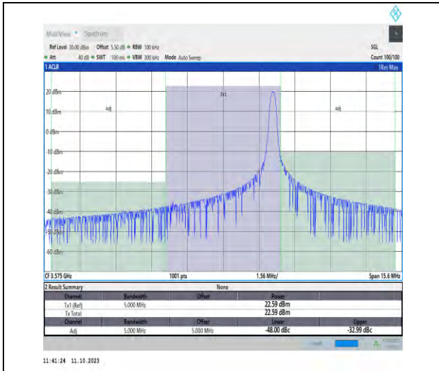
42(3550-3600)-5MHz-QPSK-43340-1RB#24-PASS
