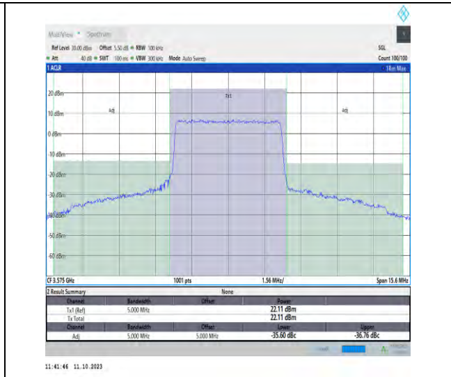
42(3550-3600)-5MHz-QPSK-43340-25RB#0-PASS
