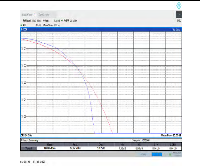
Band42-20MHz-16QAM-43190-100RB#0-PASS
