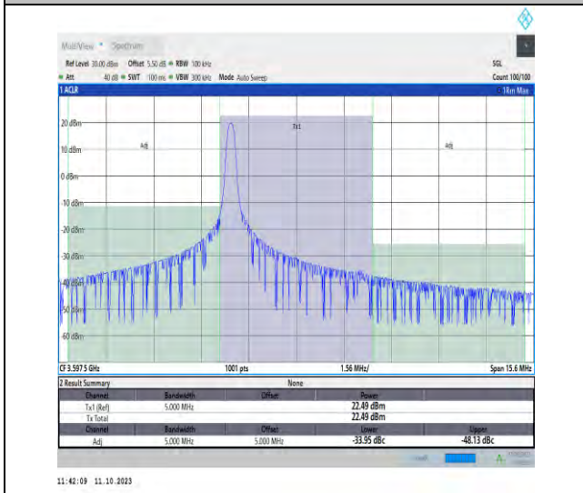
42(3550-3600)-5MHz-QPSK-43565-1RB#0-PASS
