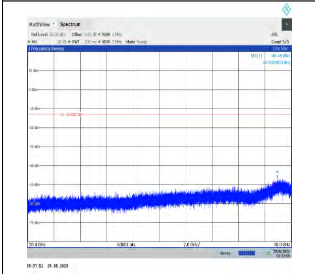
Band42_20MHz_QPSK_43490_1RB#0_20000~40000_20000~40000
