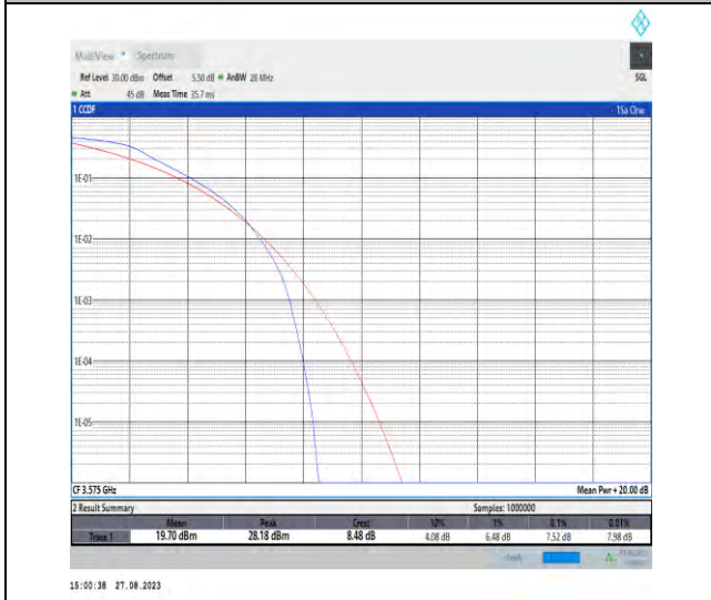
Band42-20MHz-QPSK-43340-100RB#0-PASS
