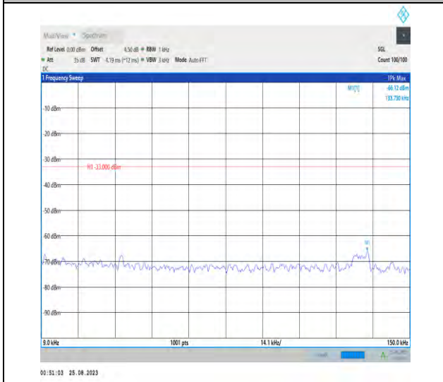
Band42_20MHz_QPSK_43490_1RB#0_0.009~0.15_09~0.15
