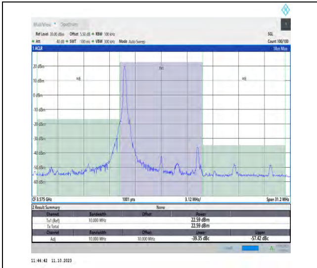
42(3550-3600)-10MHz-QPSK-43340-1RB#0-PASS
