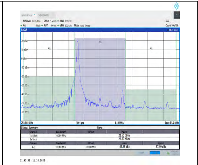
42(3550-3600)-10MHz-QPSK-43140-1RB#0-PASS
