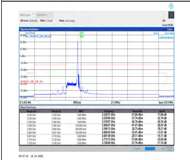
Band42_15MHz_QPSK_43515_1RB#74
