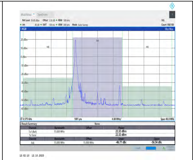
42(3550-3600)-15MHz-QPSK-43340-1RB#0-PASS
