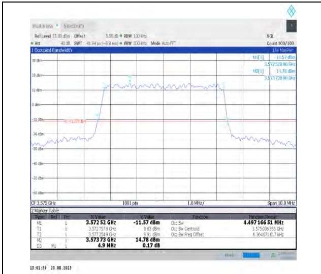
Band42-5MHz-QPSK-43340-25RB#0-PASS
