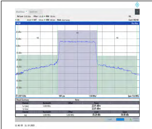
42(3550-3600)-5MHz-QPSK-43565-25RB#0-PASS
