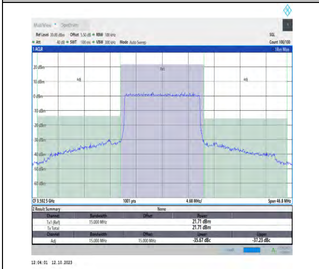
42(3550-3600)-15MHz-QPSK-43515-75RB#0-PASS
