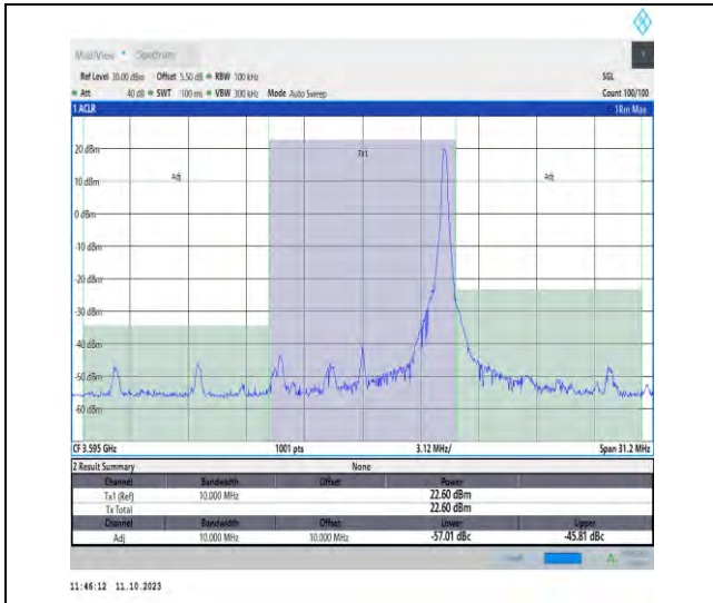
42(3550-3600)-10MHz-QPSK-43540-1RB#49-PASS
