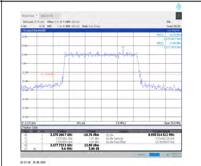
Band42-10MHz-16QAM-43340-50RB#0-PASS
