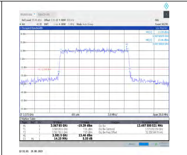
Band42-15MHz-16QAM-43340-75RB#0-PASS
