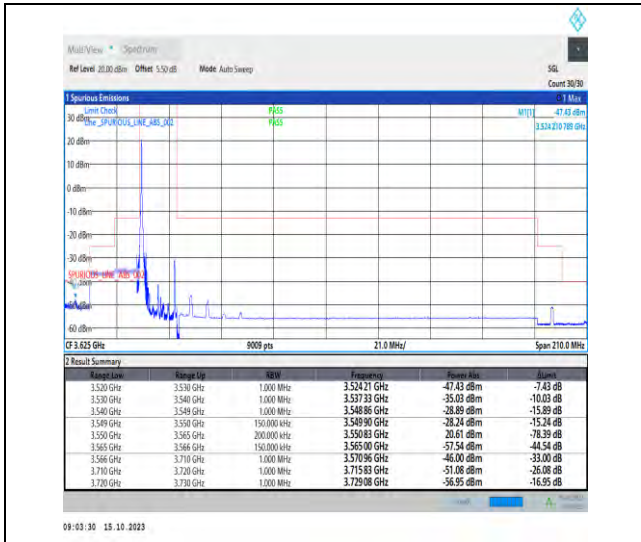
Band42_15MHz_QPSK_43165_1RB#0
