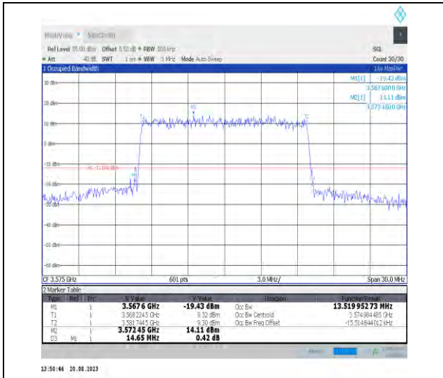
Band42-15MHz-QPSK-43340-75RB#0-PASS
