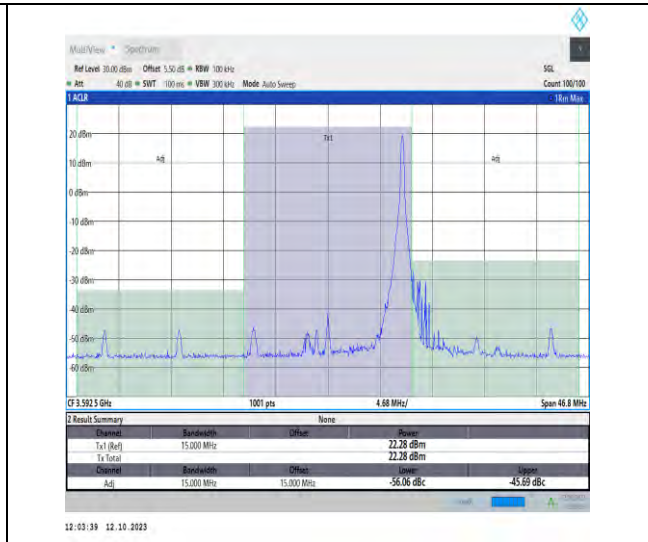
42(3550-3600)-15MHz-QPSK-43515-1RB#74-PASS
