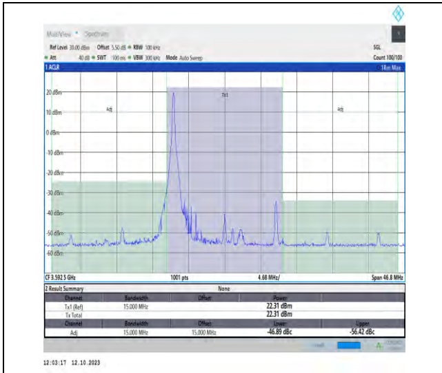
42(3550-3600)-15MHz-QPSK-43515-1RB#0-PASS
