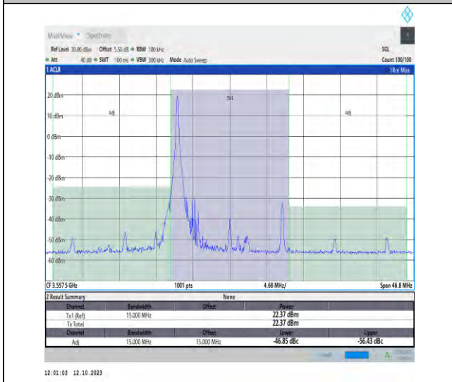
42(3550-3600)-15MHz-QPSK-43165-1RB#0-PASS
