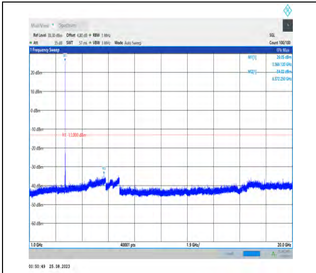
Band42_20MHz_QPSK_43340_1RB#0_1000~20000_1000~20000
