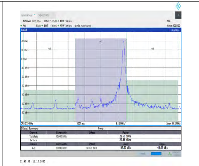
42(3550-3600)-10MHz-QPSK-43340-1RB#49-PASS
