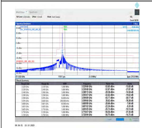
Band42_5MHz_QPSK_43565_1RB#24
