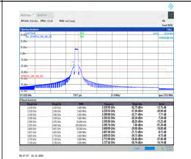
Band42_5MHz_QPSK_43565_25RB#0
