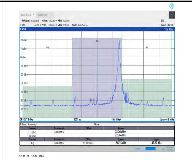
42(3550-3600)-15MHz-QPSK-43165-1RB#74-PASS
