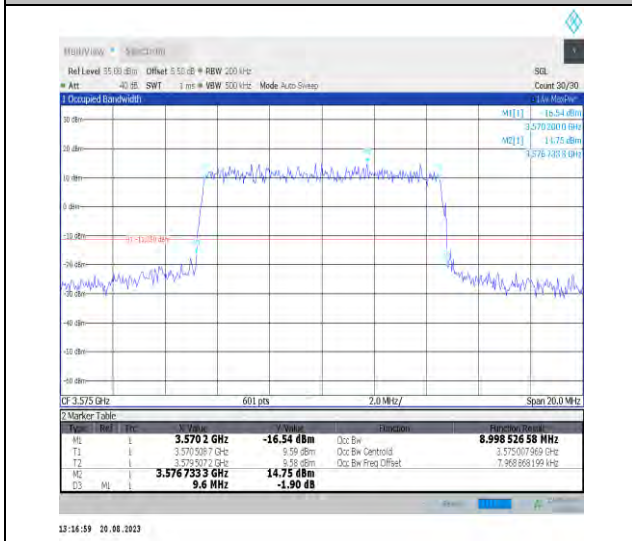
Band42-10MHz-QPSK-43340-50RB#0-PASS
