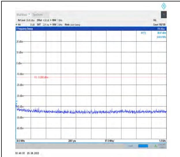
Band42_20MHz_QPSK_43490_1RB#0_30~1000_30~1000
