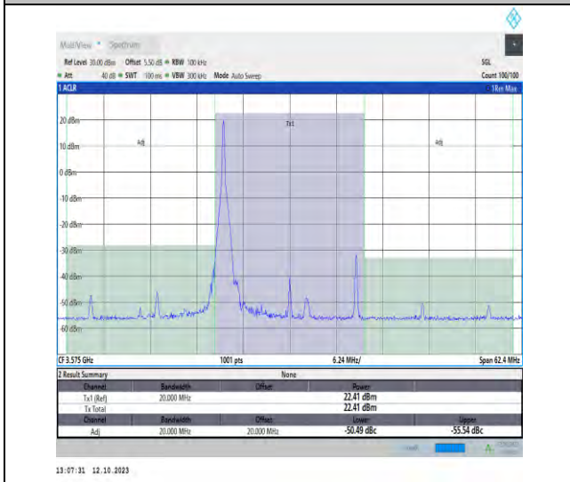
42(3550-3600)-20MHz-QPSK-43340-1RB#0-PASS
