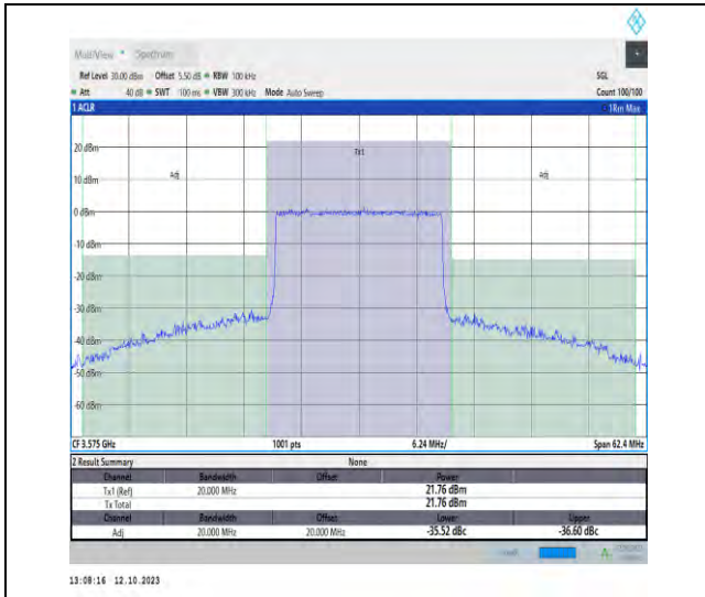
42(3550-3600)-20MHz-QPSK-43340-100RB#0-PASS
