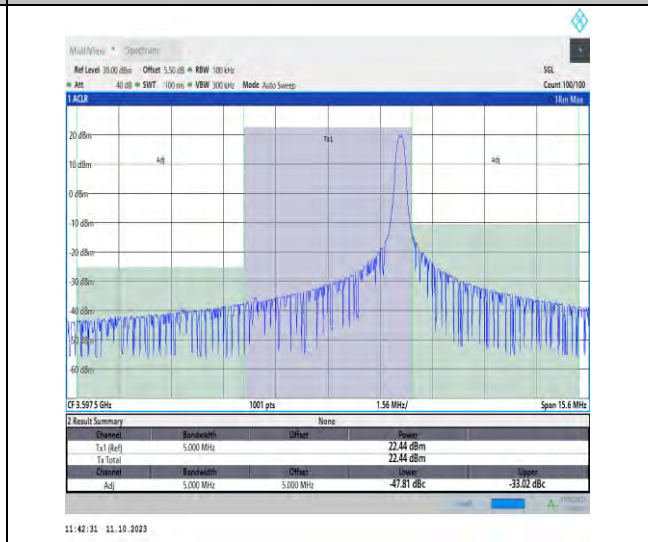
42(3550-3600)-5MHz-QPSK-43565-1RB#24-PASS
