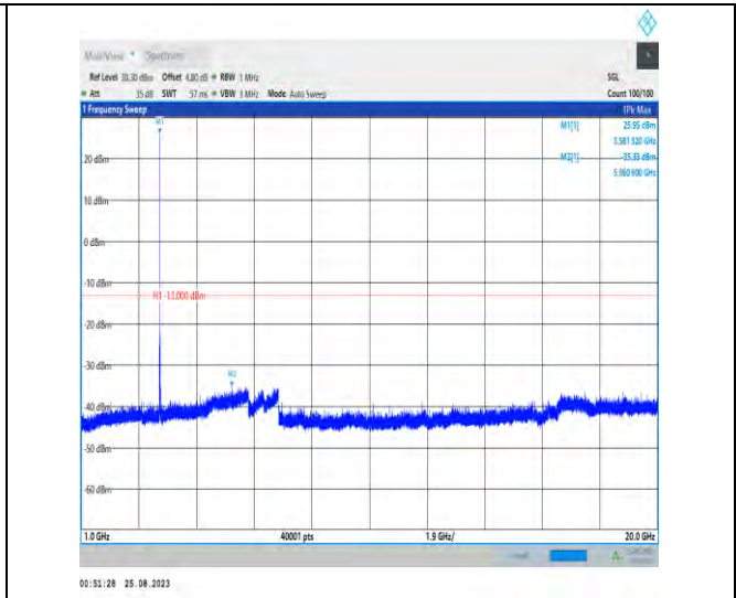
Band42_20MHz_QPSK_43490_1RB#0_1000~20000_1000~20000
