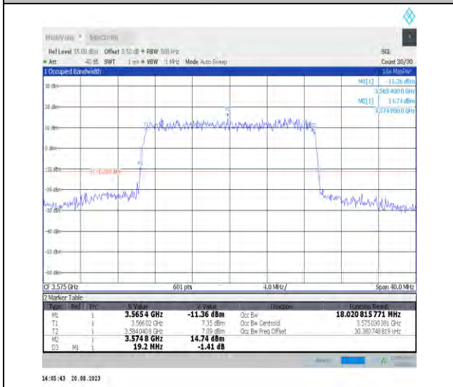
Band42-20MHz-QPSK-43340-100RB#0-PASS
