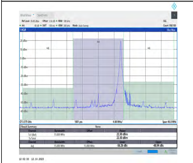
42(3550-3600)-15MHz-QPSK-43340-1RB#74-PASS
