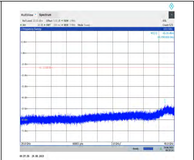
Band42_20MHz_QPSK_43340_1RB#0_20000~40000_20000~40000
