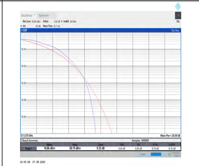
Band42-20MHz-16QAM-43340-100RB#0-PASS
