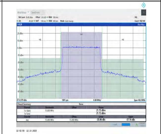
42(3550-3600)-15MHz-QPSK-43340-75RB#0-PASS
