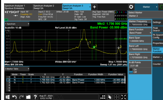
High Channel Band Edge_1 RB
