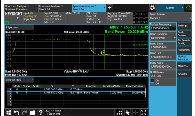
High Channel Band Edge_Full RB
