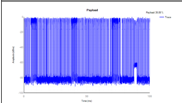
Bandwidth 80MHz
