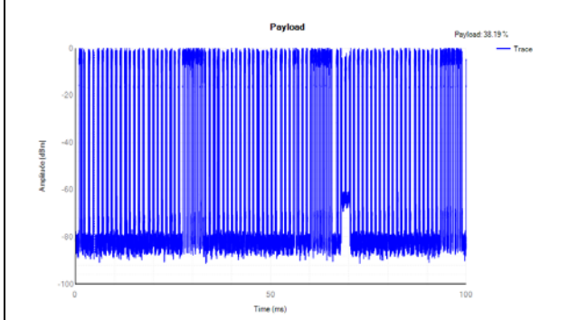
Bandwidth 40MHz
