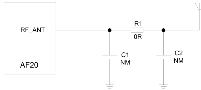
Figure 11: Reference Circuit for RF Antenna Interface
