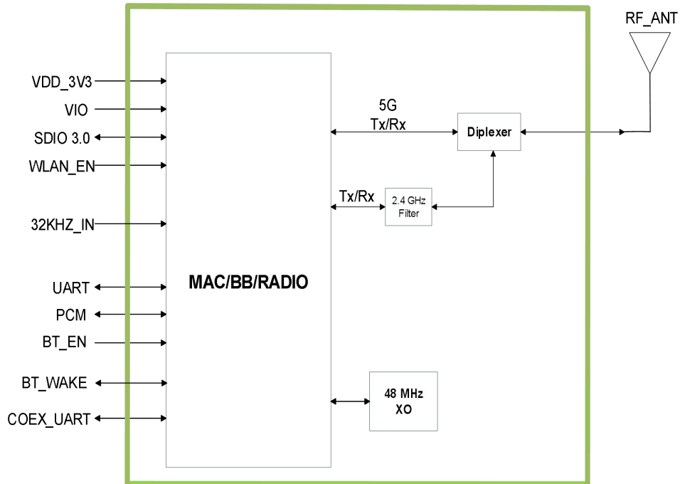
Figure 1: Functional Diagram
