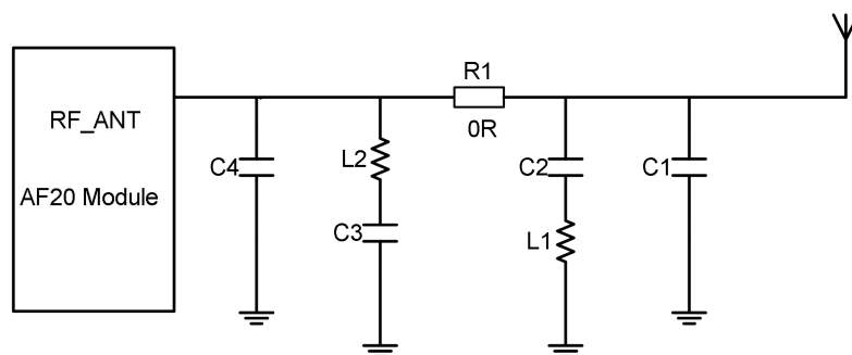
Figure 12: Reference Design of RF Antenna Interface (Vehicle Applications)
