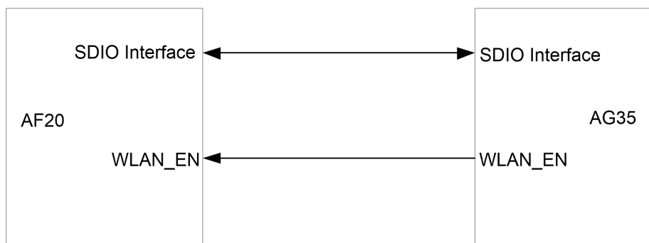
Figure 5: Wi-Fi Application Interface Connection
