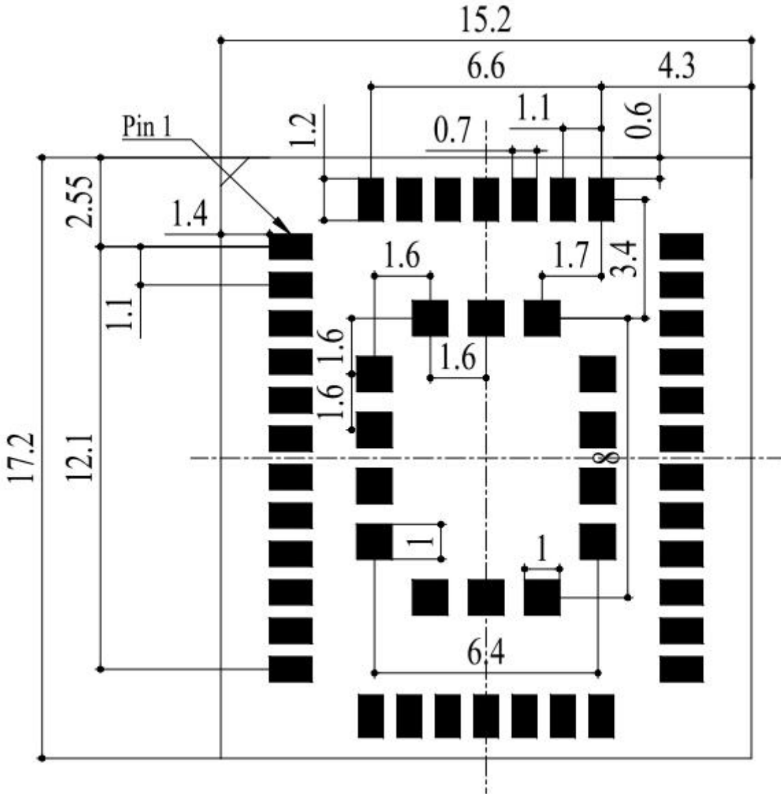
Figure 22: Recommended Footprint
