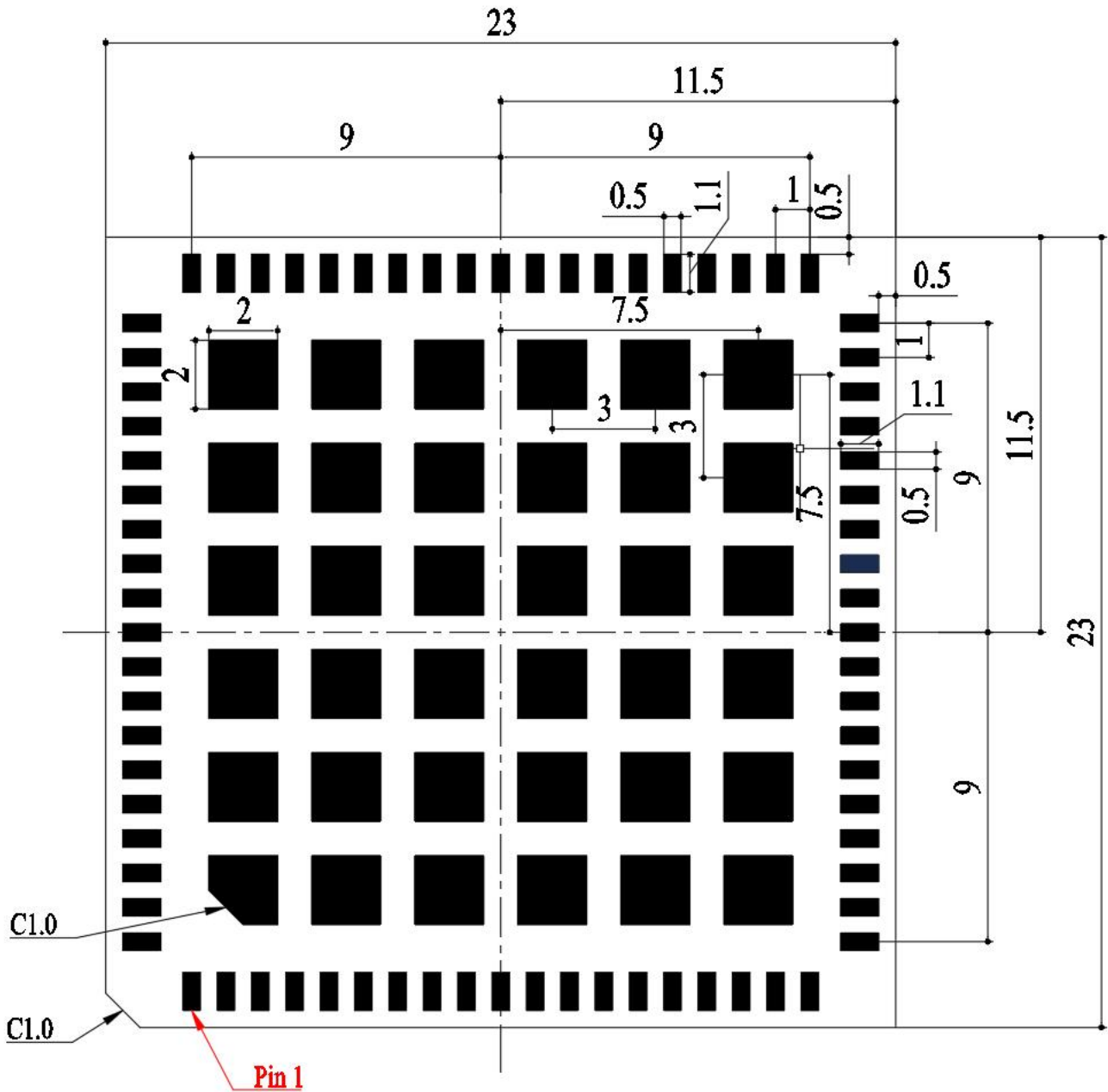
Figure 24: Recommended Footprint
