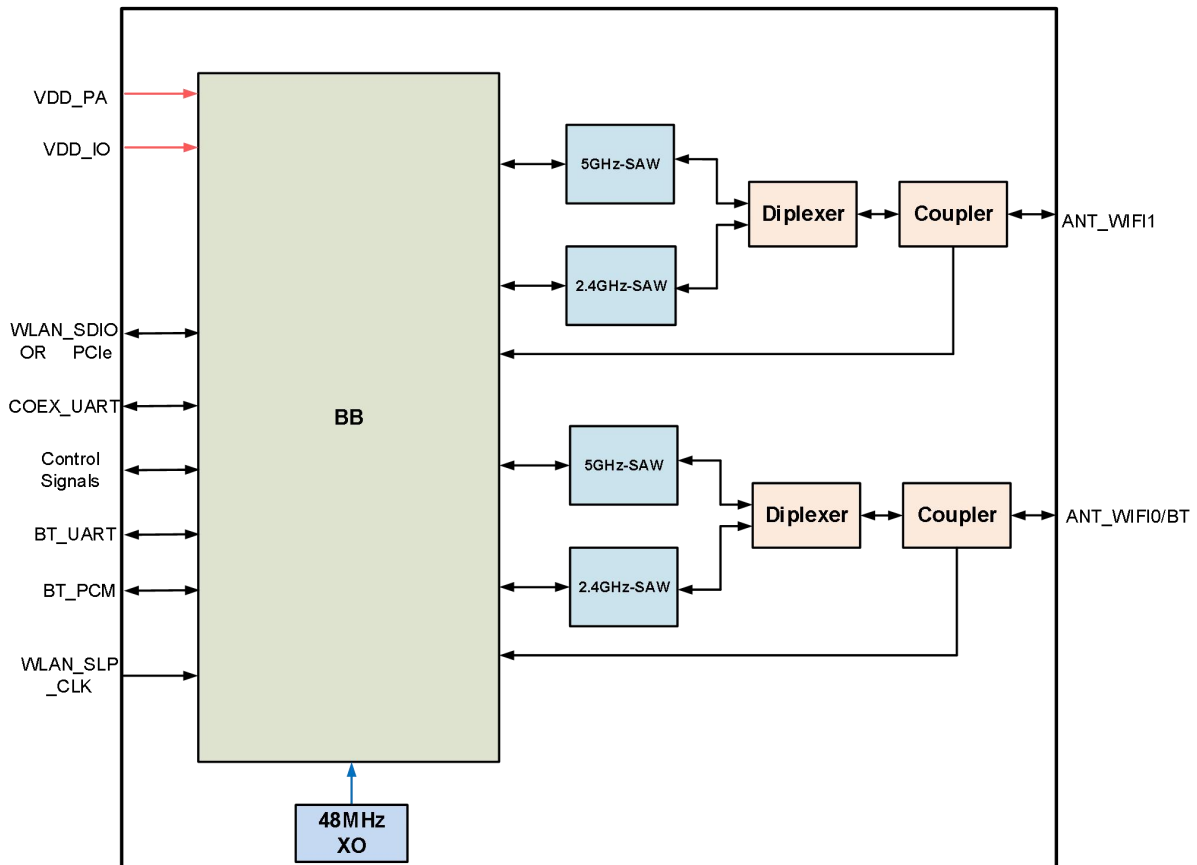
Figure 1: Functional Diagram
