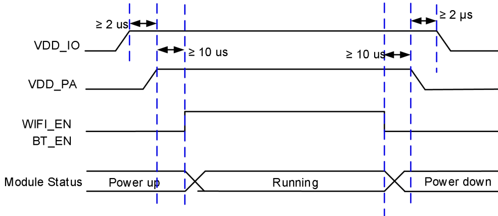
Figure 5: Power-up Timing
