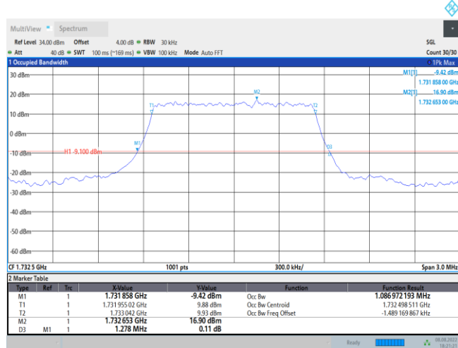
Band4-1.4MHz-QPSK-20175-6RB#0
