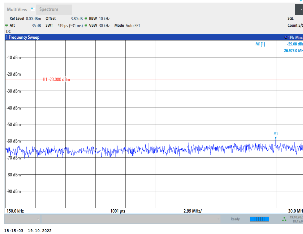
Band26-15MHz-QPSK-26865-1RB#0-Range2:0.15~30MHz
