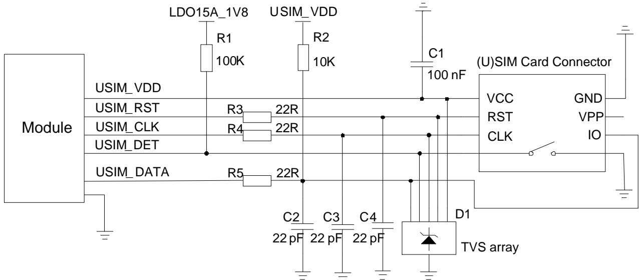
Figure 15: Reference Circuit for (U)SIM Interface with an 8-pin (U)SIM Card Connector
