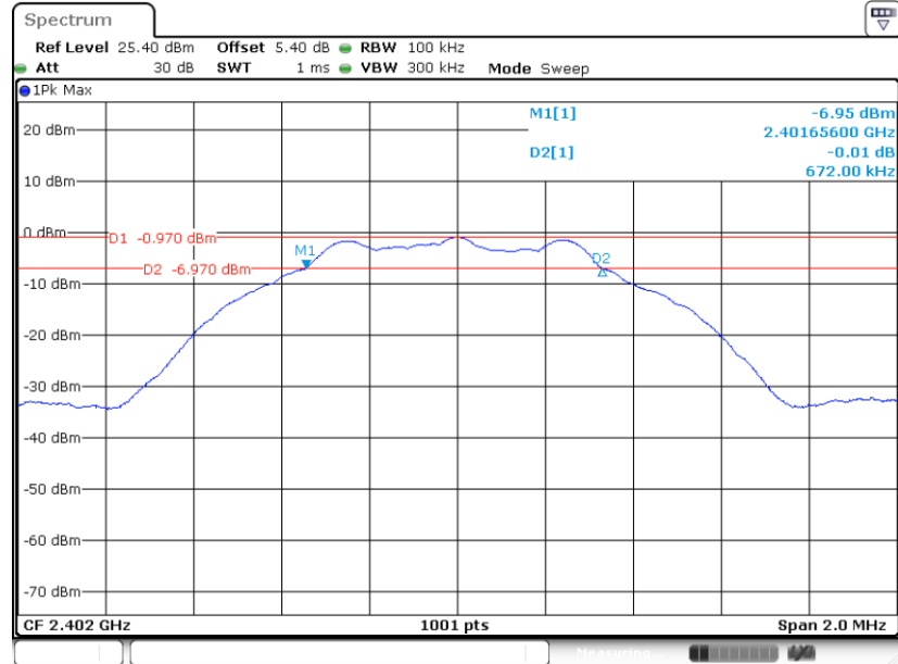
6 dB Bandwidth Plot on Channel 00
