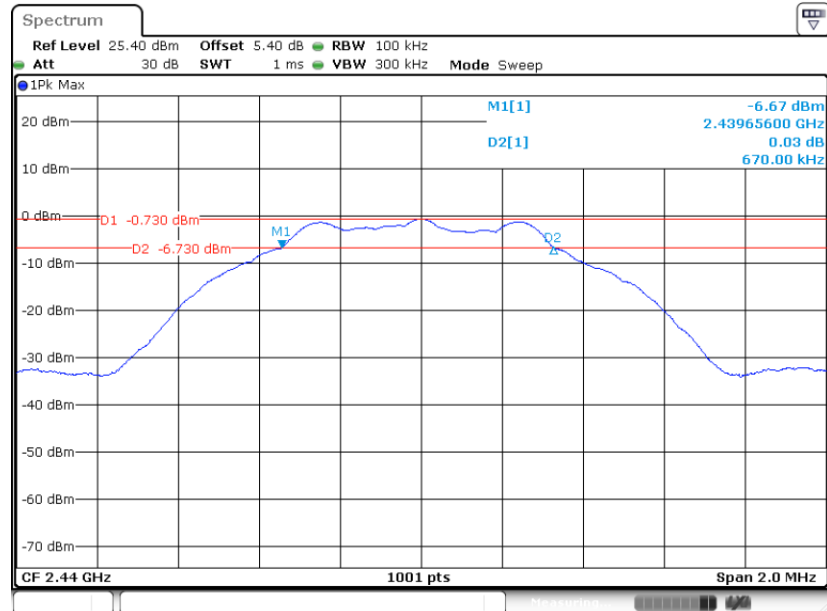
6 dB Bandwidth Plot on Channel 19
