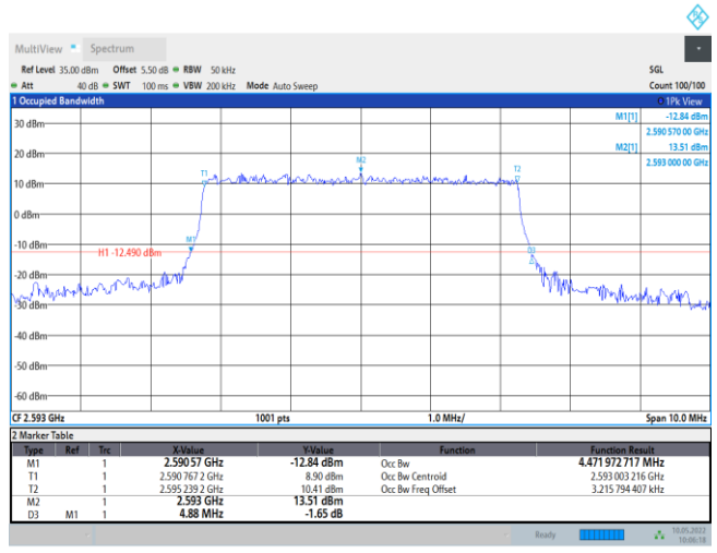
Band41-5MHz-QPSK-40620-25RB#0
