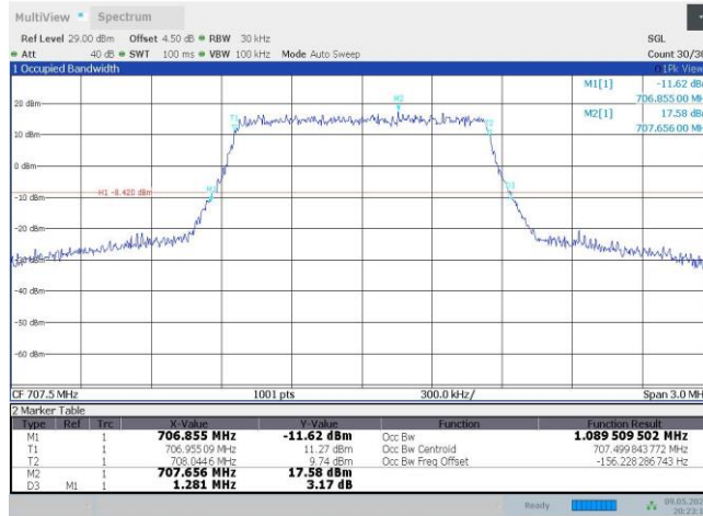
Band12-1.4MHz-QPSK-23095-6RB#0
