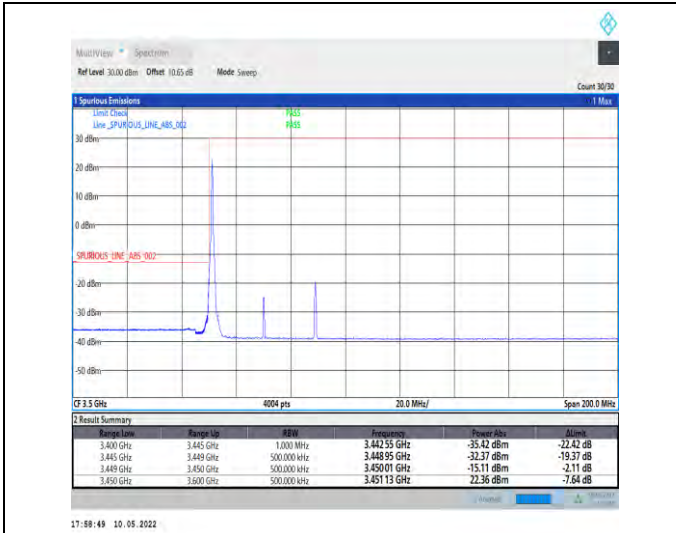
1-N78-3450-3550-PC2-30-40-L-4-CP-QPSK-Edge_1R B_Left-1@0-Ant1-PASS-see graph
