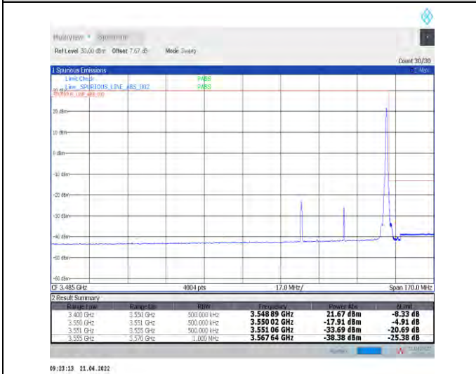
1-N78-3450-3550--30-40-H-5-CP-QPSK-Edge_1RB_R ight-1@105-Ant1-PASS-see graph
