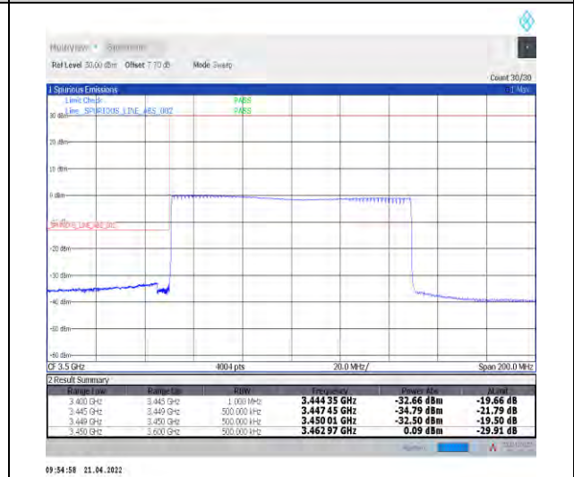
1-N78-3450-3550--30-100-L-6-CP-QPSK-Outer_F ull-273@0-Ant1-PASS-see graph
