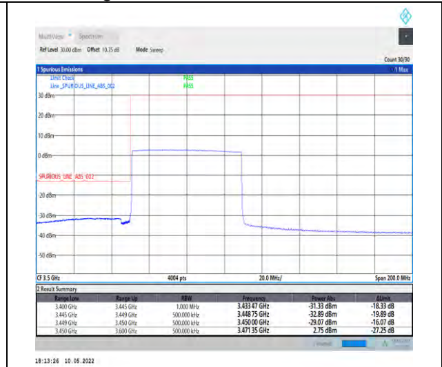
1-N78-3450-3550-PC2-30-60-L-6-CP-QPSK-Outer _Full-162@0-Ant1-PASS-see graph
