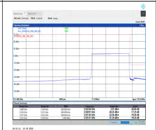
1-N78-3450-3550-PC2-30-50-H-6-CP-QPSK-Outer _Full-133@0-Ant1-PASS-see graph
