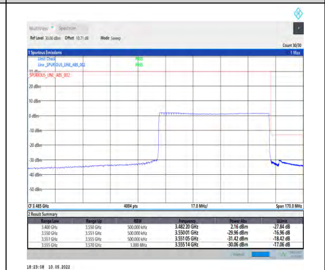
1-N78-3450-3550-PC2-30-70-H-6-CP-QPSK-Outer _Full-189@0-Ant1-PASS-see graph
