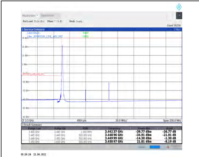
1-N78-3450-3550--30-60-L-1-DFT-PI2BPSK-Edge_1R_B_Left-1@0-Ant1-PASS-see graph
