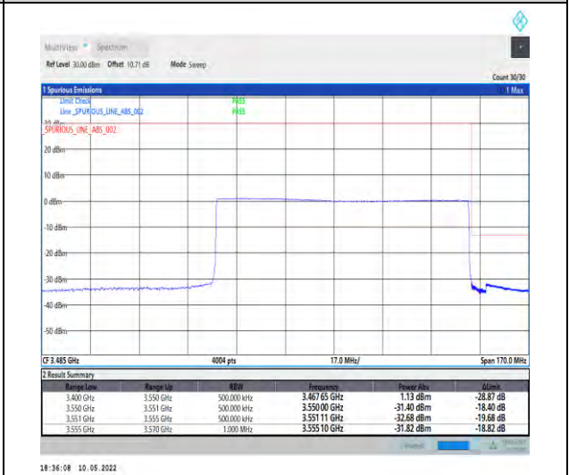
1-N78-3450-3550-PC2-30-90-H-6-CP-QPSK-Outer _Full-245@0-Ant1-PASS-see graph
