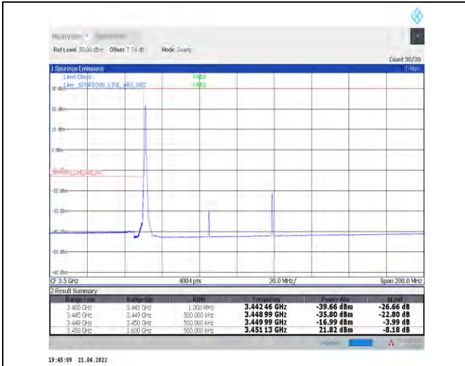
1-N78-3450-3550--30-70-L-1-DFT-PI2BPSK-Edge_1R_B_Left-1@0-Ant1-PASS-see graph
