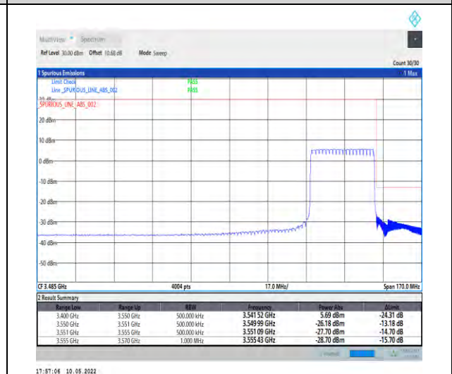
1-N78-3450-3550-PC2-30-30-H-6-CP-QPSK-Outer _Full-78@0-Ant1-PASS-see graph
