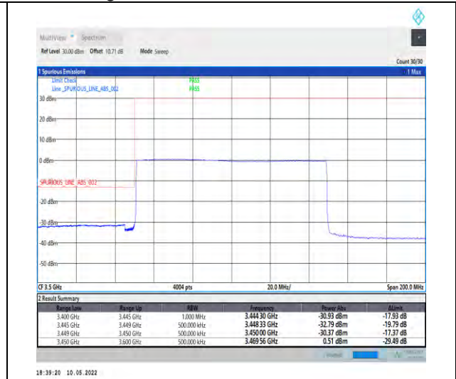
1-N78-3450-3550-PC2-30-100-L-6-CP-QPSK-Out er_Full-273@0-Ant1-PASS-see graph
