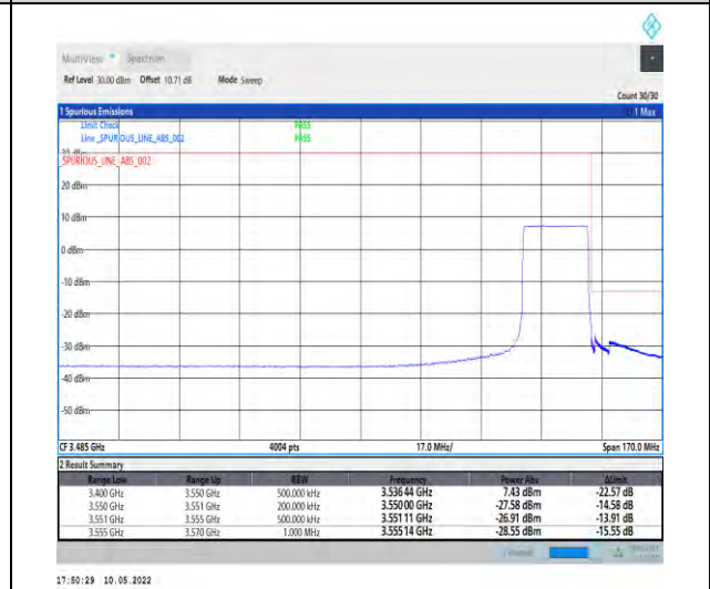
1-N78-3450-3550-PC2-30-20-H-6-CP-QPSK-Outer _Full-51@0-Ant1-PASS-see graph
