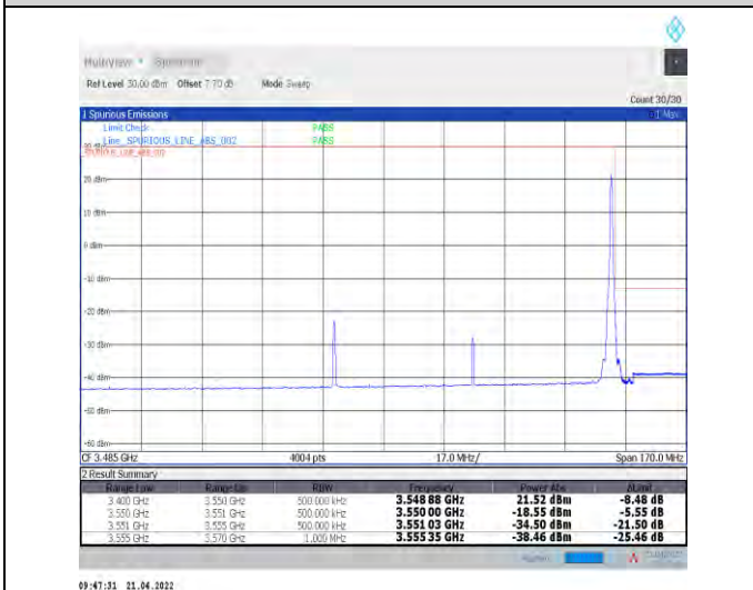
1-N78-3450-3550--30-80-H-5-CP-QPSK-Edge_1RB_Right-1@216-Ant1-PASS-see graph
