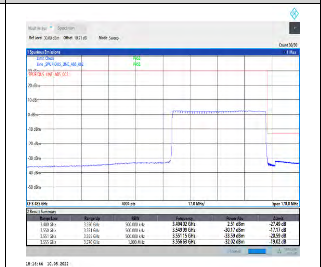
1-N78-3450-3550-PC2-30-60-H-6-CP-QPSK-Outer _Full-162@0-Ant1-PASS-see graph
