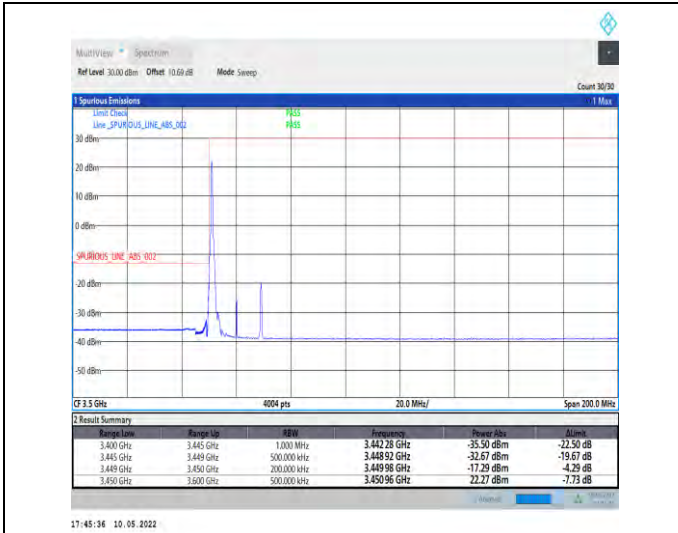
1-N78-3450-3550-PC2-30-20-L-4-CP-QPSK-Edge_1R B_Left-1@0-Ant1-PASS-see graph
