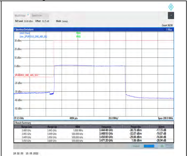
1-N78-3450-3550-PC2-30-90-L-6-CP-QPSK-Outer _Full-245@0-Ant1-PASS-see graph
