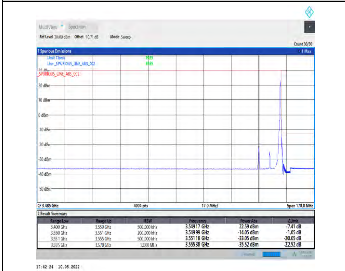
1-N78-3450-3550-PC2-30-15-H-5-CP-QPSK-Edge_1R_B_Right-1@37-Ant1-PASS-see graph
