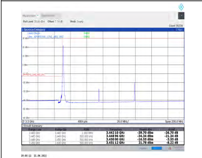
1-N78-3450-3550--30-90-L-4-CP-QPSK-Edge_1RB_L_eff-1@0-Ant1-PASS-see graph
