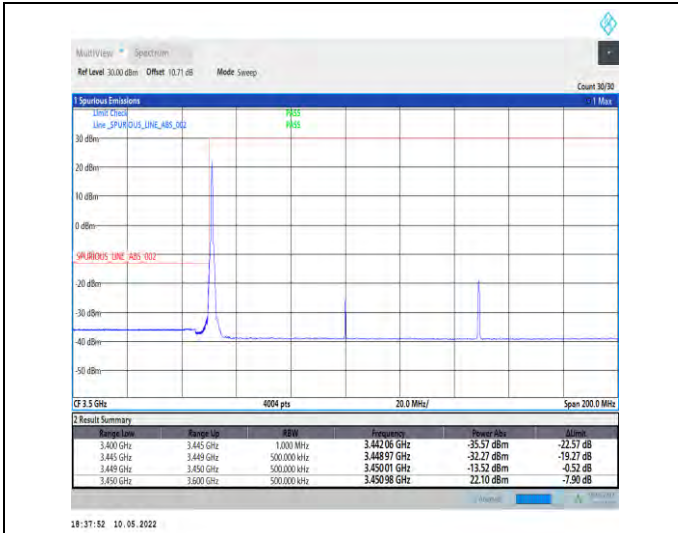
1-N78-3450-3550-PC2-30-100-L-4-CP-QPSK-Edge_1 RB_Left-1@0-Ant1-PASS-see graph
