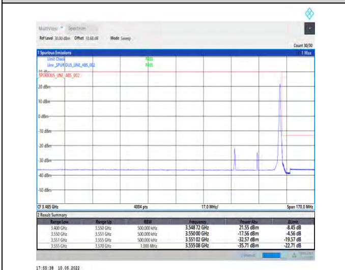
1-N78-3450-3550-PC2-30-30-H-5-CP-QPSK-Edge_1R B_Right-1@77-Ant1-PASS-see graph
