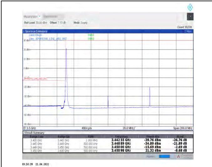
1-N78-3450-3550--30-100-L-1-DFT-PI2BPSK-Edge_1 RB_Left-1@0-Ant1-PASS-see graph
