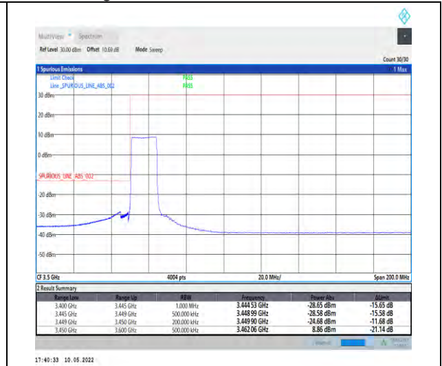
1-N78-3450-3550-PC2-30-15-L-6-CP-QPSK-Outer_Full-38@0-Ant1-PASS-see graph
