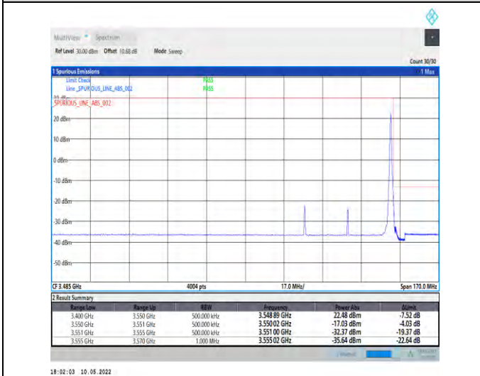
1-N78-3450-3550-PC2-30-40-H-5-CP-QPSK-Edge_1R B_Right-1@105-Ant1-PASS-see graph
