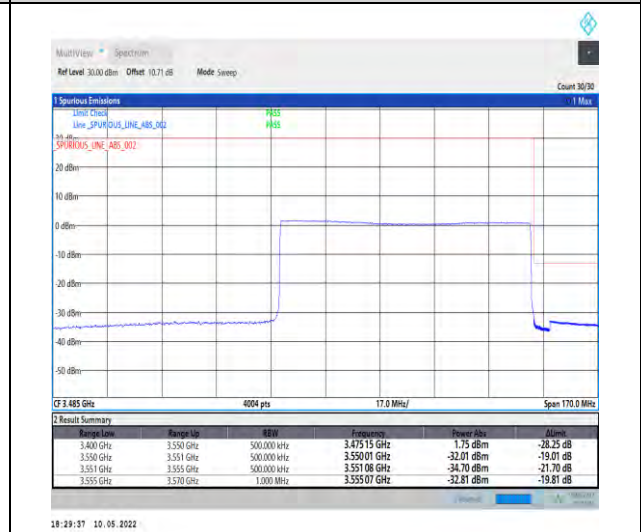
1-N78-3450-3550-PC2-30-80-H-6-CP-QPSK-Outer _Full-217@0-Ant1-PASS-see graph
