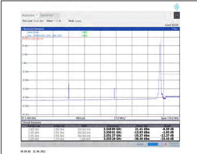
1-N78-3450-3550--30-100-H-2-DFT-PI2BPSK-Edge_1 RB_Right-1@272-Ant1-PASS-see graph
