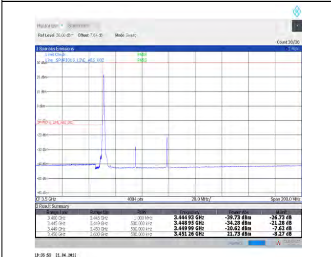
1-N78-3450-3550--30-50-L-4-CP-QPSK-Edge_1RB_L_eff-1@0-Ant1-PASS-see graph
