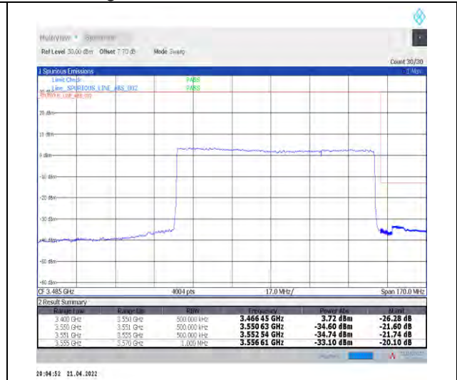
1-N78-3450-3550--30-90-H-3-DFT-PI2BPSK-Outer_Full-240@0-Ant1-PASS-see graph
