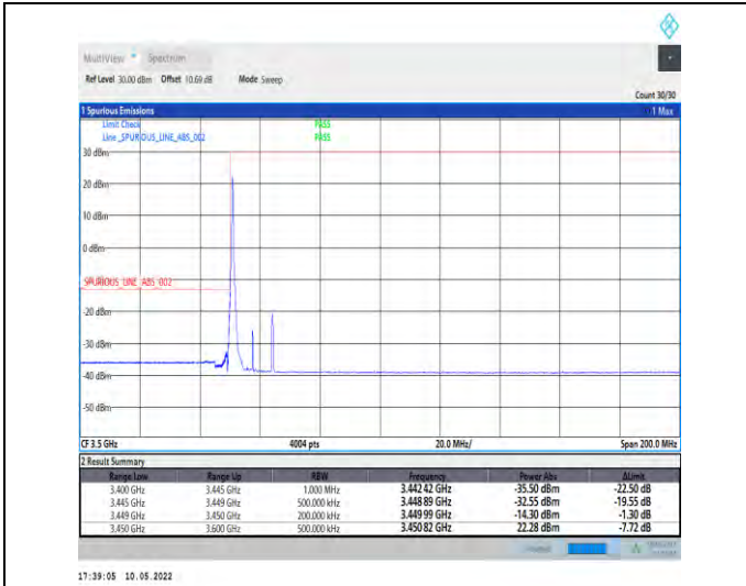
1-N78-3450-3550-PC2-30-15-L-4-CP-QPSK-Edge_1R_B_Left-1@0-Ant1-PASS-see graph
