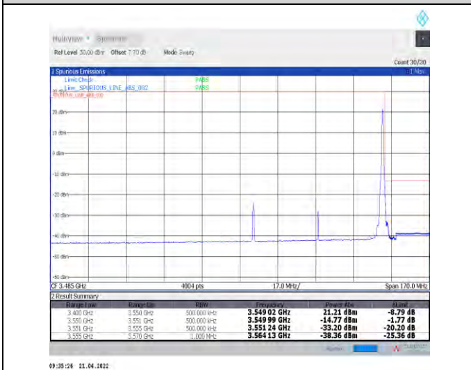
1-N78-3450-3550--30-60-H-5-CP-QPSK-Edge_1RB_R ight-1@161-Ant1-PASS-see graph
