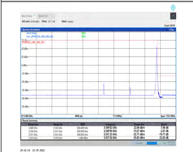
1-N78-3450-3550-PC2-30-60-H-5-CP-QPSK-Edge_1R B_Right-1@161-Ant1-PASS-see graph
