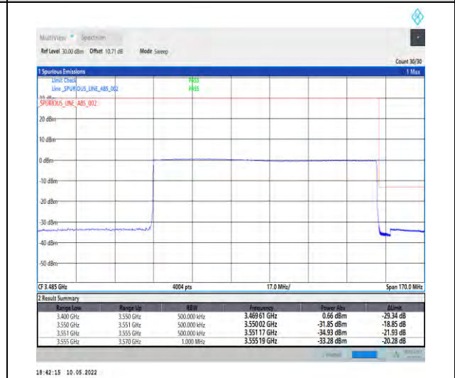
1-N78-3450-3550-PC2-30-100-H-6-CP-QPSK-Out er_Full-273@0-Ant1-PASS-see graph
