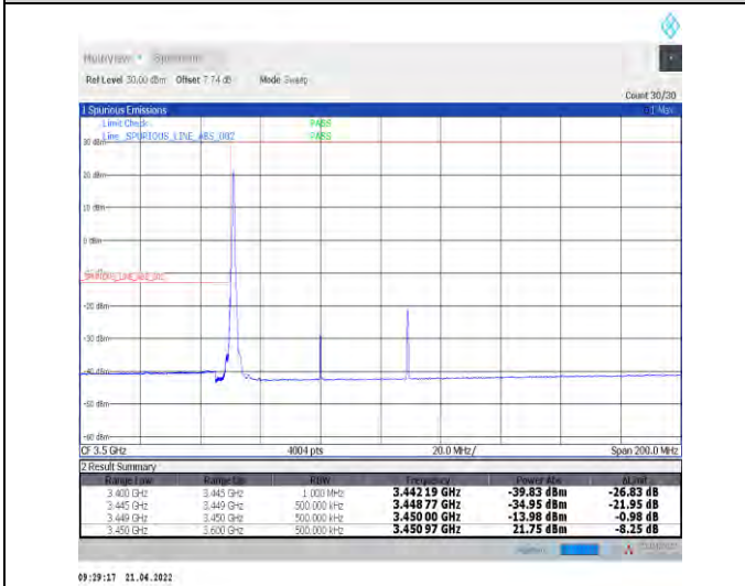
1-N78-3450-3550--30-60-L-4-CP-QPSK-Edge_1RB_L_eff-1@0-Ant1-PASS-see graph
