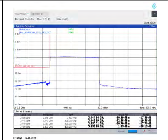
1-N78-3450-3550--30-70-L-6-CP-QPSK-Outer_Ful_I-189@0-Ant1-PASS-see graph
