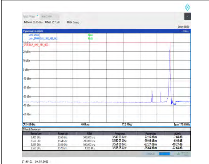
1-N78-3450-3550-PC2-30-20-H-5-CP-QPSK-Edge_1R B_Right-1@50-Ant1-PASS-see graph
