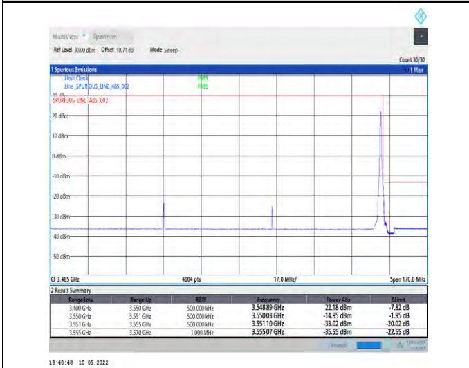
1-N78-3450-3550-PC2-30-100-H-5-CP-QPSK-Edge_1 RB_Right-1@272-Ant1-PASS-see graph
