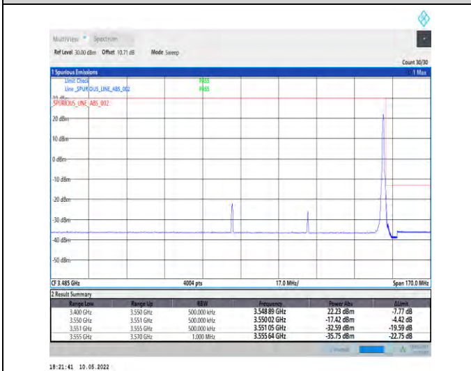
1-N78-3450-3550-PC2-30-70-H-5-CP-QPSK-Edge_1R B_Right-1@188-Ant1-PASS-see graph
