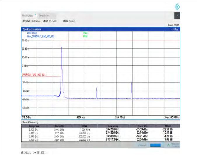
1-N78-3450-3550-PC2-30-90-L-4-CP-QPSK-Edge_1R B_Left-1@0-Ant1-PASS-see graph
