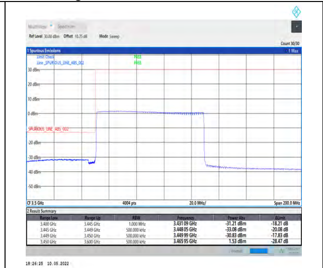
1-N78-3450-3550-PC2-30-80-L-6-CP-QPSK-Outer _Full-217@0-Ant1-PASS-see graph
