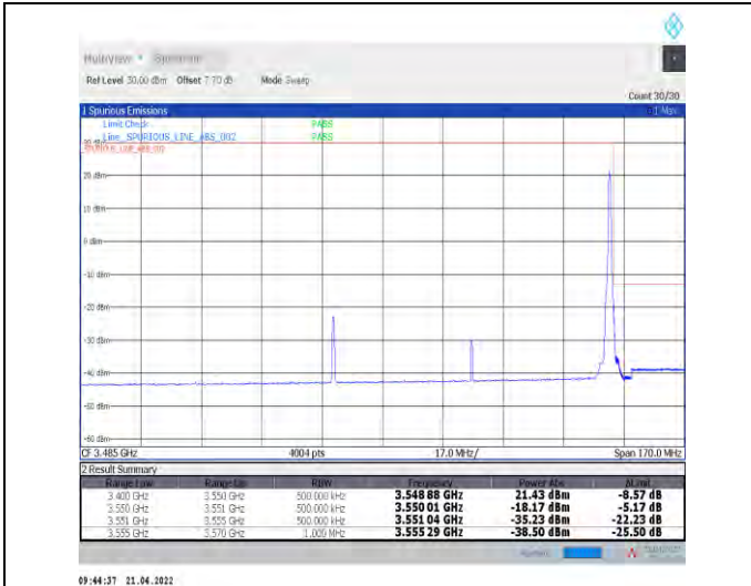
1-N78-3450-3550--30-80-H-2-DFT-PI2BPSK-Edge_1R_B_Right-1@216-Ant1-PASS-see graph
