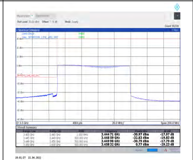
1-N78-3450-3550--30-90-L-6-CP-QPSK-Outer_Ful_I-245@0-Ant1-PASS-see graph
