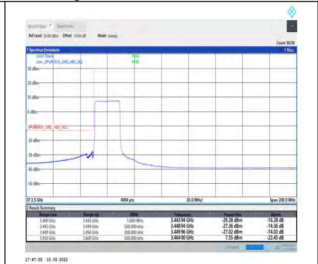
1-N78-3450-3550-PC2-30-20-L-6-CP-QPSK-Outer _Full-51@0-Ant1-PASS-see graph
