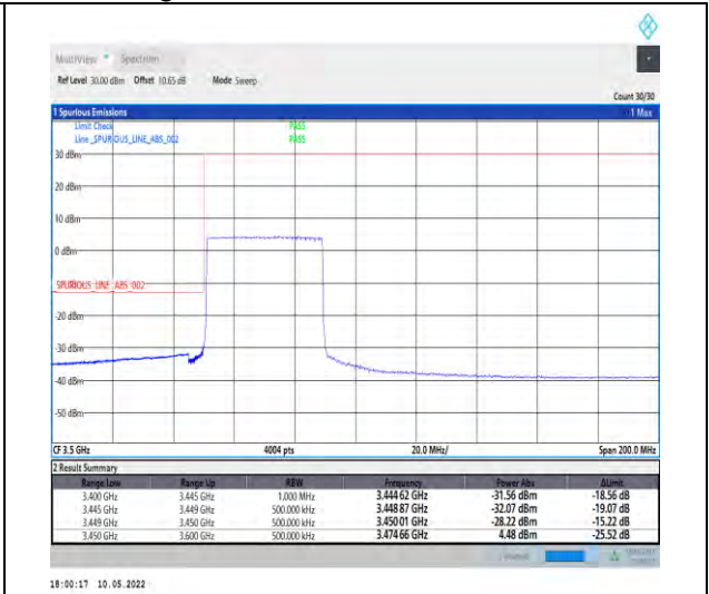
1-N78-3450-3550-PC2-30-40-L-6-CP-QPSK-Outer _Full-106@0-Ant1-PASS-see graph
