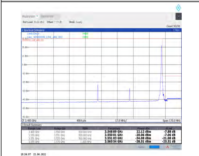
1-N78-3450-3550--30-70-H-5-CP-QPSK-Edge_1RB_R ight-1@188-Ant1-PASS-see graph
