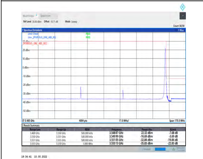
1-N78-3450-3550-PC2-30-90-H-5-CP-QPSK-Edge_1R B_Right-1@244-Ant1-PASS-see graph
