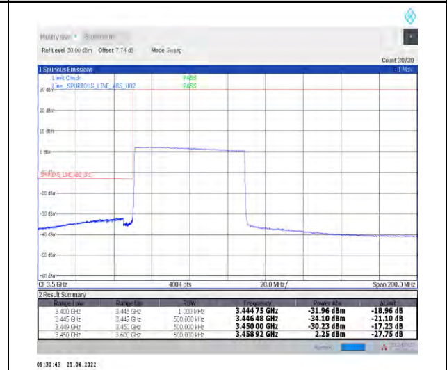
1-N78-3450-3550--30-60-L-6-CP-QPSK-Outer_Ful I-162@0-Ant1-PASS-see graph
