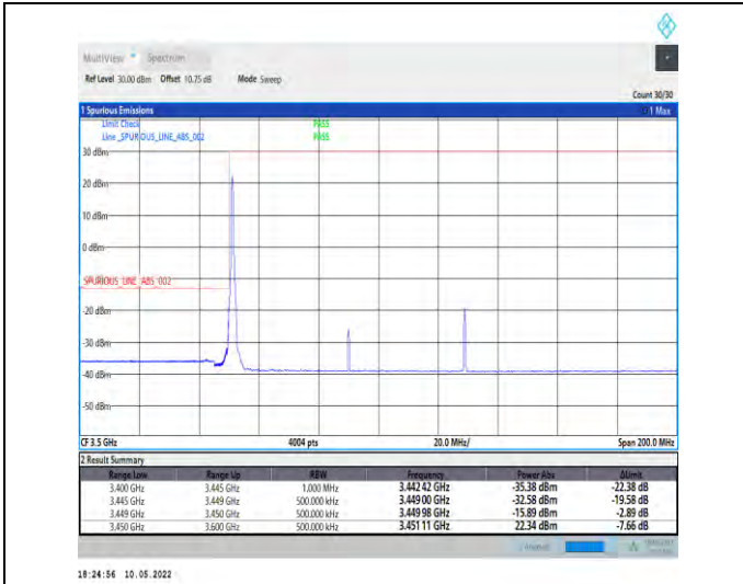
1-N78-3450-3550-PC2-30-80-L-4-CP-QPSK-Edge_1R B_Left-1@0-Ant1-PASS-see graph
