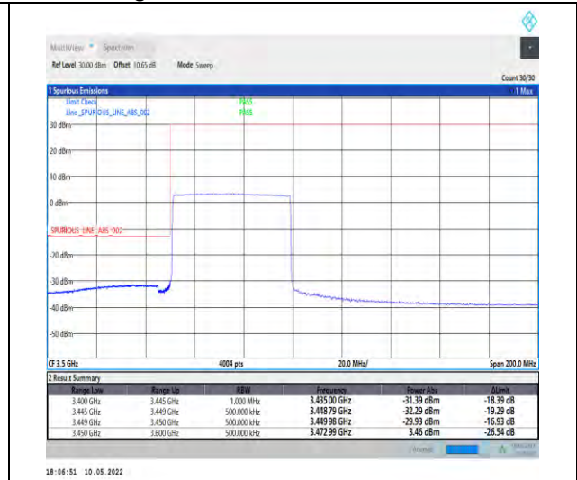
1-N78-3450-3550-PC2-30-50-L-6-CP-QPSK-Outer _Full-133@0-Ant1-PASS-see graph
