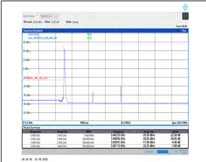
1-N78-3450-3550-PC2-30-70-L-4-CP-QPSK-Edge_1R B_Left-1@0-Ant1-PASS-see graph
