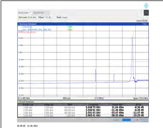
1-N78-3450-3550--30-50-H-2-DFT-PI2BPSK-Edge_1R_B_Right-1@132-Ant1-PASS-see graph
