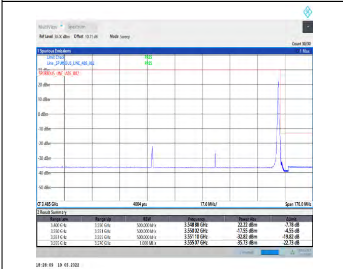
1-N78-3450-3550-PC2-30-80-H-5-CP-QPSK-Edge_1R B_Right-1@216-Ant1-PASS-see graph
