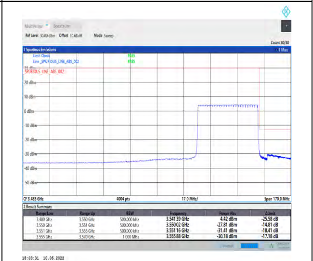
1-N78-3450-3550-PC2-30-40-H-6-CP-QPSK-Outer _Full-106@0-Ant1-PASS-see graph
