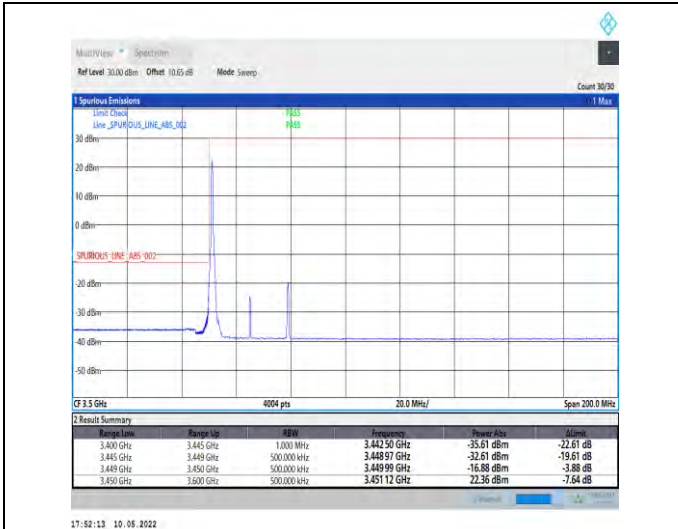
1-N78-3450-3550-PC2-30-30-L-4-CP-QPSK-Edge_1R B_Left-1@0-Ant1-PASS-see graph
