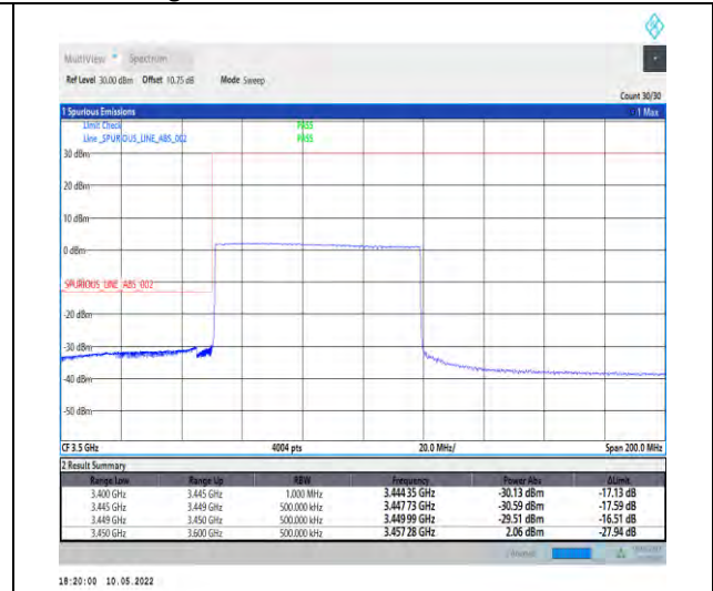
1-N78-3450-3550-PC2-30-70-L-6-CP-QPSK-Outer _Full-189@0-Ant1-PASS-see graph
