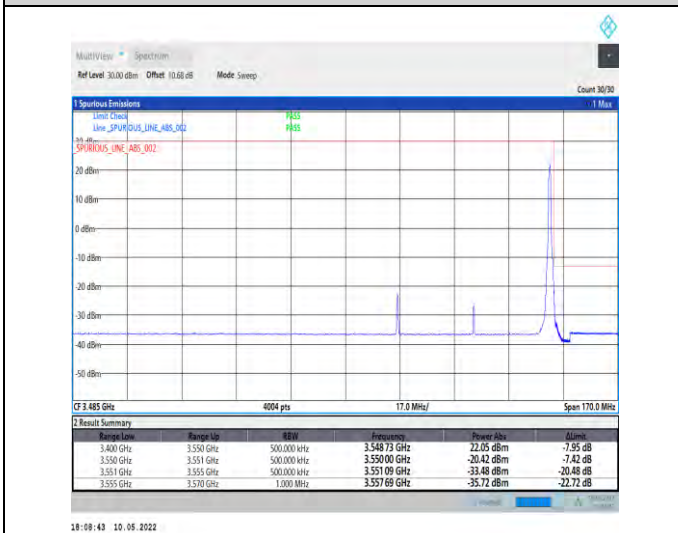
1-N78-3450-3550-PC2-30-50-H-5-CP-QPSK-Edge_1R B_Right-1@132-Ant1-PASS-see graph
