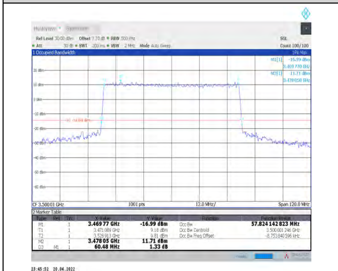
1-N78-3450-3550--30-60-M-8-CP-64QAM-Outer_Full-162@0-Ant1-57.824-60.480-<math>\leq 60</math>-PASS
