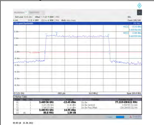
1-N78-3450-3550--30-80-H-4-DFT-64QAM-Outer_Fu II-216@0-Ant1-77.219-80.800-<math>\leq 80</math>-PASS
