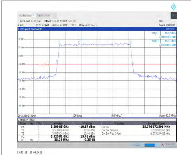
1-N78-3450-3550--30-40-H-3-DFT-16QAM-Outer_Fu II-100@0-Ant1-35.747-38.080-≤40-PASS
