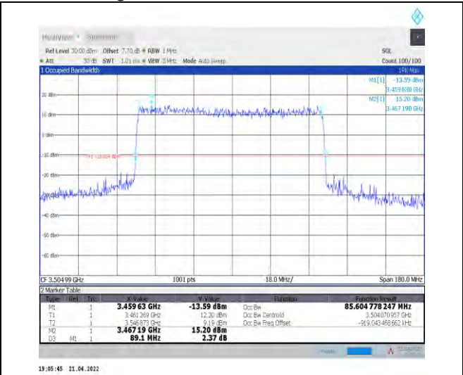
1-N78-3450-3550--30-90-H-1-DFT-QPSK-Outer_Full-240@0-Ant1-85.605-89.100-<=90-PASS
