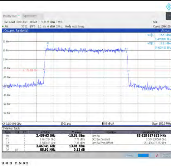
1-N78-3450-3550--30-90-H-4-DFT-64QAM-Outer_Fu II-240@0-Ant1-85.629-88.920-≤90-PASS
