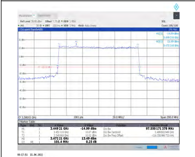
1-N78-3450-3550--30-100-M-8-CP-64QAM-Outer_Full ull-273@0-Ant1-97.55-101.400-≤100-PASS
