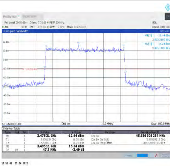
1-N78-3450-3550--30-50-M-1-DFT-QPSK-Outer_Full -128@0-Ant1-45.936-47.700-≤50-PASS
