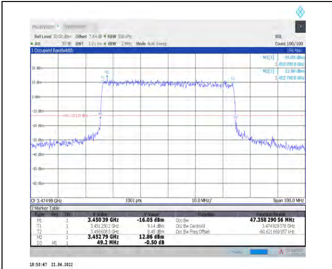
1-N78-3450-3550--30-50-L-6-CP-QPSK-Outer_Full-1 33@0-Ant1-47.358-49.200-≤50-PASS
