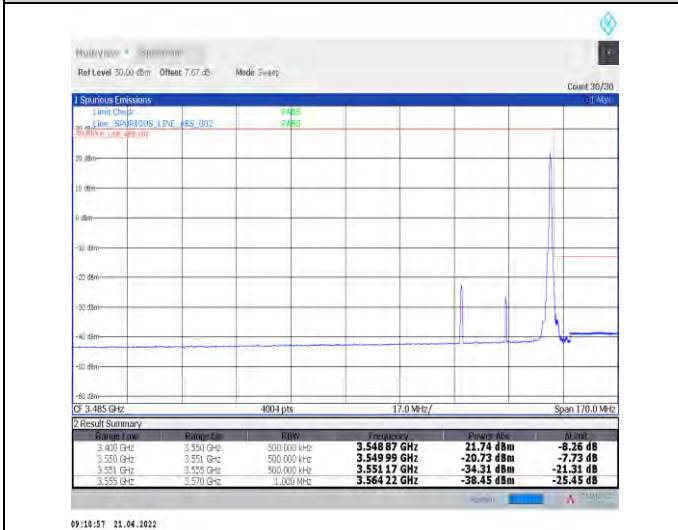
1-N78-3450-3550--30-30-H-5-CP-QPSK-Edge_1RB_R ight-1@77-Ant1-PASS-see graph
