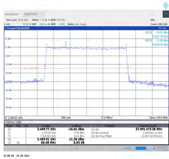
1-N78-3450-3550--30-60-M-5-DFT-256QAM-Outer_F Full-162@0-Ant1-57.991-60.480-≤60-PASS
