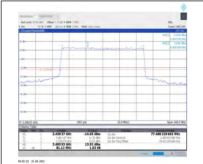
1-N78-3450-3550--30-80-M-8-CP-64QAM-Outer_Full -217@0-Ant1-77.486-81.120-≤80-PASS
