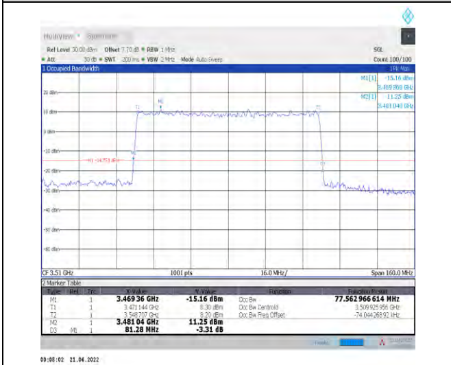
1-N78-3450-3550--30-80-H-9-CP-256QAM-Outer_Fu ll-217@0-Ant1-77.563-81.280-≤80-PASS
