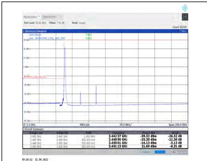
1-N78-3450-3550--30-40-L-1-DFT-PI2BPSK-Edge_1R_B_Left-1@0-Ant1-PASS-see graph
