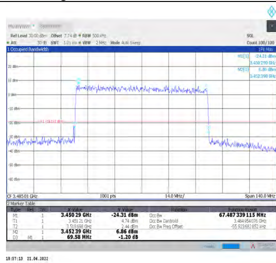
1-N78-3450-3550--30-70-L-9-CP-256QAM-Outer_Fu II-189@0-Ant1-67.487-69.580-≤70-PASS
