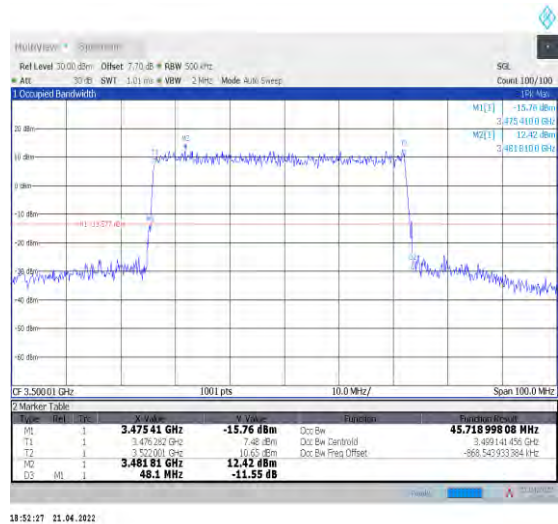
1-N78-3450-3550--30-50-M-4-DFT-64QAM-Outer_Full Full-128@0-Ant1-45.719-48.100-≤50-PASS
