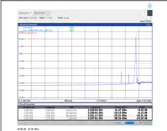
1-N78-3450-3550--30-20-H-5-CP-QPSK-Edge_1RB_R ight-1@50-Ant1-PASS-see graph
