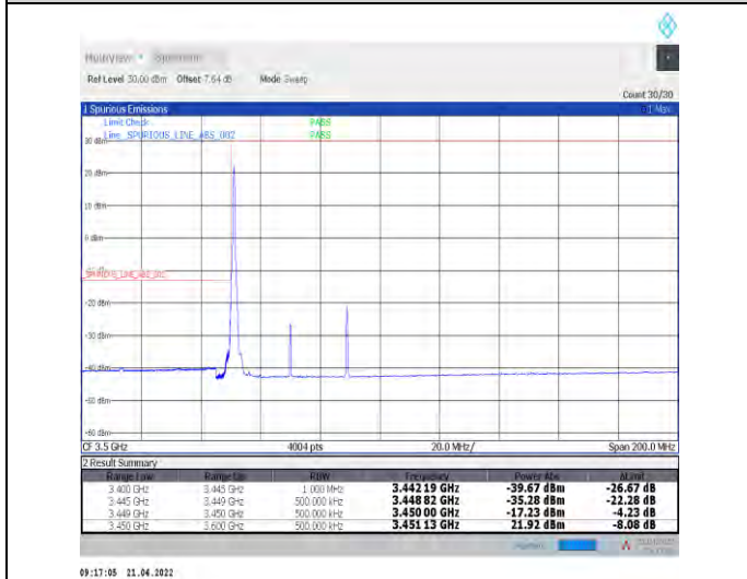
1-N78-3450-3550--30-40-L-4-CP-QPSK-Edge_1RB_L_eff-1@0-Ant1-PASS-see graph
