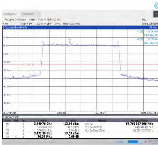
1-N78-3450-3550--30-60-L-6-CP-QPSK-Outer_Full 162@0-Ant1-57.767-60.360-≤60-PASS
