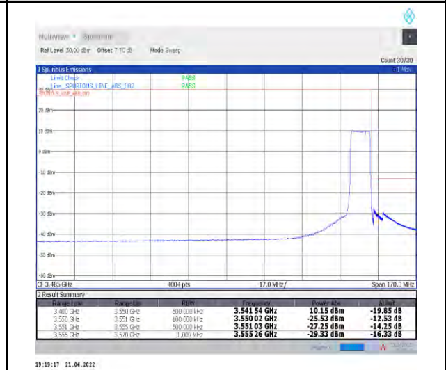
1-N78-3450-3550--30-10-H-6-CP-QPSK-Outer_Fu ll-24@0-Ant1-PASS-see graph
