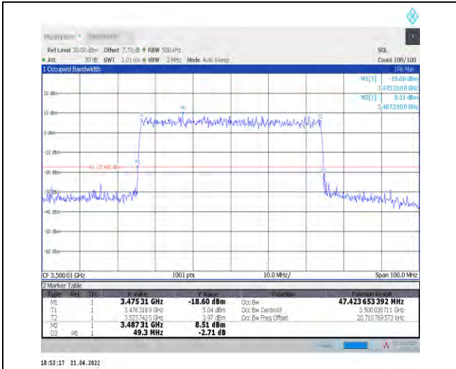
1-N78-3450-3550--30-50-M-9-CP-256QAM-Outer_Full-133@0-Ant1-47.424-49.300-≤50-PASS
