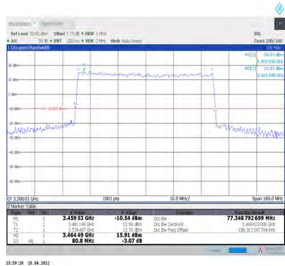
1-N78-3450-3550--30-80-M-3-DFT-16QAM-Outer_Full Full-216@0-Ant1-77.349-80.800-≤80-PASS
