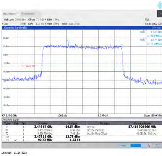
1-N78-3450-3550--30-90-L-8-CP-64QAM-Outer_Full -245@0-Ant1-87.42-90.720-<=90-PASS
