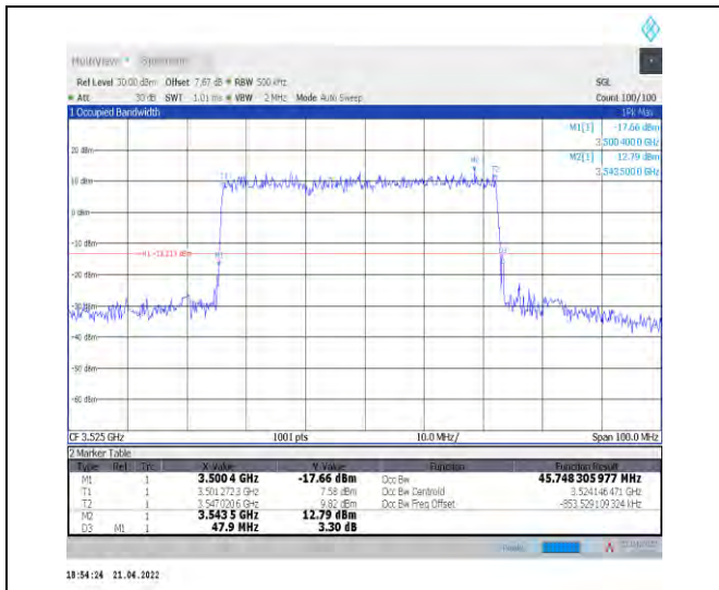
1-N78-3450-3550--30-50-H-4-DFT-64QAM-Outer_Fu II-128@0-Ant1-45.748-47.900-≤50-PASS
