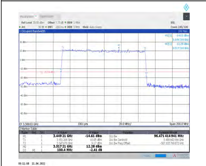
1-N78-3450-3550--30-100-L-5-DFT-256QAM-Outer_F ull-270@0-Ant1-96.471-100.400-≤100-PASS
