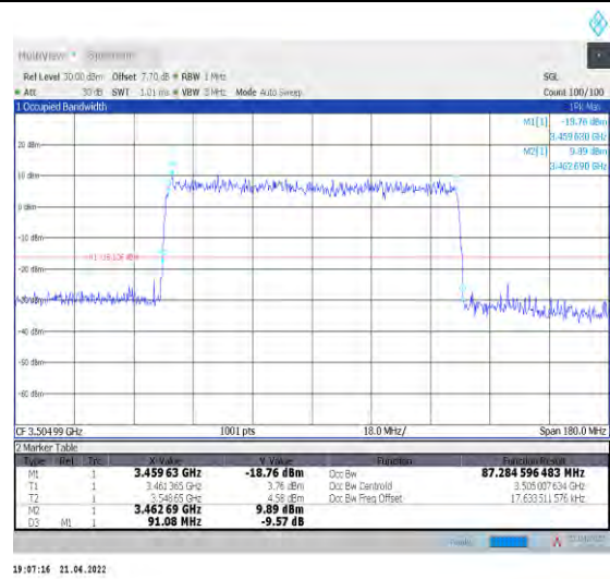
1-N78-3450-3550--30-90-H-9-CP-256QAM-Outer_Full -245@0-Ant1-87.285-91.080-≤90-PASS
