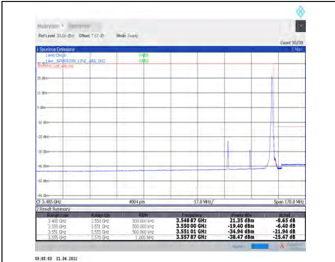
1-N78-3450-3550--30-30-H-2-DFT-PI2BPSK-Edge_1R_B_Right-1@77-Ant1-PASS-see graph
