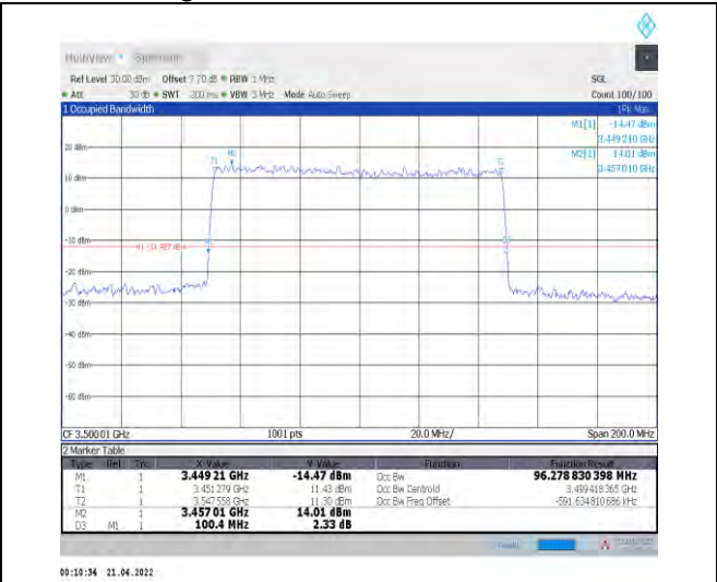
1-N78-3450-3550--30-100-L-4-DFT-64QAM-Outer_F ull-270@0-Ant1-96.279-100.400-≤100-PASS
