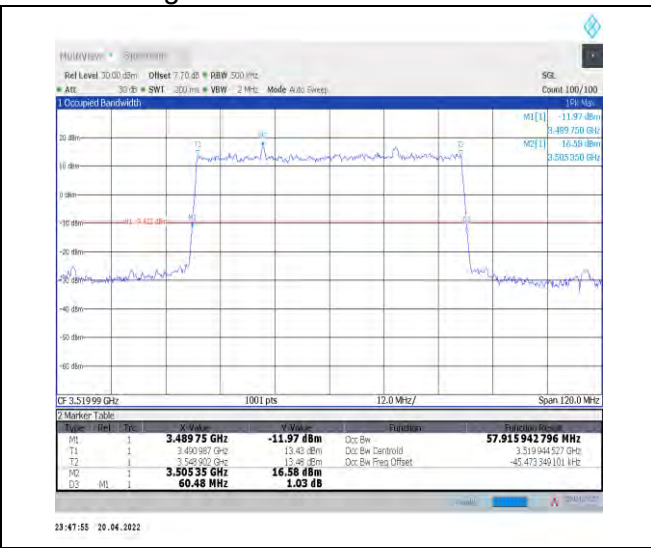
1-N78-3450-3550--30-60-H-2-DFT-PI2BPSK-Outer_Full Full-162@0-Ant1-57.916-60.480-≤60-PASS
