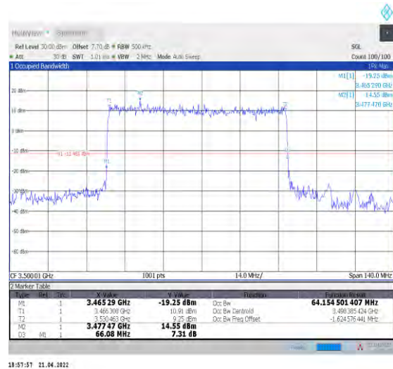
1-N78-3450-3550--30-70-M-2-DFT-PI2BPSK-Outer_Full Full-180@0-Ant1-64.155-66.080-≤70-PASS
