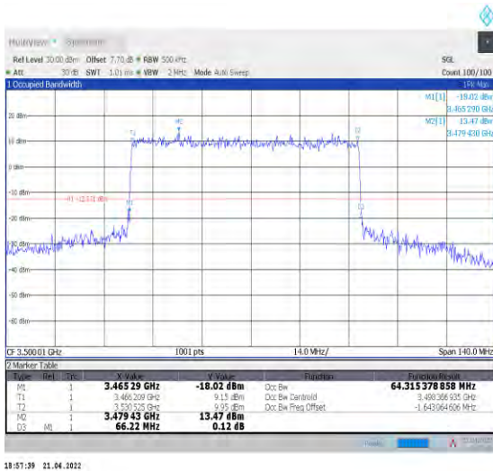
1-N78-3450-3550--30-70-M-1-DFT-QPSK-Outer_Full -180@0-Ant1-64.315-66.220-≤70-PASS
