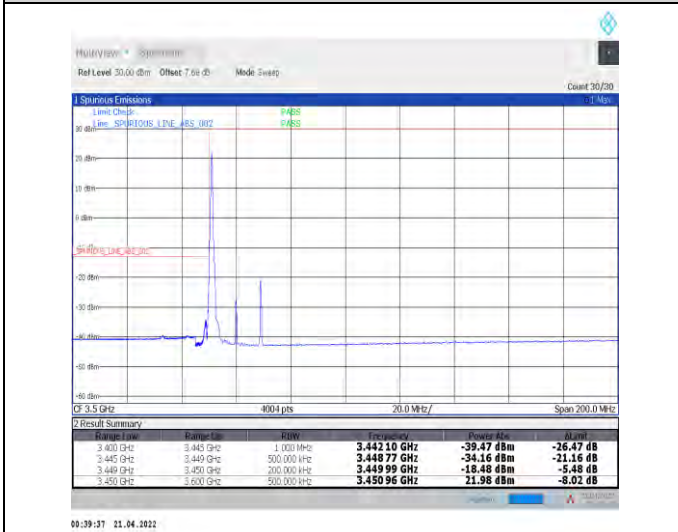
1-N78-3450-3550--30-20-L-4-CP-QPSK-Edge_1RB_L_eff-1@0-Ant1-PASS-see graph
