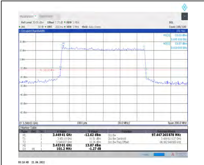
1-N78-3450-3550--30-100-M-6-CP-QPSK-Outer_Full -273@0-Ant1-97.447-101.200-≤100-PASS
