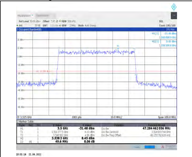
1-N78-3450-3550--30-50-H-9-CP-256QAM-Outer_Full-133@0-Ant1-47.284-49.600-≤50-PASS
