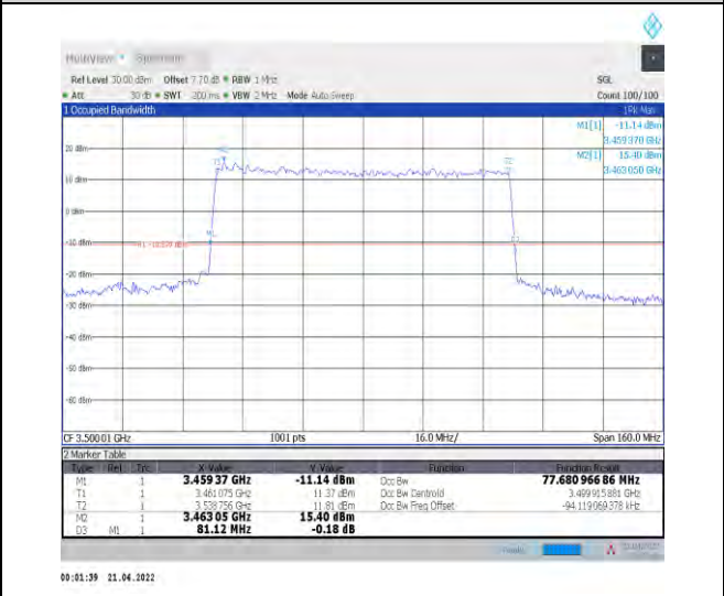
1-N78-3450-3550--30-80-M-7-CP-16QAM-Outer_Full-217@0-Ant1-77.681-81.120-<math>\leq 80</math>-PASS
