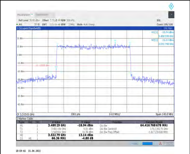
1-N78-3450-3550--30-70-H-1-DFT-QPSK-Outer_Full -180@0-Ant1-64.417-66.360-≤70-PASS
