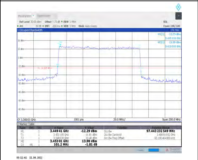
1-N78-3450-3550--30-100-L-6-CP-QPSK-Outer_F ull-273@0-Ant1-97.443-101.200-≤100-PASS
