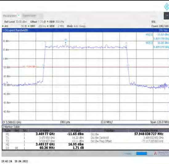
1-N78-3450-3550--30-60-M-2-DFT-PI2BPSK-Outer_F Full-162@0-Ant1-57.948-60.360-≤60-PASS
