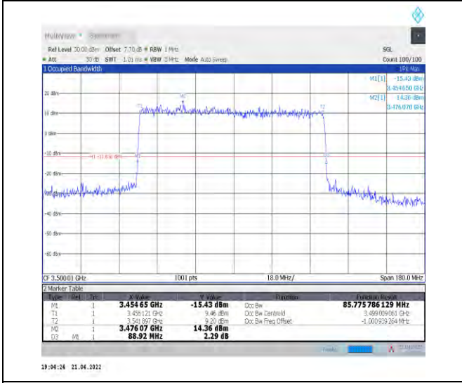
1-N78-3450-3550--30-90-M-3-DFT-16QAM-Outer_Full -240@0-Ant1-85.776-88.920-≤90-PASS
