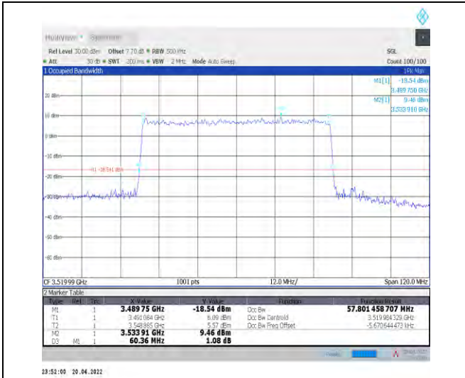
1-N78-3450-3550--30-60-H-9-CP-256QAM-Outer_Fu II-162@0-Ant1-57.801-60.360-≤60-PASS
