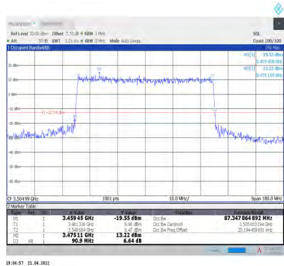
1-N78-3450-3550--30-90-H-7-CP-16QAM-Outer_Full-245@0-Ant1-87.348-90.900-≤90-PASS
