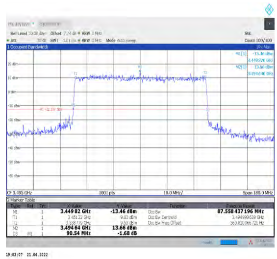
1-N78-3450-3550--30-90-L-7-CP-16QAM-Outer_Full -245@0-Ant1-87.558-90.540-<=90-PASS
