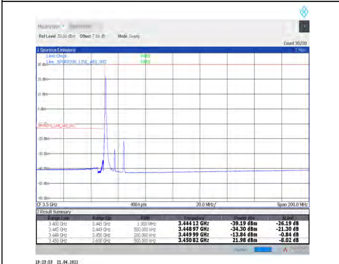
1-N78-3450-3550--30-15-L-4-CP-QPSK-Edge_1RB_L_eff-1@0-Ant1-PASS-see graph
