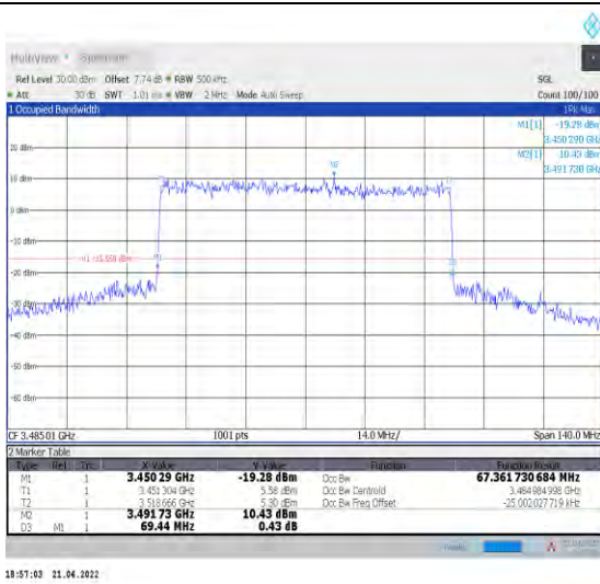
1-N78-3450-3550--30-70-L-8-CP-64QAM-Outer_Full -189@0-Ant1-67.362-69.440-≤70-PASS
