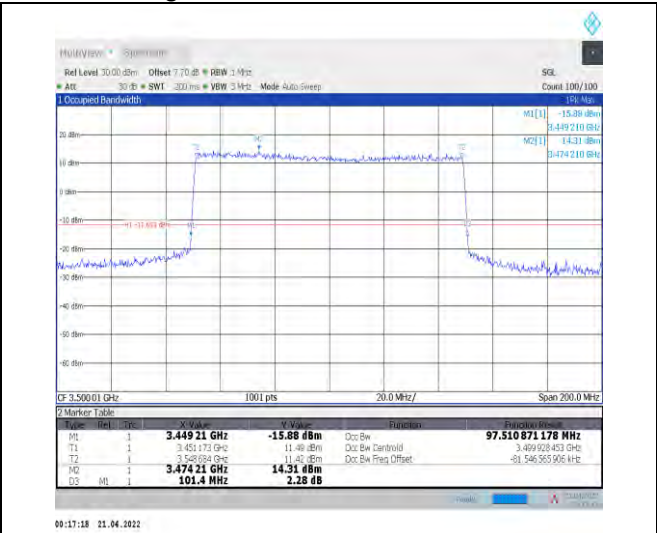
1-N78-3450-3550--30-100-M-7-CP-16QAM-Outer_Full ull-273@0-Ant1-97.511-101.400-≤100-PASS
