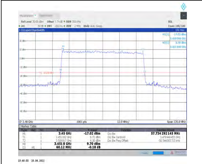
1-N78-3450-3550--30-60-L-9-CP-256QAM-Outer_Fu II-162@0-Ant1-57.734-60.120-≤60-PASS
