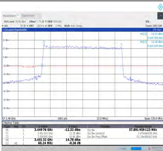
1-N78-3450-3550--30-60-L-3-DFT-16QAM-Outer_Full I-162@0-Ant1-57.892-60.240-≤60-PASS
