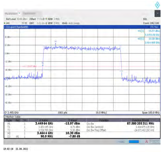
1-N78-3450-3550--30-90-L-9-CP-256QAM-Outer_Fu II-245@0-Ant1-87.58-90.900-<=90-PASS
