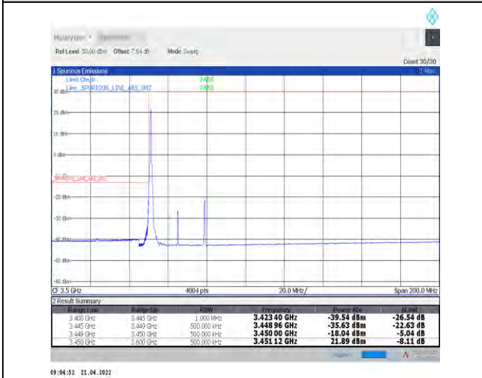
1-N78-3450-3550--30-30-L-4-CP-QPSK-Edge_1RB_L_eff-1@0-Ant1-PASS-see graph
