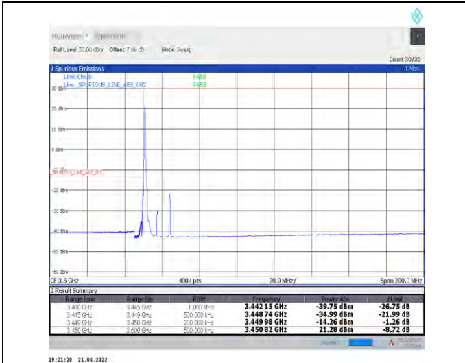
1-N78-3450-3550--30-15-L-1-DFT-PI2BPSK-Edge_1R_B_Left-1@0-Ant1-PASS-see graph
