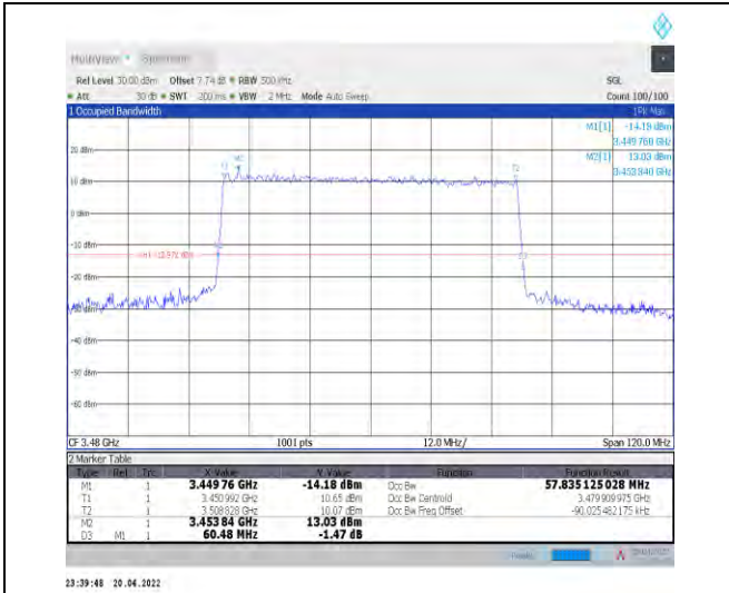
1-N78-3450-3550--30-60-L-7-CP-16QAM-Outer_Full -162@0-Ant1-57.835-60.480-≤60-PASS
