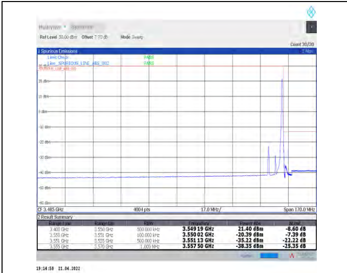
1-N78-3450-3550--30-10-H-2-DFT-PI2BPSK-Edge_1R_B_Right-1@23-Ant1-PASS-see graph
