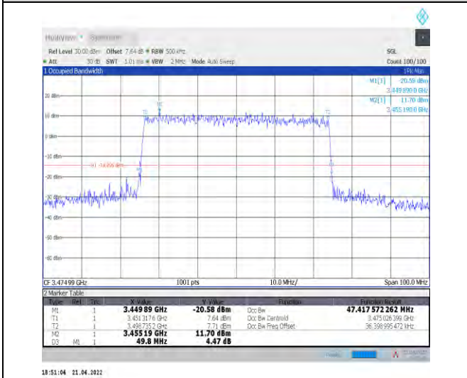
1-N78-3450-3550--30-50-L-8-CP-64QAM-Outer_Full -133@0-Ant1-47.418-49.800-≤50-PASS
