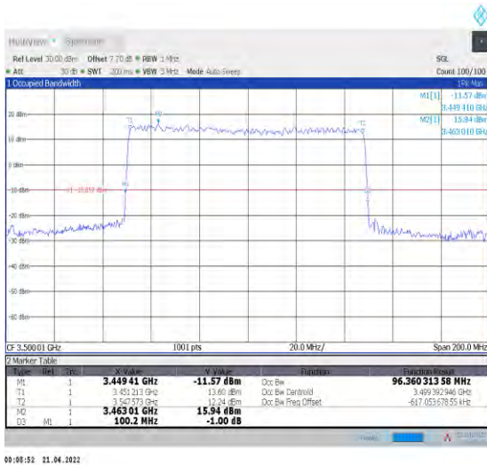
1-N78-3450-3550--30-100-L-1-DFT-QPSK-Outer_Full I-270@0-Ant1-96.36-100.200-≤100-PASS
