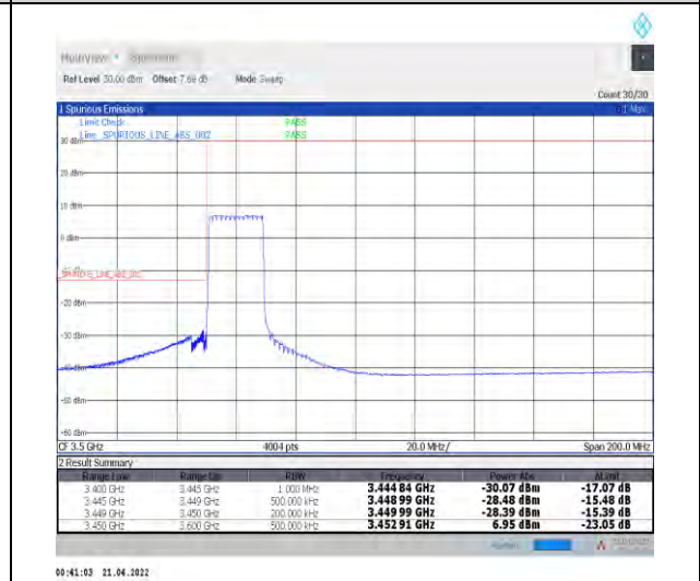
1-N78-3450-3550--30-20-L-6-CP-QPSK-Outer_Ful-I-51@0-Ant1-PASS-see graph
