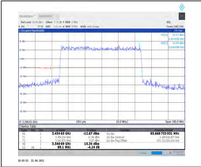
1-N78-3450-3550--30-90-M-1-DFT-QPSK-Outer_Full -240@0-Ant1-85.669-89.100-≤90-PASS
