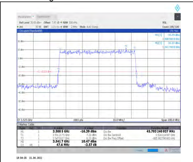
1-N78-3450-3550--30-50-H-5-DFT-256QAM-Outer_F uII-128@0-Ant1-45.793-47.600-≤50-PASS
