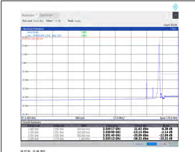
1-N78-3450-3550--30-15-H-2-DFT-PI2BPSK-Edge_1R_B_Right-1@37-Ant1-PASS-see graph
