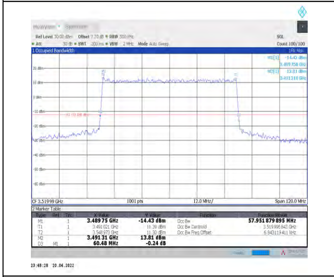
1-N78-3450-3550--30-60-H-3-DFT-16QAM-Outer_Fu ll-162@0-Ant1-57.952-60.480-≤60-PASS
