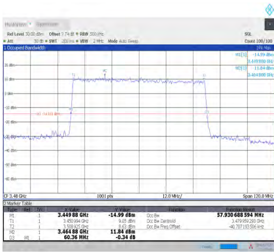
1-N78-3450-3550--30-60-L-5-DFT-256QAM-Outer_Full ull-162@0-Ant1-57.931-60.360-≤60-PASS
