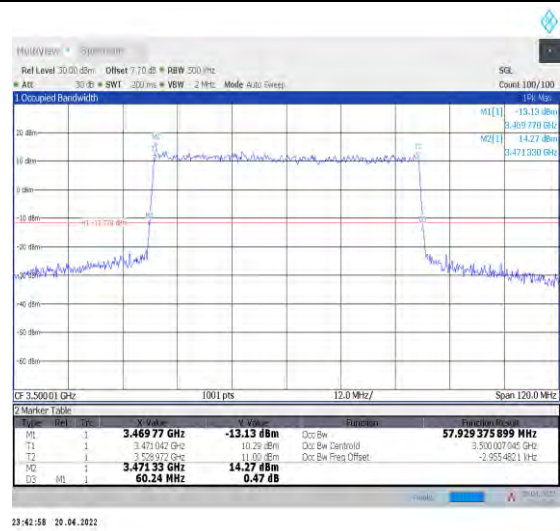
1-N78-3450-3550--30-60-M-3-DFT-16QAM-Outer_F Full-162@0-Ant1-57.929-60.240-≤60-PASS
