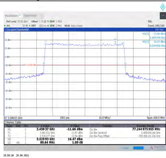
1-N78-3450-3550--30-80-M-1-DFT-QPSK-Outer_Full -216@0-Ant1-77.245-80.640-≤80-PASS
