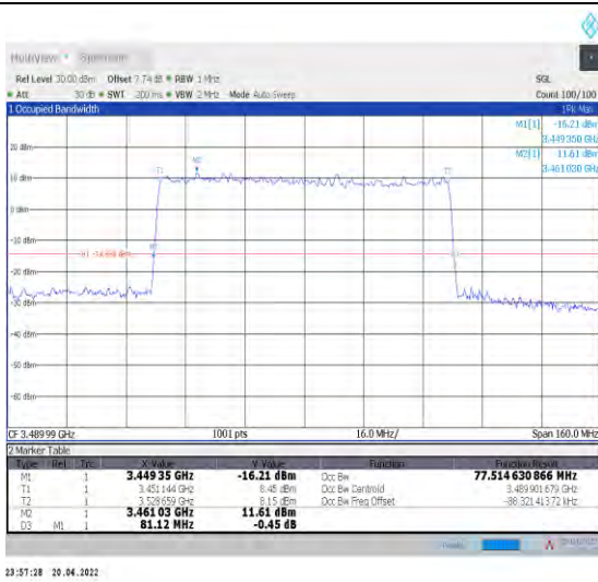
1-N78-3450-3550--30-80-L-9-CP-256QAM-Outer_Fu ll-217@0-Ant1-77.515-81.120-≤80-PASS
