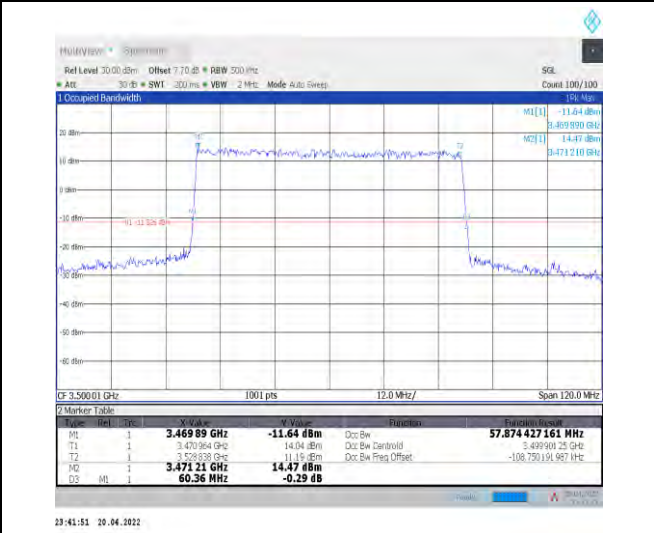
1-N78-3450-3550--30-60-M-1-DFT-QPSK-Outer_Full -162@0-Ant1-57.874-60.360-≤60-PASS
