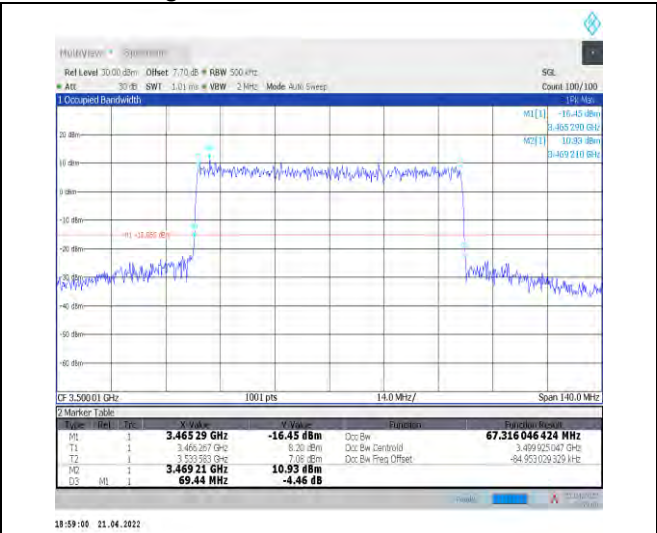
1-N78-3450-3550--30-70-M-8-CP-64QAM-Outer_Ful I-189@0-Ant1-67.316-69.440-≤70-PASS
