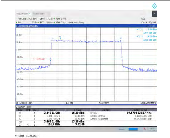
1-N78-3450-3550--30-100-L-7-CP-16QAM-Outer_Fu II-273@0-Ant1-97.58-101.400-≤100-PASS
