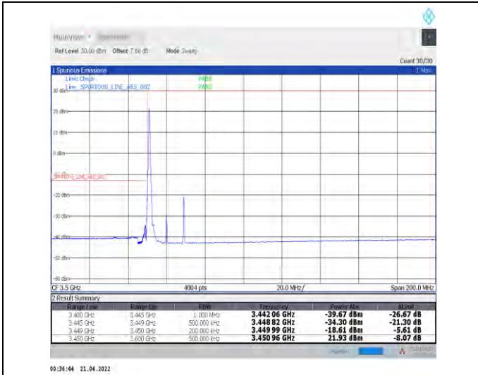
1-N78-3450-3550--30-20-L-1-DFT-PI2BPSK-Edge_1R_B_Left-1@0-Ant1-PASS-see graph
