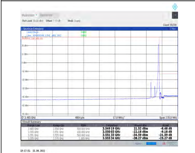
1-N78-3450-3550--30-10-H-5-CP-QPSK-Edge_1RB_R ight-1@23-Ant1-PASS-see graph
