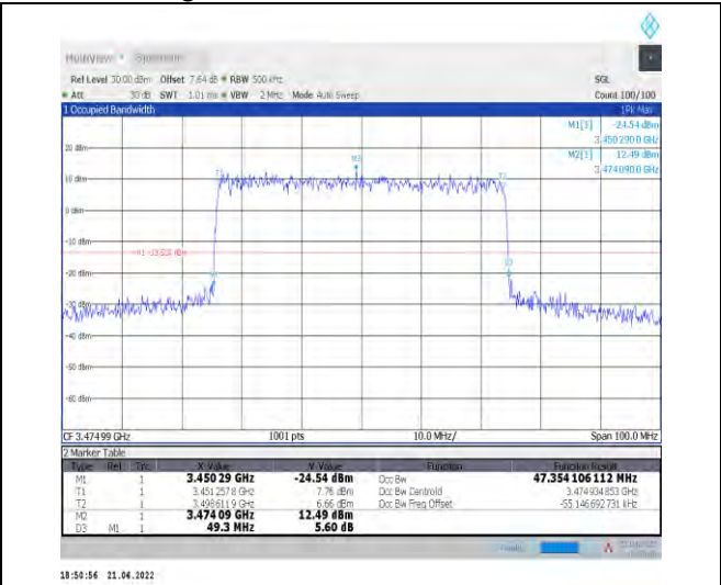
1-N78-3450-3550--30-50-L-7-CP-16QAM-Outer_Full -133@0-Ant1-47.354-49.300-≤50-PASS
