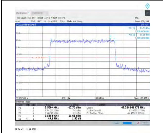
1-N78-3450-3550--30-50-H-6-CP-QPSK-Outer_Full-133@0-Ant1-47.325-49.100-≤50-PASS
