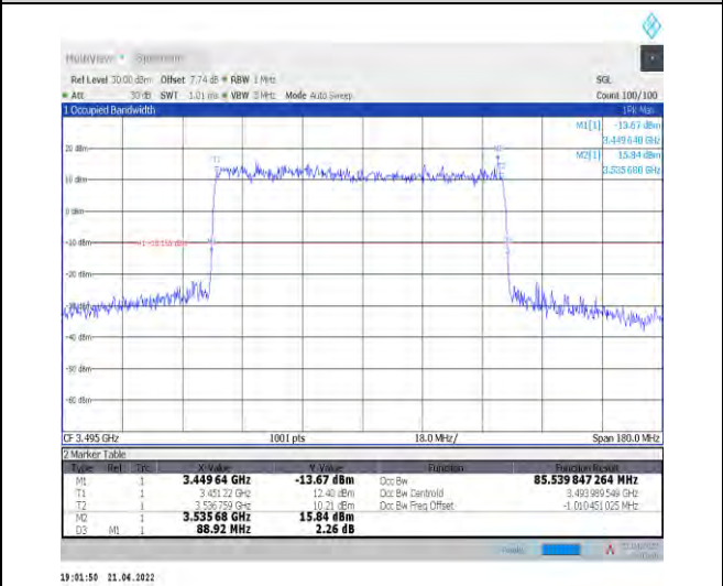
1-N78-3450-3550--30-90-L-1-DFT-QPSK-Outer_Full- 240@0-Ant1-85.54-88.920-≤90-PASS
