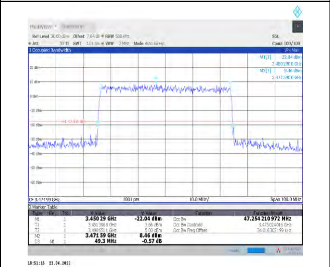
1-N78-3450-3550--30-50-L-9-CP-256QAM-Outer_Fu ll-133@0-Ant1-47.254-49.300-≤50-PASS
