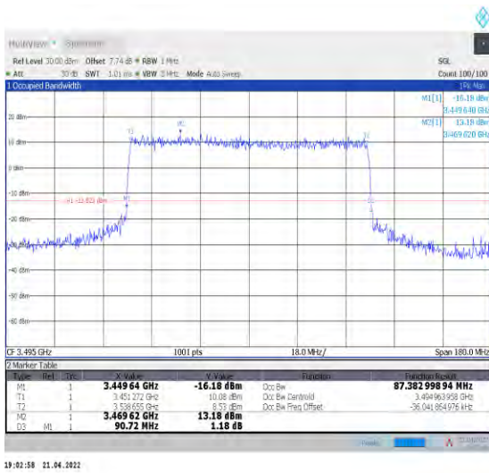
1-N78-3450-3550--30-90-L-6-CP-QPSK-Outer_Full-2 45@0-Ant1-87.383-90.720-<=90-PASS
