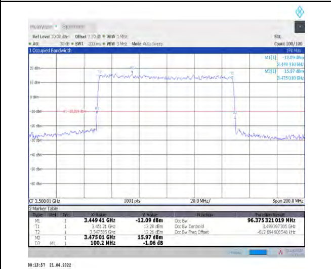
1-N78-3450-3550--30-100-M-1-DFT-QPSK-Outer_F ull-270@0-Ant1-96.375-100.200-≤100-PASS
