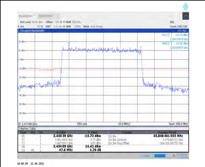
1-N78-3450-3550--30-50-L-1-DFT-QPSK-Outer_Full- 128@0-Ant1-45.848-47.600-≤50-PASS
